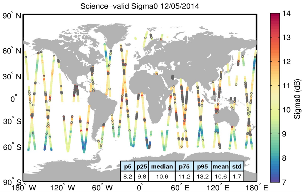
Figure 27. Geographical distribution of science-valid sigma0 data over oceans and lakes for 12/05/2014. The statistical values shown in the table refer to the sigma0 in dB and are calculated over all measurements shown in the figure. Gray circles denote records that have been rejected based on the editing criteria described in Table 4.
