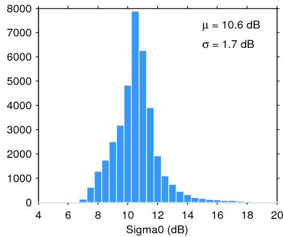
Figure 28. Histogram of science-valid sigma0 over oceans and lakes for 12/05/2014. The mean ( \mu ) and standard deviation ( \sigma ) are also shown. Note that values outside [4 20] dB are excluded from the histogram for the sake of readability but not from the computation of \mu and \sigma .
