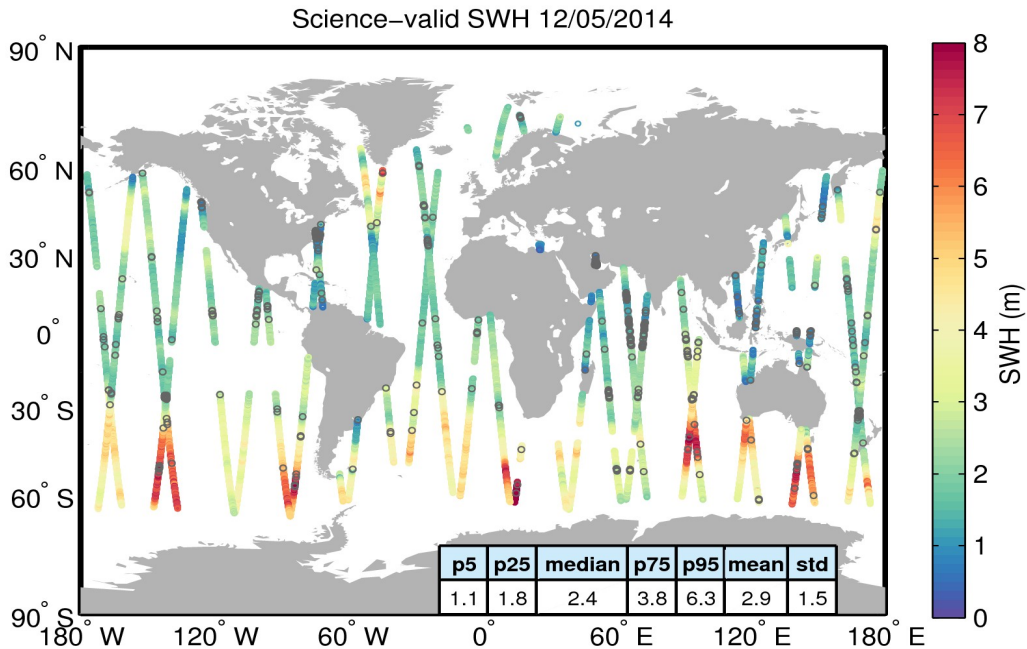
Figure 19. Geographical distribution of science-valid SWH data over oceans and lakes for 12/05/2014. The statistical values shown in the table refer to the SWH in m and are calculated over all measurements shown in the figure. Gray circles denote records that have been rejected based on the editing criteria described in Table 3.
