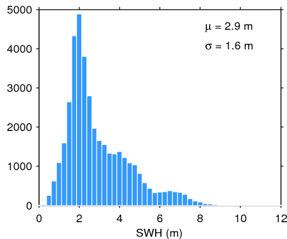
Figure 17. Histogram of flag-valid SWH over oceans and lakes for 12/05/2014. The mean ( \mu ) and standard deviation ( \sigma ) are also shown. Note that values larger than 12 m are excluded from the histogram for the sake of readability but not from the computation of \mu and \sigma .
