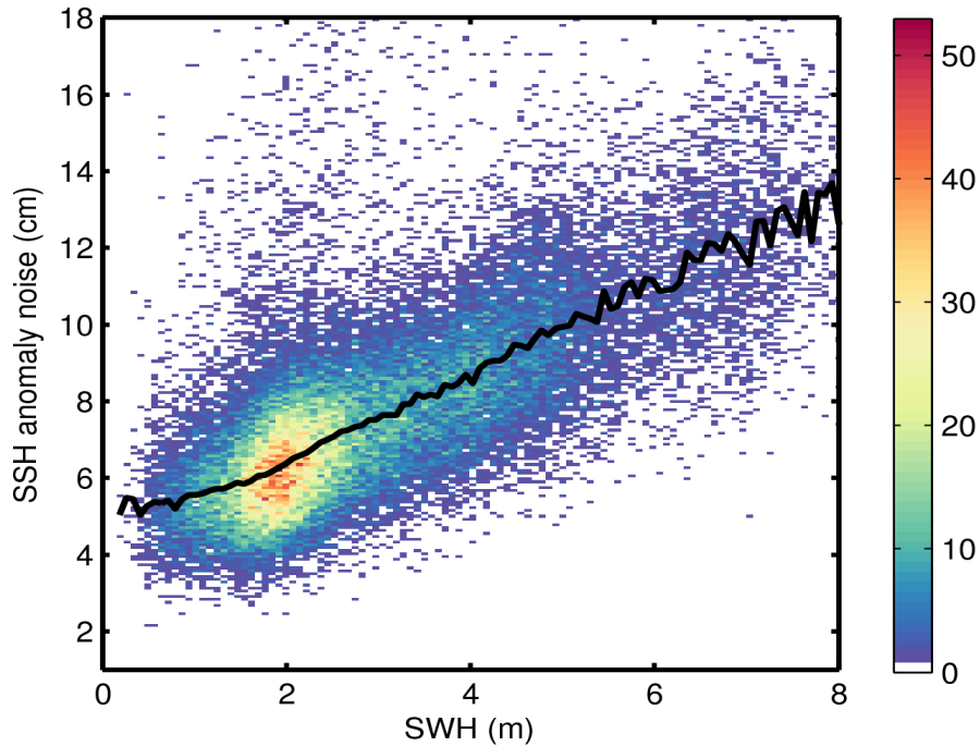
Figure 9. 2D histogram showing flag-valid SSH anomaly noise as a function of SWH for 12/05/2014. The black line denotes the median SSH anomaly as a function of SWH.
