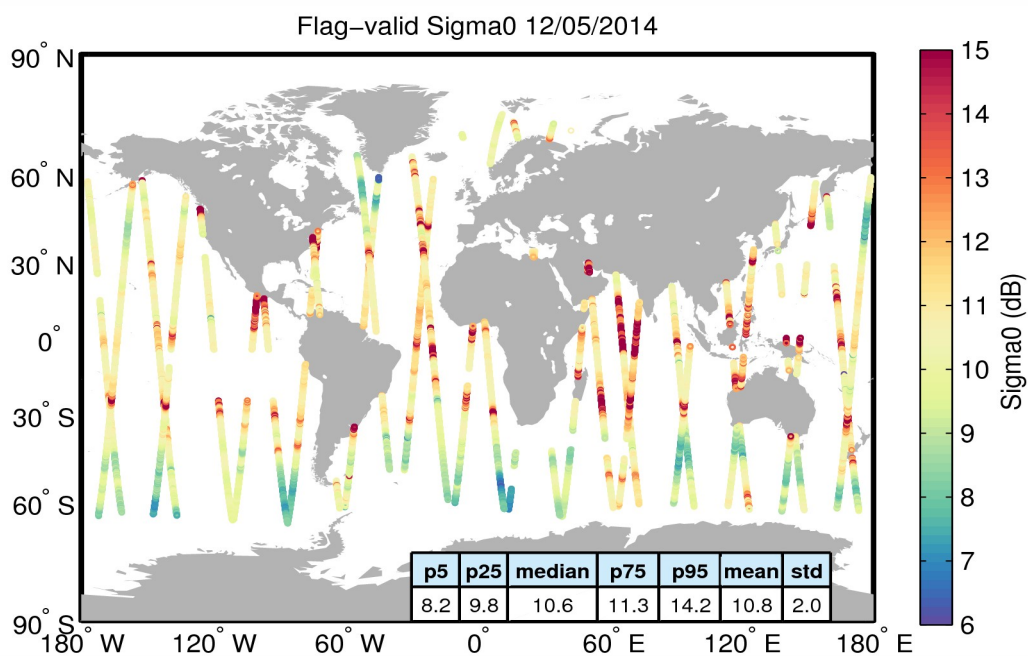
Figure 23. Geographical distribution of flag-valid sigma0 data over oceans and lakes for 12/05/2014. The statistical values shown in the table refer to the sigma0 in dB and are calculated over all measurements shown in the figure.
