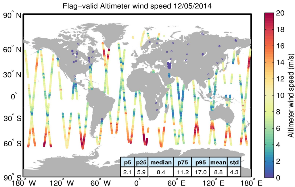
Figure 31. Geographical distribution of flag-valid wind data over oceans and lakes for 12/05/2014. The statistical values shown in the table refer to the wind in m/s and are calculated over all measurements shown in the figure.
