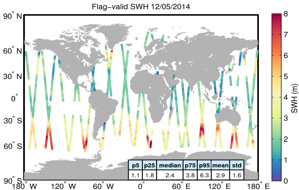
Figure 15. Geographical distribution of flag-valid SWH data over oceans and lakes for 12/05/2014. The statistical values shown in the table refer to the SWH in m and are calculated over all measurements shown in the figure.
