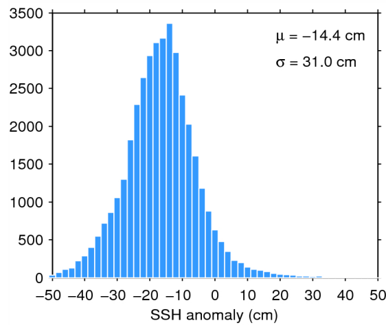
Figure 7. Histogram of flag-valid SSH anomaly over oceans and lakes for 12/05/2014. The mean ( \mu ) and standard deviation ( \sigma ) are also shown. Note that values outside [-50\ 50] cm are excluded from the histogram for the sake of readability but not from the computation of \mu and \sigma .
