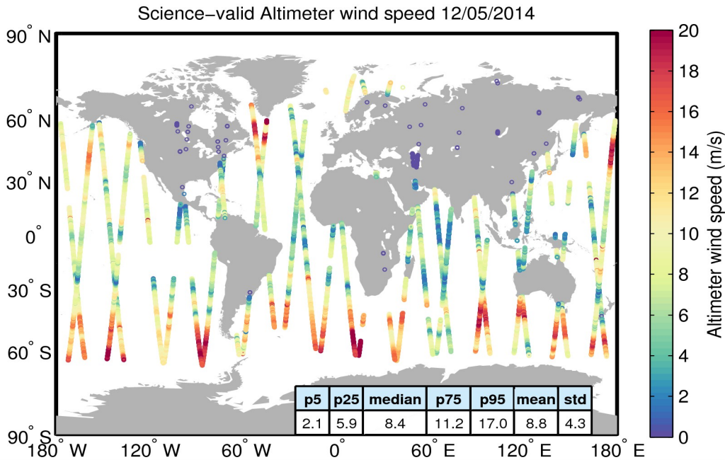
Figure 34. Geographical distribution of science-valid wind data over oceans and lakes for 12/05/2014. The statistical values shown in the table refer to the wind in m/s and are calculated over all measurements shown in the figure. Gray circles denote records that have been rejected based on the editing criteria described in Table 5.
