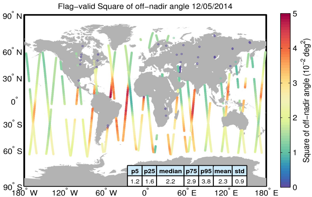
Figure 37. Geographical distribution of flag-valid mispointing data over oceans and lakes for 12/05/2014. The statistical values shown in the table refer to the mispointing in 10^{-2} \text{deg}^2 and are calculated over all measurements shown in the figure.
