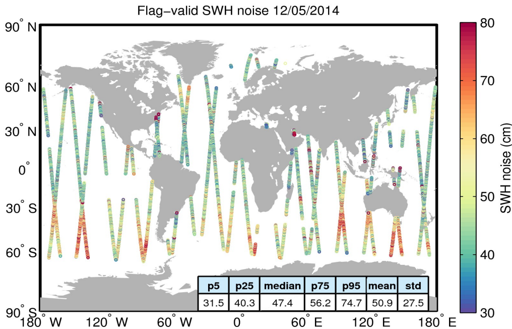
Figure 18. Geographical distribution of flag-valid 20-Hz SWH measurement noise over oceans and lakes for 12/05/2014. The statistical values shown in the figure refer to the SWH noise and are calculated over all measurements shown in the figure.
