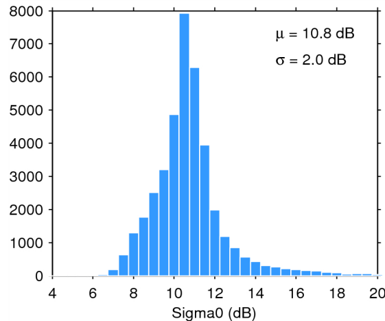
Figure 25. Histogram of flag-valid sigma0 over oceans and lakes for 12/05/2014. The mean ( \mu ) and standard deviation ( \sigma ) are also shown. Note that values outside [4 20] dB are excluded from the histogram for the sake of readability but not from the computation of \mu and \sigma .
