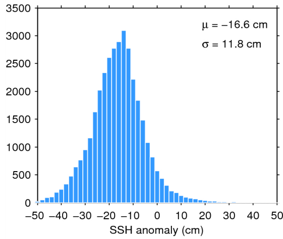
Figure 11. Histogram of science-valid SSH anomaly over oceans and lakes for 12/05/2014. The mean ( \mu ) and standard deviation ( \sigma ) are also shown. Note that values outside [-50 50] cm are excluded from the histogram for the sake of readability but not from the computation of \mu and \sigma .
