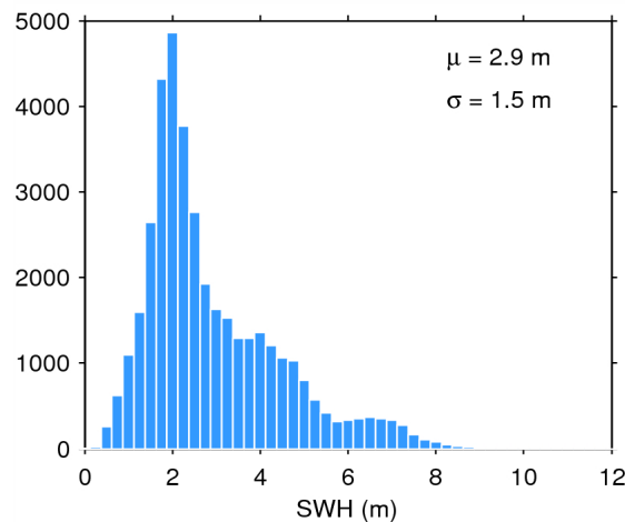
Figure 20. Histogram of science-valid SWH over oceans and lakes for 12/05/2014. The mean ( \mu ) and standard deviation ( \sigma ) are also shown. Note that values larger than 12 m are excluded from the histogram for the sake of readability but not from the computation of \mu and \sigma .
