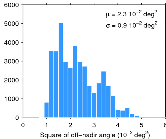
Figure 39. Histogram of flag-valid mispointing over oceans and lakes for 12/05/2014. The mean ( \mu ) and standard deviation ( \sigma ) are also shown. Note that values than 6 \cdot 10^{-2} \text{ deg}^2 are excluded from the histogram for the sake of readability but not from the computation of \mu and \sigma .
