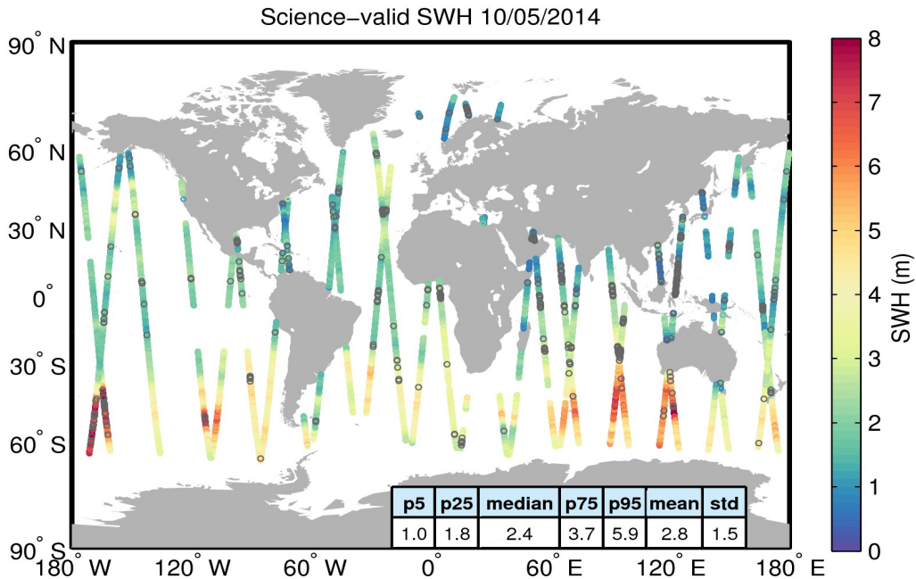
Figure 19. Geographical distribution of science-valid SWH data over oceans and lakes for 10/05/2014. The statistical values shown in the table refer to the SWH in m and are calculated over all measurements shown in the figure. Gray circles denote records that have been rejected based on the editing criteria described in Table 3.
