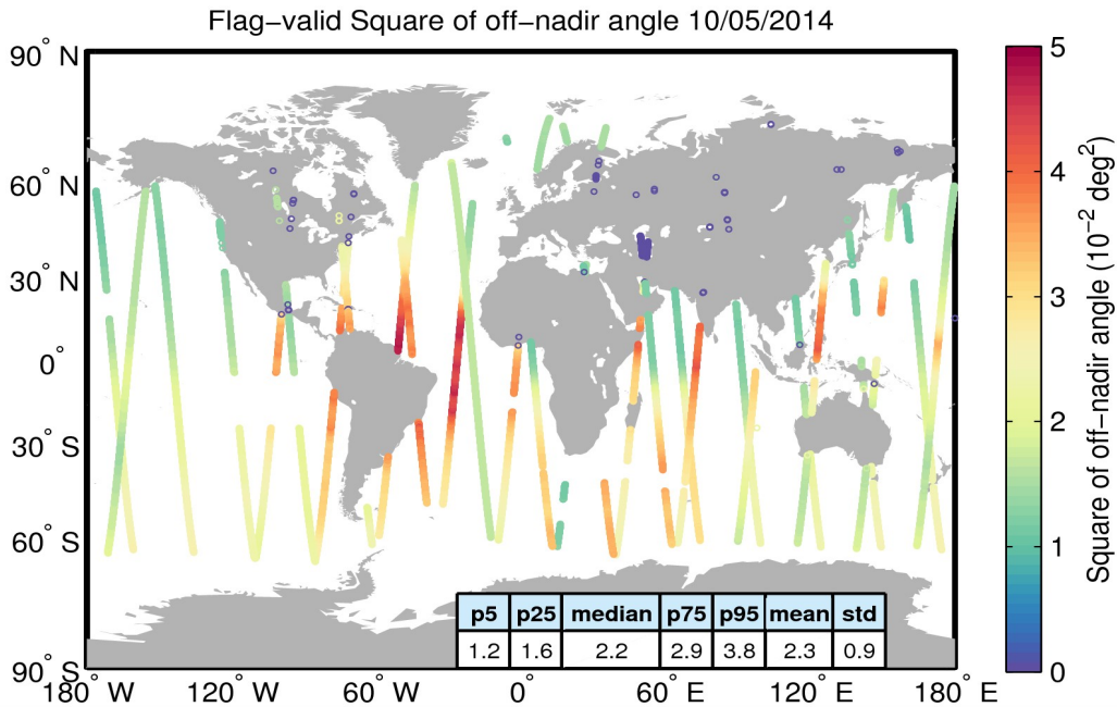
Figure 37. Geographical distribution of flag-valid mispointing data over oceans and lakes for 10/05/2014. The statistical values shown in the table refer to the mispointing in 10^{-2} deg 2 and are calculated over all measurements shown in the figure.
