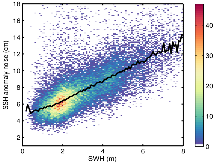
Figure 9. 2D histogram showing flag-valid SSH anomaly noise as a function of SWH for 10/05/2014. The black line denotes the median SSH anomaly as a function of SWH.
