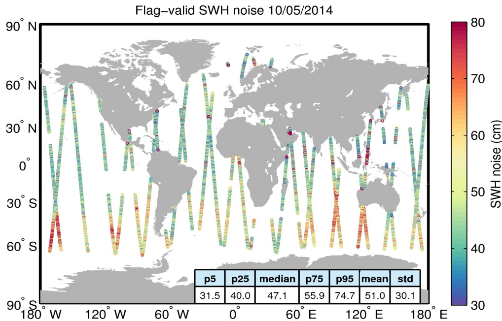
Figure 18. Geographical distribution of flag-valid 20-Hz SWH measurement noise over oceans and lakes for 10/05/2014. The statistical values shown in the figure refer to the SWH noise and are calculated over all measurements shown in the figure.
