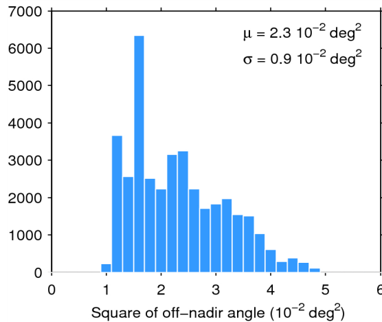
Figure 39. Histogram of flag-valid mispointing over oceans and lakes for 10/05/2014. The mean ( \mu ) and standard deviation ( \sigma ) are also shown. Note that values than 6 \cdot 10^{-2} \text{ deg}^2 are excluded from the histogram for the sake of readability but not from the computation of \mu and \sigma .
