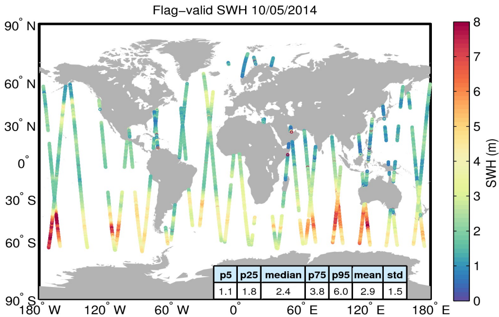
Figure 15. Geographical distribution of flag-valid SWH data over oceans and lakes for 10/05/2014. The statistical values shown in the table refer to the SWH in m and are calculated over all measurements shown in the figure.
