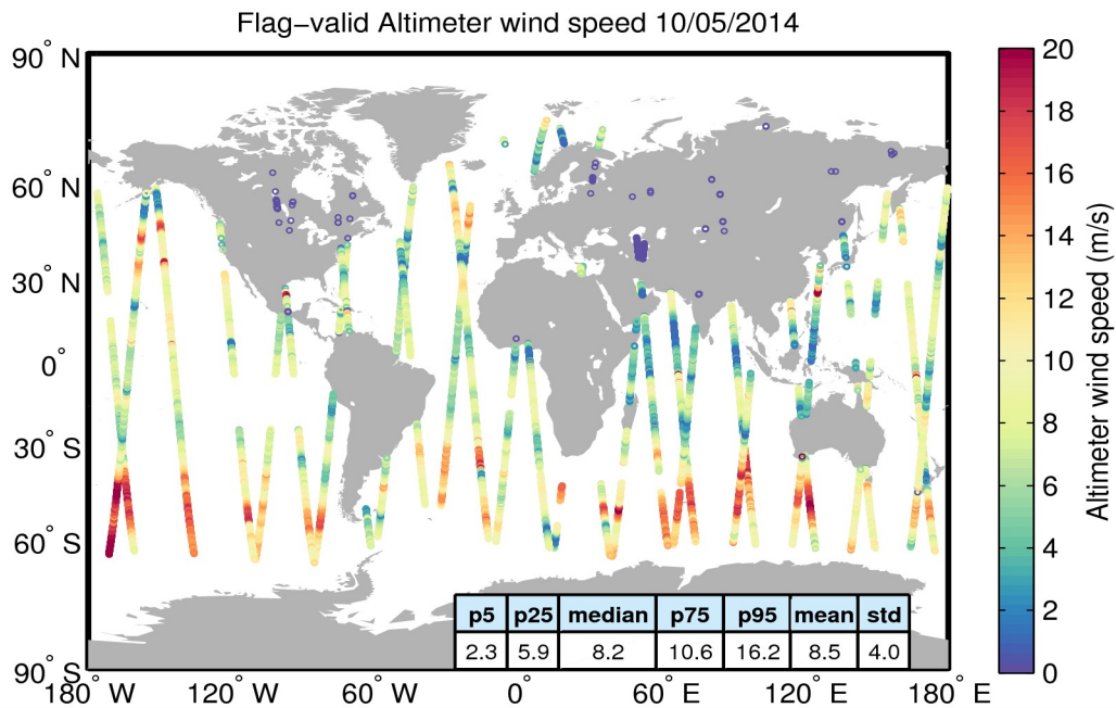
Figure 31. Geographical distribution of flag-valid wind data over oceans and lakes for 10/05/2014. The statistical values shown in the table refer to the wind in m/s and are calculated over all measurements shown in the figure.
