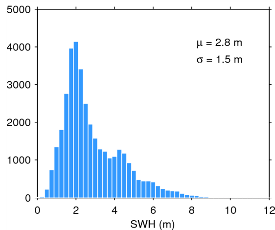
Figure 20. Histogram of science-valid SWH over oceans and lakes for 10/05/2014. The mean ( \mu ) and standard deviation ( \sigma ) are also shown. Note that values larger than 12 m are excluded from the histogram for the sake of readability but not from the computation of \mu and \sigma .
