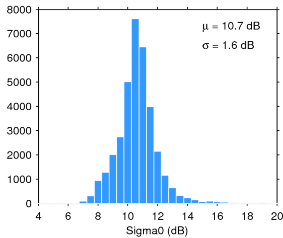
Figure 28. Histogram of science-valid sigma0 over oceans and lakes for 10/05/2014. The mean ( \mu ) and standard deviation ( \sigma ) are also shown. Note that values outside [4 20] dB are excluded from the histogram for the sake of readability but not from the computation of \mu and \sigma .
