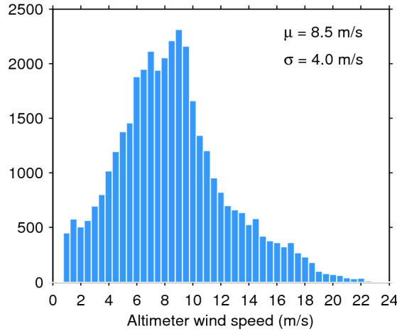
Figure 33. Histogram of flag-valid wind over oceans and lakes for 10/05/2014. The mean ( \mu ) and standard deviation ( \sigma ) are also shown. Note that values larger than 24 m/s are excluded from the histogram for the sake of readability but not from the computation of \mu and \sigma .
