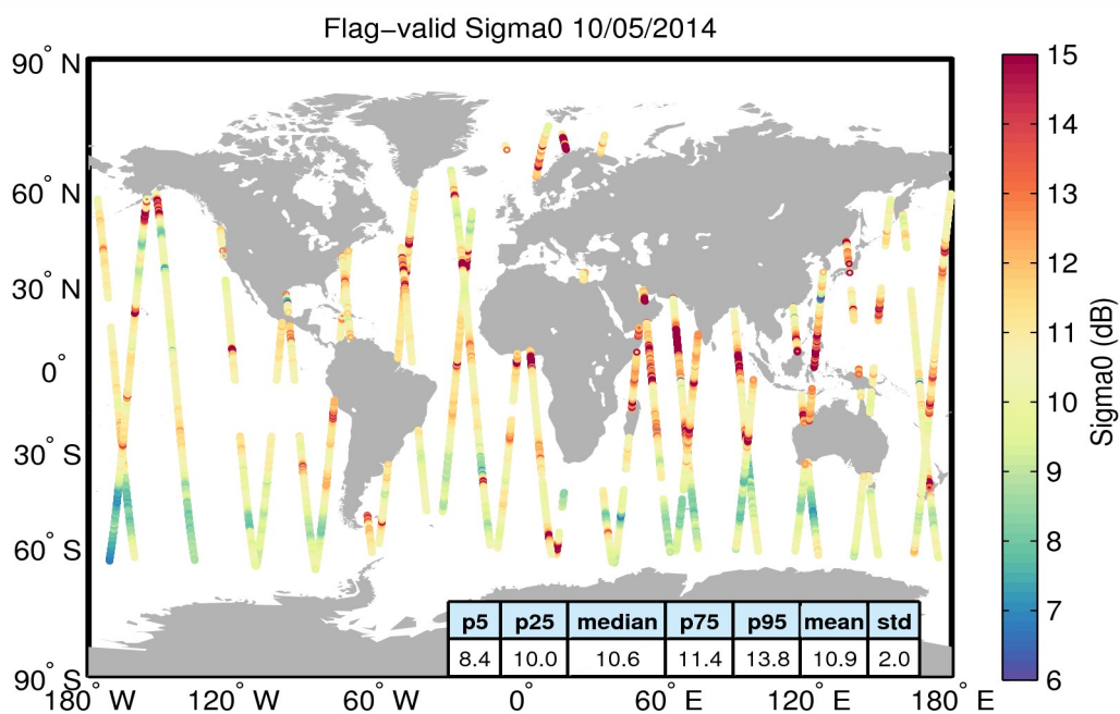
Figure 23. Geographical distribution of flag-valid sigma0 data over oceans and lakes for 10/05/2014. The statistical values shown in the table refer to the sigma0 in dB and are calculated over all measurements shown in the figure.
