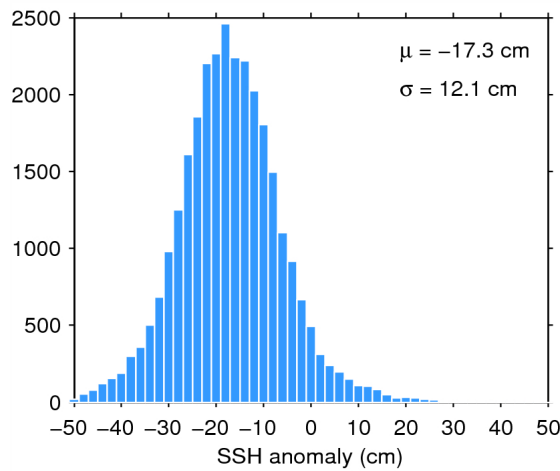
Figure 11. Histogram of science-valid SSH anomaly over oceans and lakes for 10/05/2014. The mean ( \mu ) and standard deviation ( \sigma ) are also shown. Note that values outside [-50 50] cm are excluded from the histogram for the sake of readability but not from the computation of \mu and \sigma .
