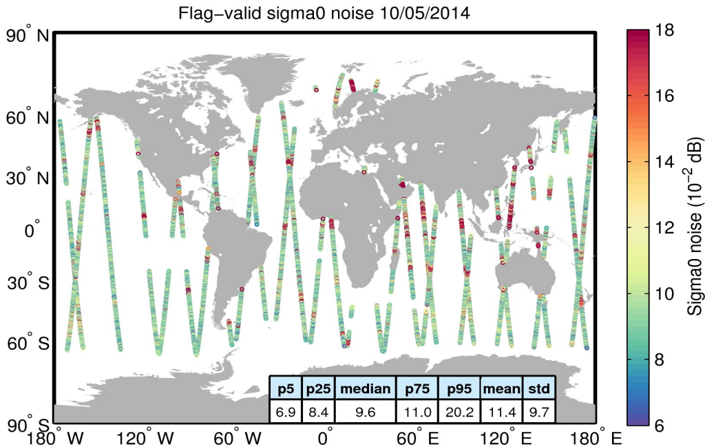
Figure 26. Geographical distribution of flag-valid 20-Hz sigma0 measurement noise over oceans and lakes for 10/05/2014. The statistical values shown in the table refer to the sigma0 noise and are calculated over all measurements shown in the figure.
