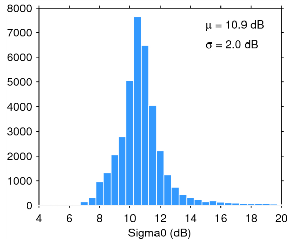
Figure 25. Histogram of flag-valid sigma0 over oceans and lakes for 10/05/2014. The mean ( \mu ) and standard deviation ( \sigma ) are also shown. Note that values outside [4 20] dB are excluded from the histogram for the sake of readability but not from the computation of \mu and \sigma .
