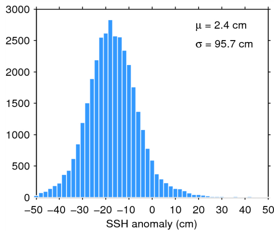
Figure 7. Histogram of flag-valid SSH anomaly over oceans and lakes for 10/05/2014. The mean ( \mu ) and standard deviation ( \sigma ) are also shown. Note that values outside [-50\ 50] cm are excluded from the histogram for the sake of readability but not from the computation of \mu and \sigma .
