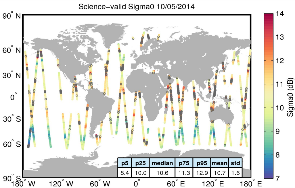
Figure 27. Geographical distribution of science-valid sigma0 data over oceans and lakes for 10/05/2014. The statistical values shown in the table refer to the sigma0 in dB and are calculated over all measurements shown in the figure. Gray circles denote records that have been rejected based on the editing criteria described in Table 4.
