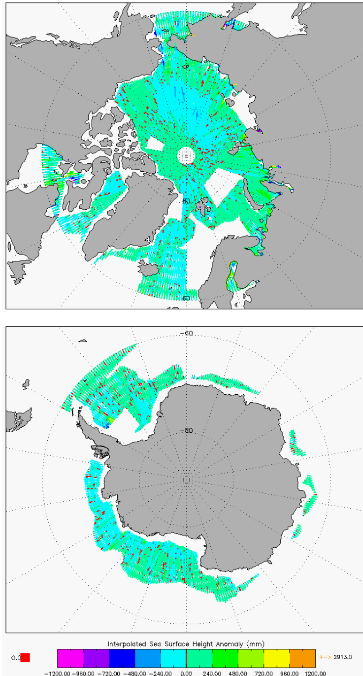
Figure 8 –Polar plots of SSHA for cycle #163.
