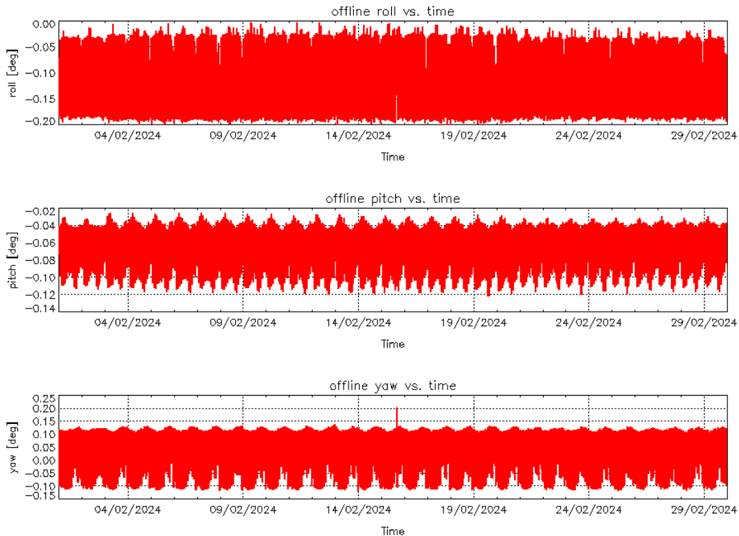
Figure 4 – Roll (top), Pitch (middle) and Yaw (bottom) values for L1B Products during cycle #163.
