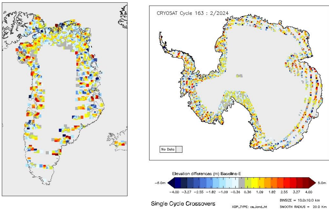
Figure 20 - Greenland and Antarctica maps of SARIn elevation differences for cycle #163.
