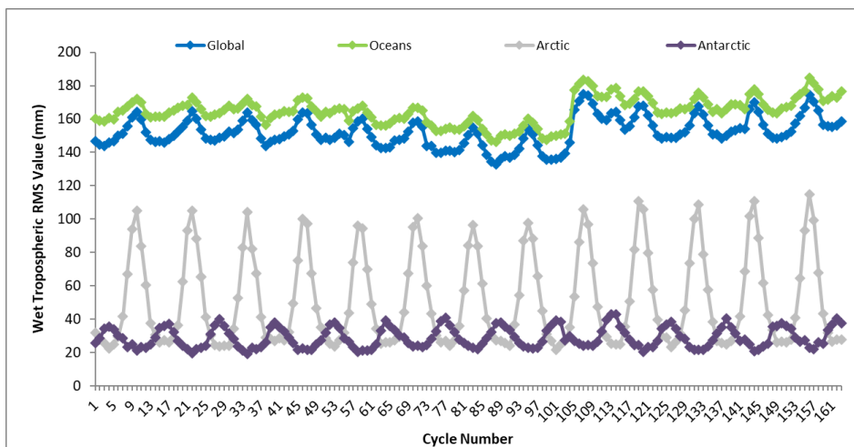
Figure 24 – Wet Tropospheric Correction RMS value trend from beginning of mission
