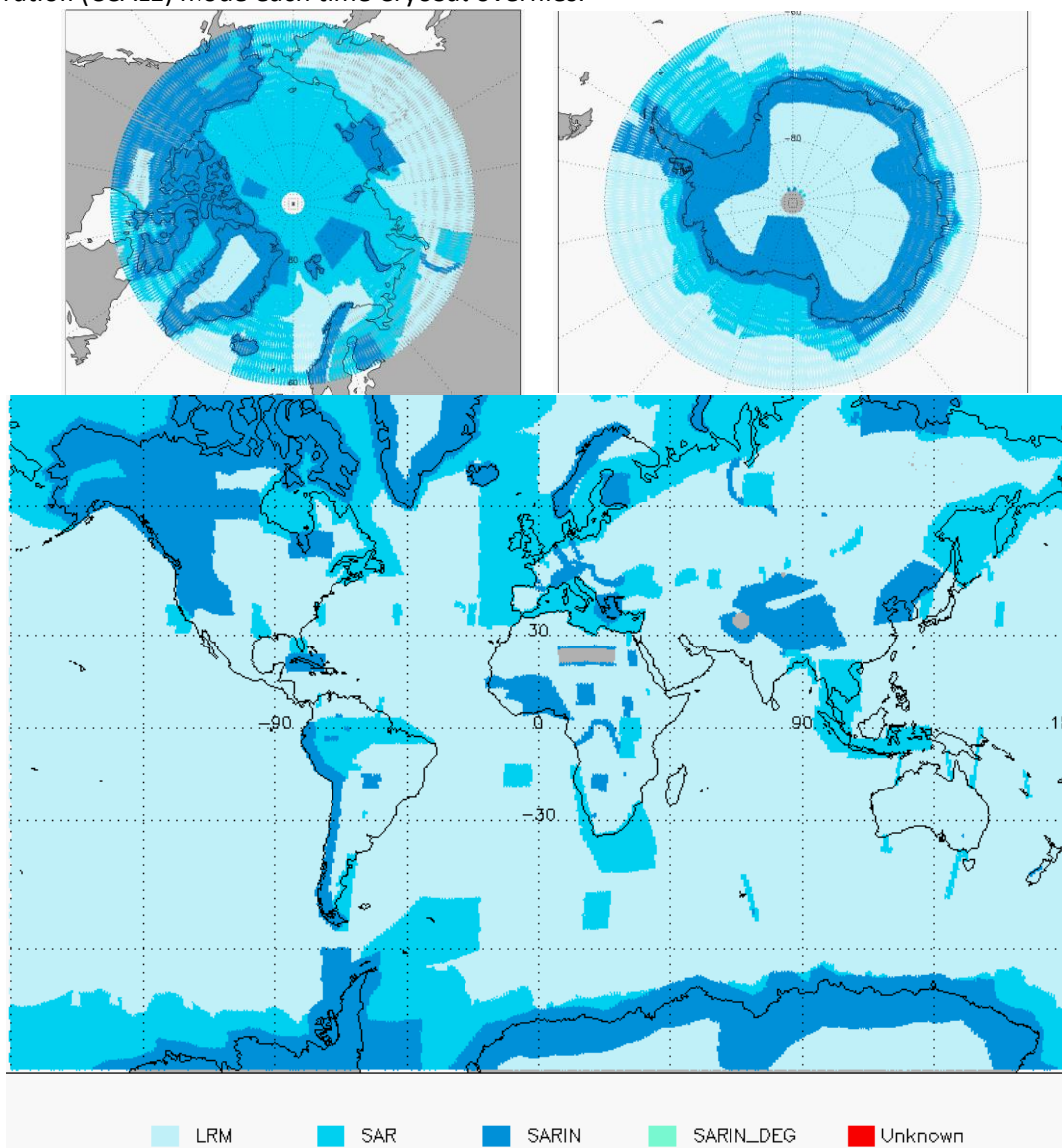
Figure 3 - Global and Polar plots of SIRAL Modes for cycle #163.
