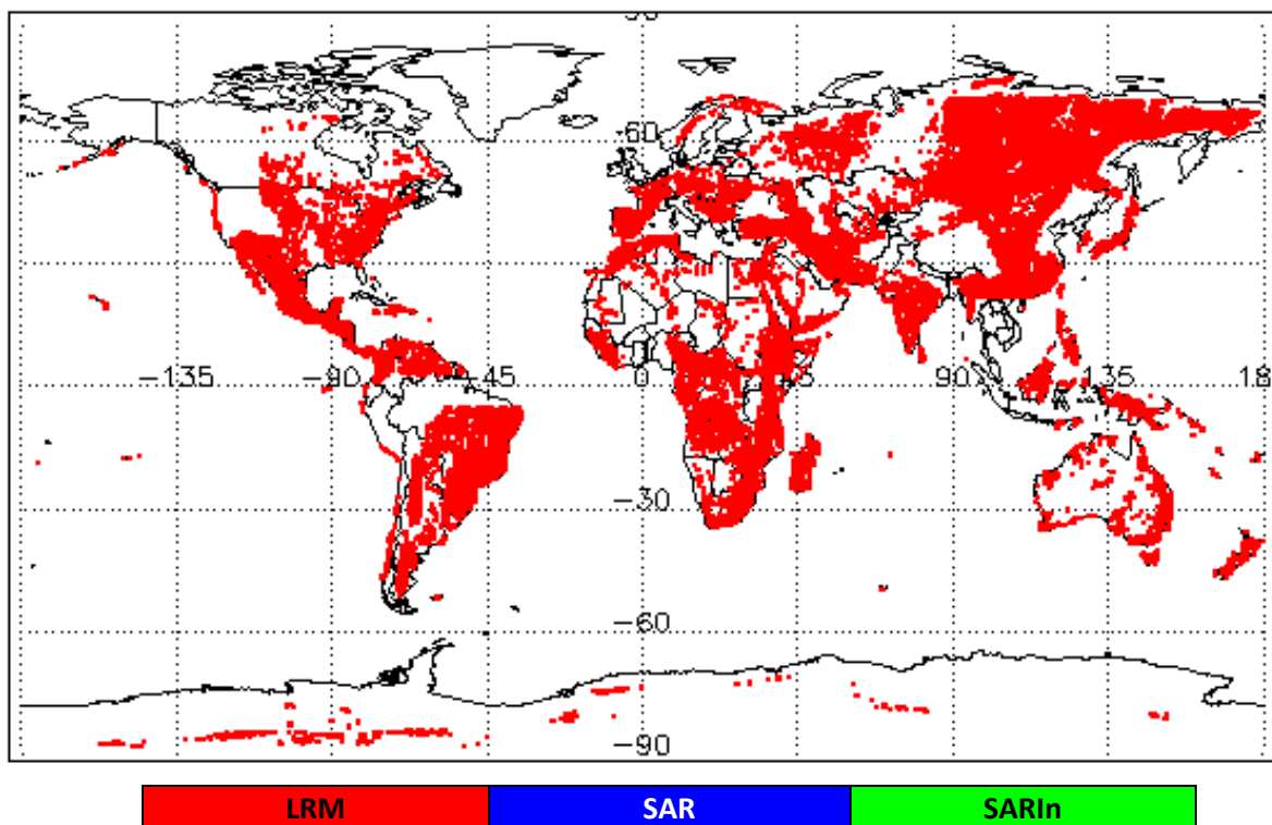
Figure 1 – Global plot showing areas of loss of track in all SIRAL modes L0 data during February 2024
