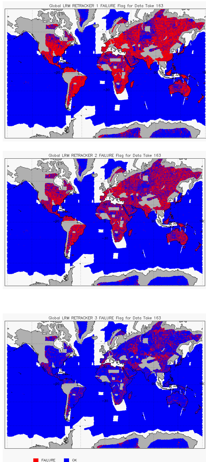
Figure 14 – Global plots showing Retracker Failure Flags for LRM mode for cycle #163: LRM CFI (top), LRM LIRT (middle), LRM OCOG (bottom)
