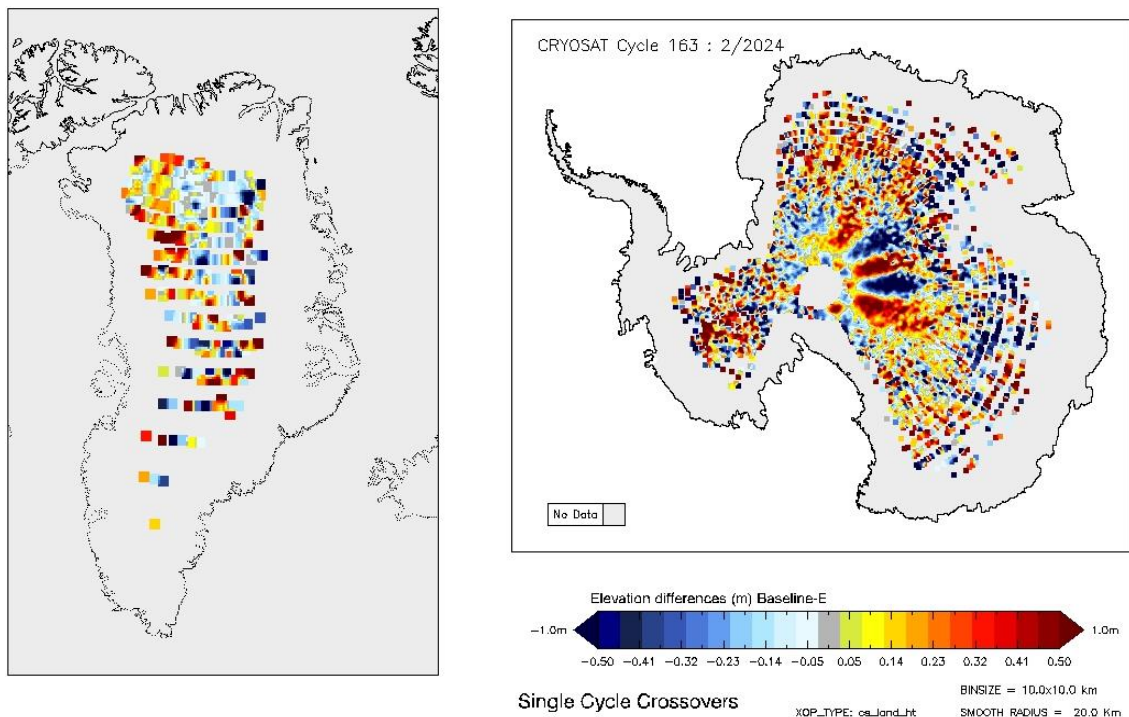
Figure 19 - Greenland and Antarctica maps of LRM elevation differences for cycle #163.
