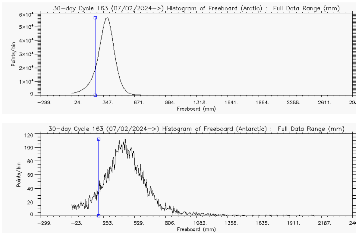
Figure 5 – Histogram of Freeboard for Arctic (above) and Antarctic (below) for cycle #163
