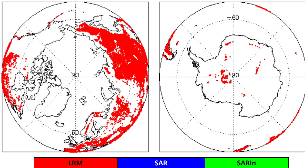
Figure 2 - Polar plots showing areas of loss of track in all SIRAL modes L0 data during February 2024.
