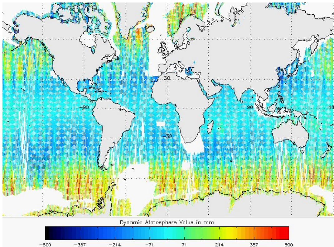
Figure 27 - Global plot of Dynamic Atmospheric Correction for cycle #162
