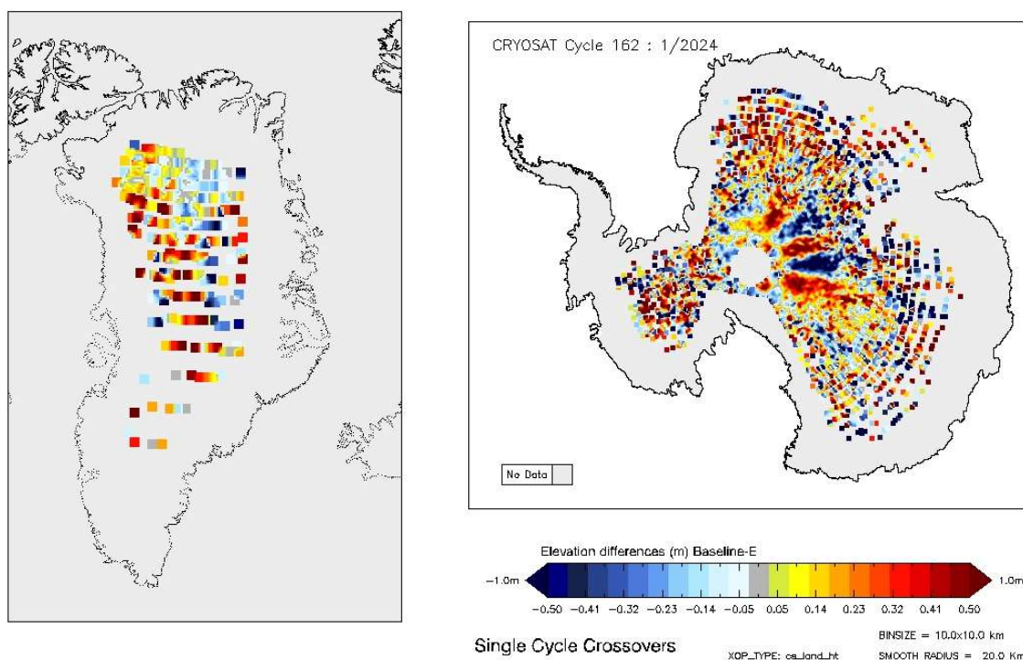
Figure 19 - Greenland and Antarctica maps of LRM elevation differences for cycle #162.
