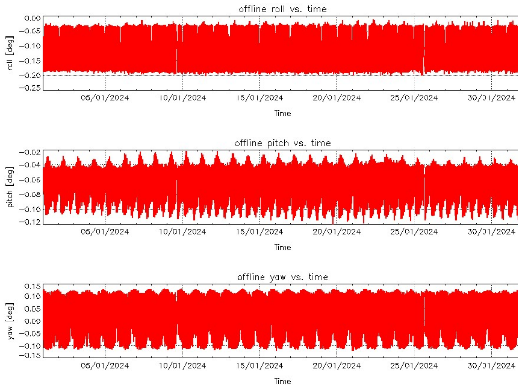
Figure 4 – Roll (top), Pitch (middle) and Yaw (bottom) values for L1B Products during cycle #162.
