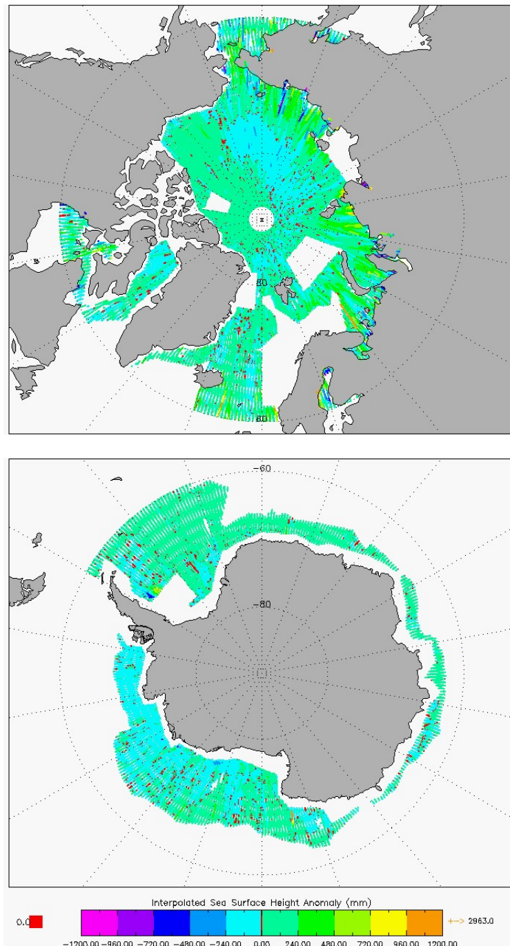
Figure 8 –Polar plots of SSHA for cycle #162.
