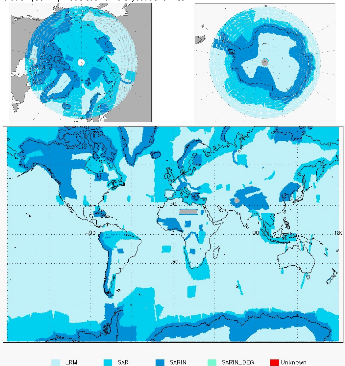
Figure 3 - Global and Polar plots of SIRAL Modes for cycle #162.
