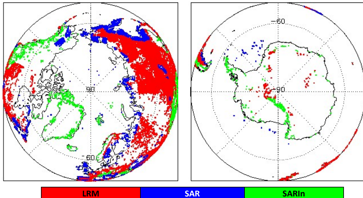
Figure 2 - Polar plots showing areas of loss of track in all SIRAL modes L0 data during January 2024.
