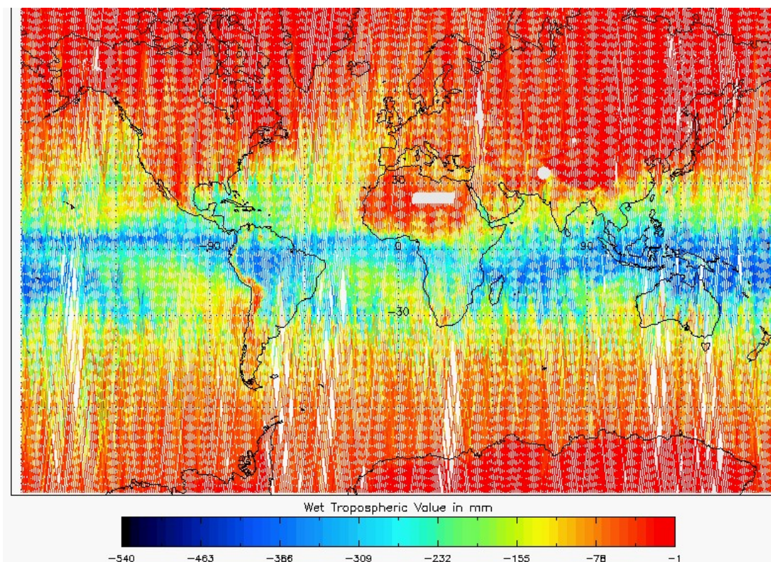
Figure 23 - Global plot of Wet Tropospheric Correction for cycle #162
