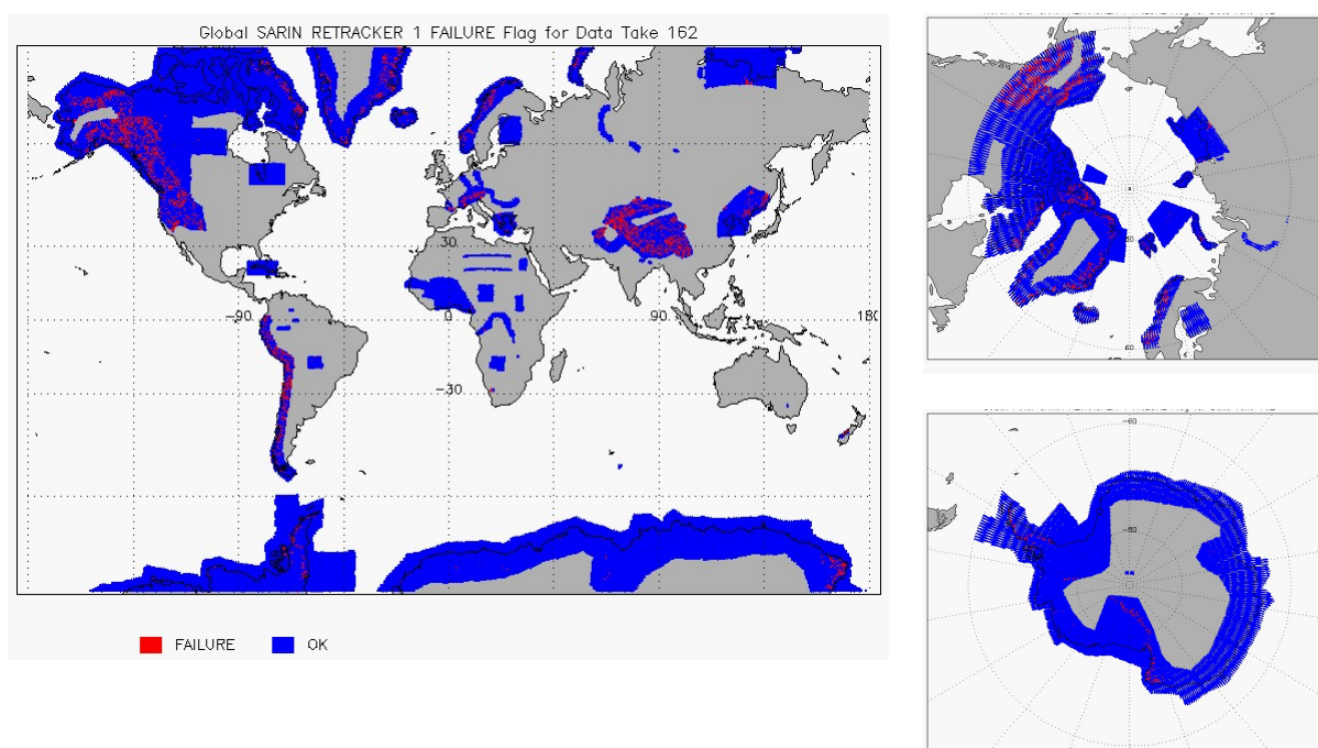
Figure 16 – Global plots showing Retracker Failure Flags for SARIn mode for cycle #162
