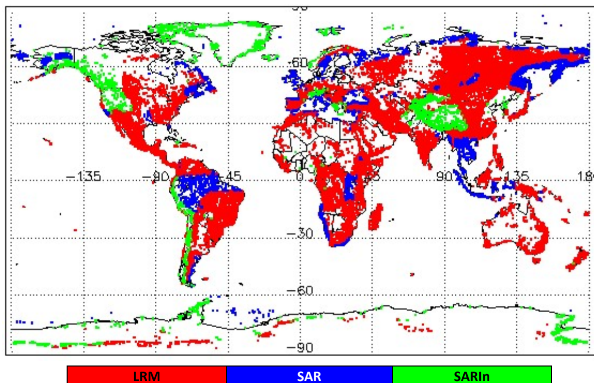
Figure 1 – Global plot showing areas of loss of track in all SIRAL modes L0 data during January 2024
