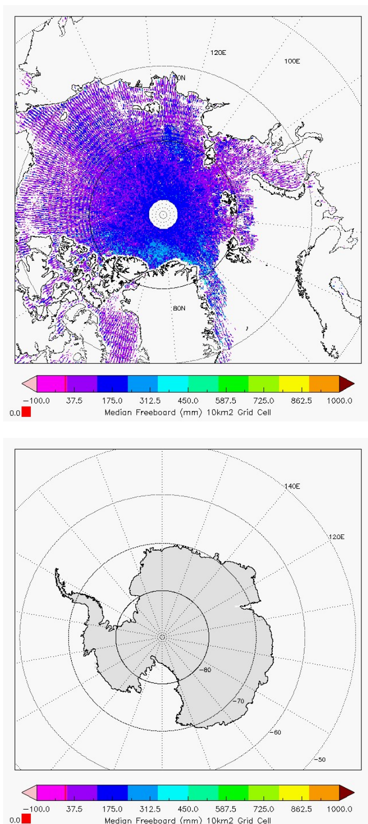
Figure 6 - Polar plots of 10km Gridded Freeboard values from L2 SAR products in cycle #162.
