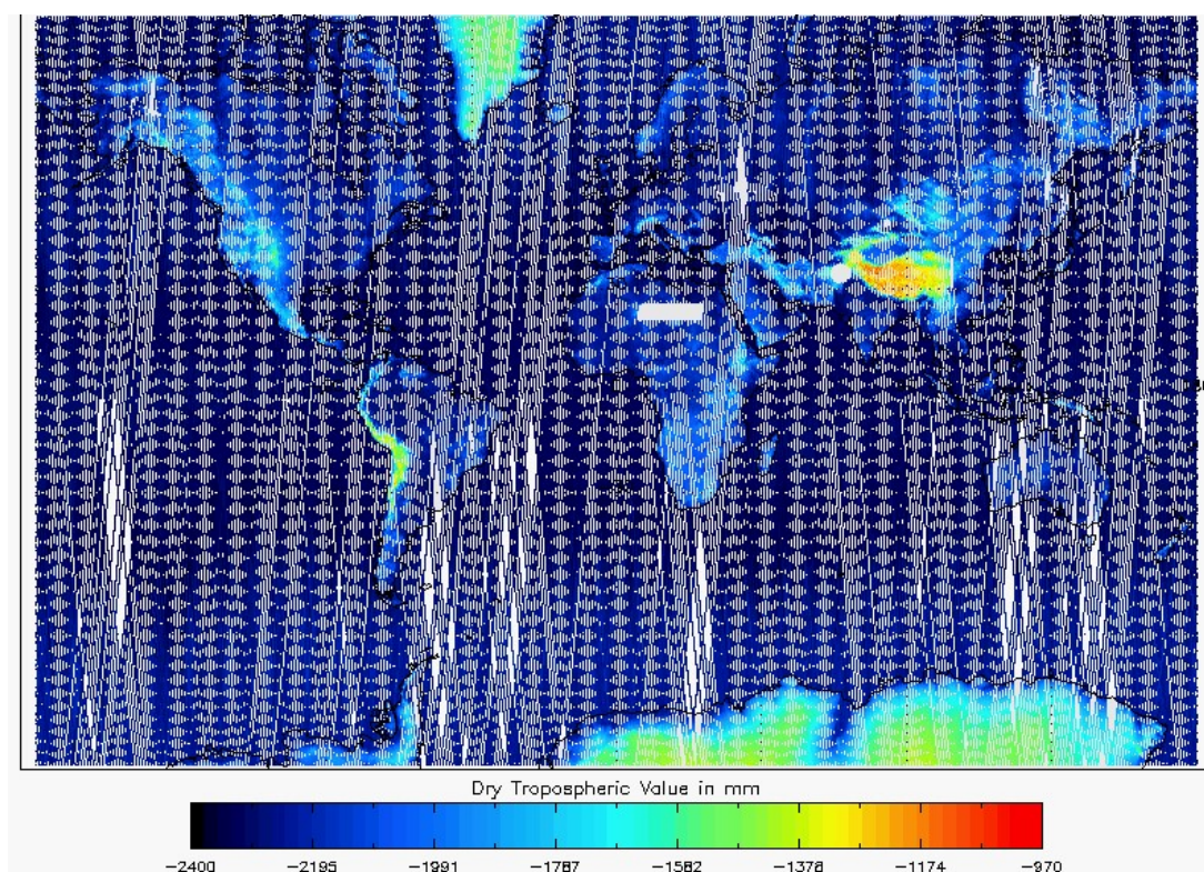
Figure 21 - Global plot of Dry Tropospheric Correction for cycle #162
