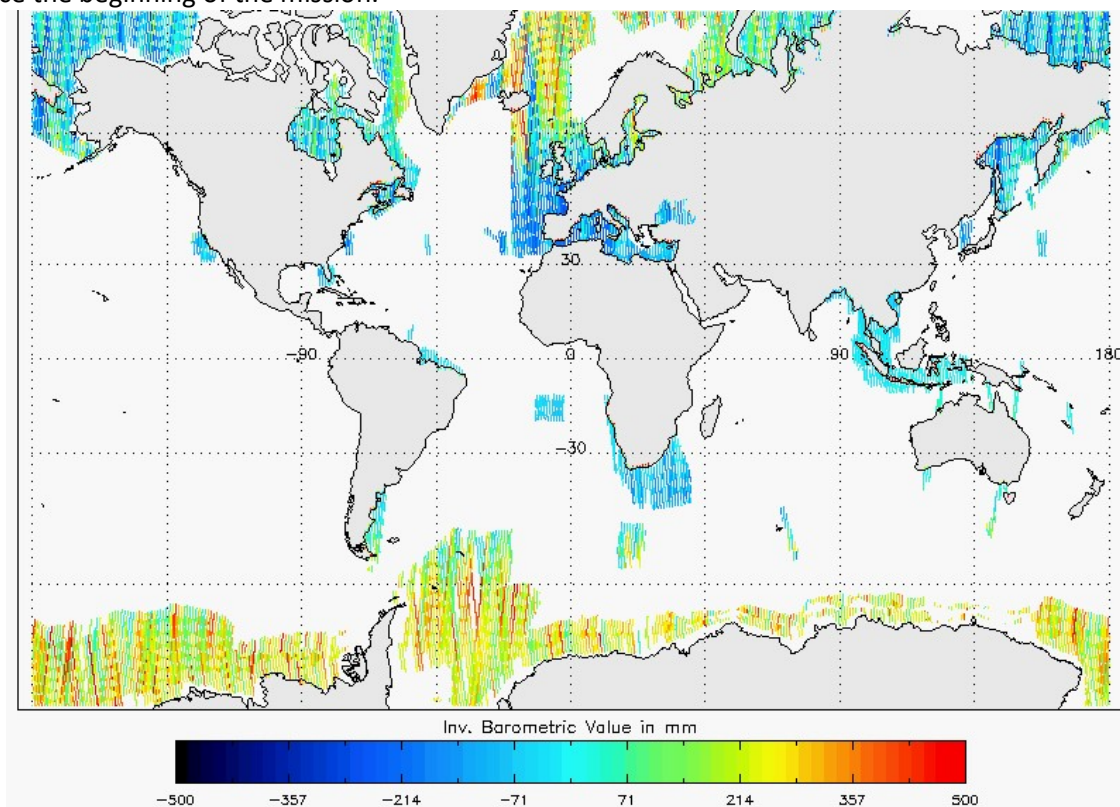
Figure 25 - Global plot of Inverse Barometric Correction for cycle #162
