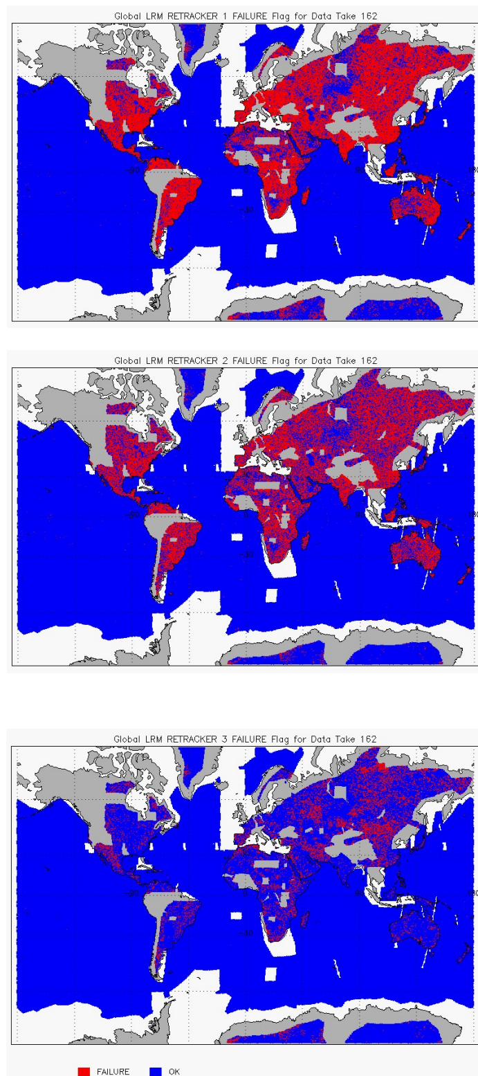
Figure 14 – Global plots showing Retracker Failure Flags for LRM mode for cycle #162:
