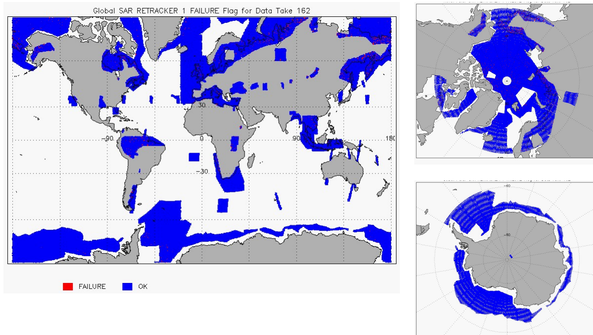
Figure 15 - Global plots showing Retracker Failure Flags for SAR mode for cycle #162
