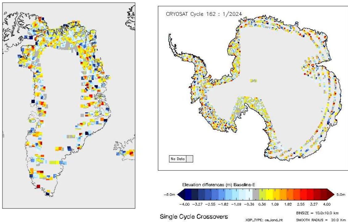
Figure 20 - Greenland and Antarctica maps of SARIn elevation differences for cycle #162.
