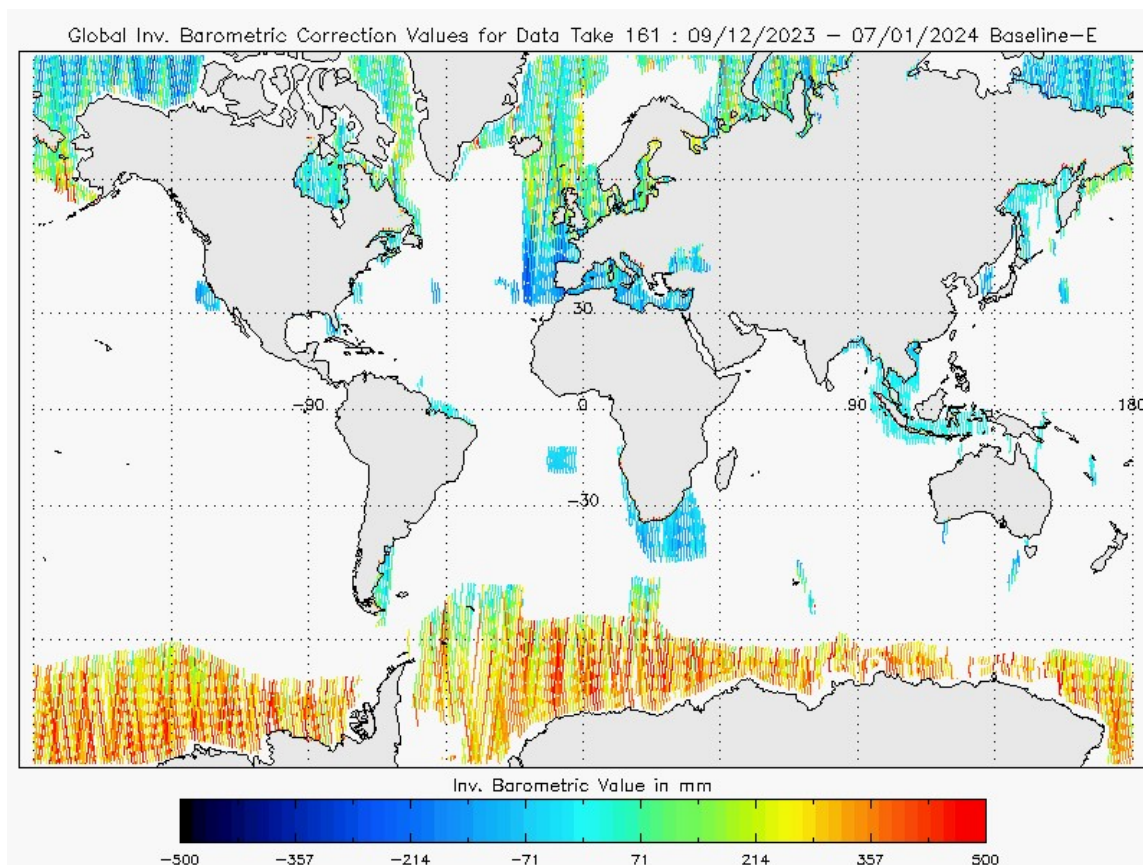
Figure 25 - Global plot of Inverse Barometric Correction for cycle #161
