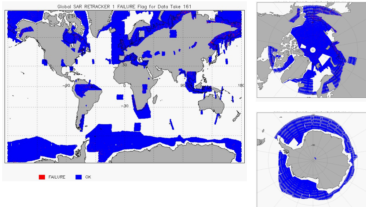
Figure 15 - Global plots showing Retracker Failure Flags for SAR mode for cycle #161
