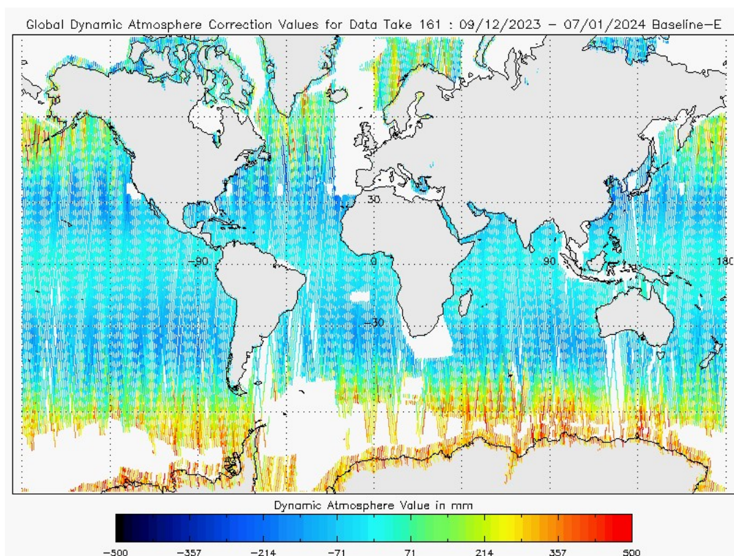
Figure 27 - Global plot of Dynamic Atmospheric Correction for cycle #161
