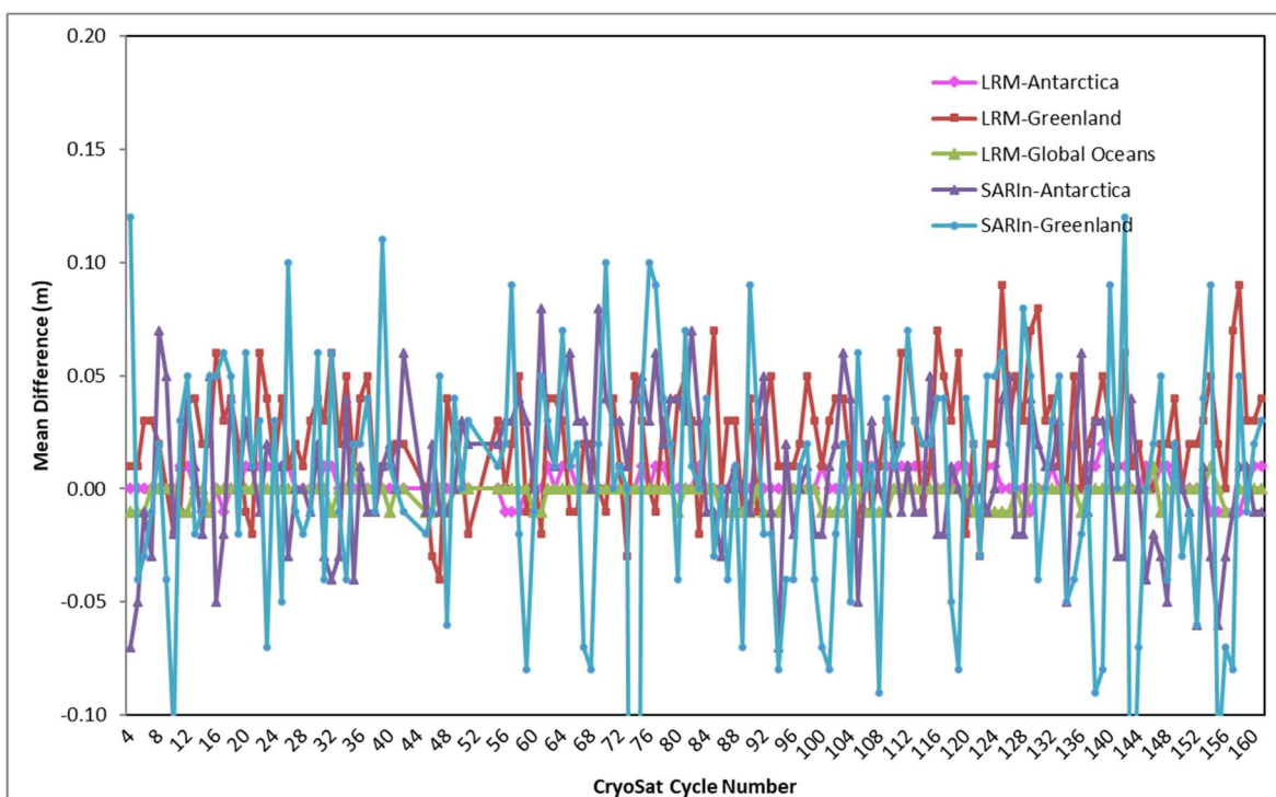
Figure 18 - Time series for Mean Difference in elevation at crossovers from beginning of the mission
