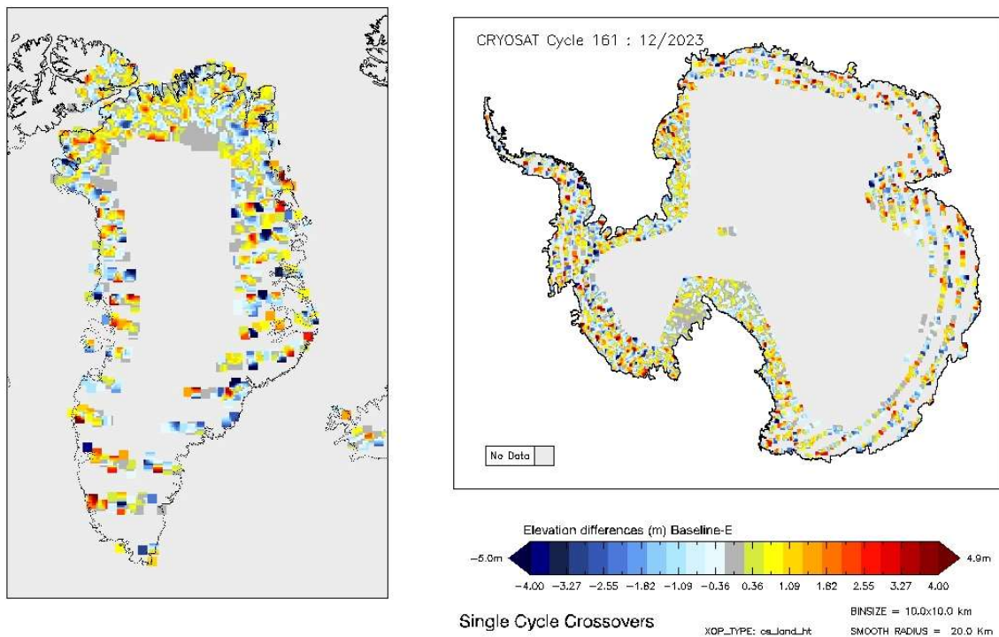
Figure 20 - Greenland and Antarctica maps of SARIn elevation differences for cycle #161.
