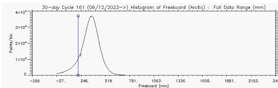
Figure 5 – Histogram of Freeboard for Arctic (above) for cycle #161
