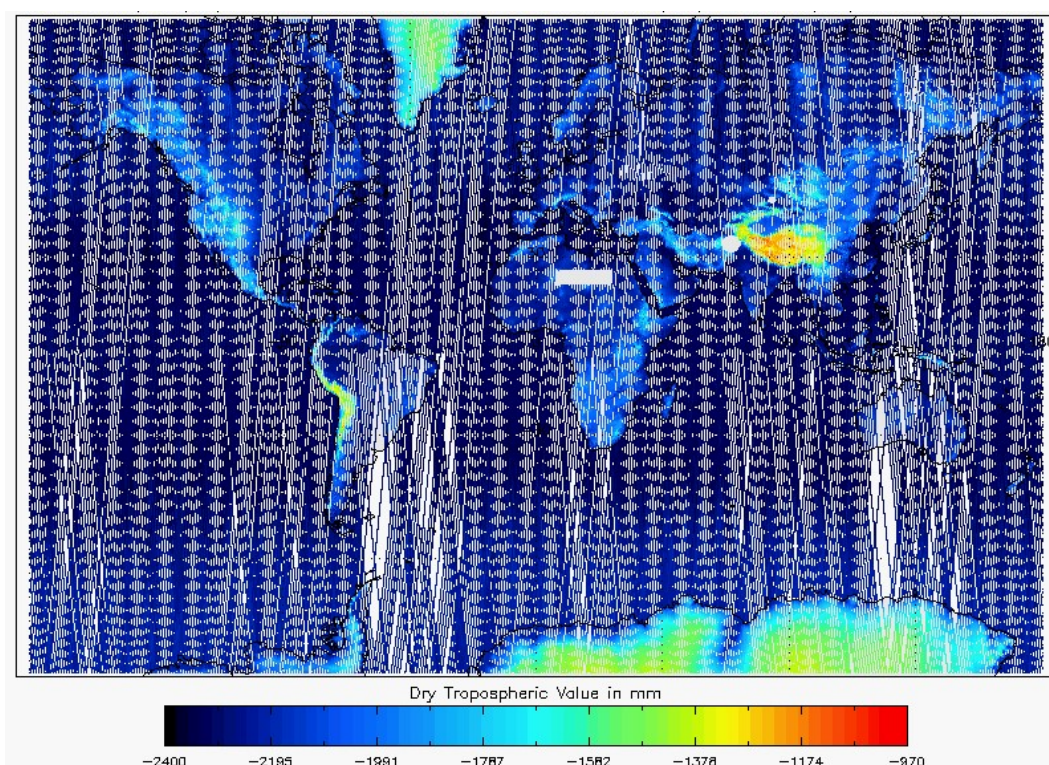
Figure 21 - Global plot of Dry Tropospheric Correction for cycle #161
