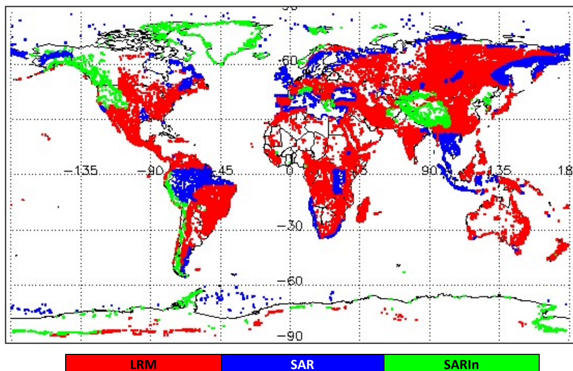
Figure 1 – Global plot showing areas of loss of track in all SIRAL modes L0 data during December 2023
