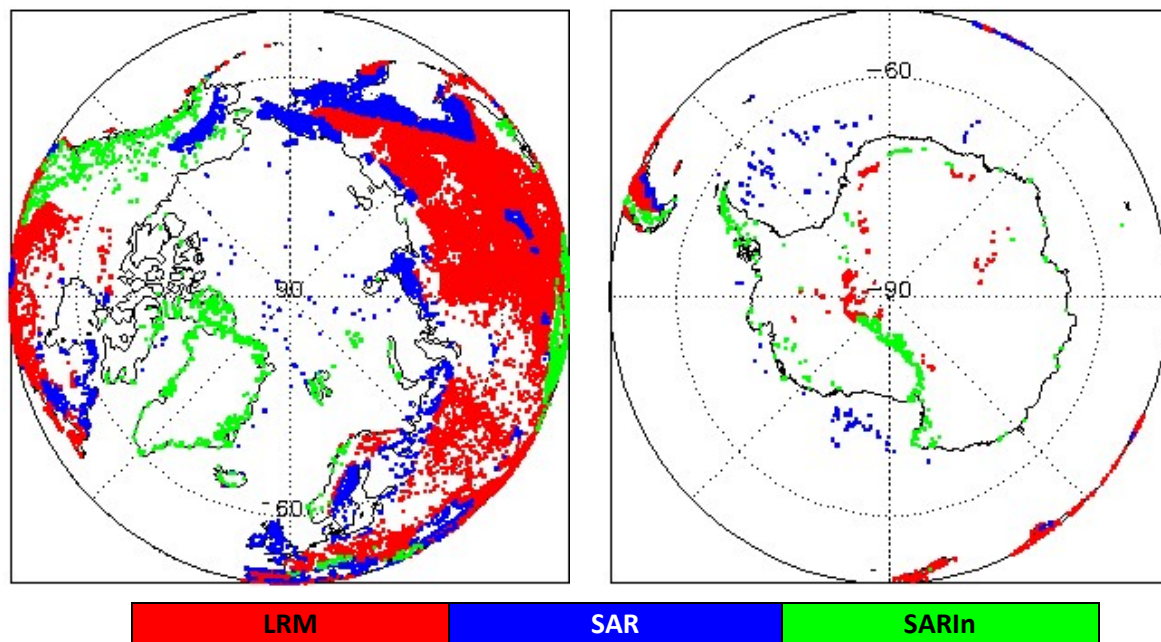
Figure 2 - Polar plots showing areas of loss of track in all SIRAL modes L0 data during December 2023.
