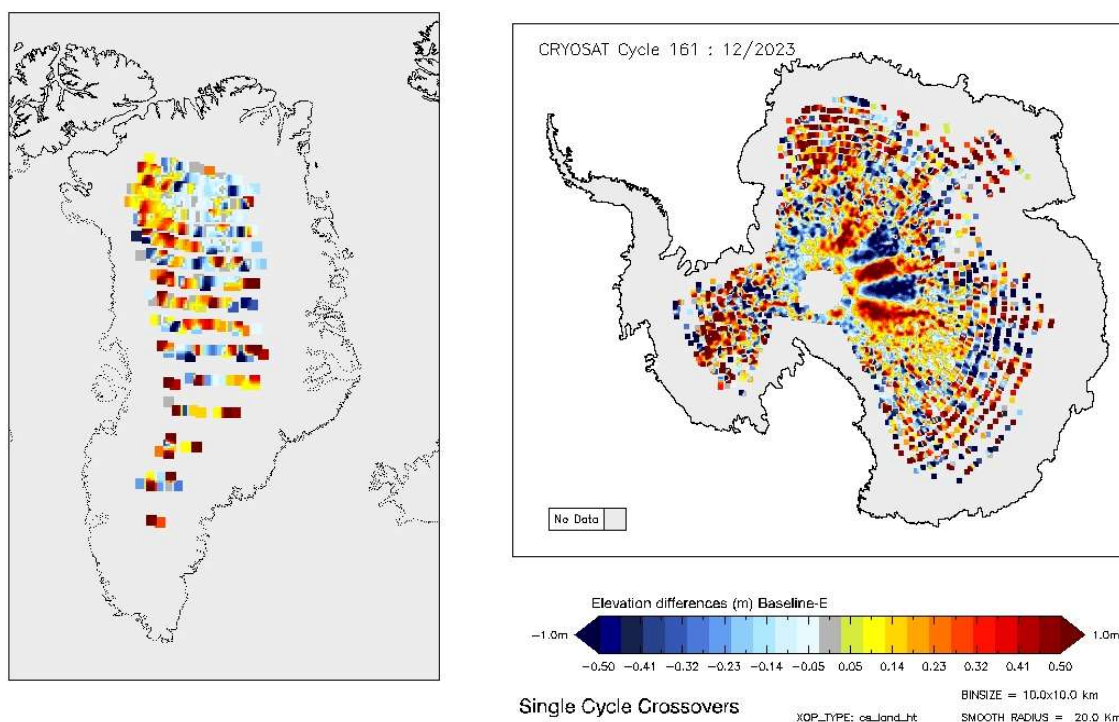
Figure 19 - Greenland and Antarctica maps of LRM elevation differences for cycle #161.
