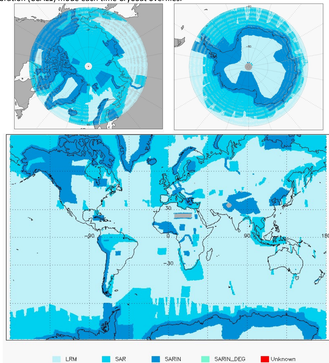
Figure 3 - Global and Polar plots of SIRAL Modes for cycle #161.
