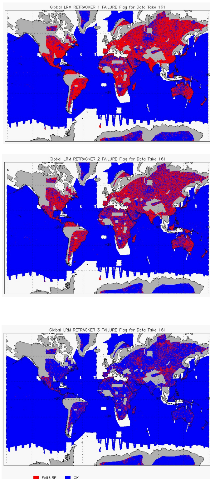
Figure 14 – Global plots showing Retracker Failure Flags for LRM mode for cycle #161:
