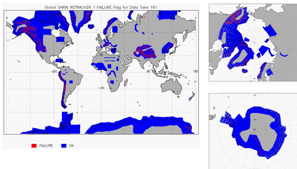
Figure 16 – Global plots showing Retracker Failure Flags for SARIn mode for cycle #161
