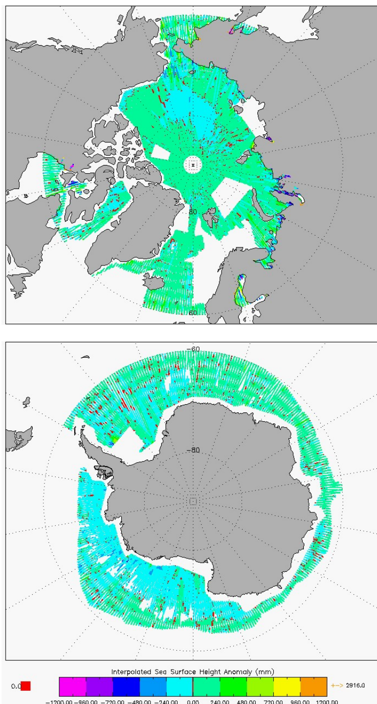
Figure 8 –Polar plots of SSHA for cycle #161.
