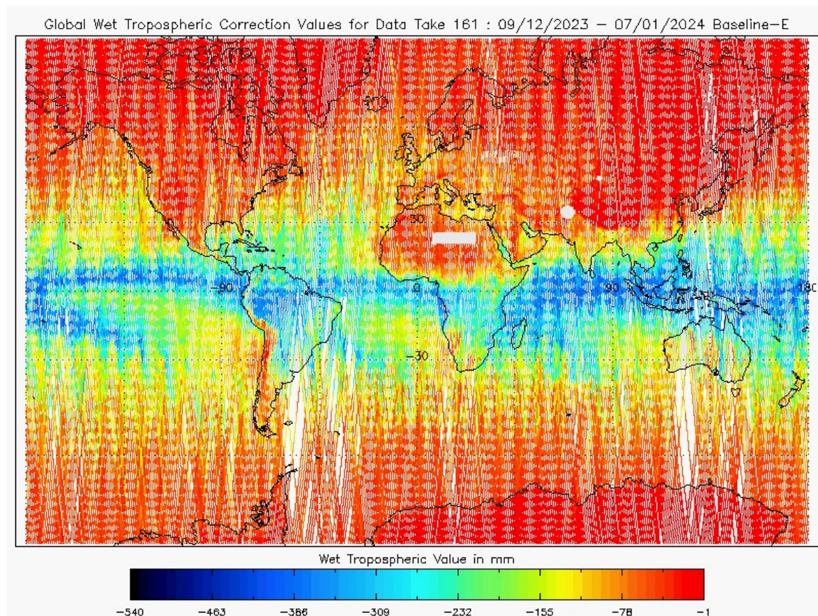
Figure 23 - Global plot of Wet Tropospheric Correction for cycle #161
