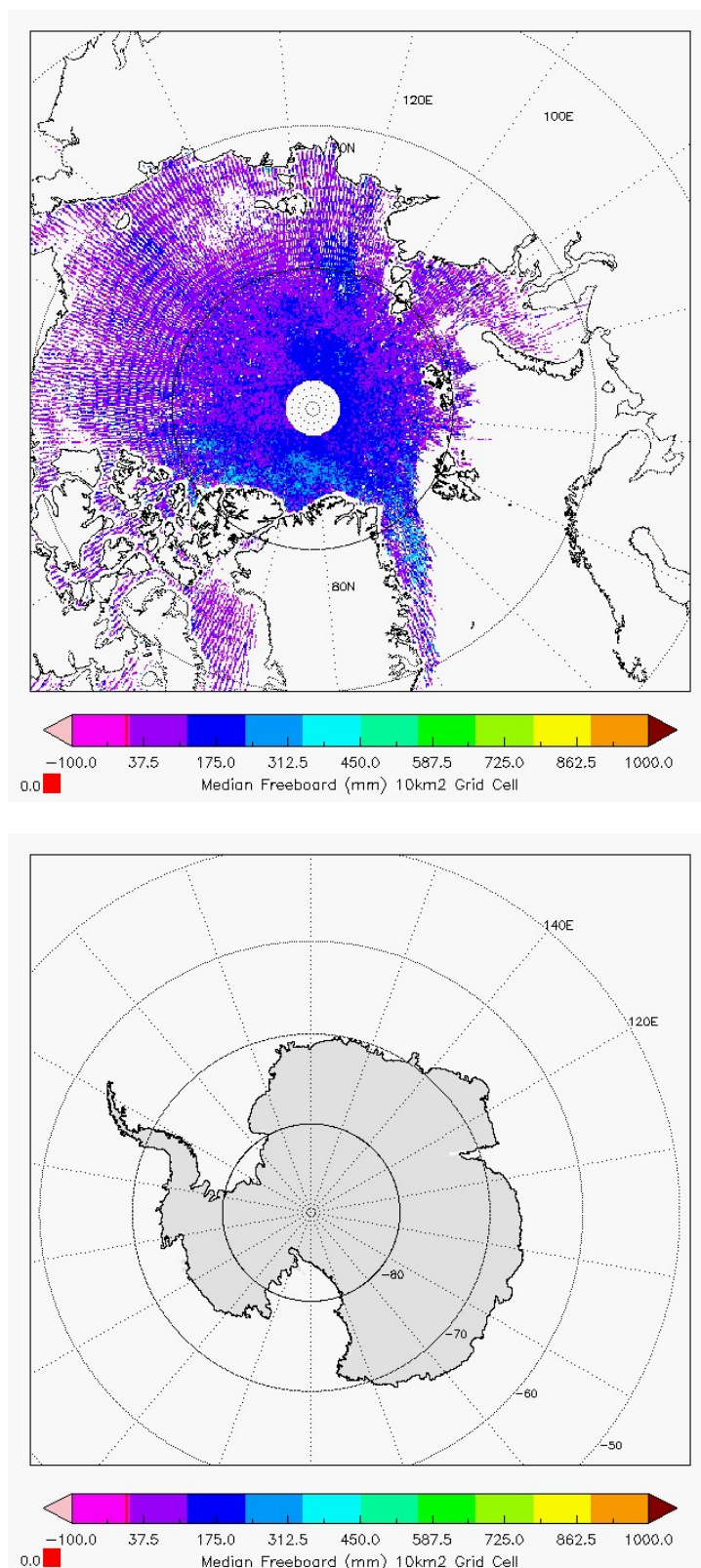
Figure 6 - Polar plots of 10km Gridded Freeboard values from L2 SAR products in cycle #161.
