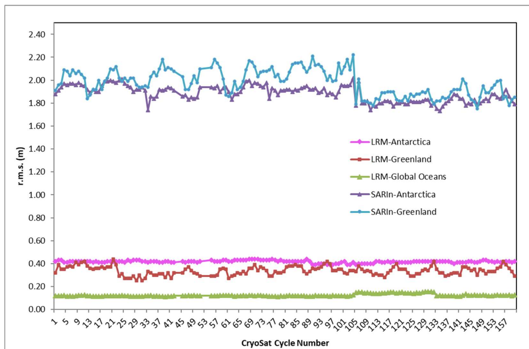
Figure 18 - Time series for crossover elevation r.m.s values from beginning of the mission
