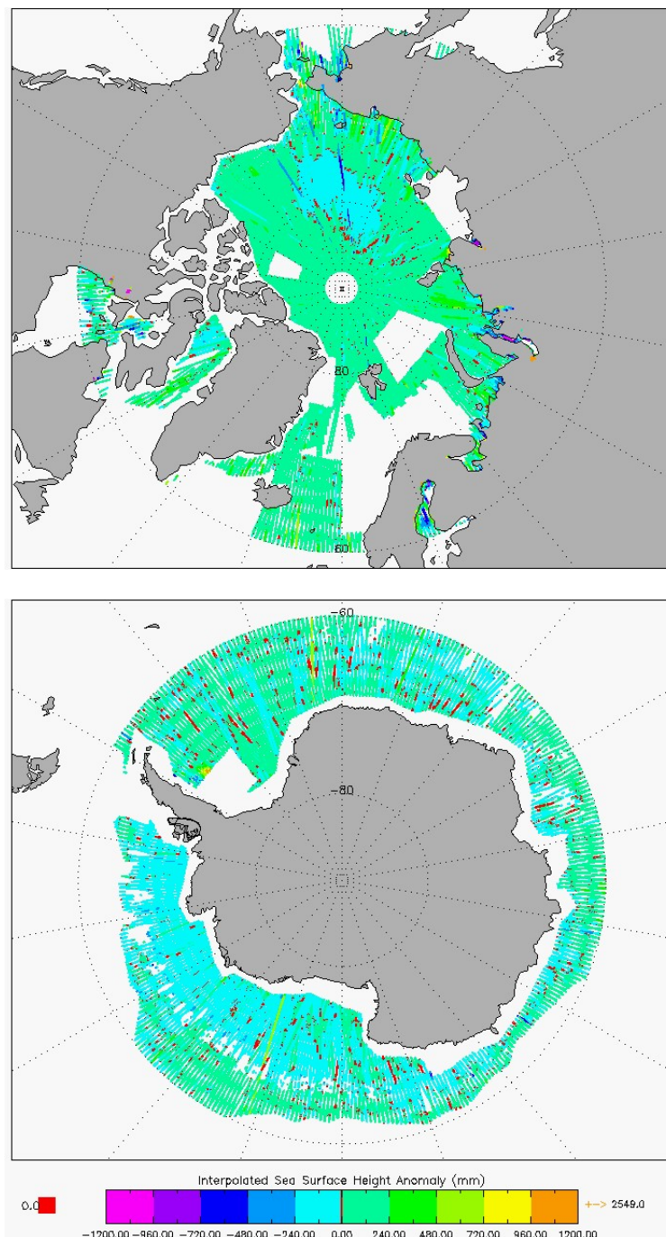
Figure 9 –Polar plots of SSHA for cycle #160.
