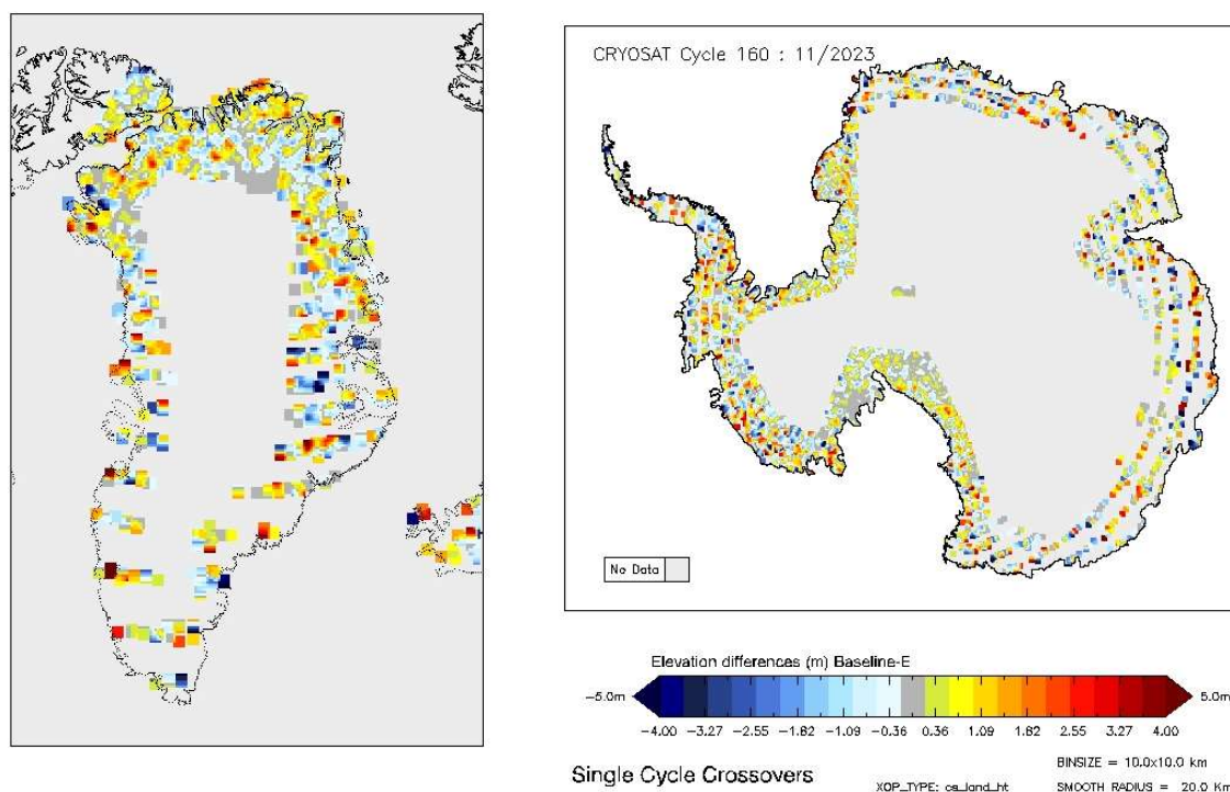
Figure 21 - Greenland and Antarctica maps of SARIn elevation differences for cycle #160.
