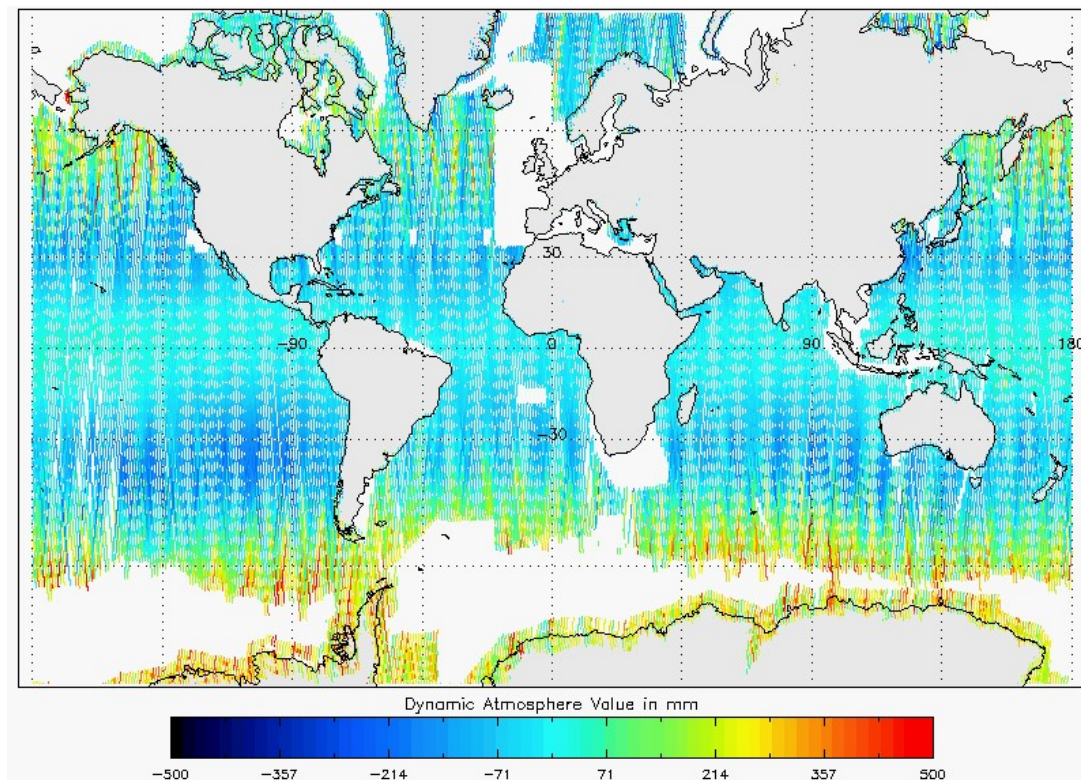
Figure 28 - Global plot of Dynamic Atmospheric Correction for cycle #160
