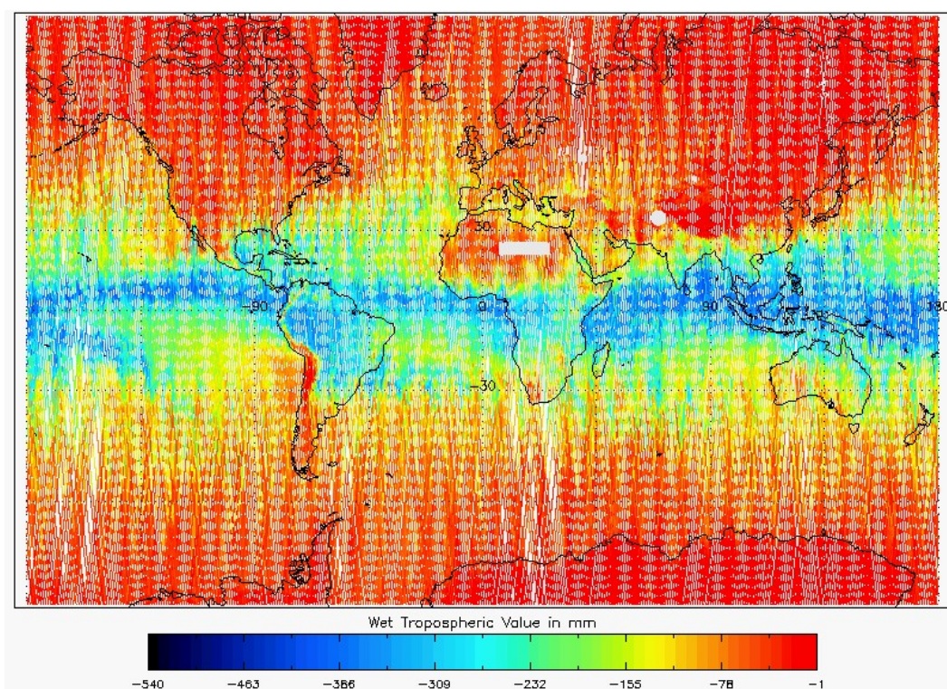
Figure 24 - Global plot of Wet Tropospheric Correction for cycle #146
