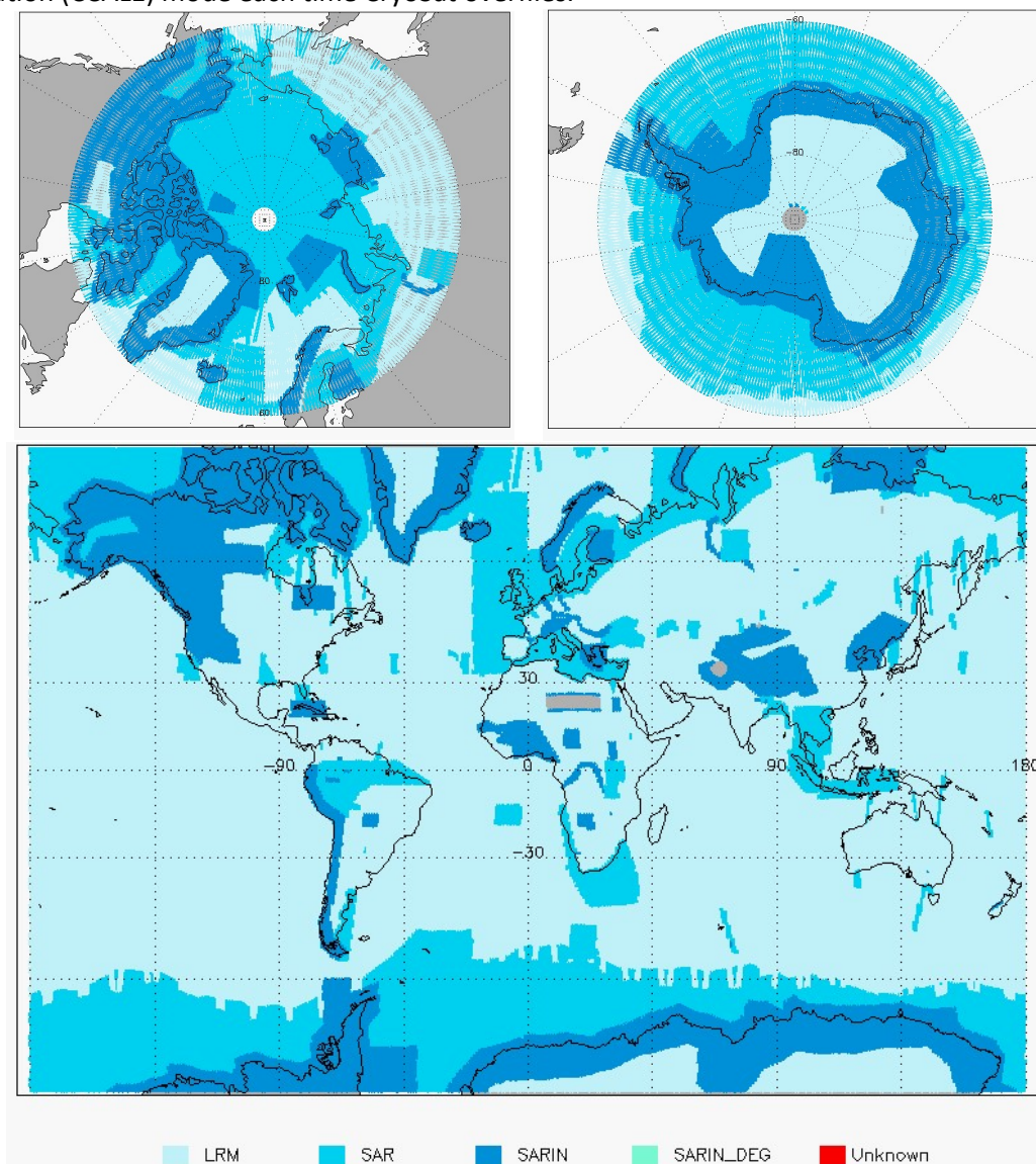
Figure 3 - Global and Polar plots of SIRAL Modes for cycle #160.
