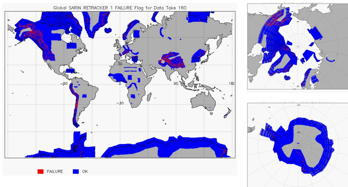
Figure 17 – Global plots showing Retracker Failure Flags for SARIn mode for cycle #160
