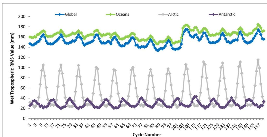
Figure 25 – Wet Tropospheric Correction RMS value trend from beginning of mission
