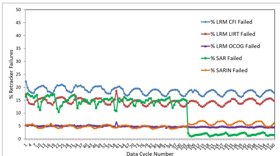
Figure 14 – Time Series for Retracker Failure Flags
