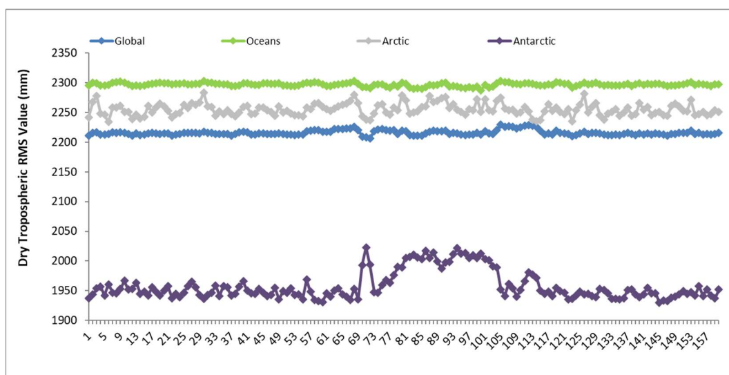
Figure 23 - Dry Tropospheric Correction RMS value trend from beginning of mission
