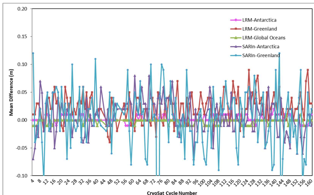
Figure 19 - Time series for Mean Difference in elevation at crossovers from beginning of the mission
