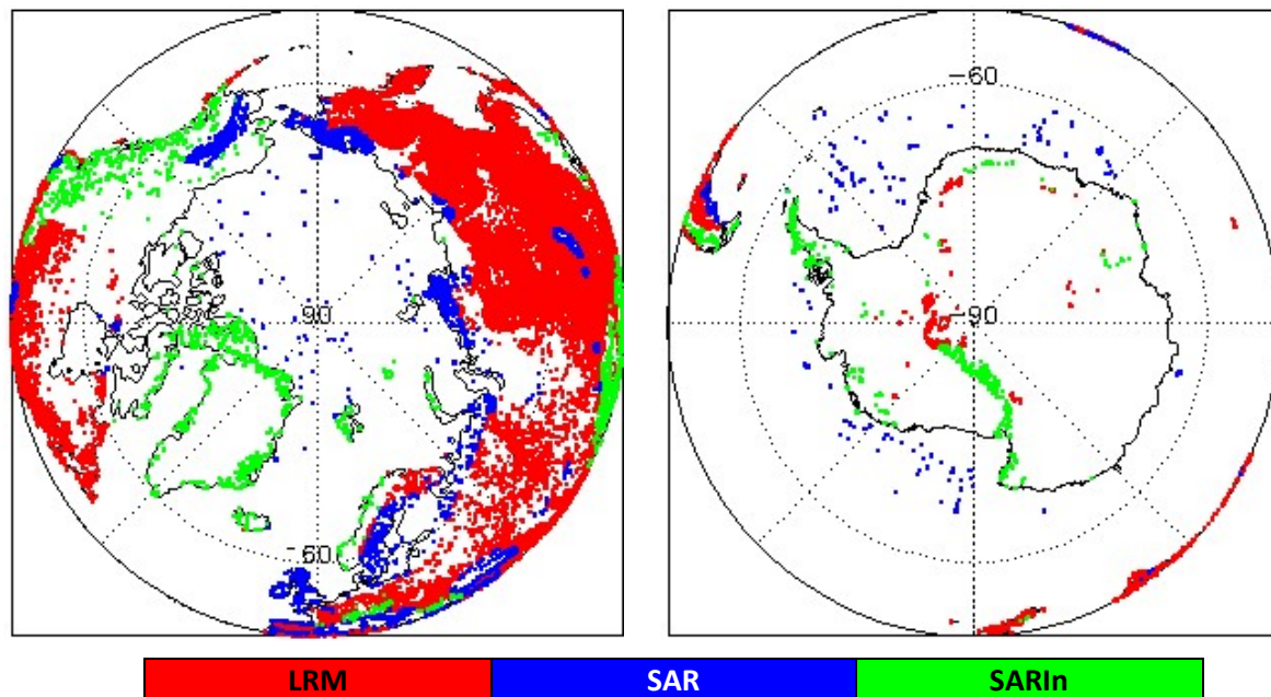
Figure 2 - Polar plots showing areas of loss of track in all SIRAL modes L0 data during November 2023.
