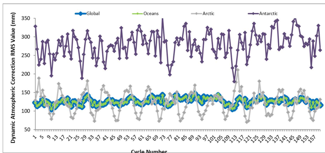
Figure 29 – Dynamic Atmospheric Correction RMS value trend from beginning of mission
