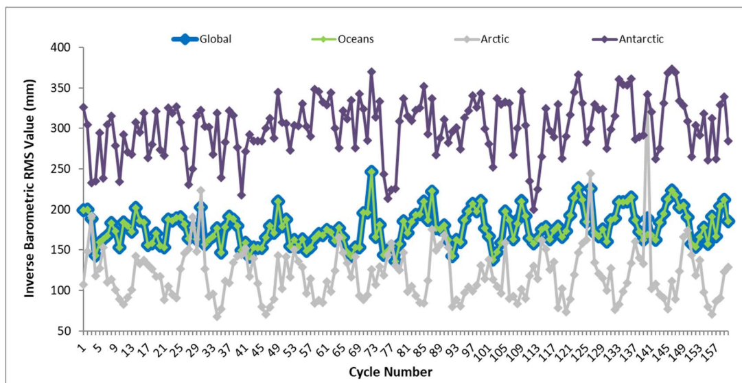
Figure 27 – Inverse Barometric Correction RMS value trend from beginning of mission
