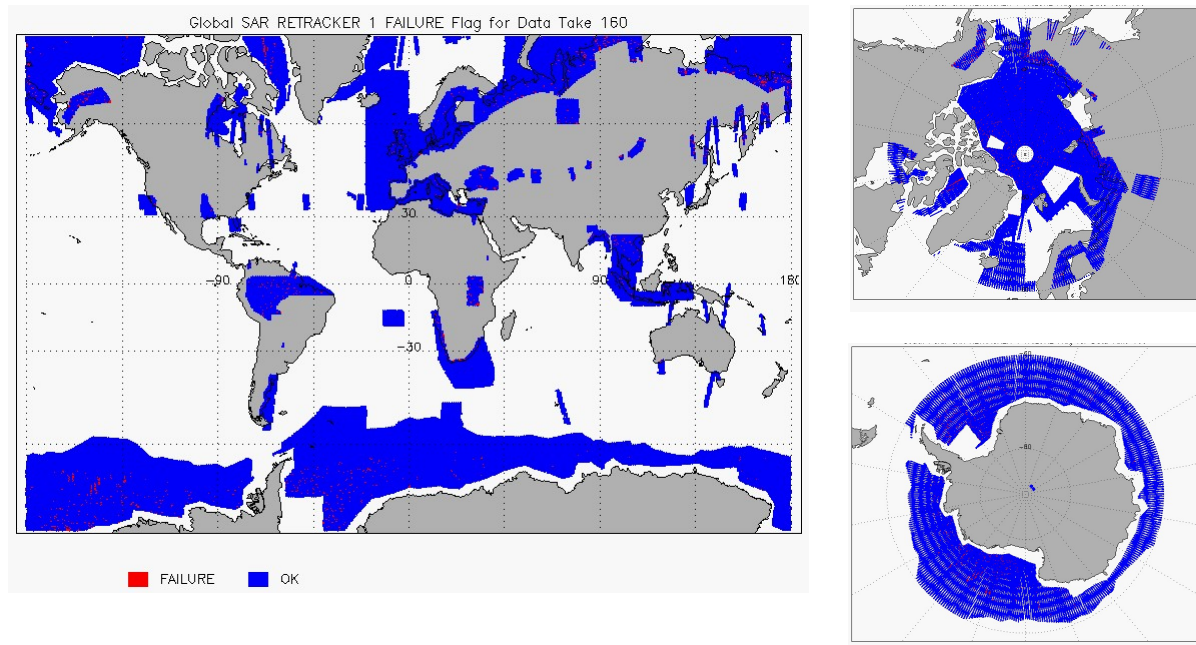
Figure 16 - Global plots showing Retracker Failure Flags for SAR mode for cycle #160
