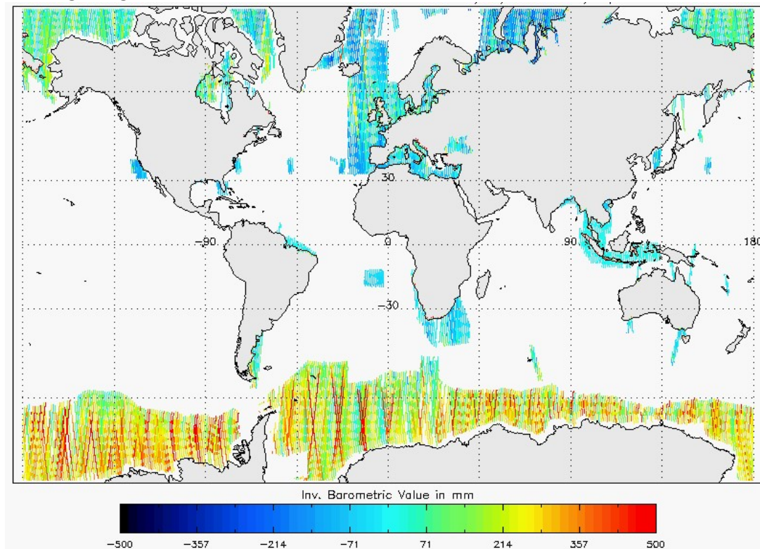
Figure 26 - Global plot of Inverse Barometric Correction for cycle #146
