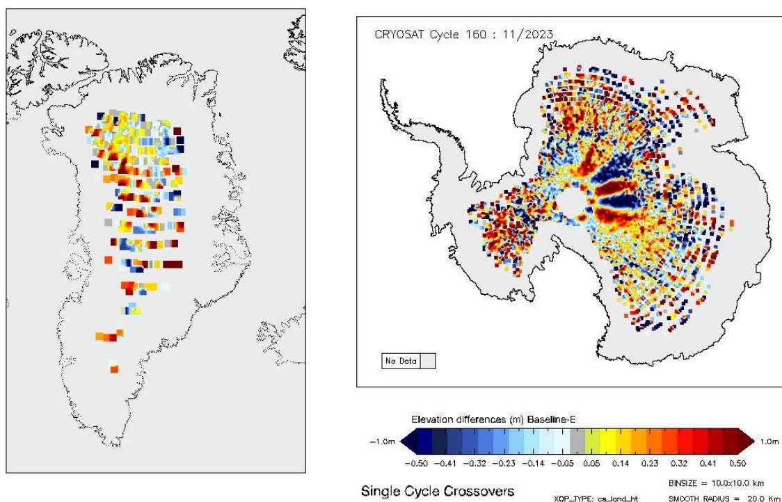
Figure 20 - Greenland and Antarctica maps of LRM elevation differences for cycle #160.
