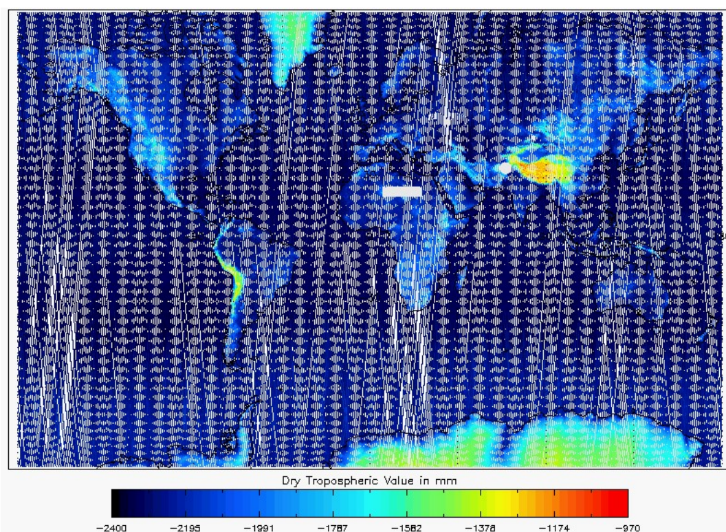
Figure 22 - Global plot of Dry Tropospheric Correction for cycle #160
