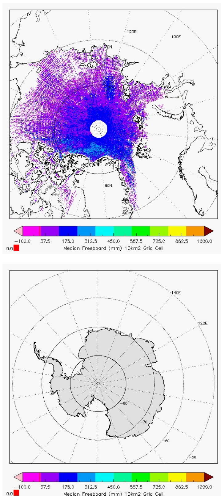
Figure 7 - Polar plots of 10km Gridded Freeboard values from L2 SAR products in cycle #160.
