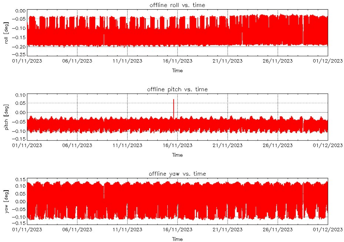
Figure 4 – Roll (top), Pitch (middle) and Yaw (bottom) values for L1B Products during cycle #160.
