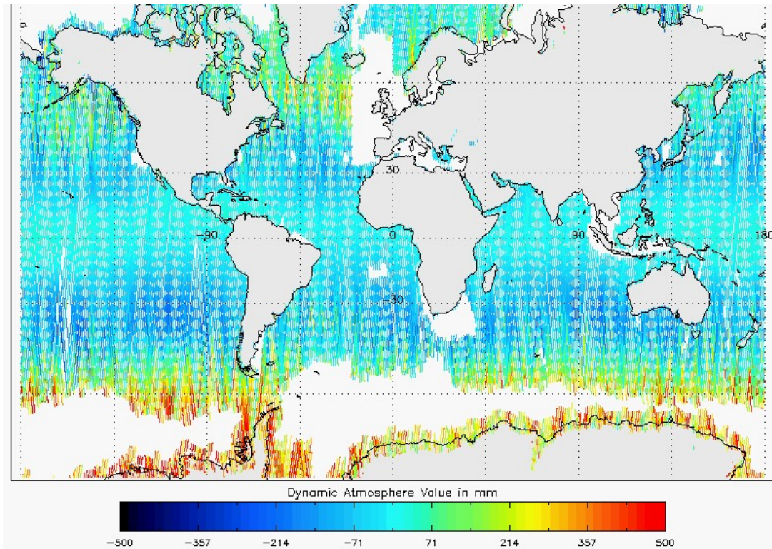
Figure 28 - Global plot of Dynamic Atmospheric Correction for cycle #159
