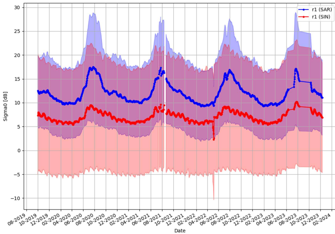
Figure 12 – Sigma0 (dB) daily mean and standard deviation for L2 SAR and SIN products.
