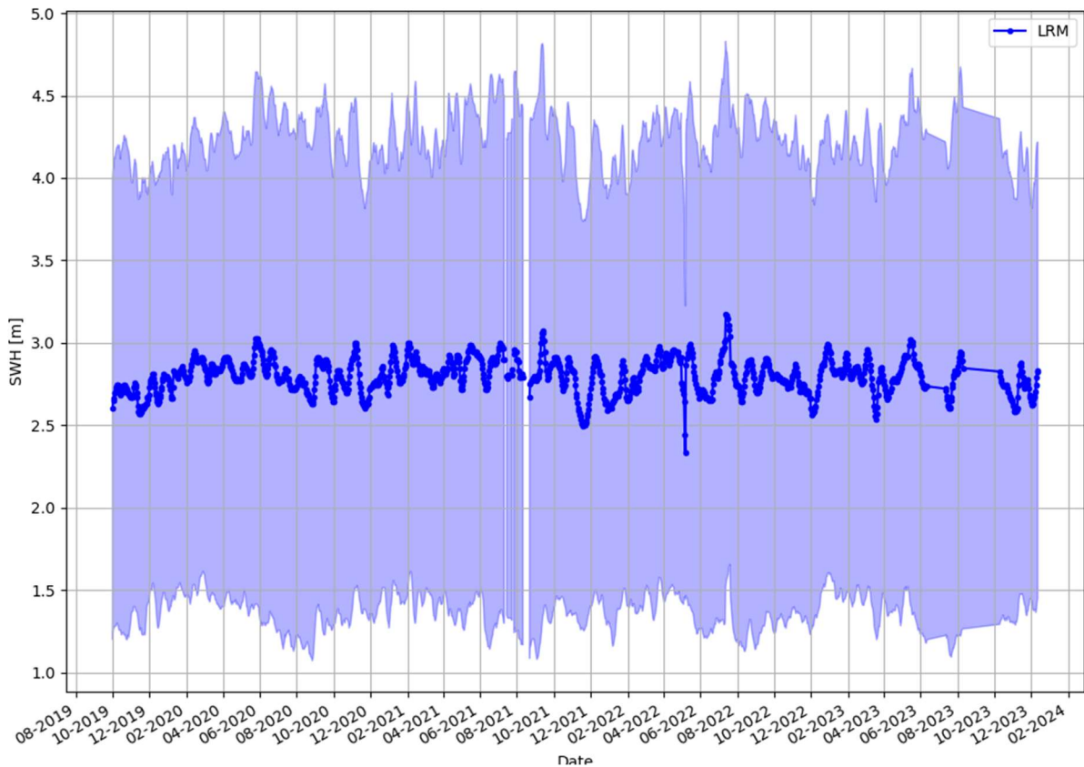
Figure 13 –SWH (m) daily mean and standard deviation for L2 LRM products.
