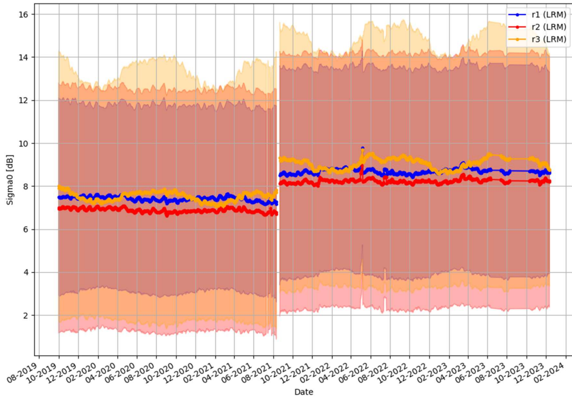
Figure 11 - Sigma0 (dB) daily mean and standard deviation for L2 LRM products.
