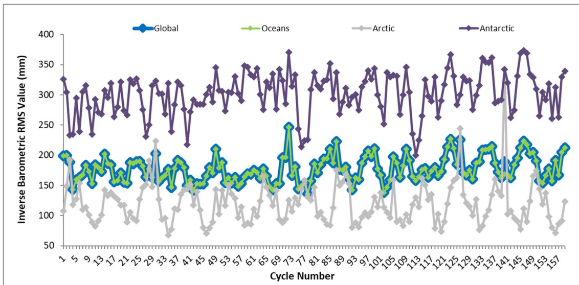
Figure 27 – Inverse Barometric Correction RMS value trend from beginning of mission
