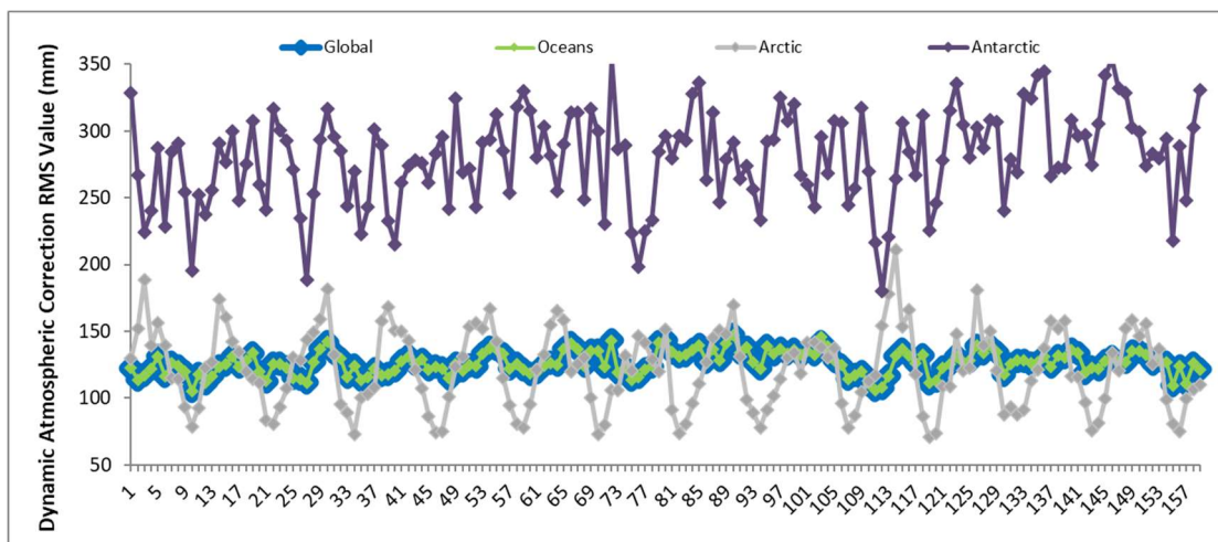
Figure 29 – Dynamic Atmospheric Correction RMS value trend from beginning of mission
