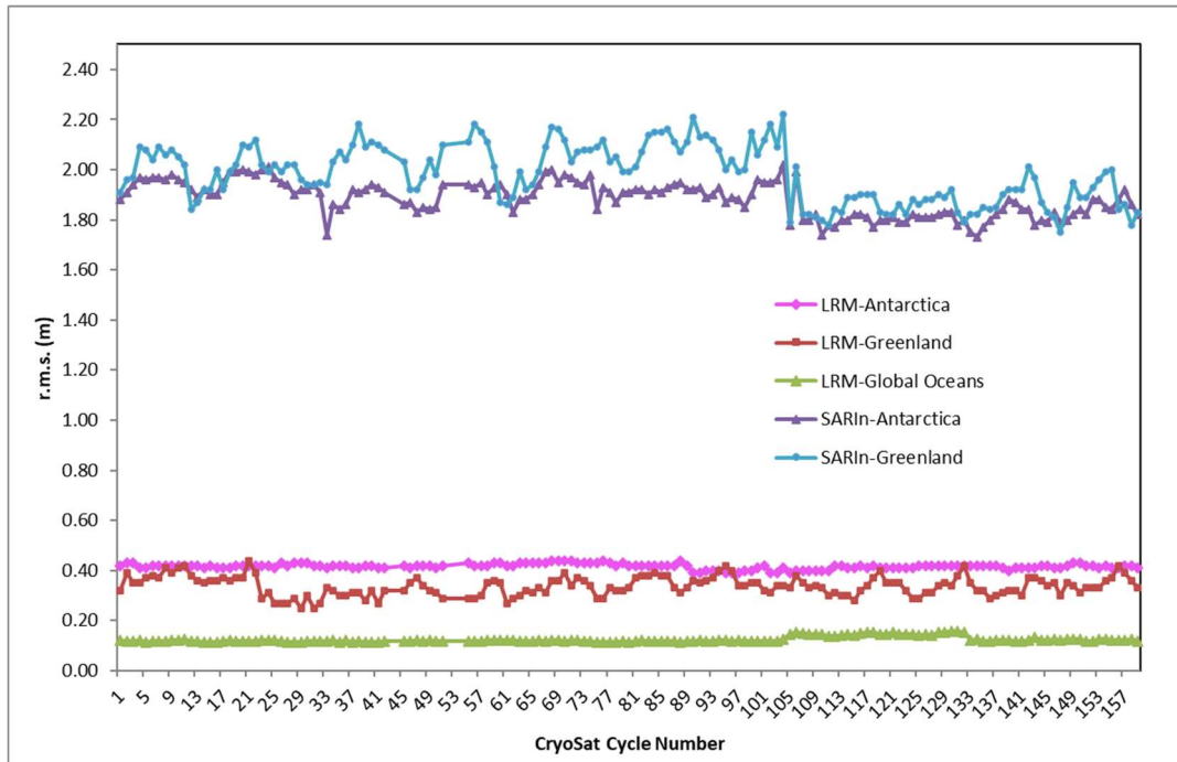
Figure 18 - Time series for crossover elevation r.m.s values from beginning of the mission
