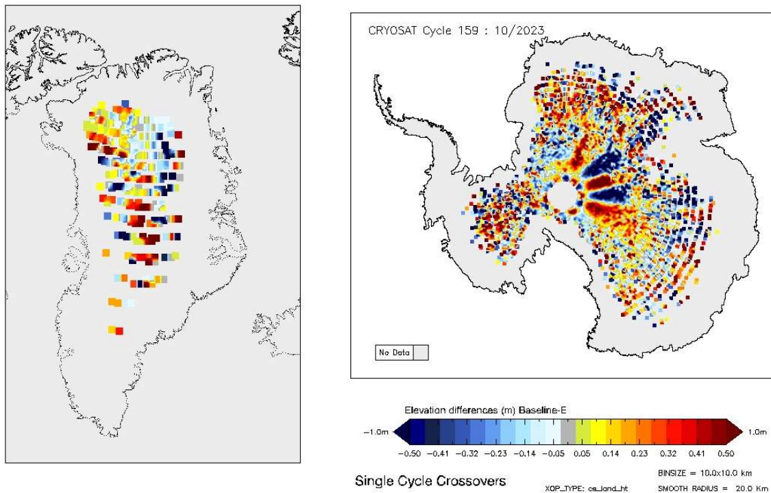
Figure 20 - Greenland and Antarctica maps of LRM elevation differences for cycle #159.
