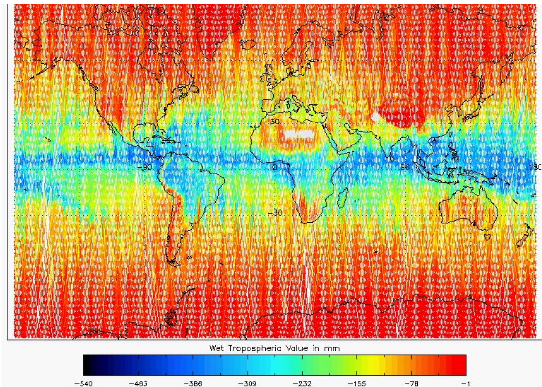
Figure 24 - Global plot of Wet Tropospheric Correction for cycle #159
