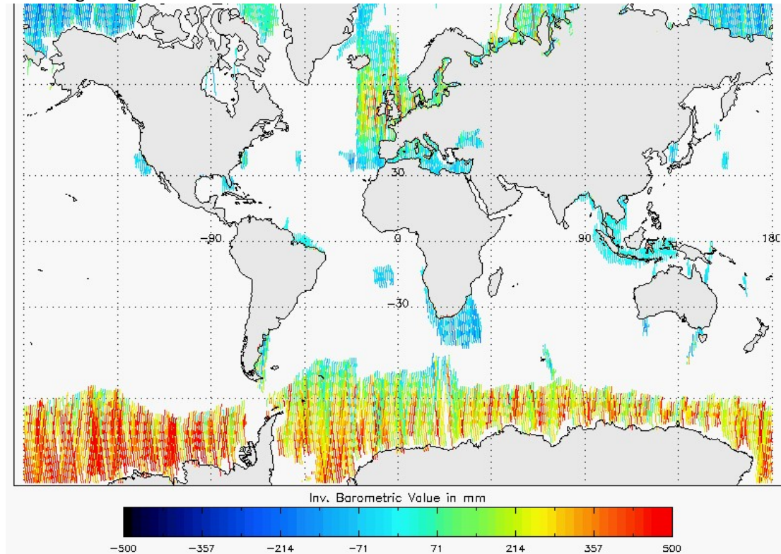
Figure 26 - Global plot of Inverse Barometric Correction for cycle #159
