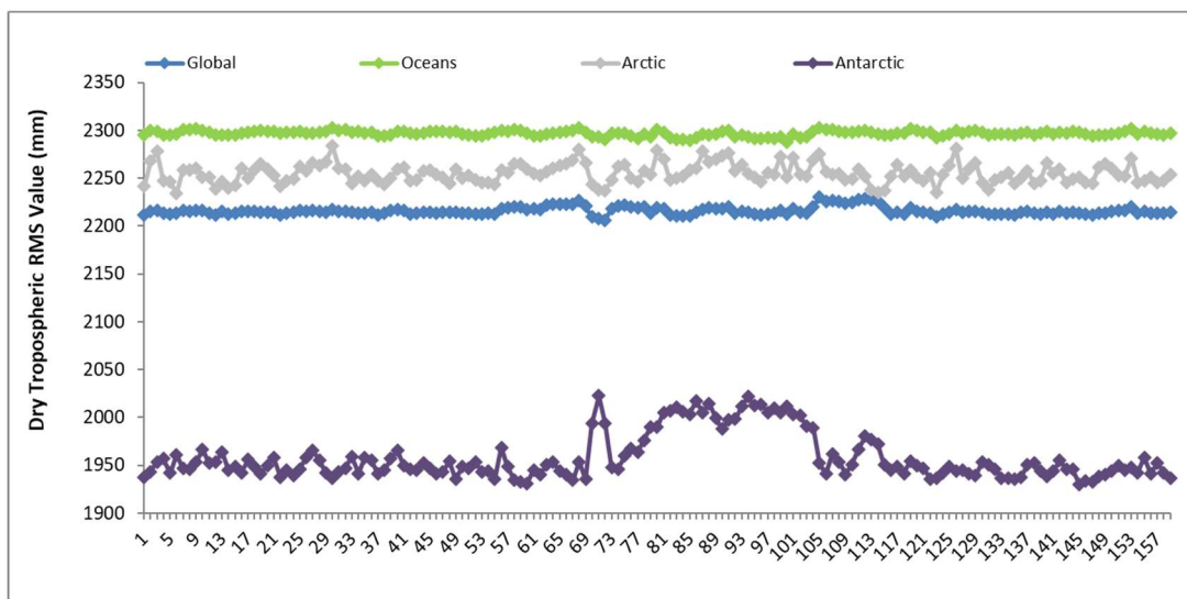
Figure 23 - Dry Tropospheric Correction RMS value trend from beginning of mission
