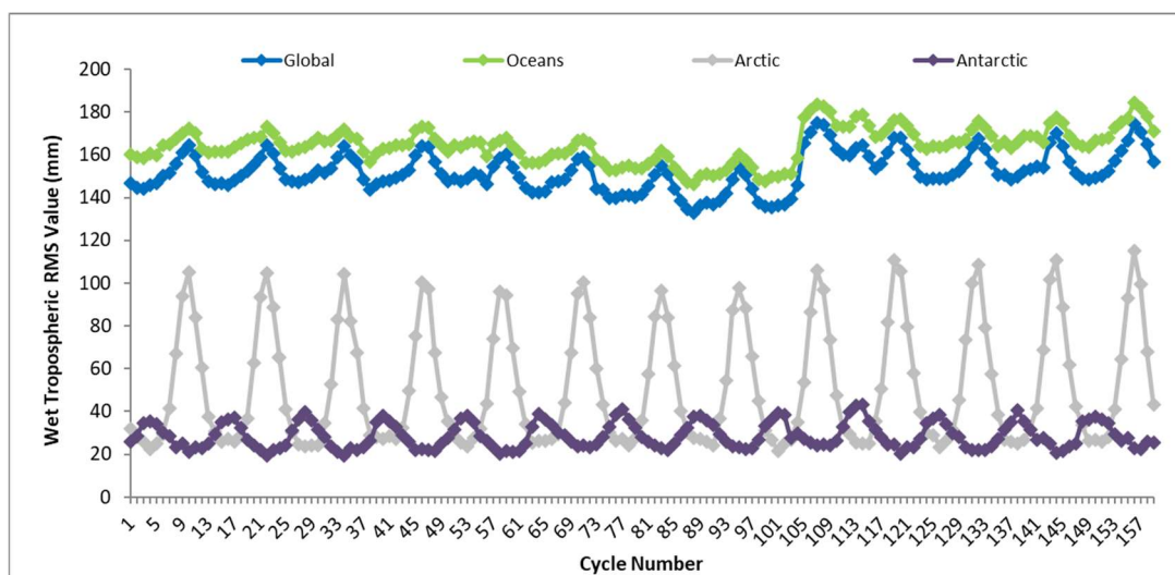
Figure 25 – Wet Tropospheric Correction RMS value trend from beginning of mission
