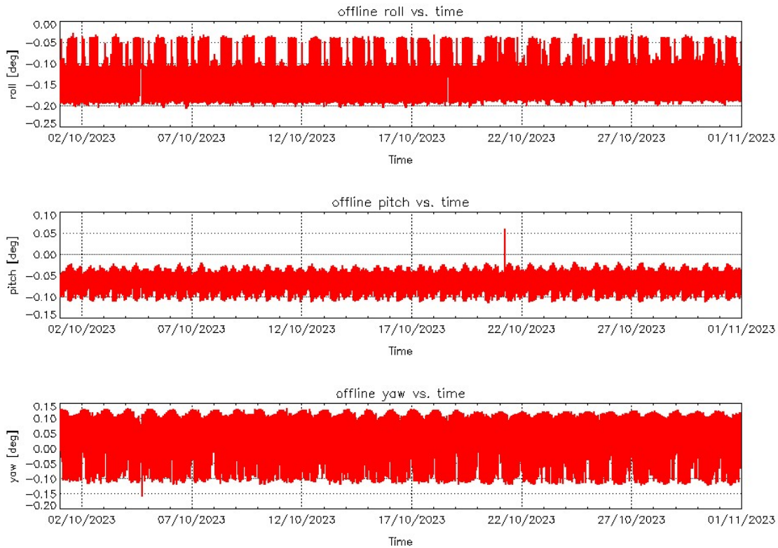
Figure 4 – Roll (top), Pitch (middle) and Yaw (bottom) values for L1B Products during cycle #159.
