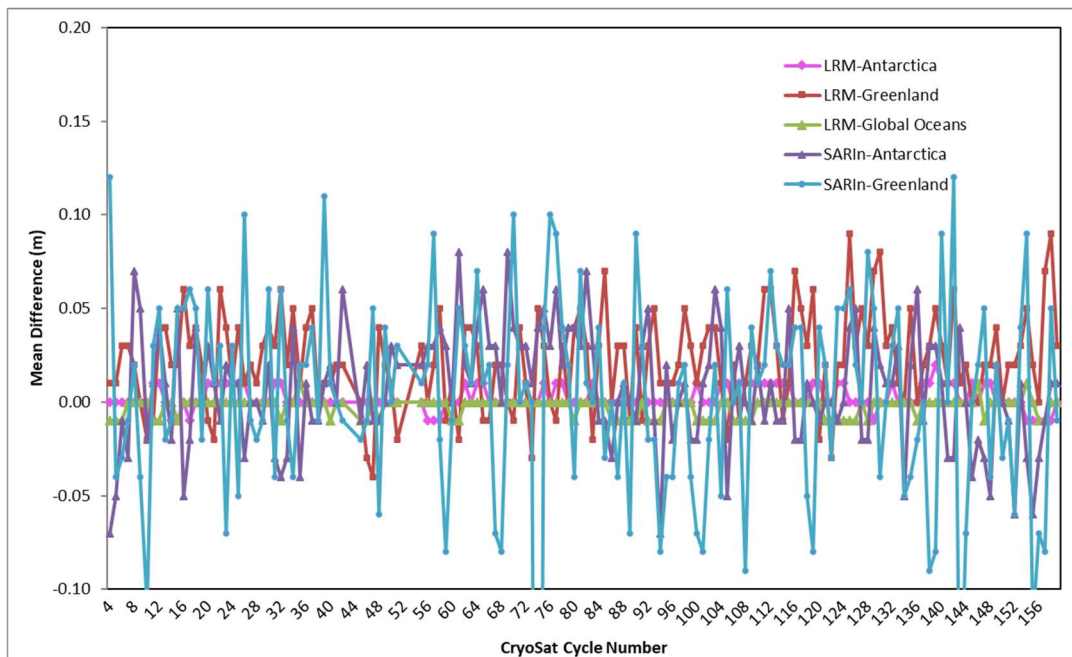
Figure 19 - Time series for Mean Difference in elevation at crossovers from beginning of the mission
