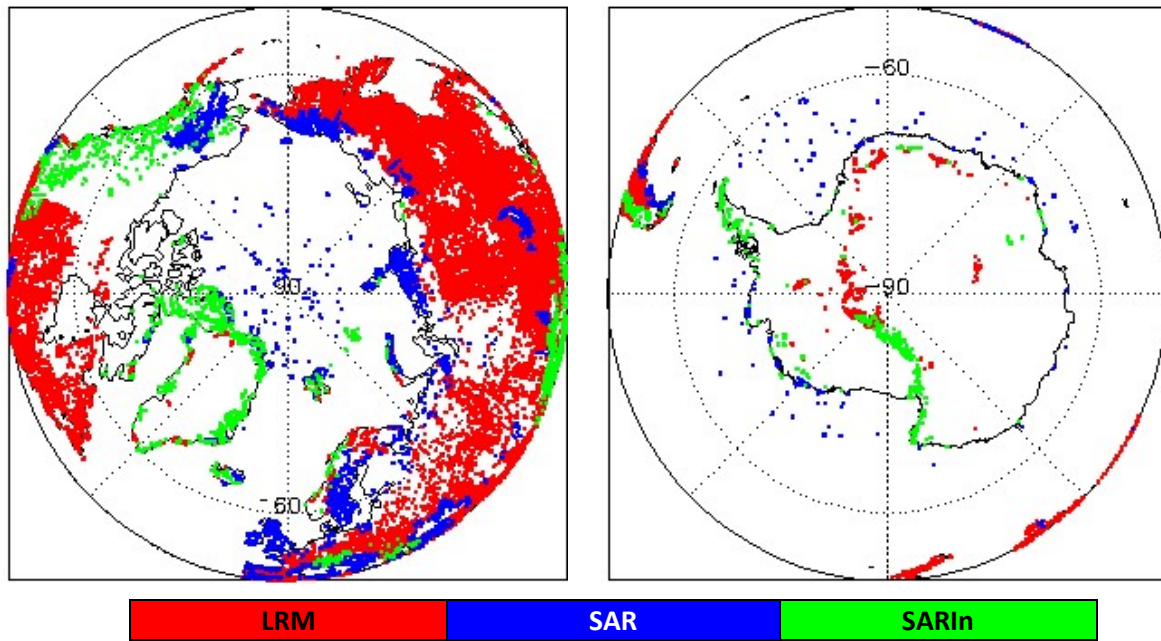
Figure 2 - Polar plots showing areas of loss of track in all SIRAL modes L0 data during October 2023.
