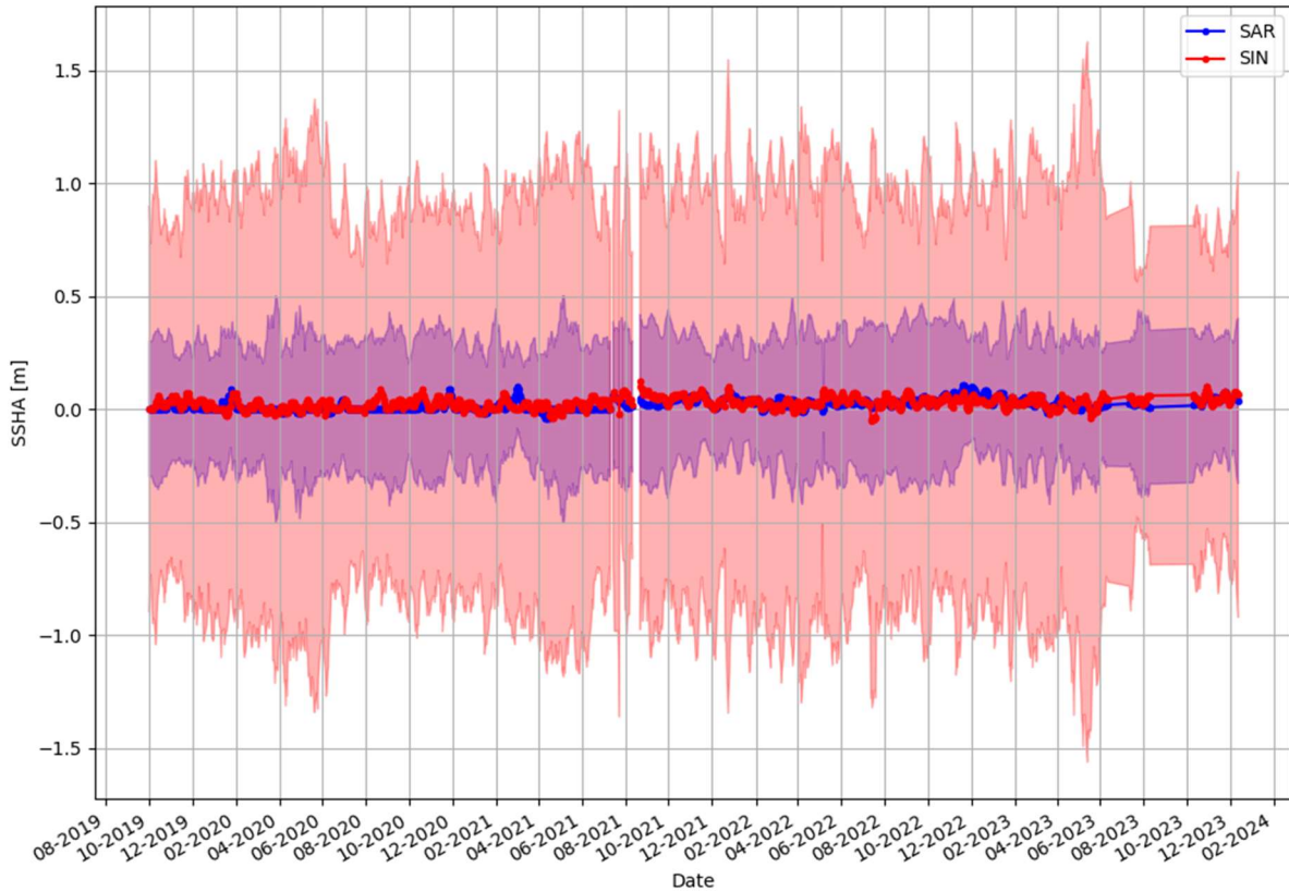
Figure 10 SSHA (m) daily mean and standard deviation for L2 SAR and SIN products.
