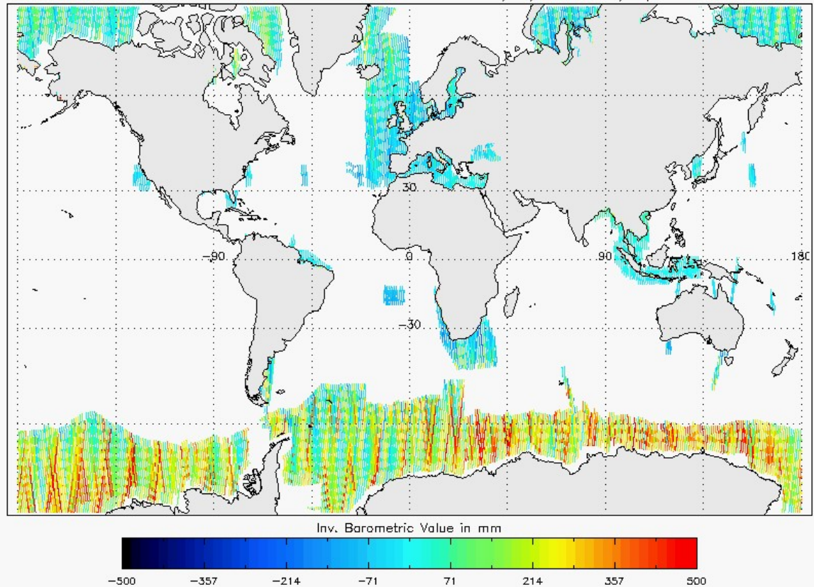
Figure 25 - Global plot of Inverse Barometric Correction for cycle #157
