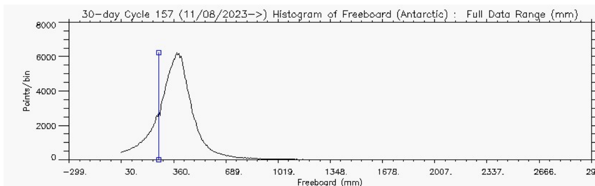
Figure 5 – Histogram of Freeboard for Antarctic for cycle #157
