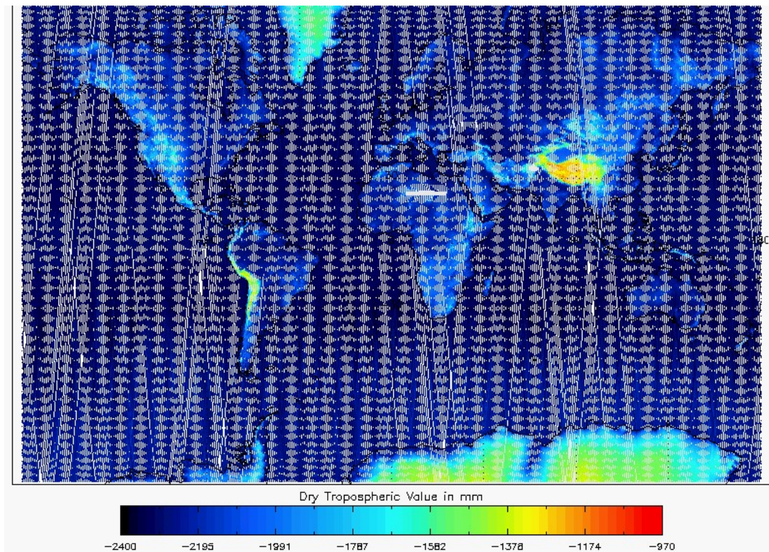
Figure 21 - Global plot of Dry Tropospheric Correction for cycle #157
