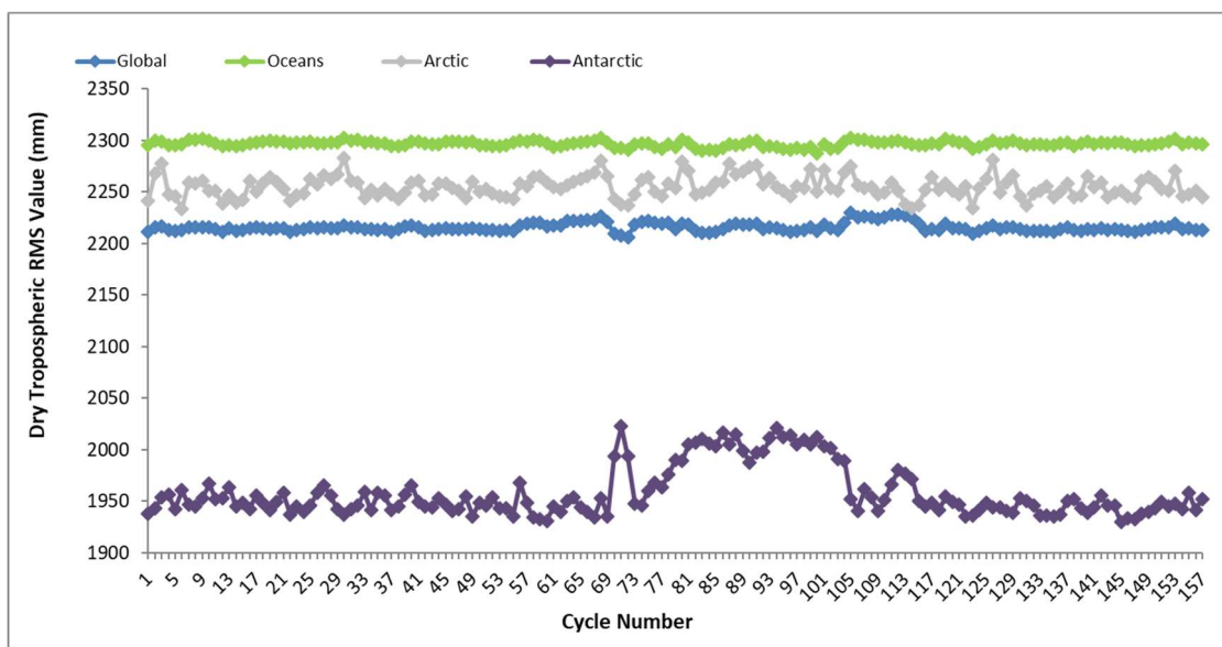
Figure 22 - Dry Tropospheric Correction RMS value trend from beginning of mission
