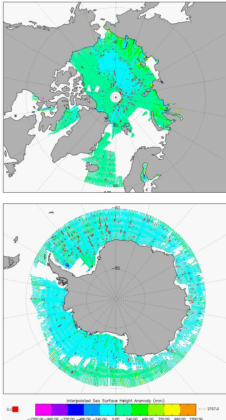
Figure 8 –Polar plots of SSHA for cycle #157.
