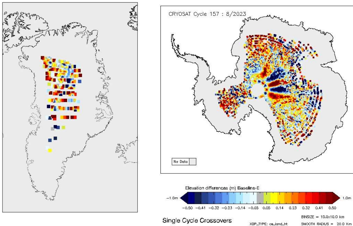
Figure 19 - Greenland and Antarctica maps of LRM elevation differences for cycle #157.
