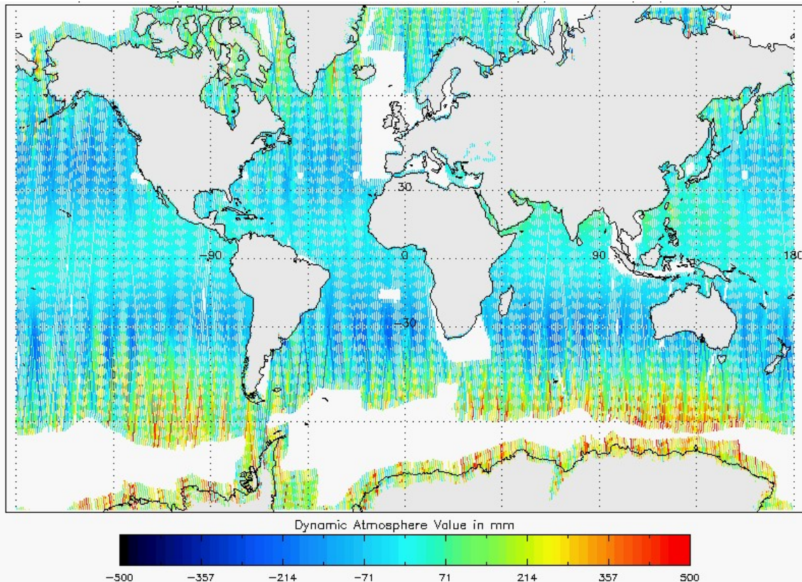
Figure 27 - Global plot of Dynamic Atmospheric Correction for cycle #157
