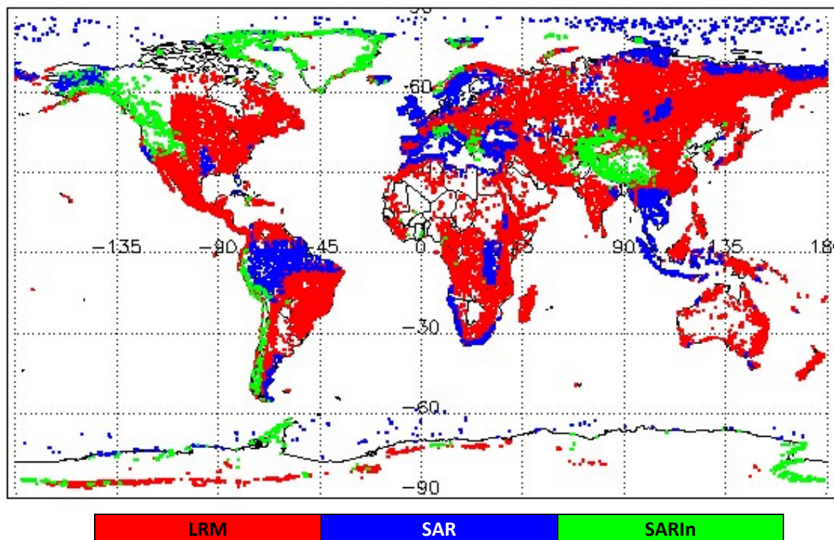
Figure 1 – Global plot showing areas of loss of track in all SIRAL modes L0 data during September 2023
