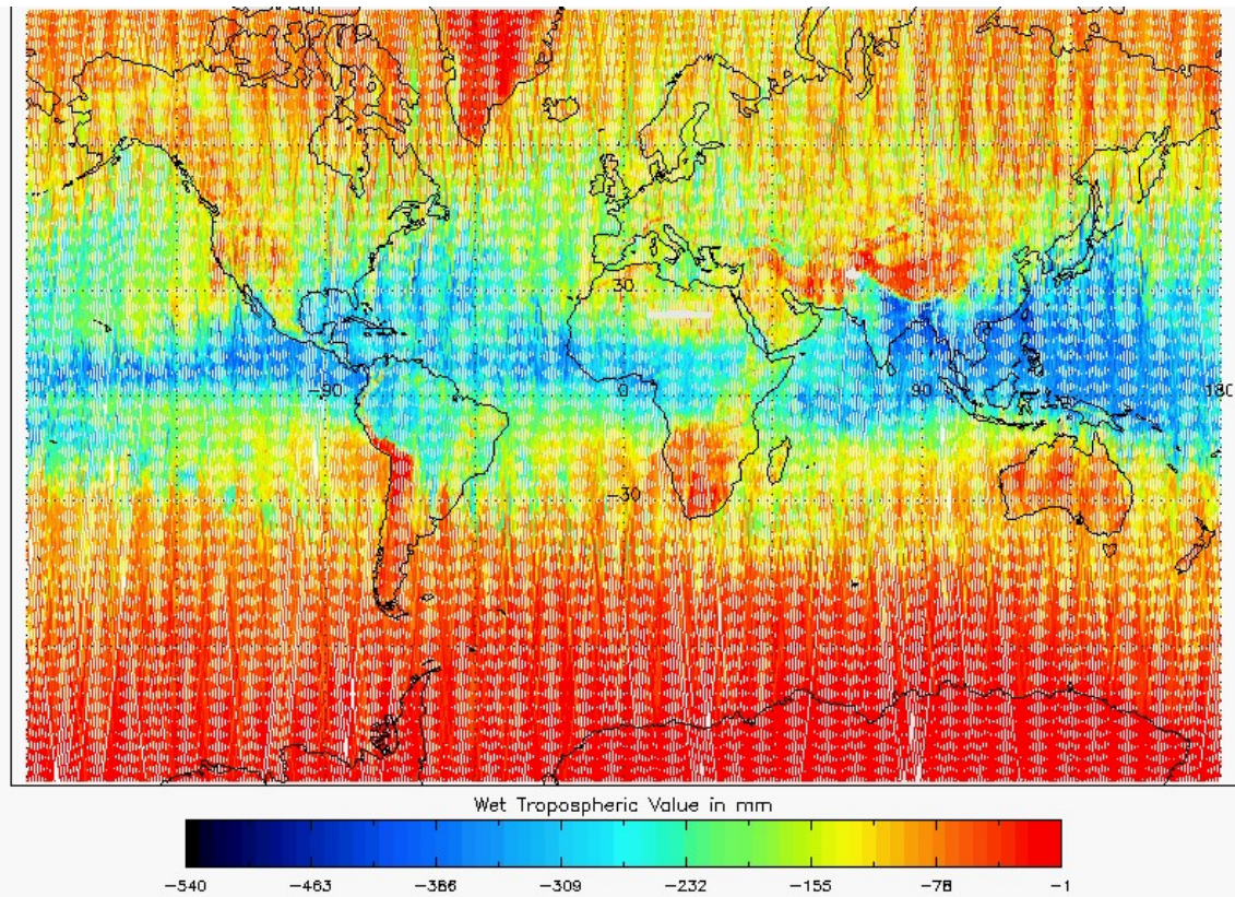
Figure 23 - Global plot of Wet Tropospheric Correction for cycle #157
