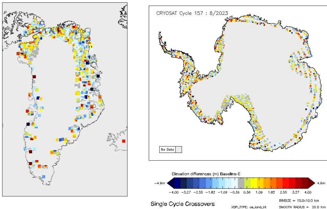
Figure 20 - Greenland and Antarctica maps of SARIn elevation differences for cycle #157.
