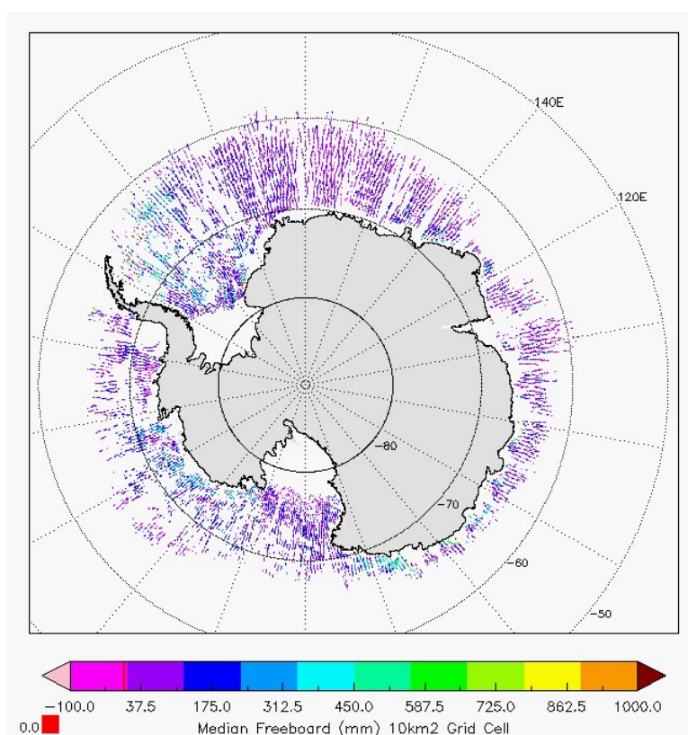
Figure 6 - Polar plots of 10km Gridded Freeboard values from L2 SAR products in cycle #157.
