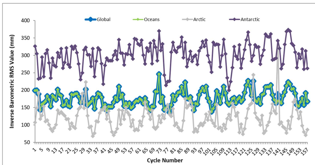
Figure 26 – Inverse Barometric Correction RMS value trend from beginning of mission
