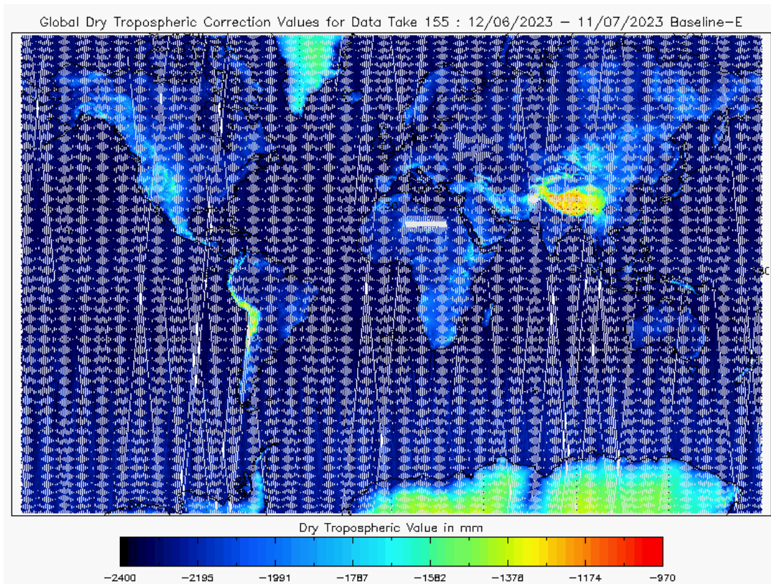
Figure 21 - Global plot of Dry Tropospheric Correction for cycle #155
