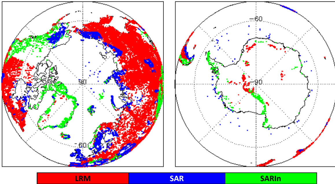
Figure 2 - Polar plots showing areas of loss of track in all SIRAL modes L0 data during July 2023.
