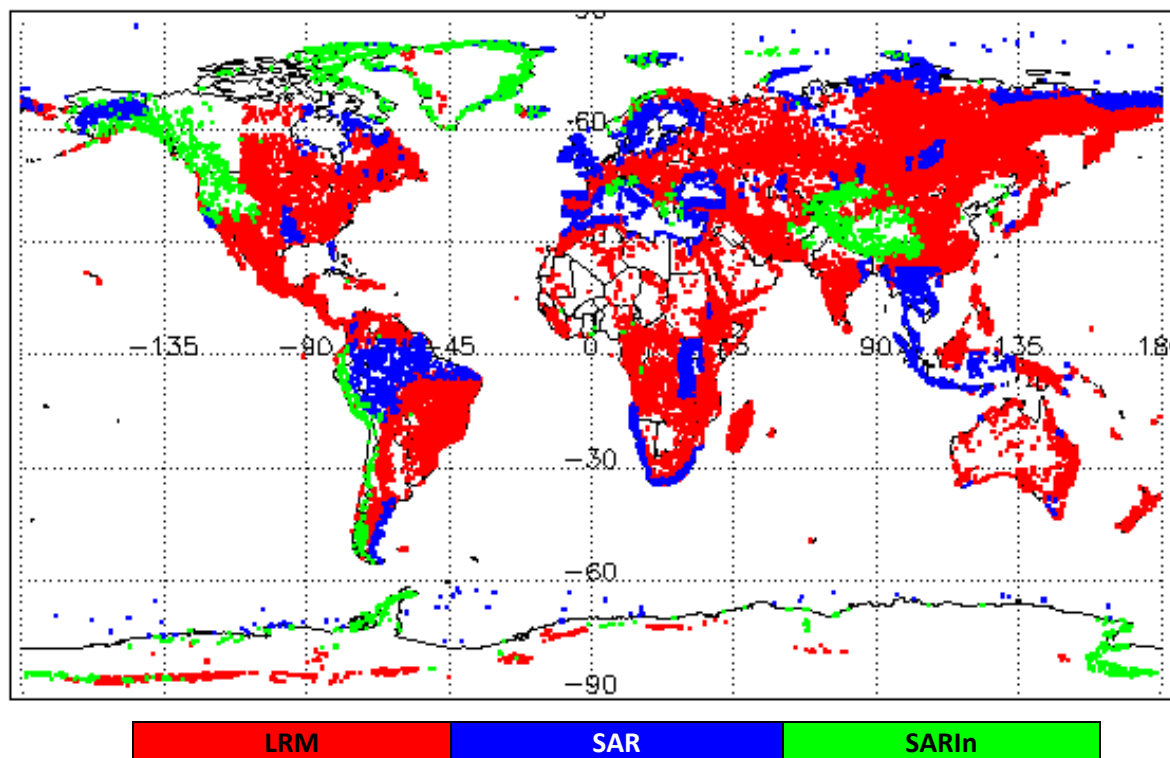
Figure 1 – Global plot showing areas of loss of track in all SIRAL modes L0 data during July 2023
