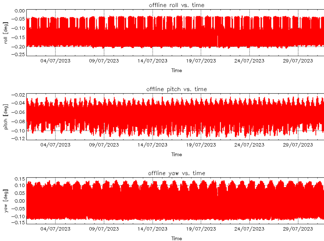
Figure 4 – Roll (top), Pitch (middle) and Yaw (bottom) values for L1B Products during cycle #155.
