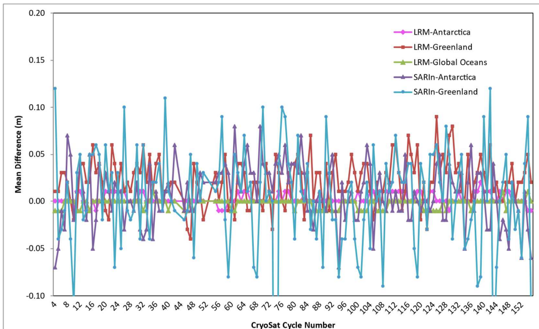
Figure 18 - Time series for Mean Difference in elevation at crossovers from beginning of the mission
