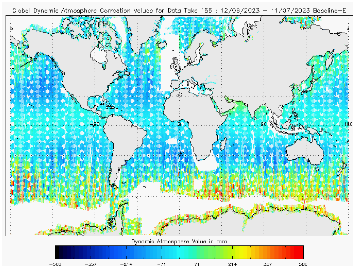
Figure 27 - Global plot of Dynamic Atmospheric Correction for cycle #155
