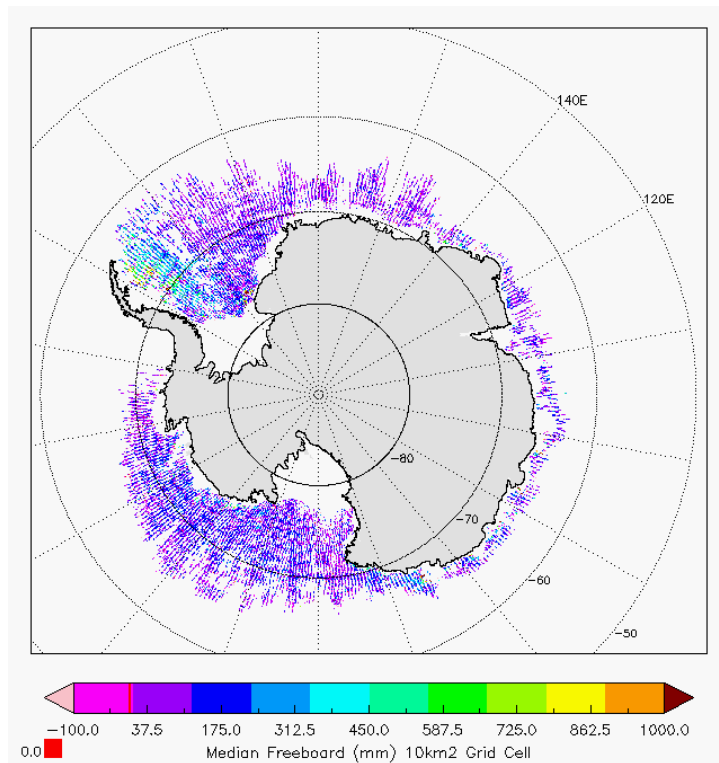
Figure 6 - Polar plots of 10km Gridded Freeboard values from L2 SAR products in cycle #155.
