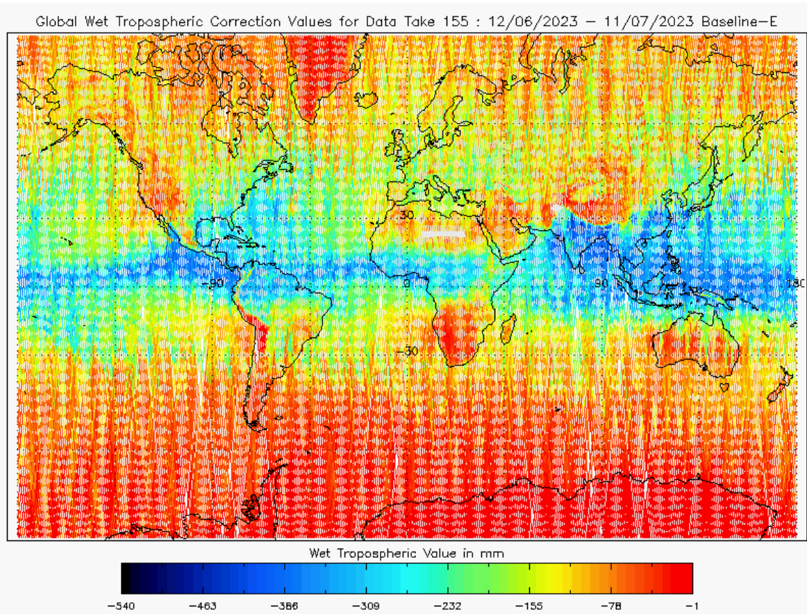
Figure 23 - Global plot of Wet Tropospheric Correction for cycle #155
