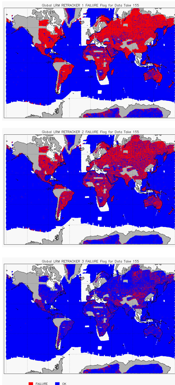
Figure 14 – Global plots showing Retracker Failure Flags for LRM mode for cycle #155:
