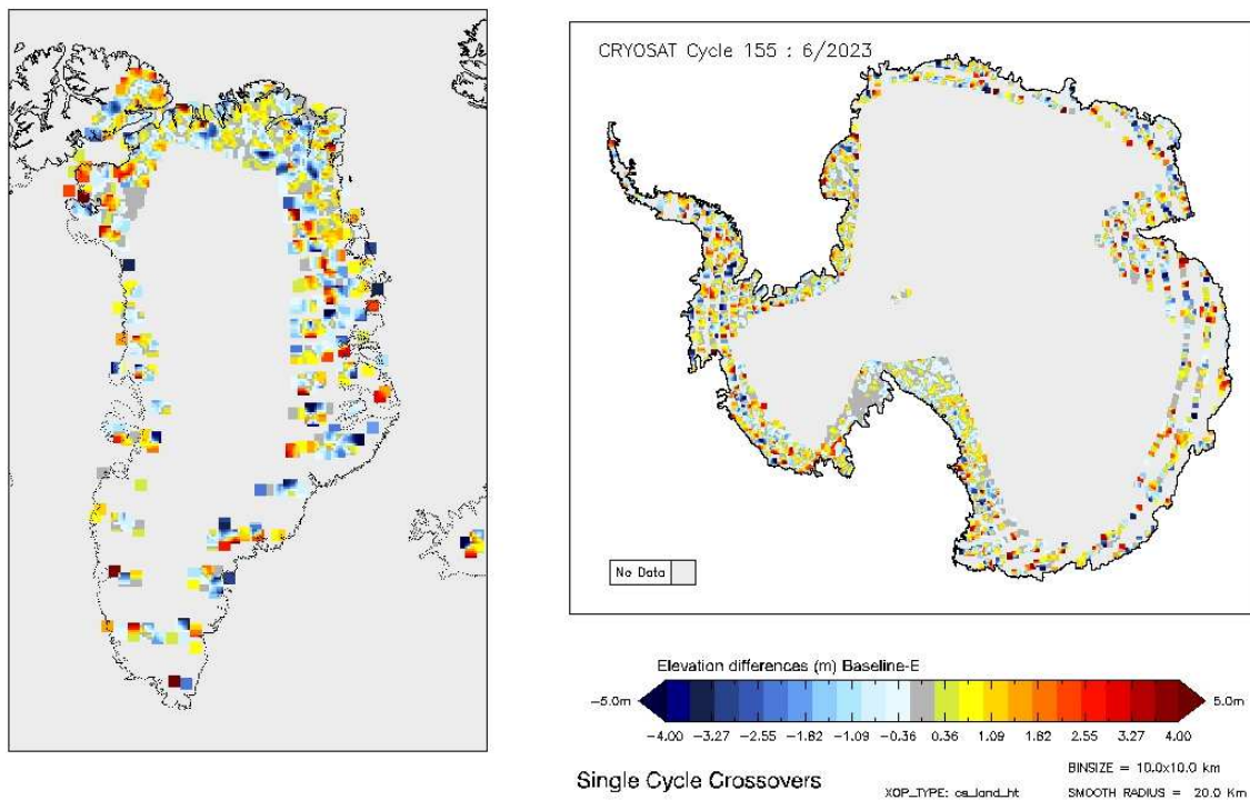
Figure 20 - Greenland and Antarctica maps of SARIn elevation differences for cycle #155.
