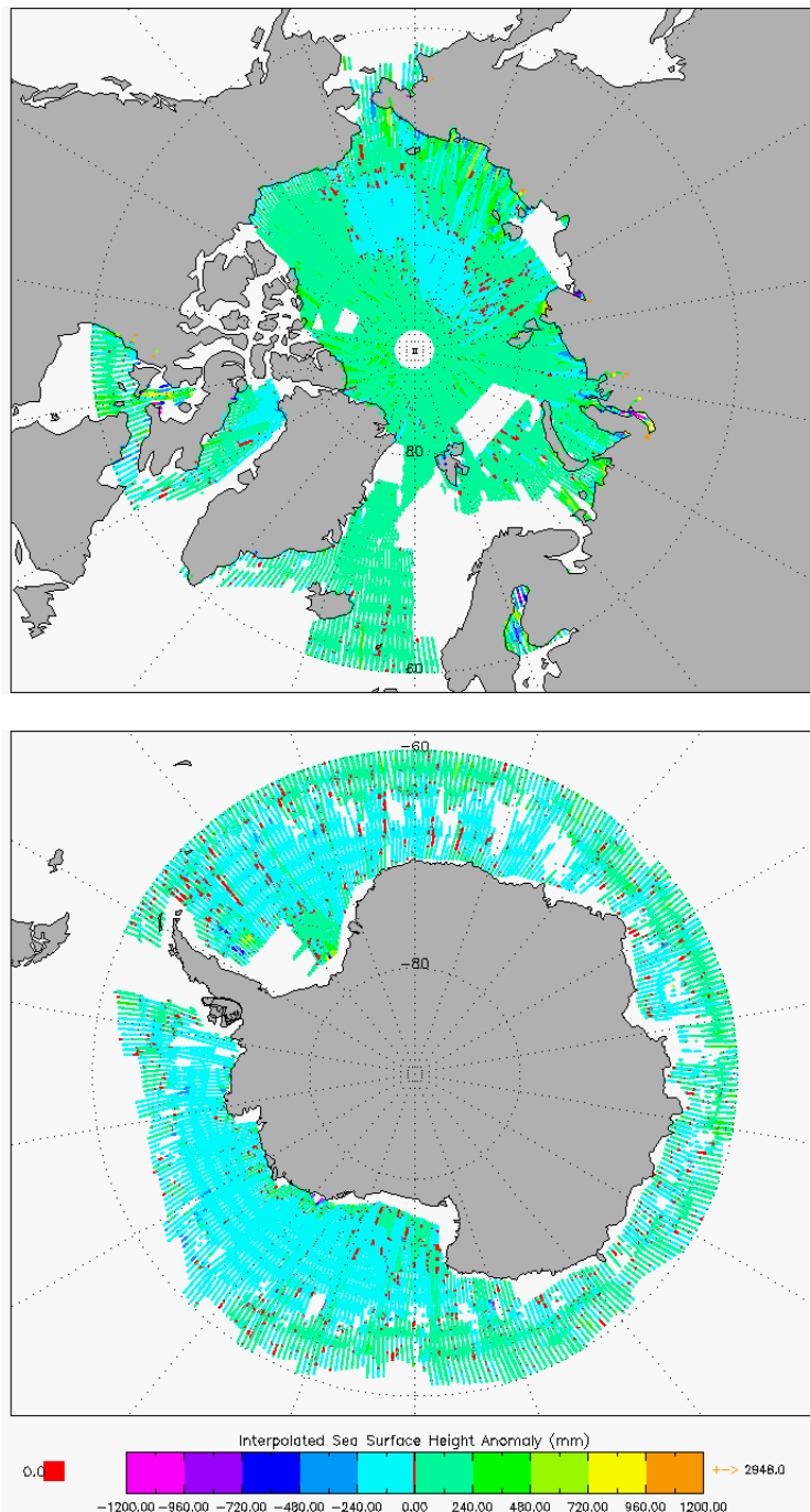
Figure 8 –Polar plots of SSHA for cycle #155.
