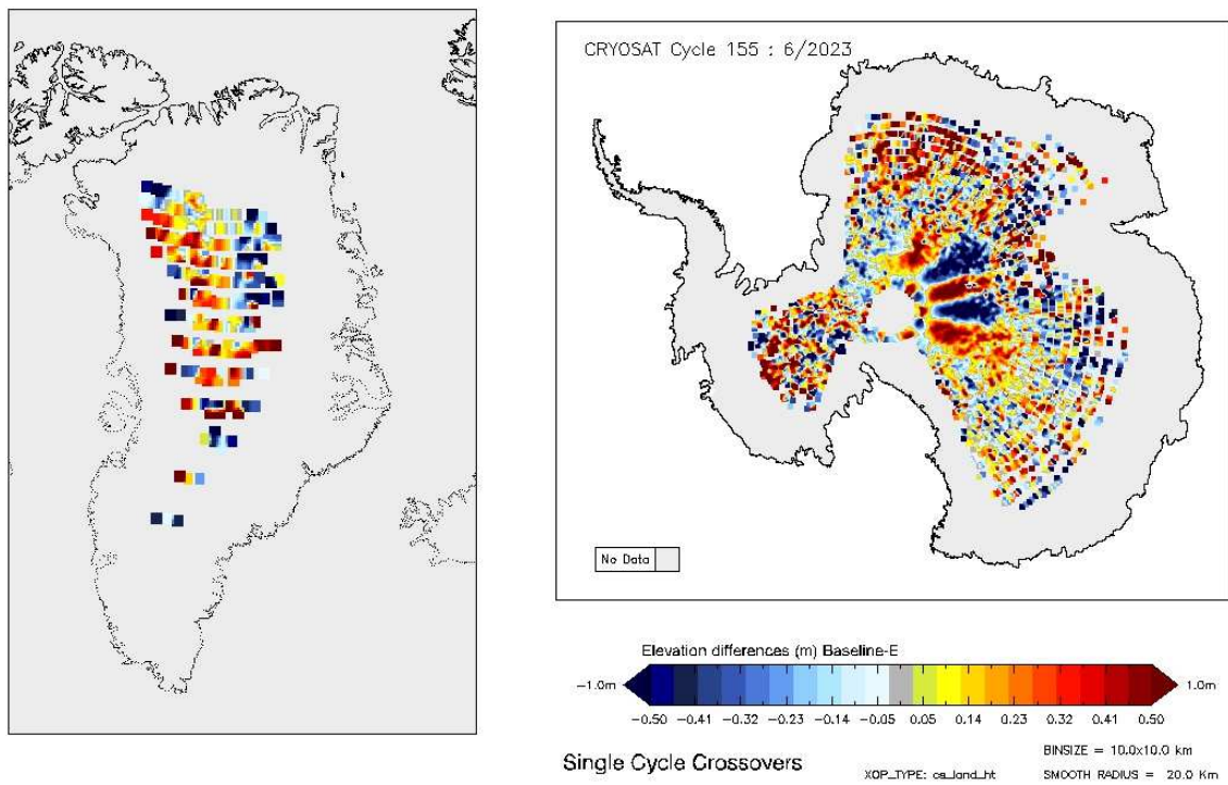
Figure 19 - Greenland and Antarctica maps of LRM elevation differences for cycle #155.
