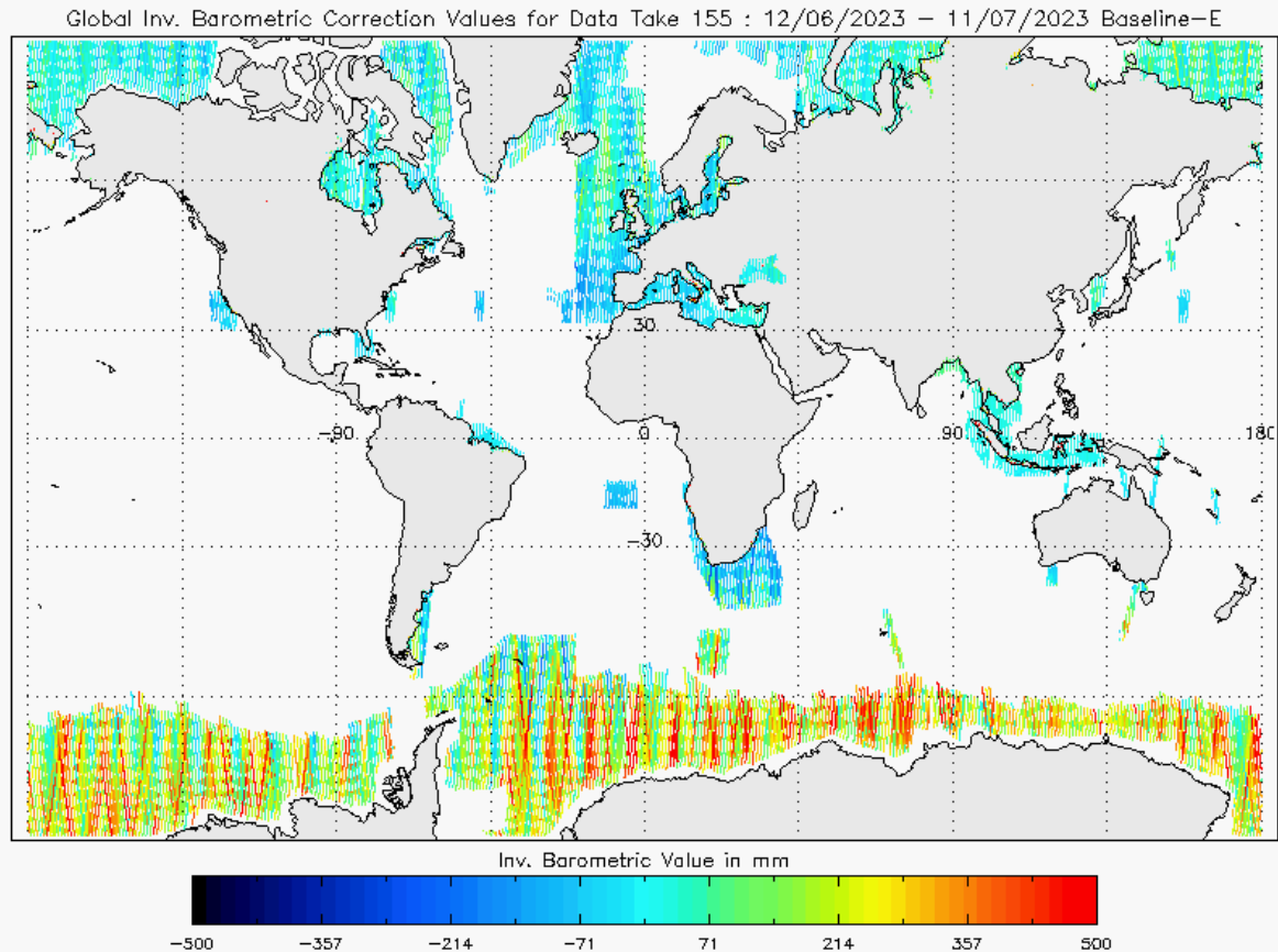
Figure 25 - Global plot of Inverse Barometric Correction for cycle #155
