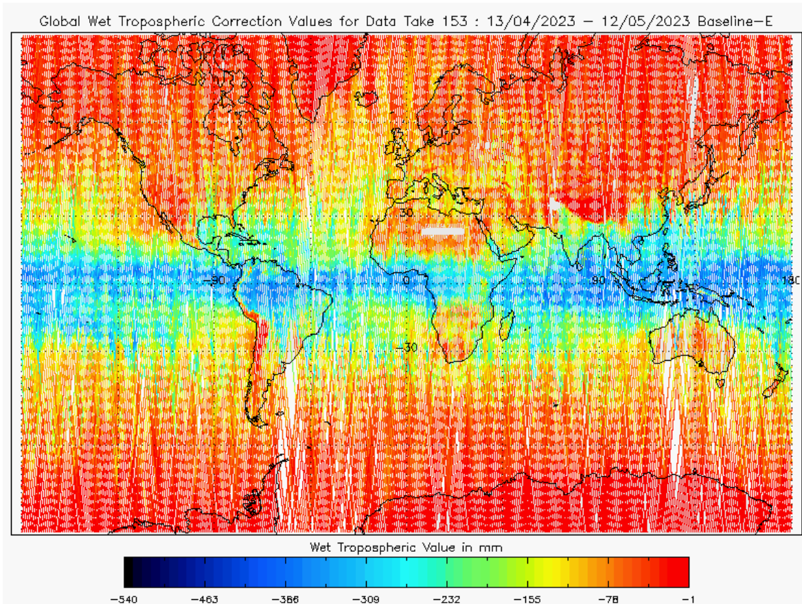
Figure 23 - Global plot of Wet Tropospheric Correction for cycle #153
