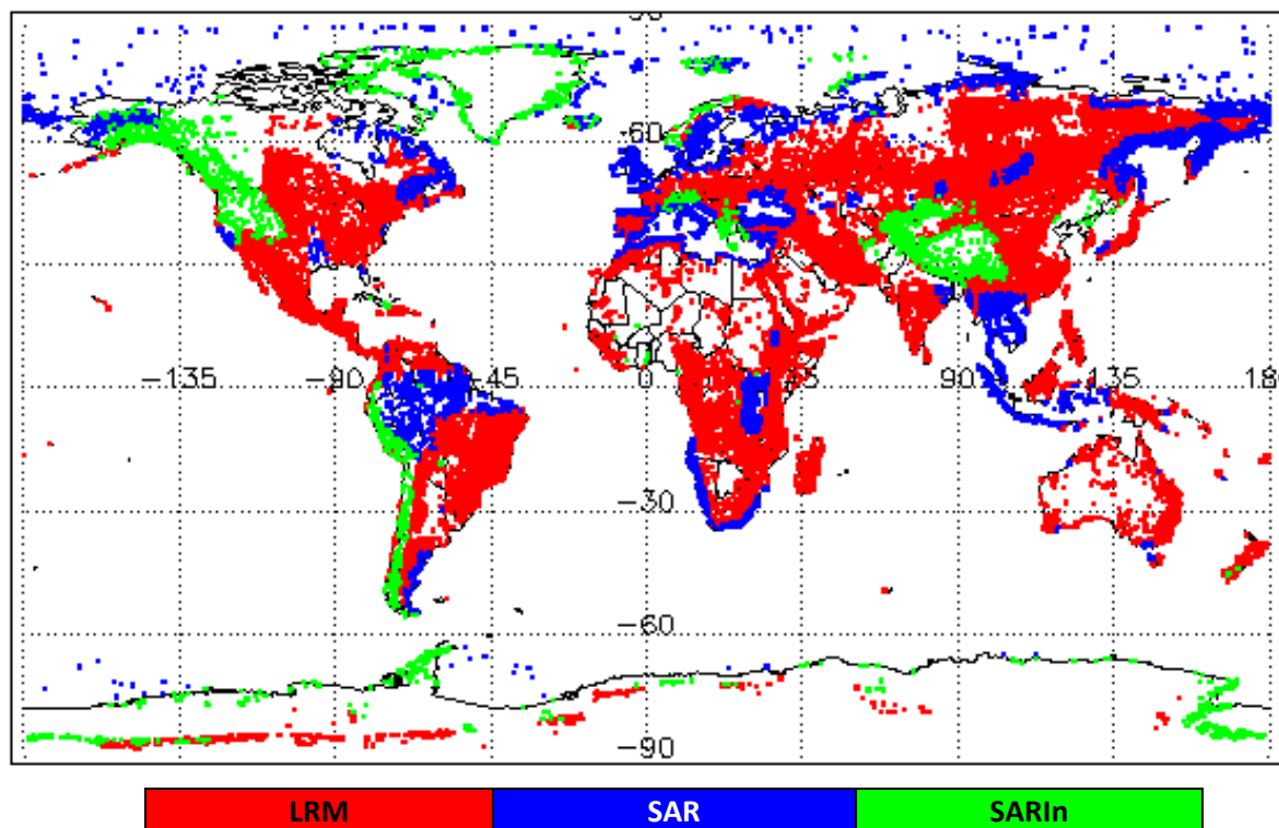
Figure 1 – Global plot showing areas of loss of track in all SIRAL modes L0 data during May 2023
