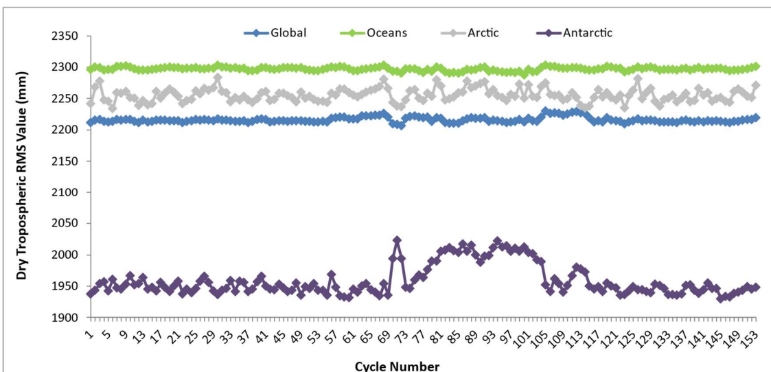
Figure 21 - Global plot of Dry Tropospheric Correction for cycle #153
