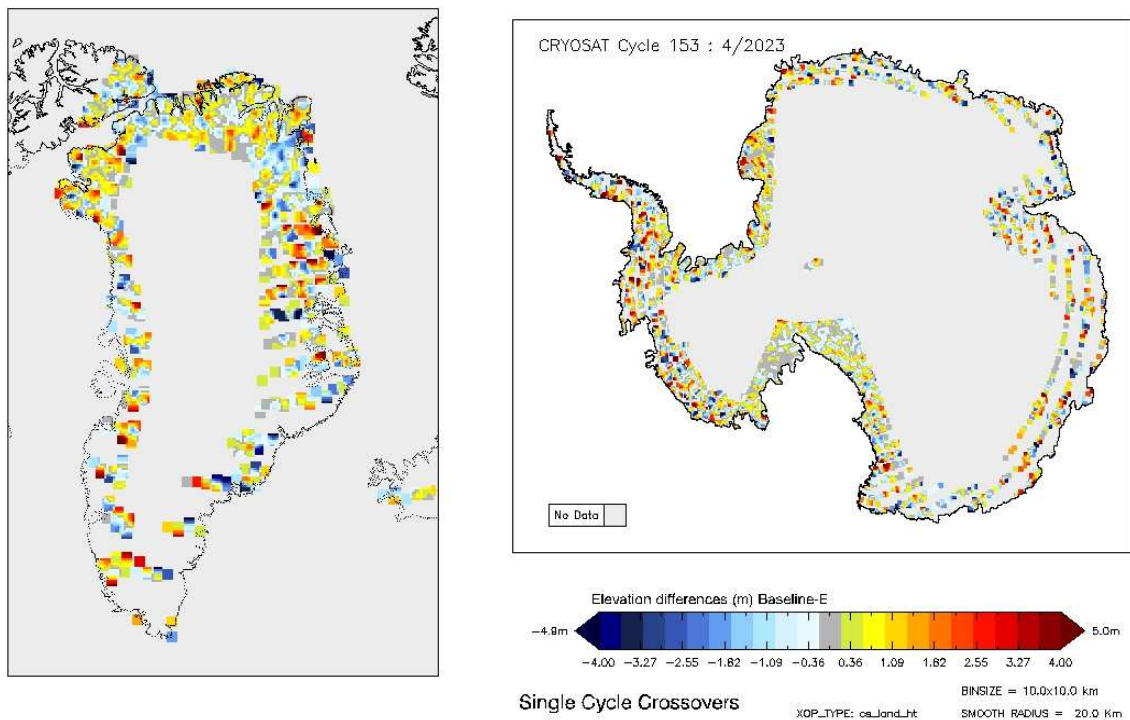
Figure 20 - Greenland and Antarctica maps of SARIn elevation differences for cycle #153.
