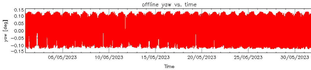
Figure 4 – Roll (top), Pitch (middle) and Yaw (bottom) values for L1B Products during cycle #153.
