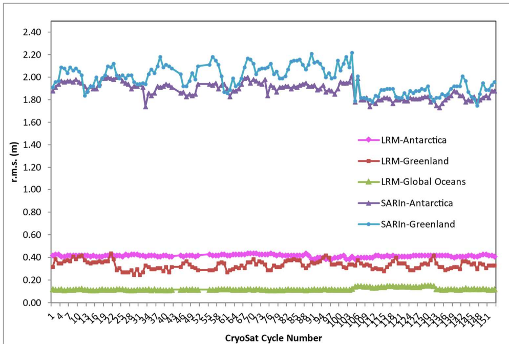
Figure 17 - Time series for crossover elevation r.m.s. values from beginning of the mission
