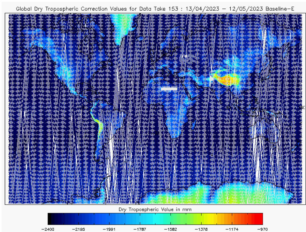
Figure 21 - Global plot of Dry Tropospheric Correction for cycle #153
