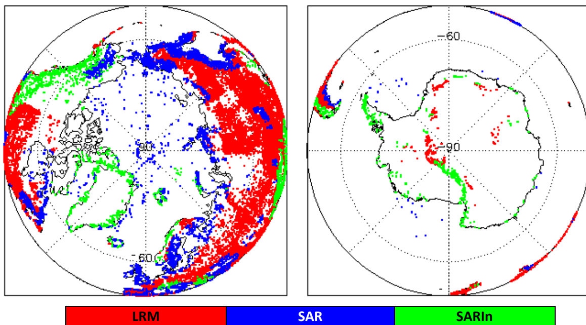
Figure 2 - Polar plots showing areas of loss of track in all SIRAL modes L0 data during May 2023.
