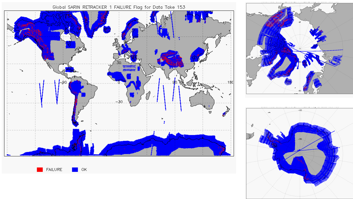
Figure 16 – Global plots showing Retracker Failure Flags for SARIn mode for cycle #153
