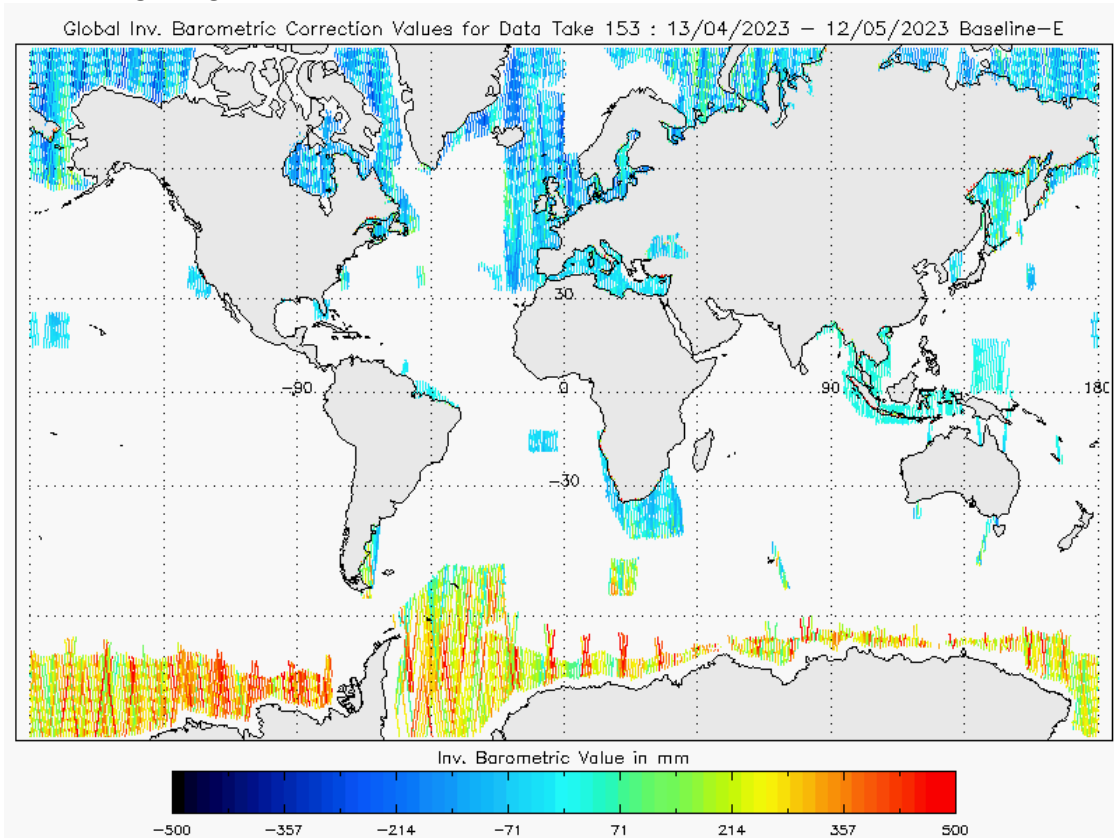
Figure 25 - Global plot of Inverse Barometric Correction for cycle #153
