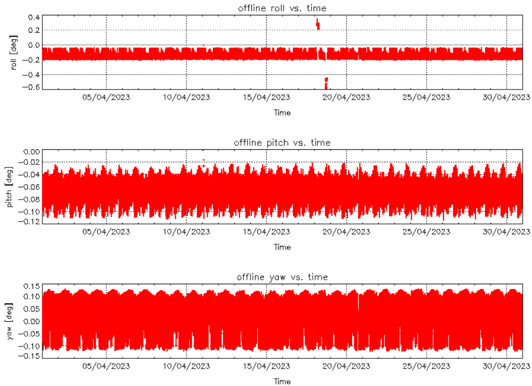
Figure 4 – Roll (top), Pitch (middle) and Yaw (bottom) values for L1B Products during cycle #152.
