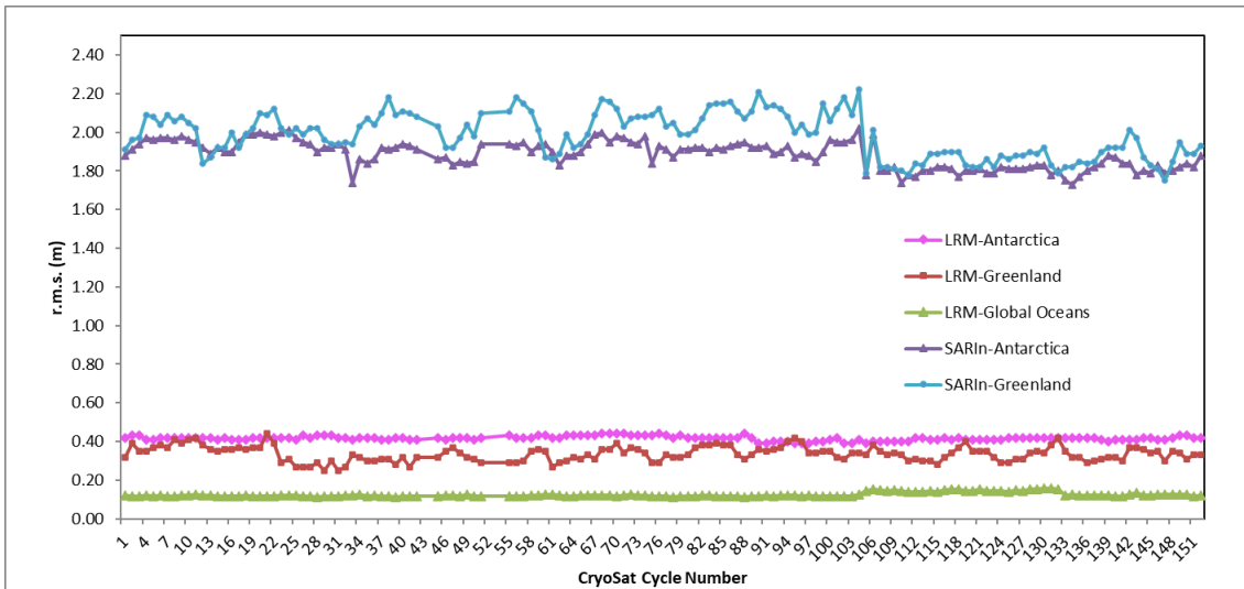
Figure 17 - Time series for crossover elevation r.m.s values from beginning of the mission
