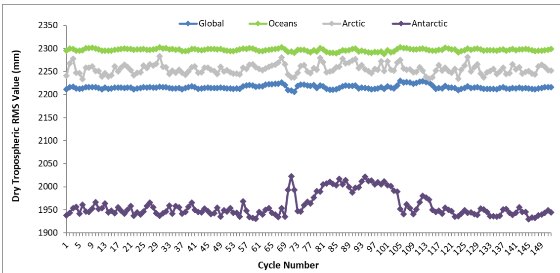
Figure 22 - Dry Tropospheric Correction RMS value trend from beginning of mission
