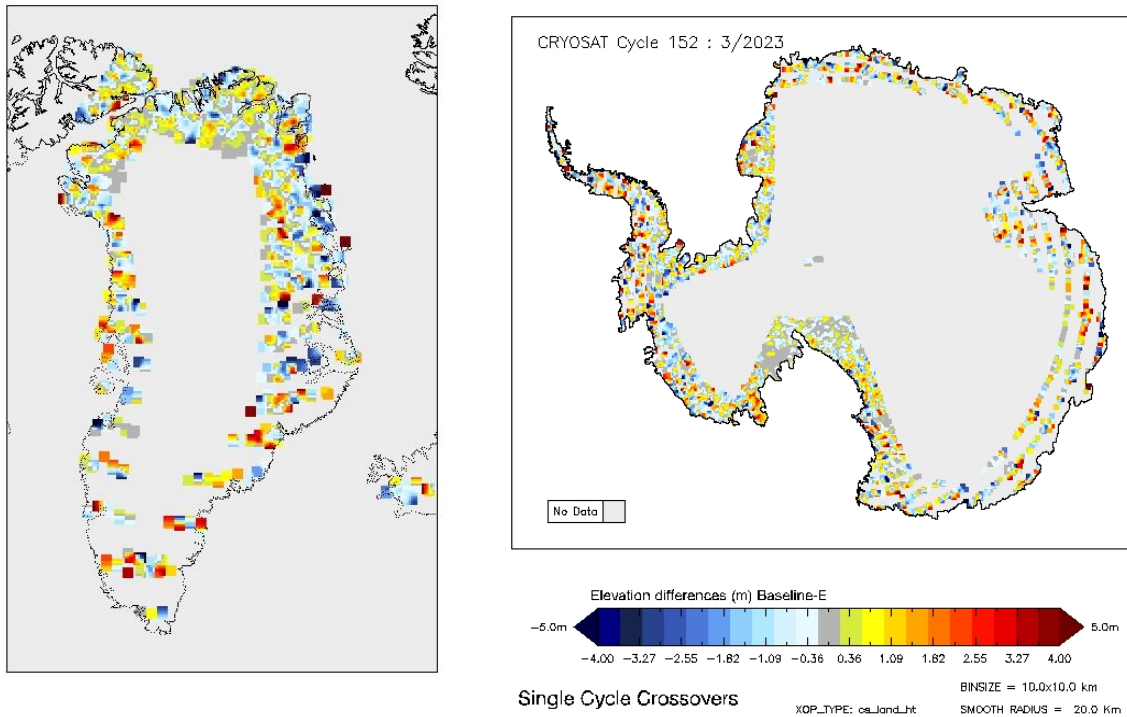
Figure 20 - Greenland and Antarctica maps of SARIn elevation differences for cycle #152.
