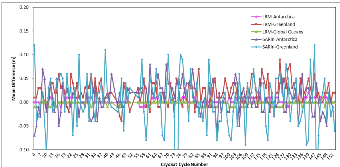
Figure 18 - Time series for Mean Difference in elevation at crossovers from beginning of the mission
