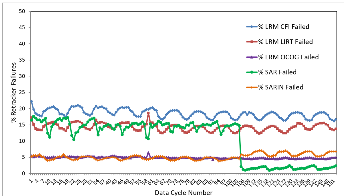
Figure 13 – Time Series for Retracker Failure Flags
