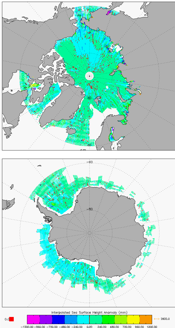
Figure 8 –Polar plots of SSHA for cycle #152.
