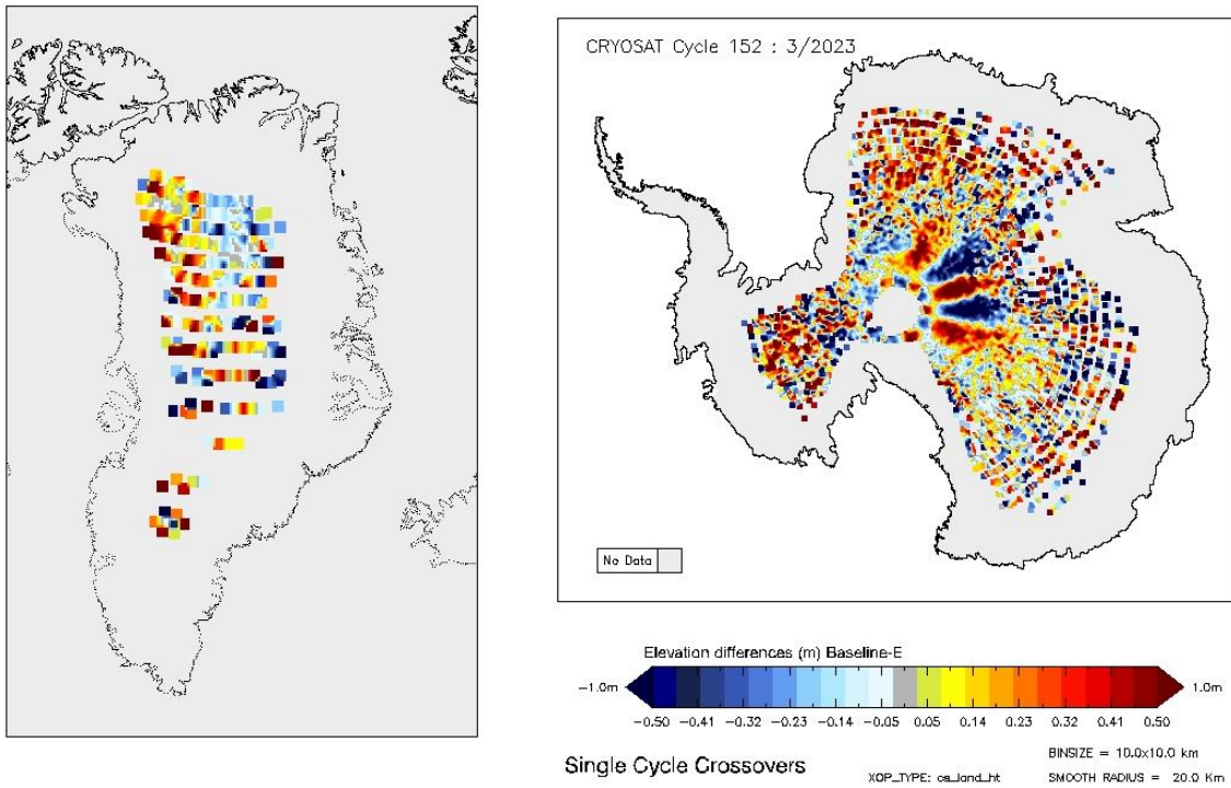
Figure 19 - Greenland and Antarctica maps of LRM elevation differences for cycle #152.
