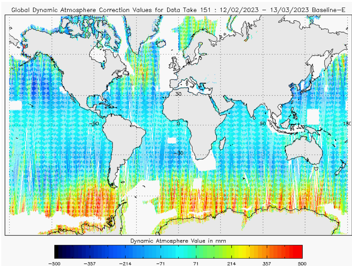
Figure 27 - Global plot of Dynamic Atmospheric Correction for cycle #151
