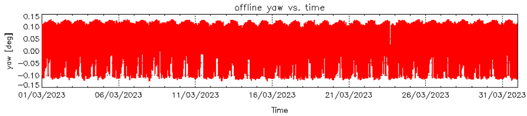
Figure 4 – Roll (top), Pitch (middle) and Yaw (bottom) values for L1B Products during cycle #151.
