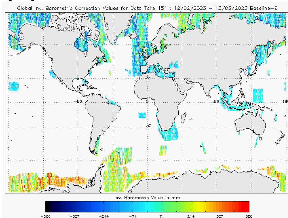
Figure 25 - Global plot of Inverse Barometric Correction for cycle #151
