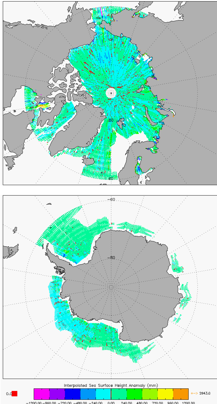
Figure 8 –Polar plots of SSHA for cycle #151.
