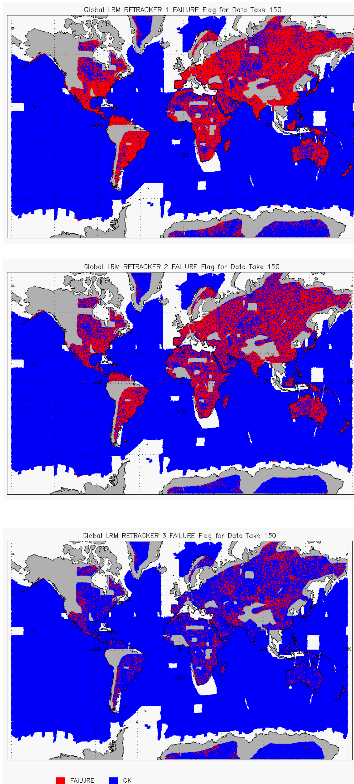
Figure 14 – Global plots showing Retracker Failure Flags for LRM mode for cycle #150:
