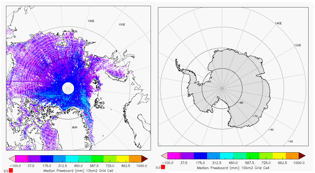
Figure 6 - Polar plots of 10km Gridded Freeboard values from L2 SAR products in cycle #150.
