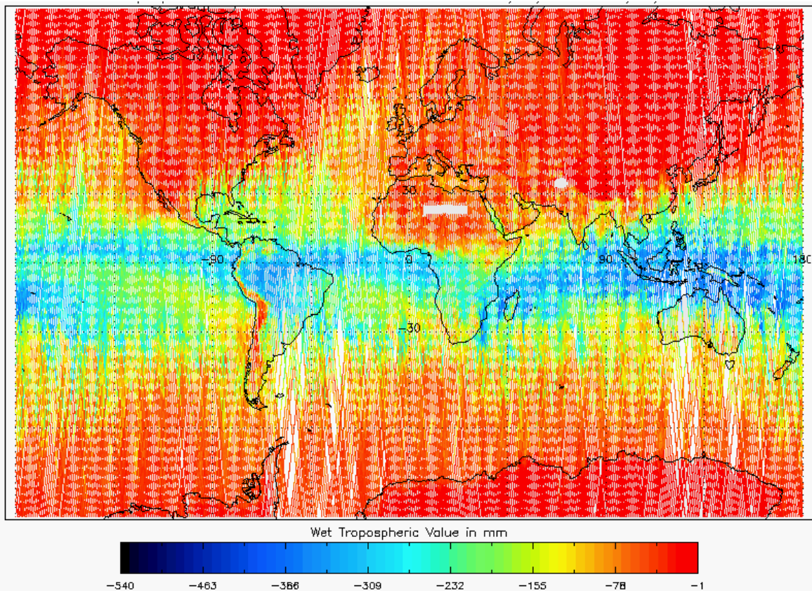
Figure 23 - Global plot of Wet Tropospheric Correction for cycle #150
