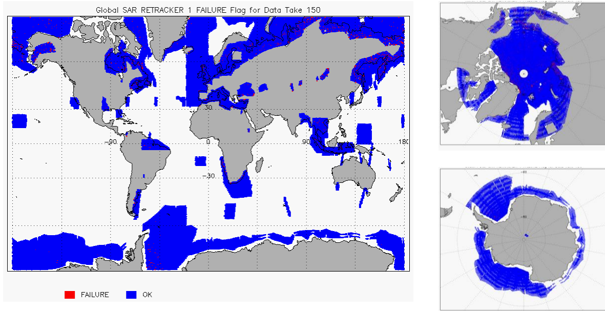
Figure 15 - Global plots showing Retracker Failure Flags for SAR mode for cycle #150
