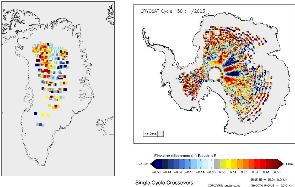
Figure 19 - Greenland and Antarctica maps of LRM elevation differences for cycle #150.
