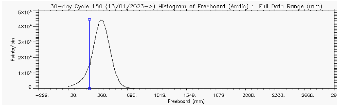
Figure 5 – Histogram of Freeboard for Arctic (above) and Antarctic (below) for cycle #150
