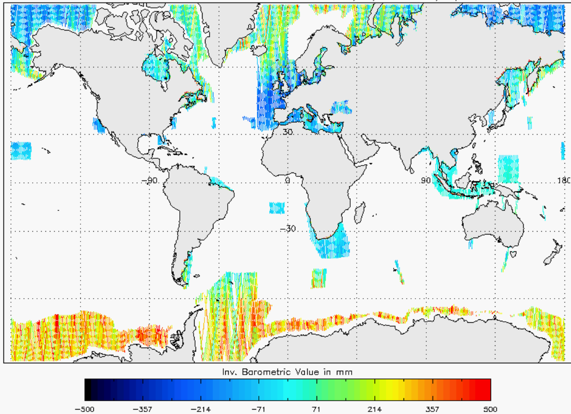
Figure 25 - Global plot of Inverse Barometric Correction for cycle #150
