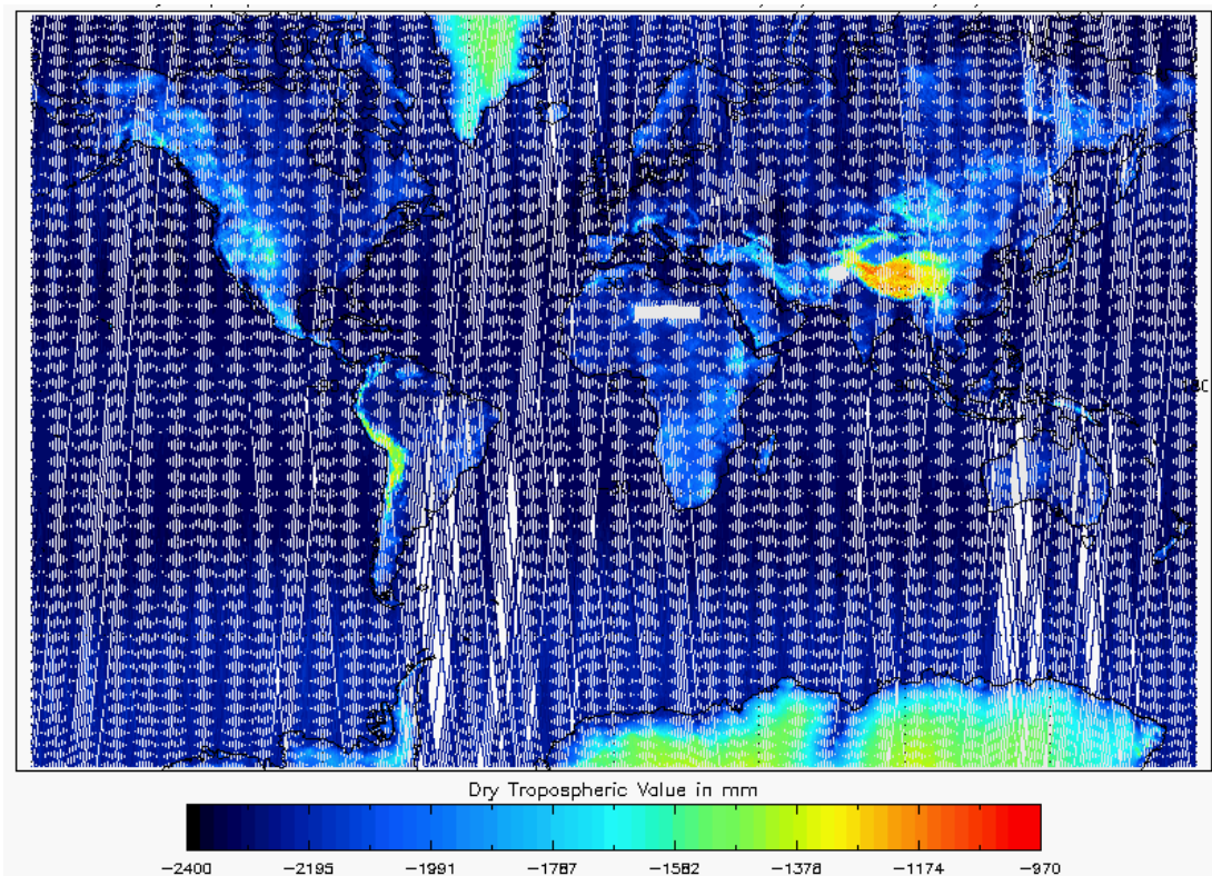
Figure 21 - Global plot of Dry Tropospheric Correction for cycle #150
