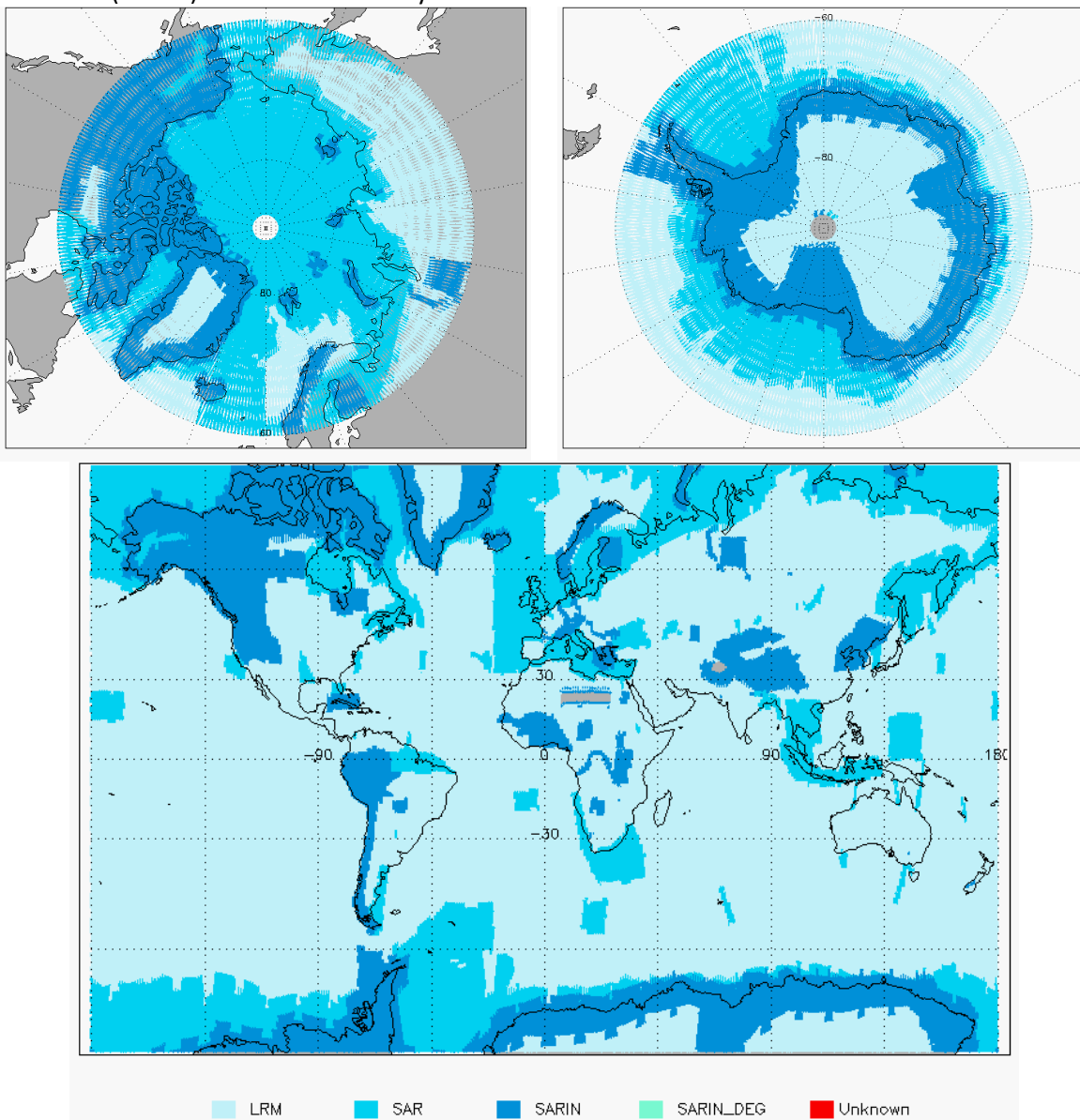
Figure 3 - Global and Polar plots of SIRAL Modes for cycle #150.
