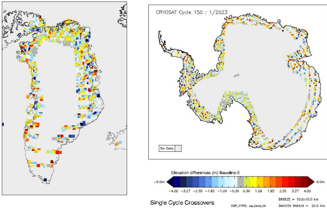
Figure 20 - Greenland and Antarctica maps of SARIn elevation differences for cycle #150.
