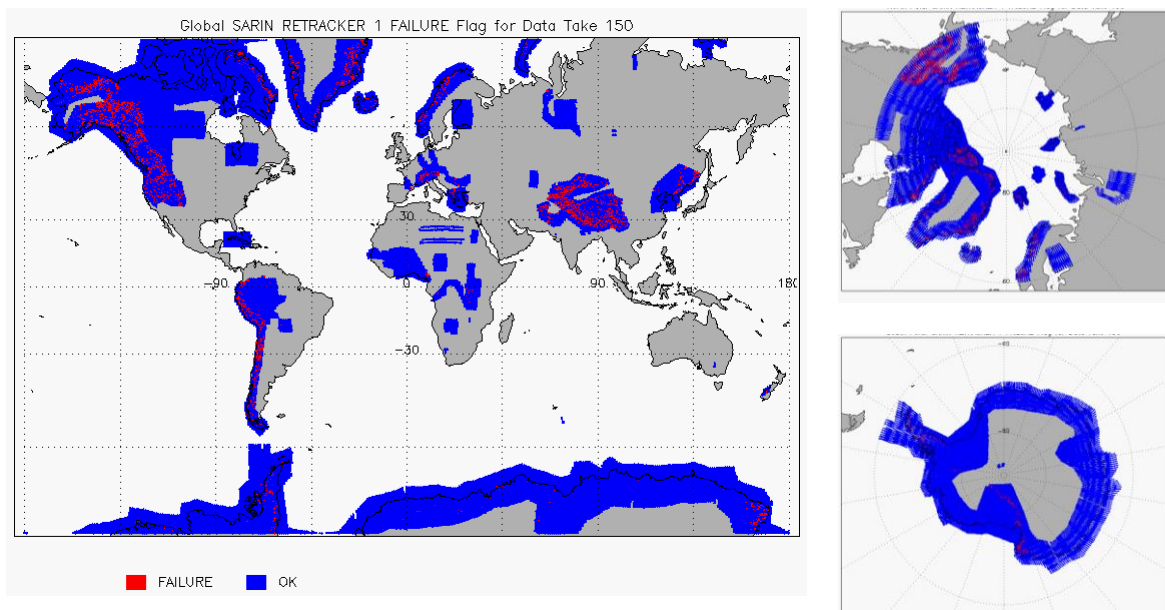
Figure 16 – Global plots showing Retracker Failure Flags for SARIn mode for cycle #150
