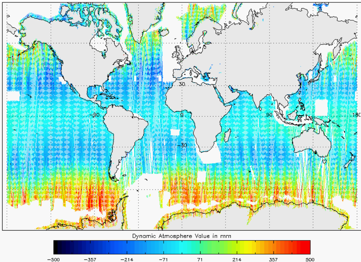
Figure 27 - Global plot of Dynamic Atmospheric Correction for cycle #150
