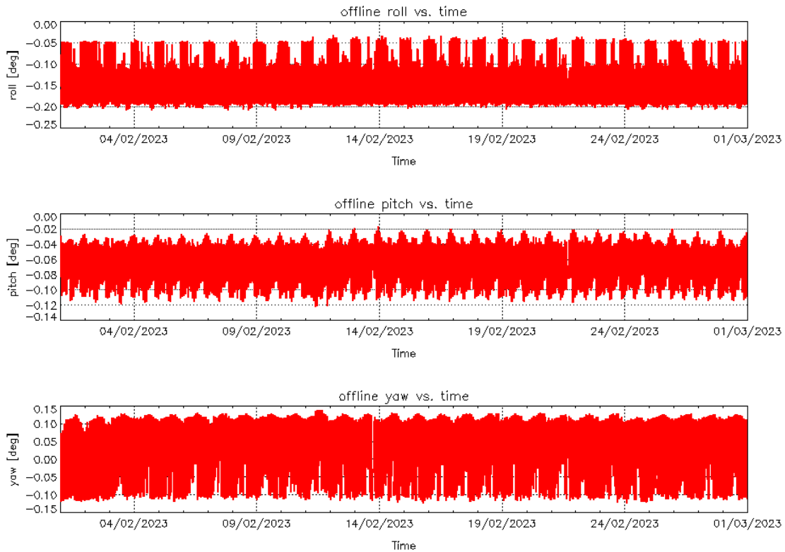
Figure 4 – Roll (top), Pitch (middle) and Yaw (bottom) values for L1B Products during cycle #150.
