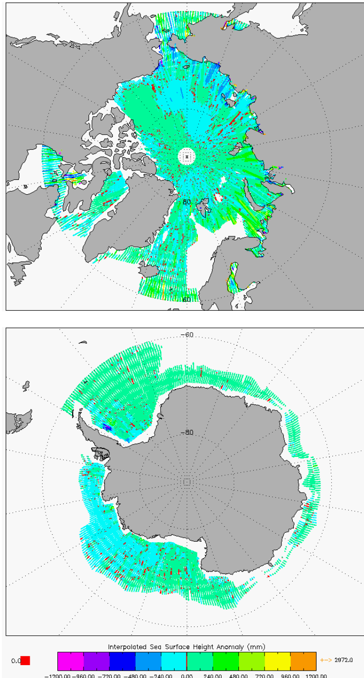
Figure 8 –Polar plots of SSHA for cycle #150.
