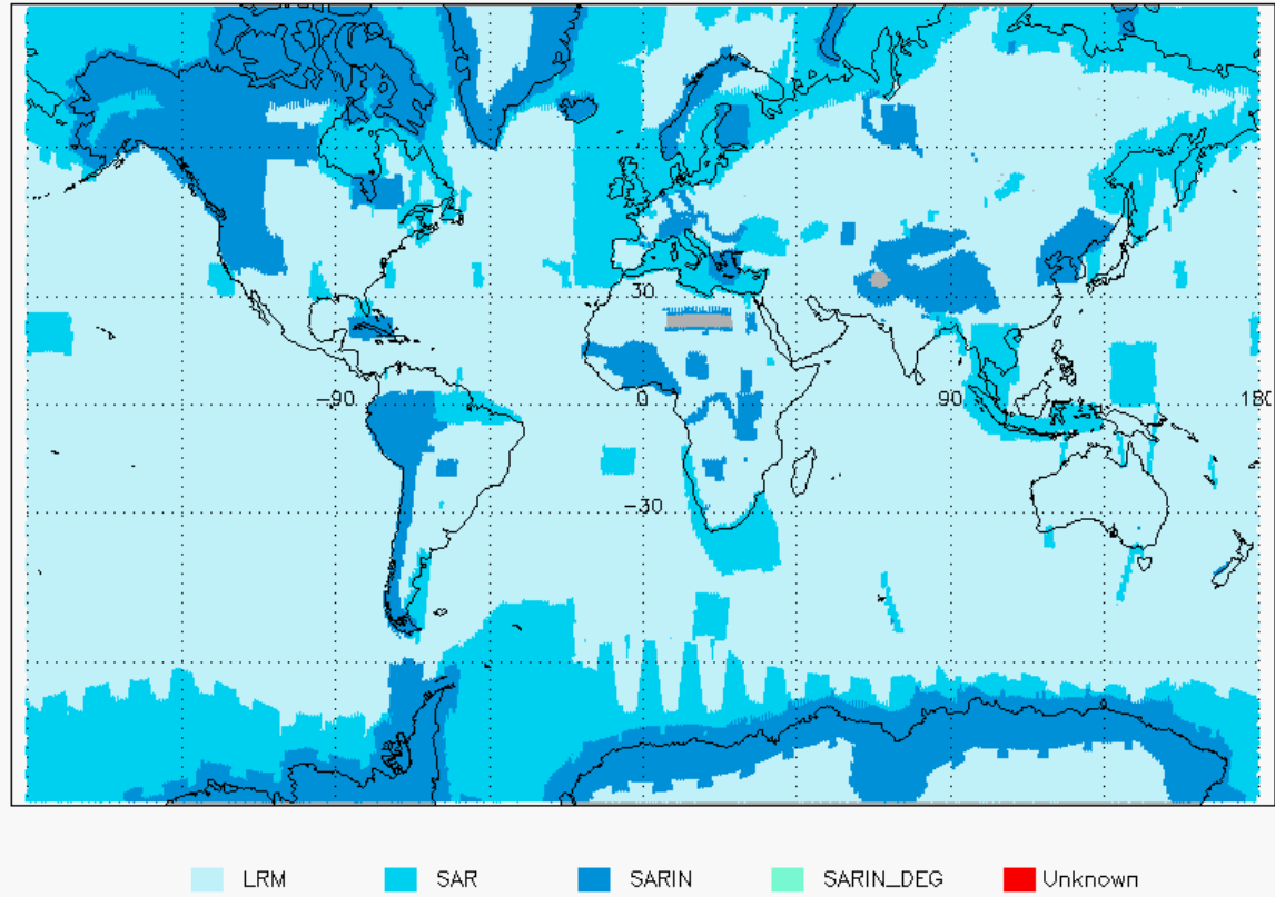
Figure 3 - Global and Polar plots of SIRAL Modes for cycle #149.
