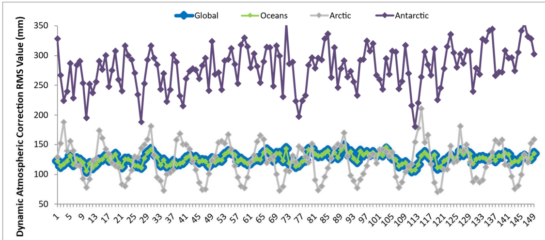
Figure 28 – Dynamic Atmospheric Correction RMS value trend from beginning of mission
