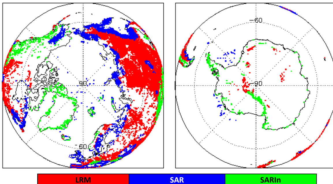
Figure 2 - Polar plots showing areas of loss of track in all SIRAL modes L0 data during January 2023.
