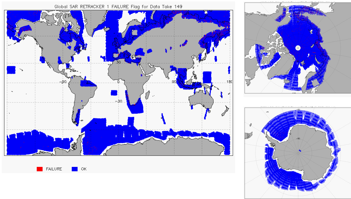
Figure 15 - Global plots showing Retracker Failure Flags for SAR mode for cycle #149
