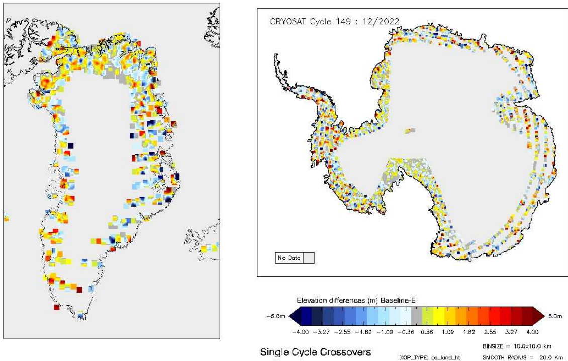
Figure 20 - Greenland and Antarctica maps of SARIn elevation differences for cycle #149.
