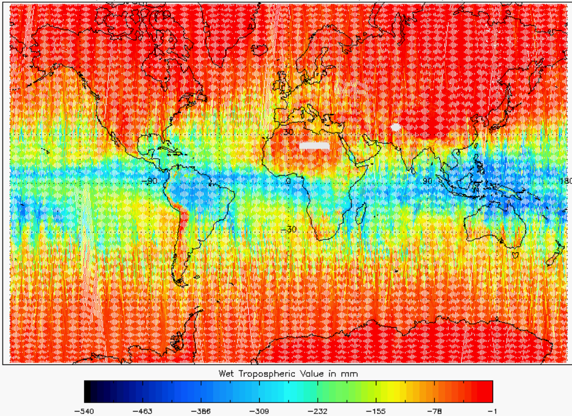
Figure 23 - Global plot of Wet Tropospheric Correction for cycle #149
