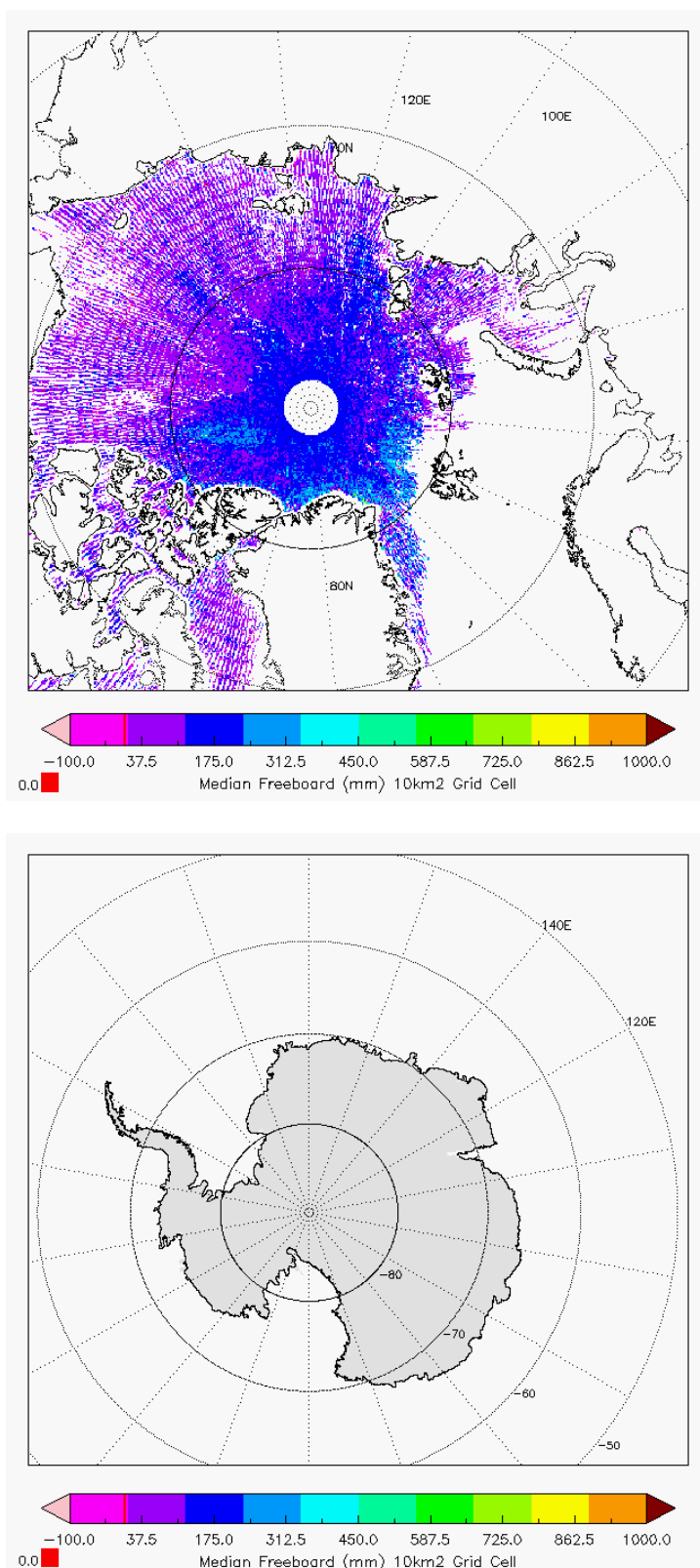
Figure 6 - Polar plots of 10km Gridded Freeboard values from L2 SAR products in cycle #149.
