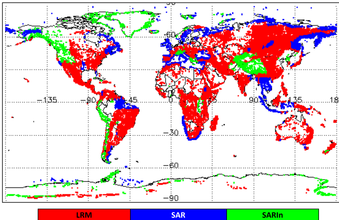
Figure 1 – Global plot showing areas of loss of track in all SIRAL modes L0 data during January 2023
