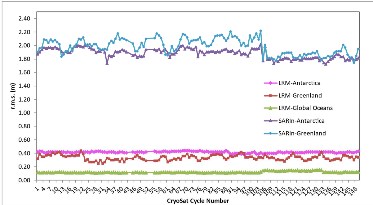
Figure 17 - Time series for crossover elevation r.m.s values from beginning of the mission
