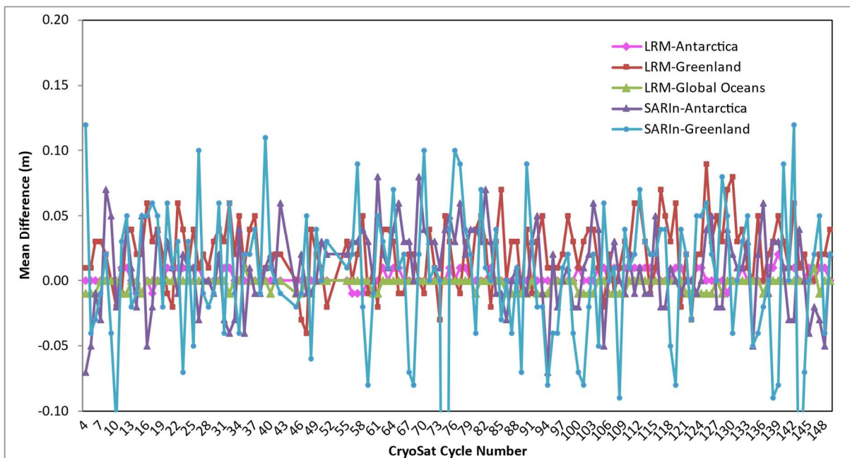
Figure 18 - Time series for Mean Difference in elevation at crossovers from beginning of the mission
