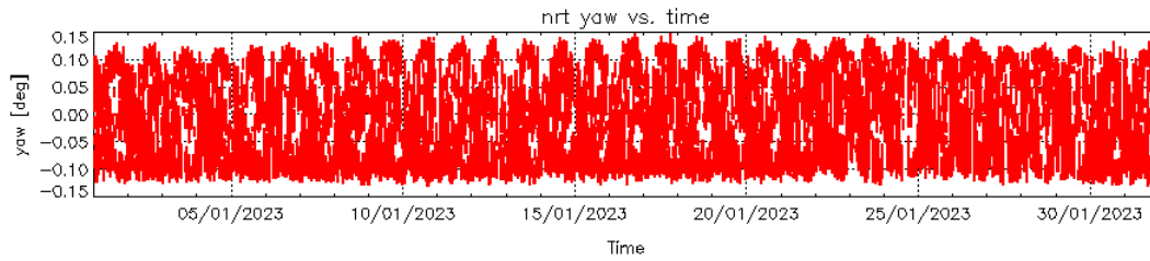
Figure 4 – Roll (top), Pitch (middle) and Yaw (bottom) values for L1B Products during cycle #149.
