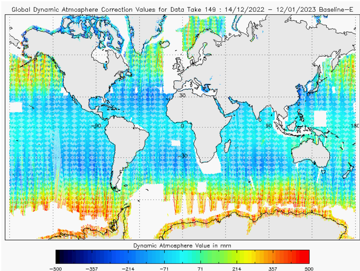
Figure 27 - Global plot of Dynamic Atmospheric Correction for cycle #149
