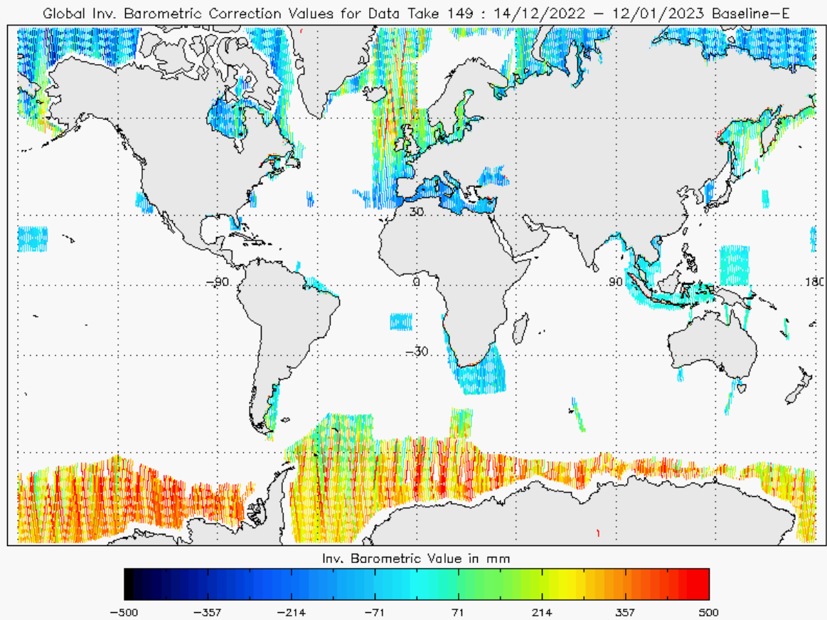
Figure 25 - Global plot of Inverse Barometric Correction for cycle #149
