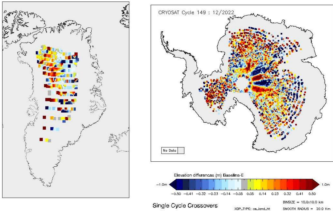
Figure 19 - Greenland and Antarctica maps of LRM elevation differences for cycle #149.
