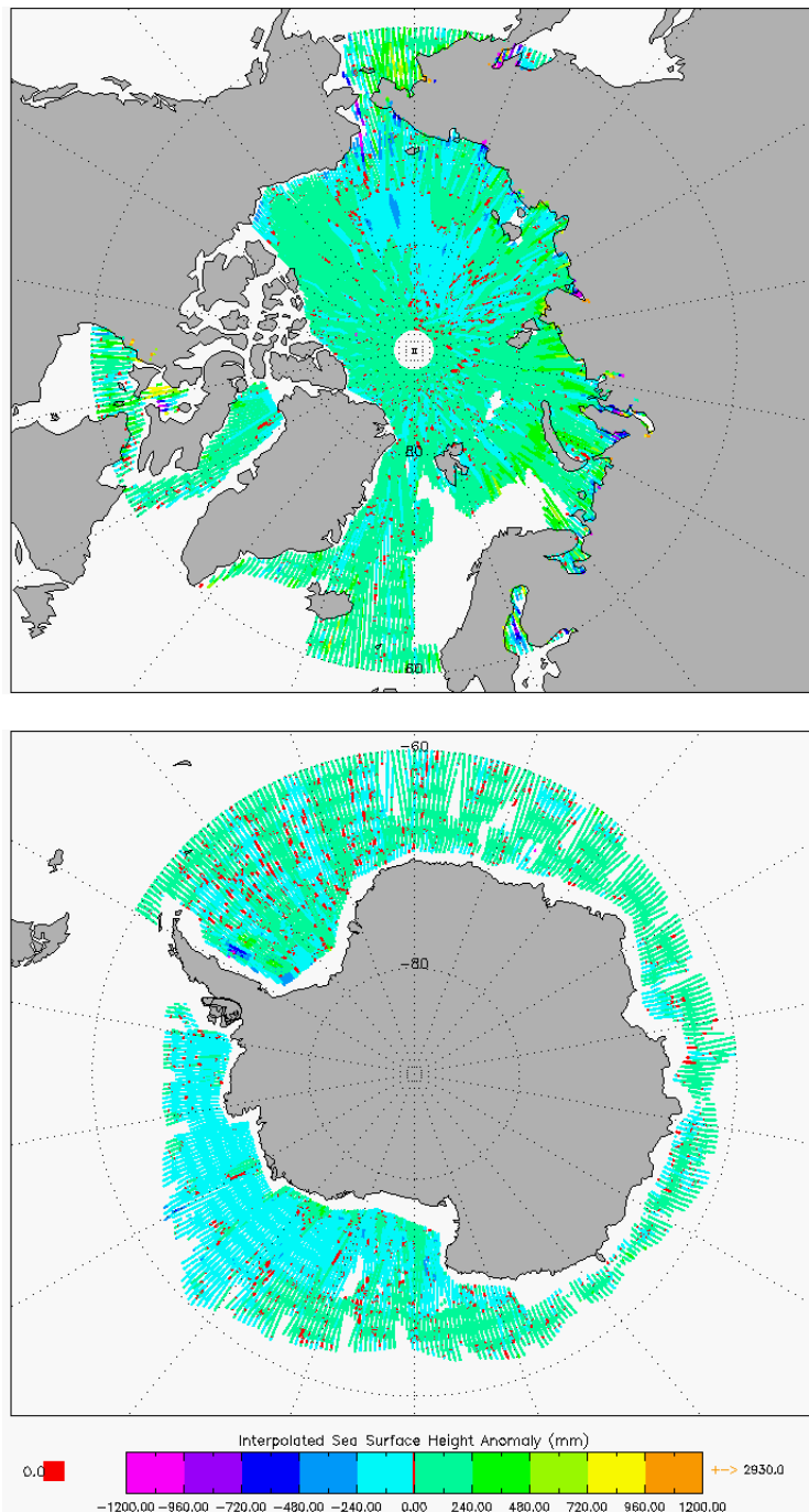
Figure 8 –Polar plots of SSHA for cycle #149.
