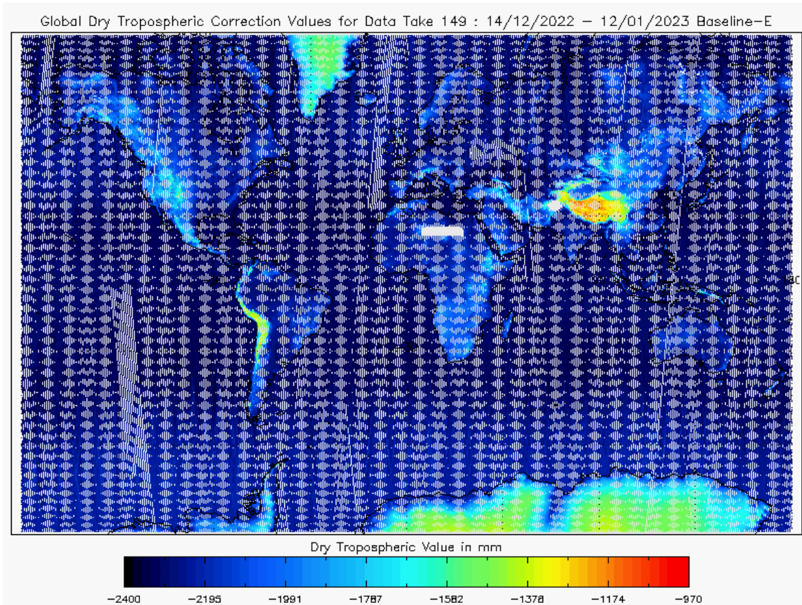
Figure 21 - Global plot of Dry Tropospheric Correction for cycle #149
