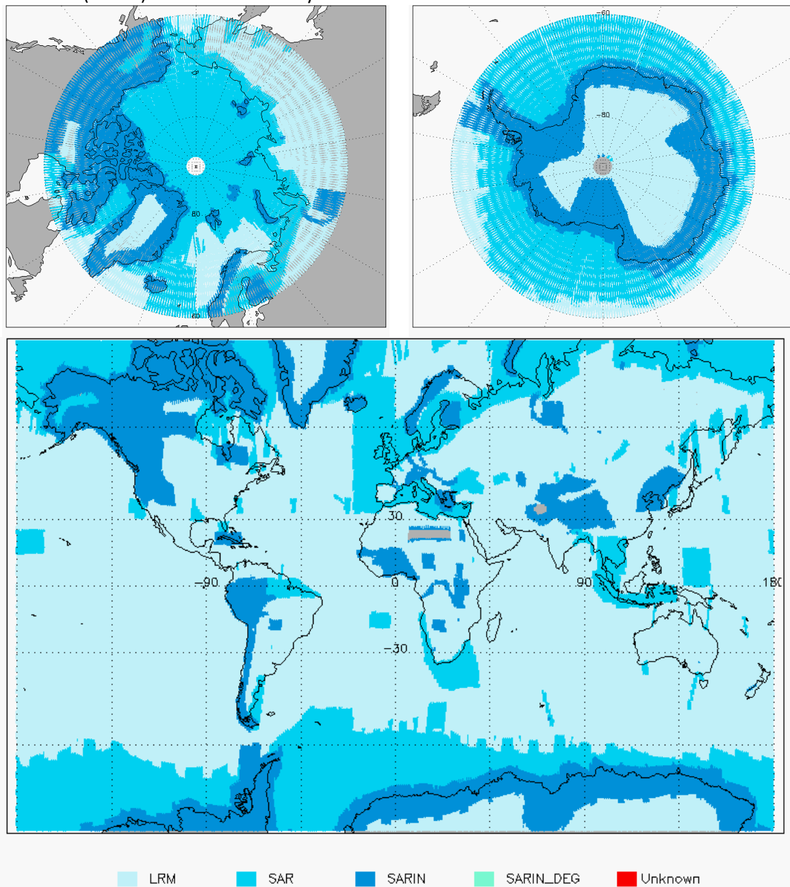
Figure 3 - Global and Polar plots of SIRAL Modes for cycle #148.
