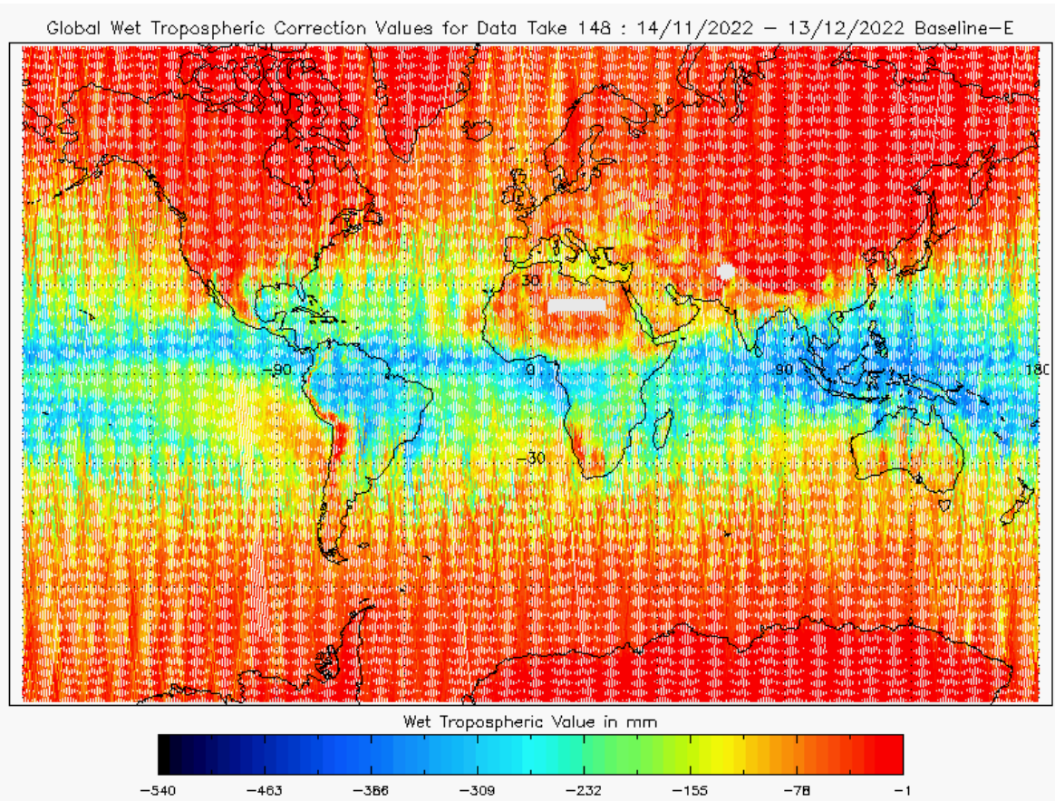
Figure 23 - Global plot of Wet Tropospheric Correction for cycle #148
