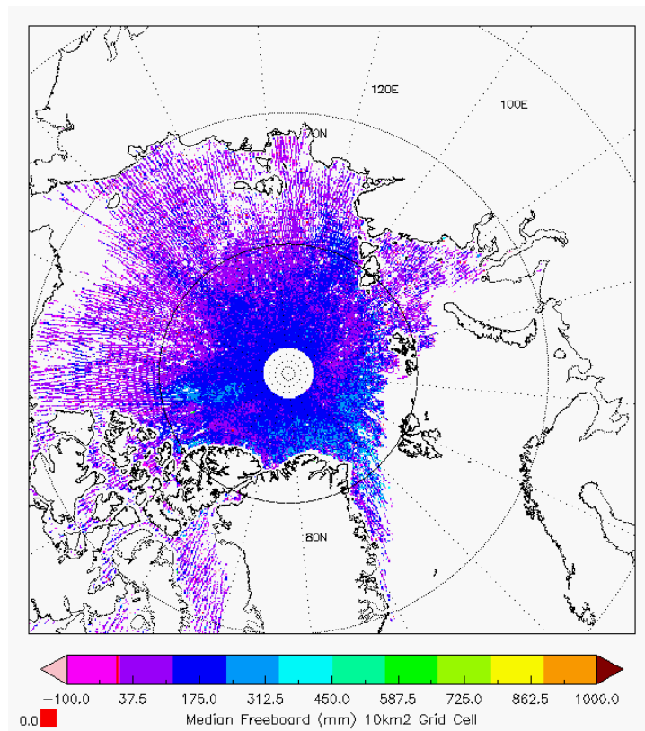
Figure 6 - Polar plots of 10km Gridded Freeboard values from L2 SAR products in cycle #148.
