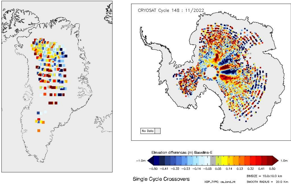
Figure 19 - Greenland and Antarctica maps of LRM elevation differences for cycle #148.
