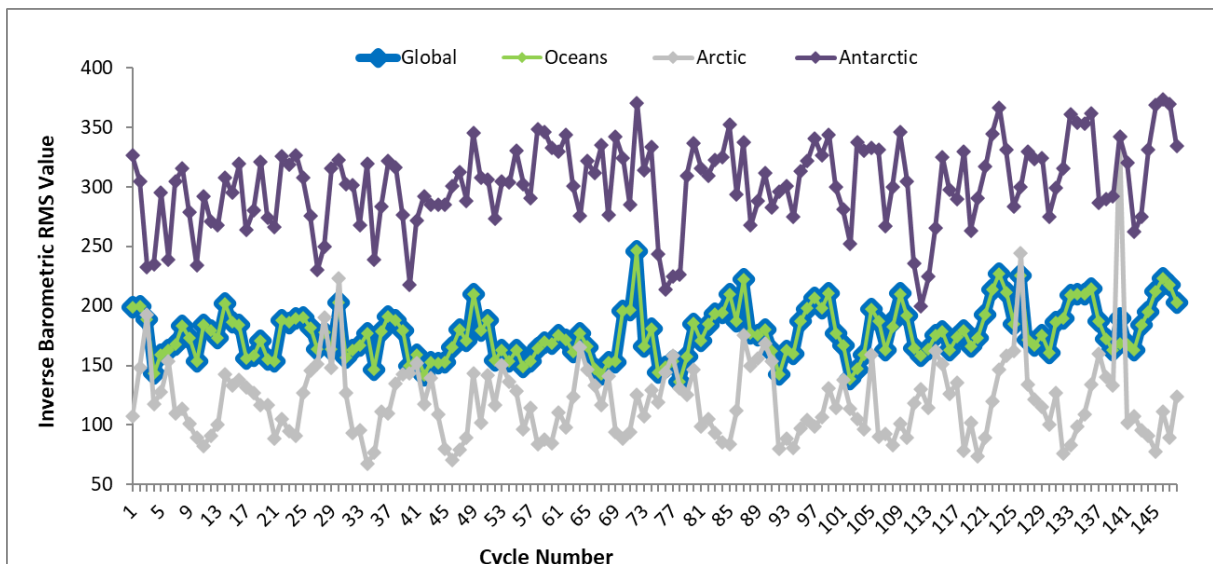
Figure 26 – Inverse Barometric Correction RMS value trend from beginning of mission
