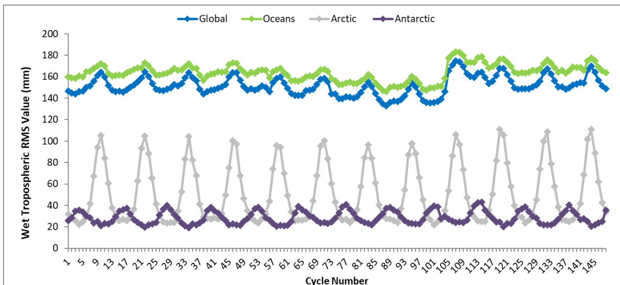
Figure 24 – Wet Tropospheric Correction RMS value trend from beginning of mission
