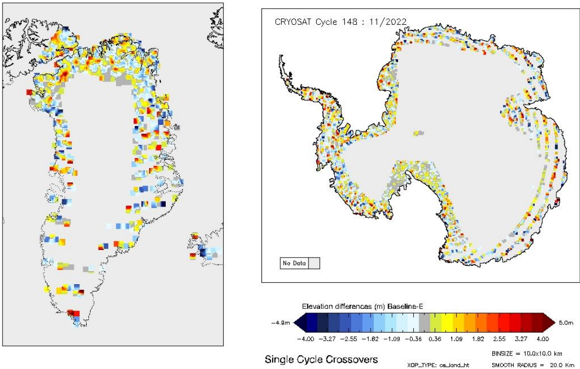
Figure 20 - Greenland and Antarctica maps of SARIn elevation differences for cycle #148.
