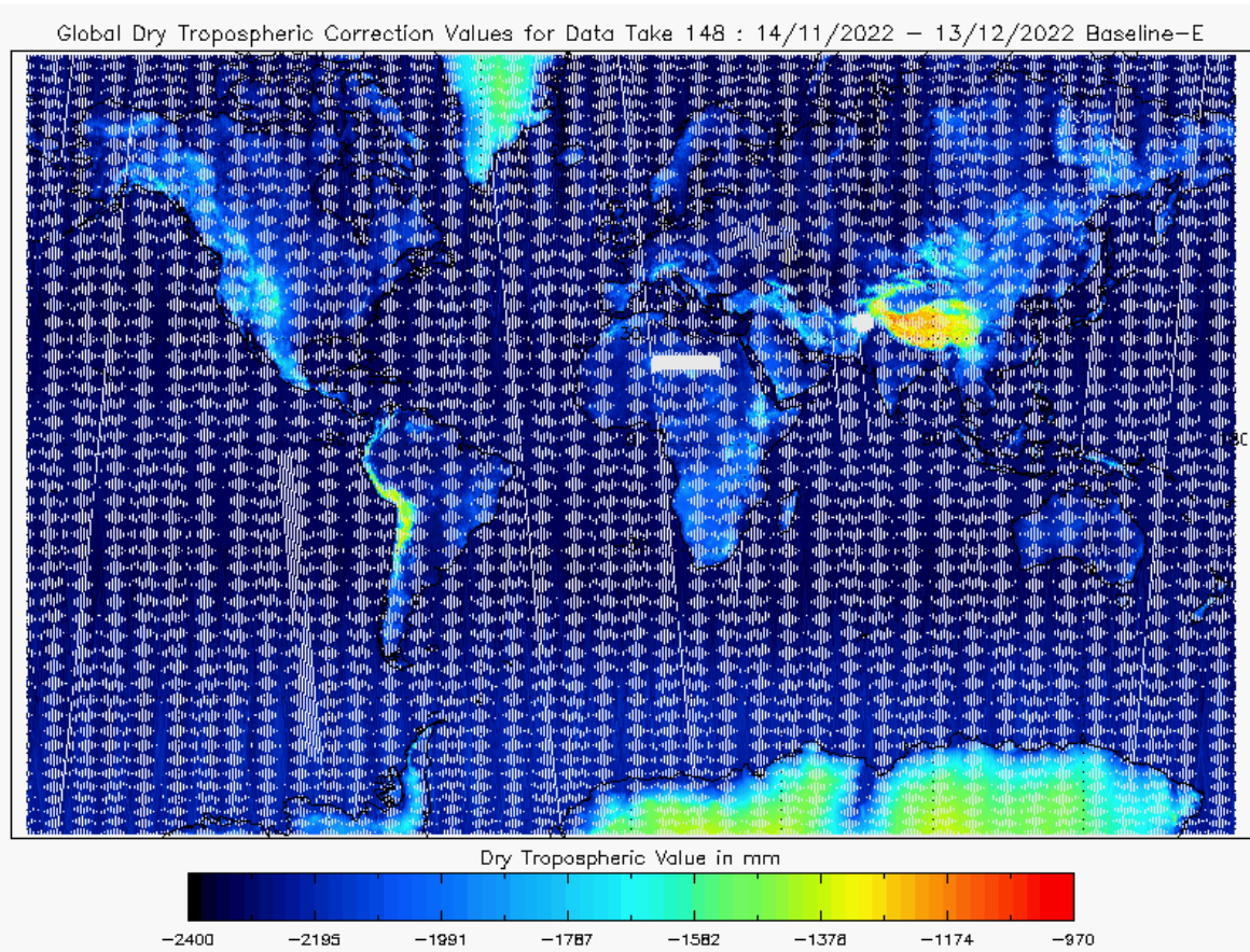
Figure 21 - Global plot of Dry Tropospheric Correction for cycle #148
