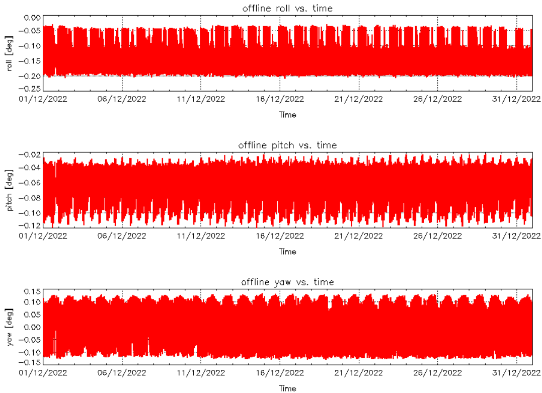
Figure 4 – Roll (top), Pitch (middle) and Yaw (bottom) values for L1B Products during cycle #148.
