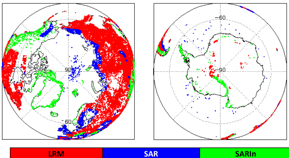
Figure 3 - Polar plots showing areas of loss of track in all SIRAL modes L0 data during October 2022.
