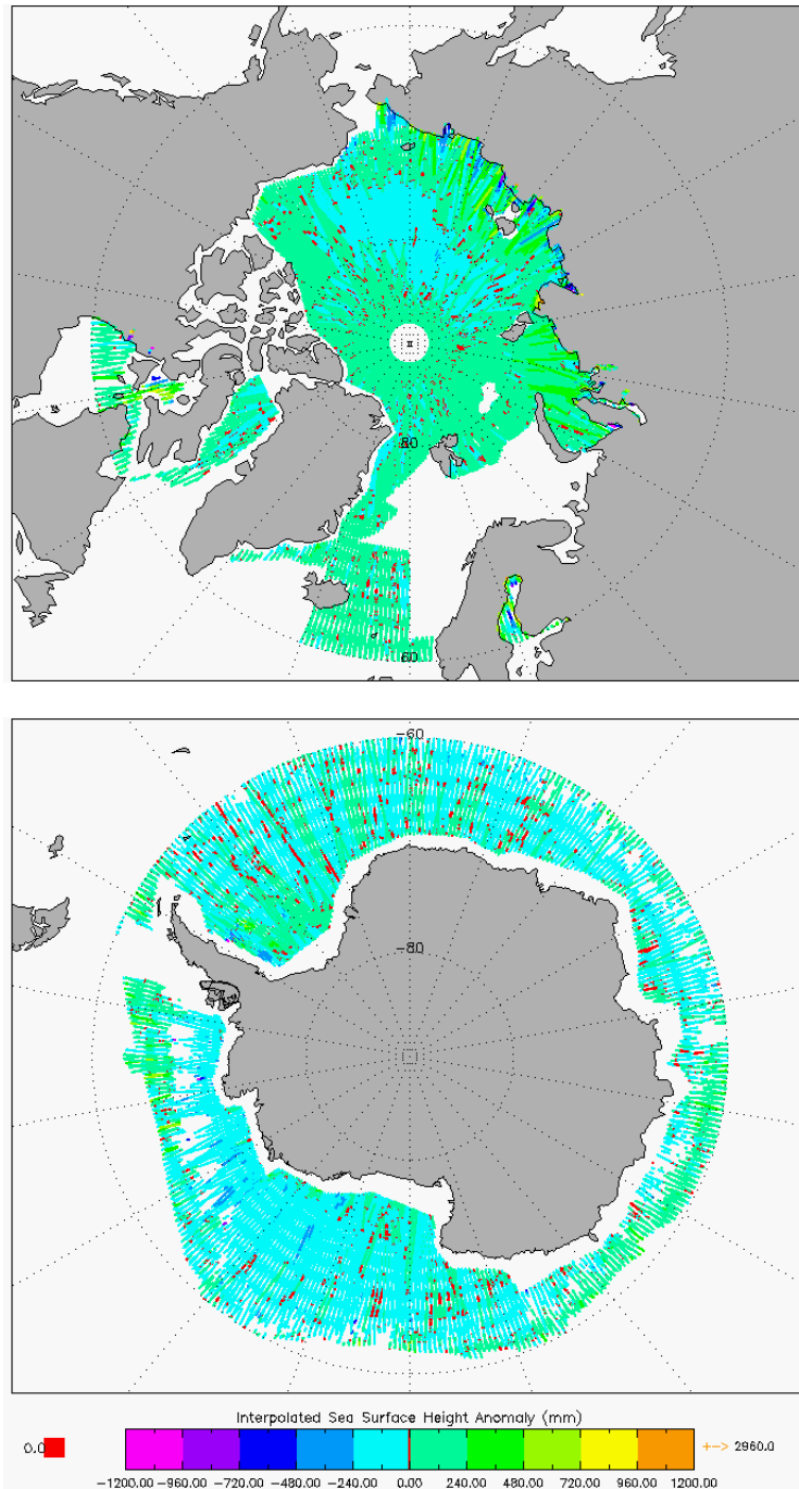
Figure 8 –Polar plots of SSHA for cycle #146.
