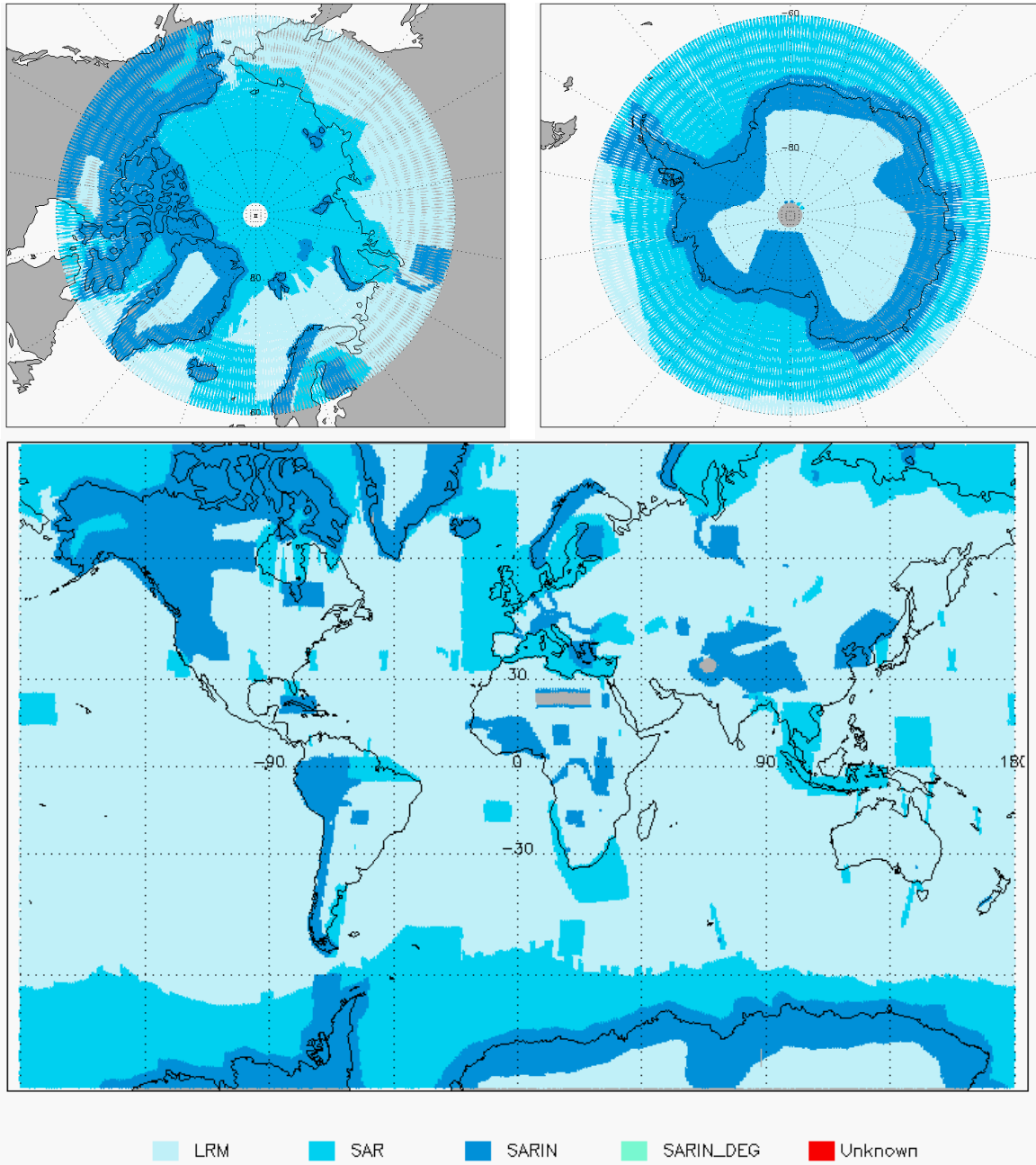
Figure 4 - Global and Polar plots of SIRAL Modes for cycle #146.
