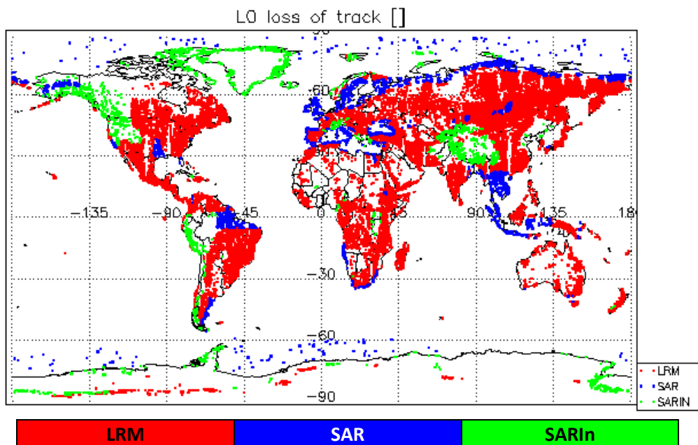
Figure 2 – Global plot showing areas of loss of track in all SIRAL modes L0 data during October 2022
