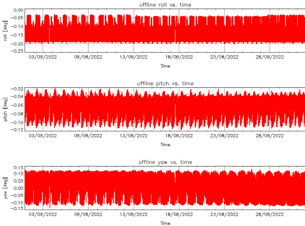
Figure 5 – Roll (top), Pitch (middle) and Yaw (bottom) values for L1B Products during cycle #146.
