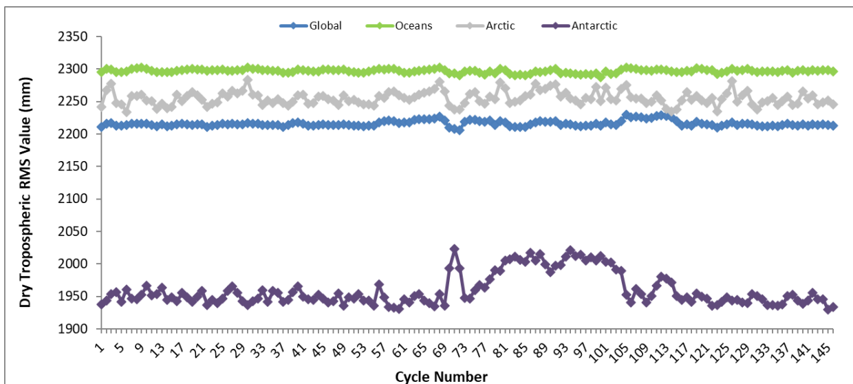
Figure 18 - Dry Tropospheric Correction RMS value trend from beginning of mission
