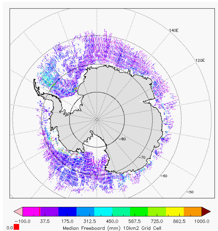
Figure 7 - Polar plots of 10km Gridded Freeboard values from L2 SAR products in cycle in Antarctica #146.
