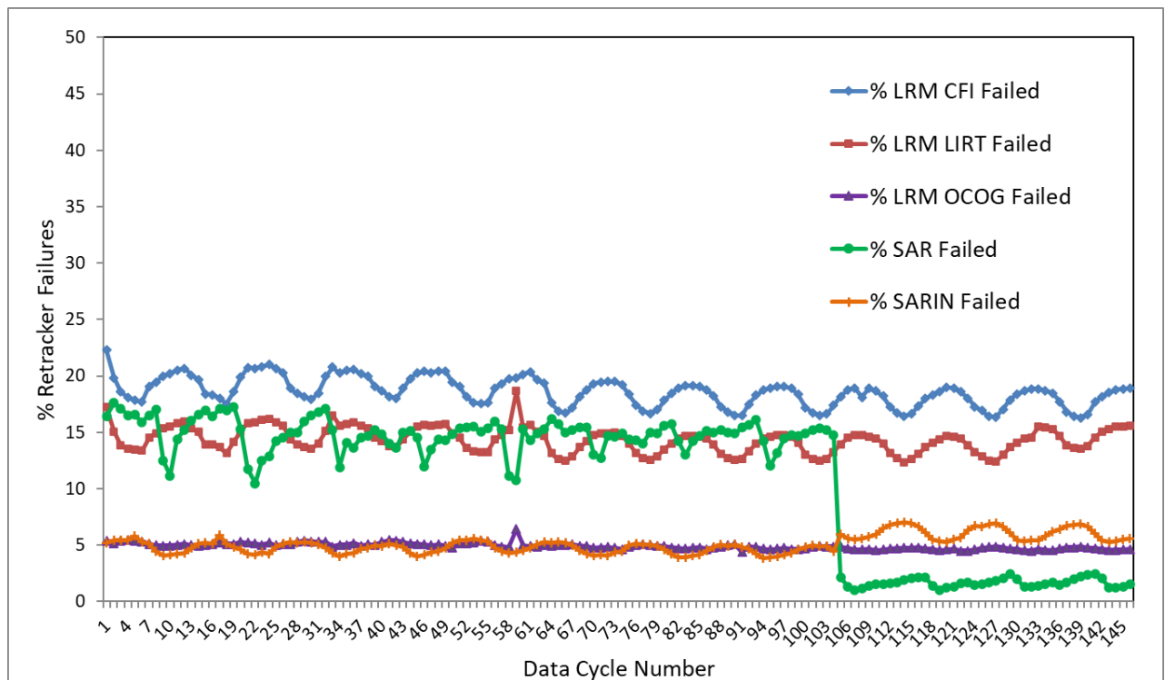
Figure 9 – Time Series for Retracker Failure Flags
