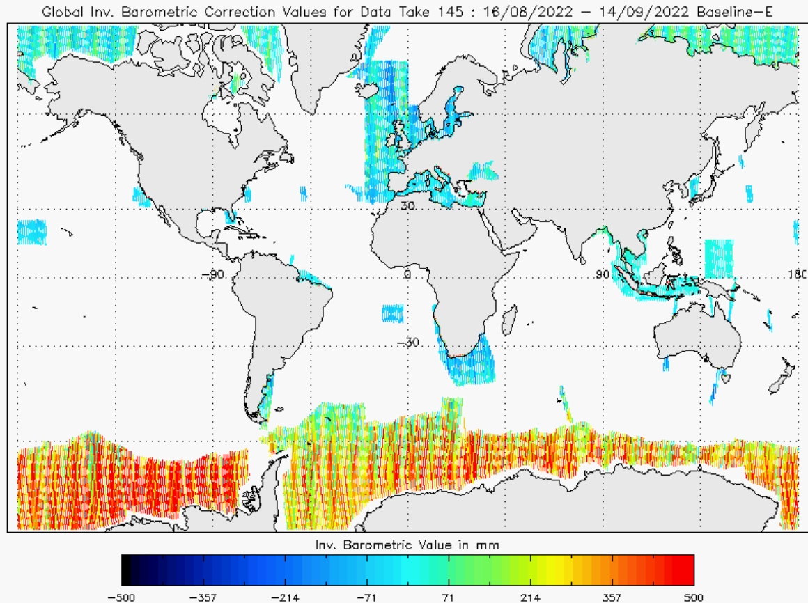
Figure 20 - Global plot of Inverse Barometric Correction for cycle #145
