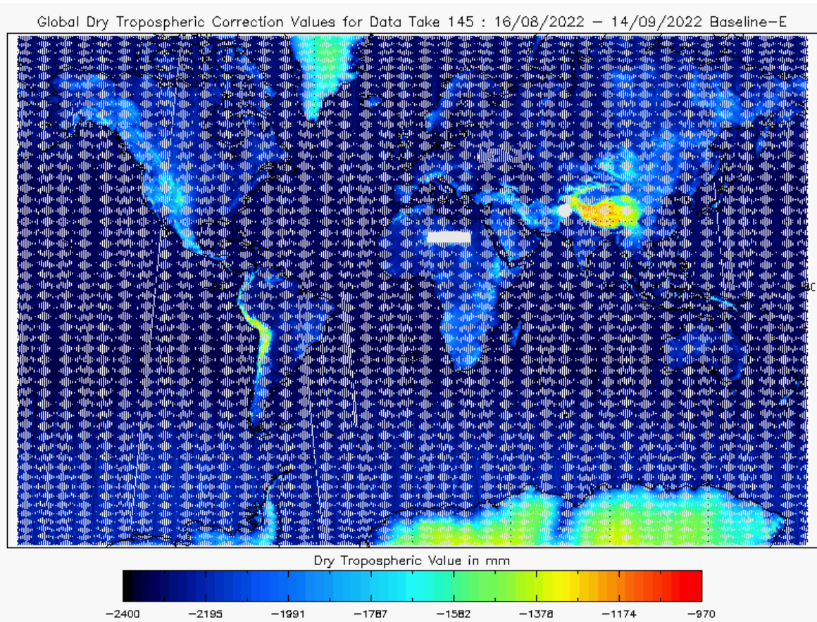
Figure 16 - Global plot of Dry Tropospheric Correction for cycle #145
