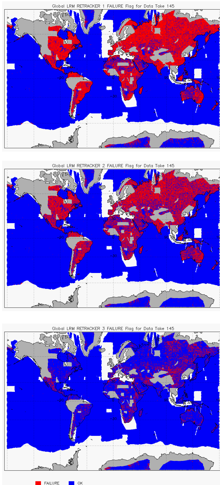
Figure 9 – Global plots showing Retracker Failure Flags for LRM mode for cycle #145:
