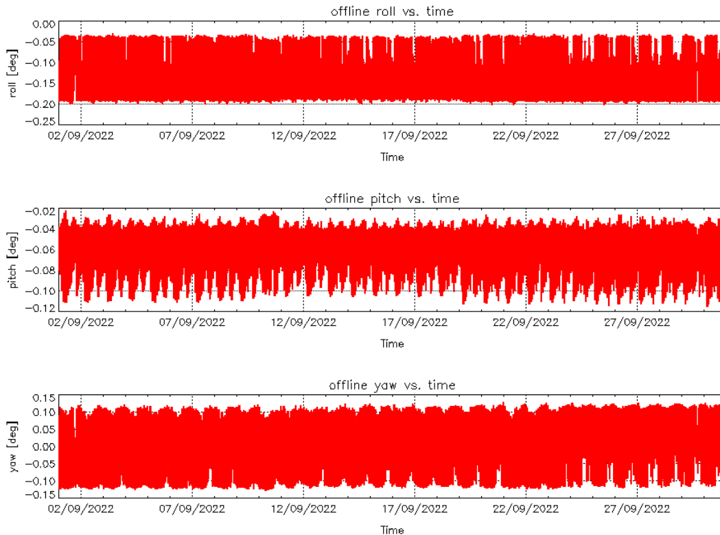
Figure 4 – Roll (top), Pitch (middle) and Yaw (bottom) values for L1B Products during cycle #145.
