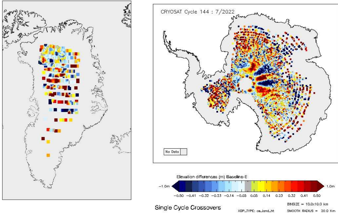
Figure 14 - Greenland and Antarctica maps of LRM elevation differences for cycle #144.
