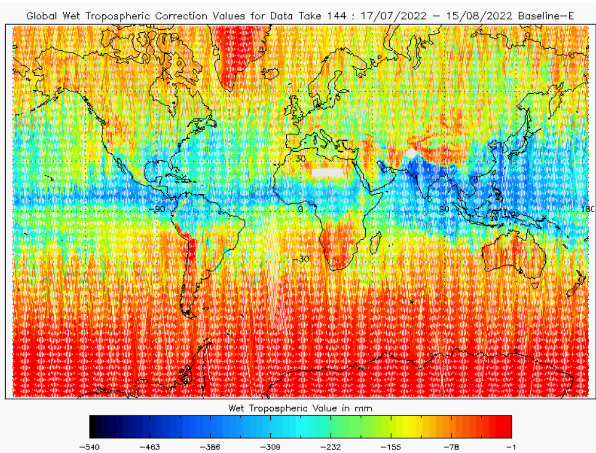
Figure 18 - Global plot of Wet Tropospheric Correction for cycle #144
