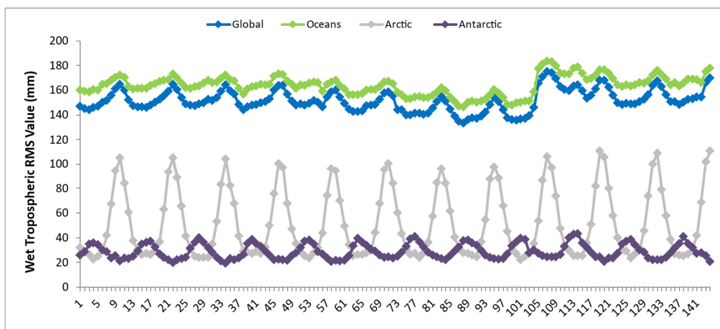
Figure 19 – Wet Tropospheric Correction RMS value trend from beginning of mission
