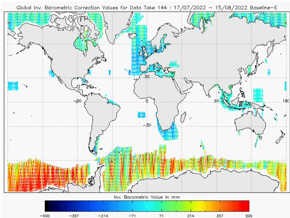
Figure 20 - Global plot of Inverse Barometric Correction for cycle #144
