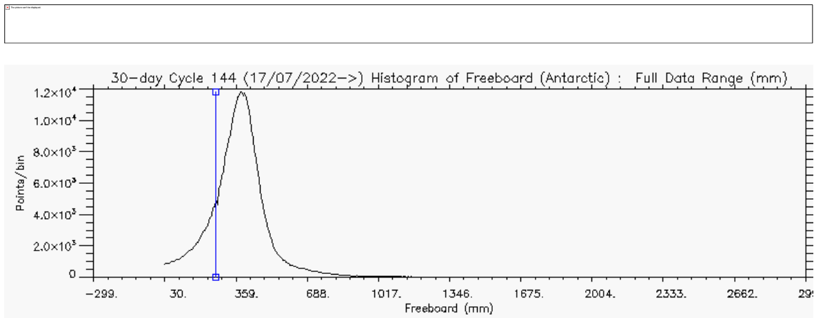
Figure 5 – Histogram of Freeboard for Arctic (above) and Antarctic (below) for cycle #144
