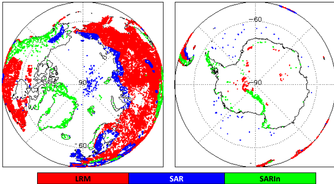
Figure 2 - Polar plots showing areas of loss of track in all SIRAL modes L0 data during August 2022.
