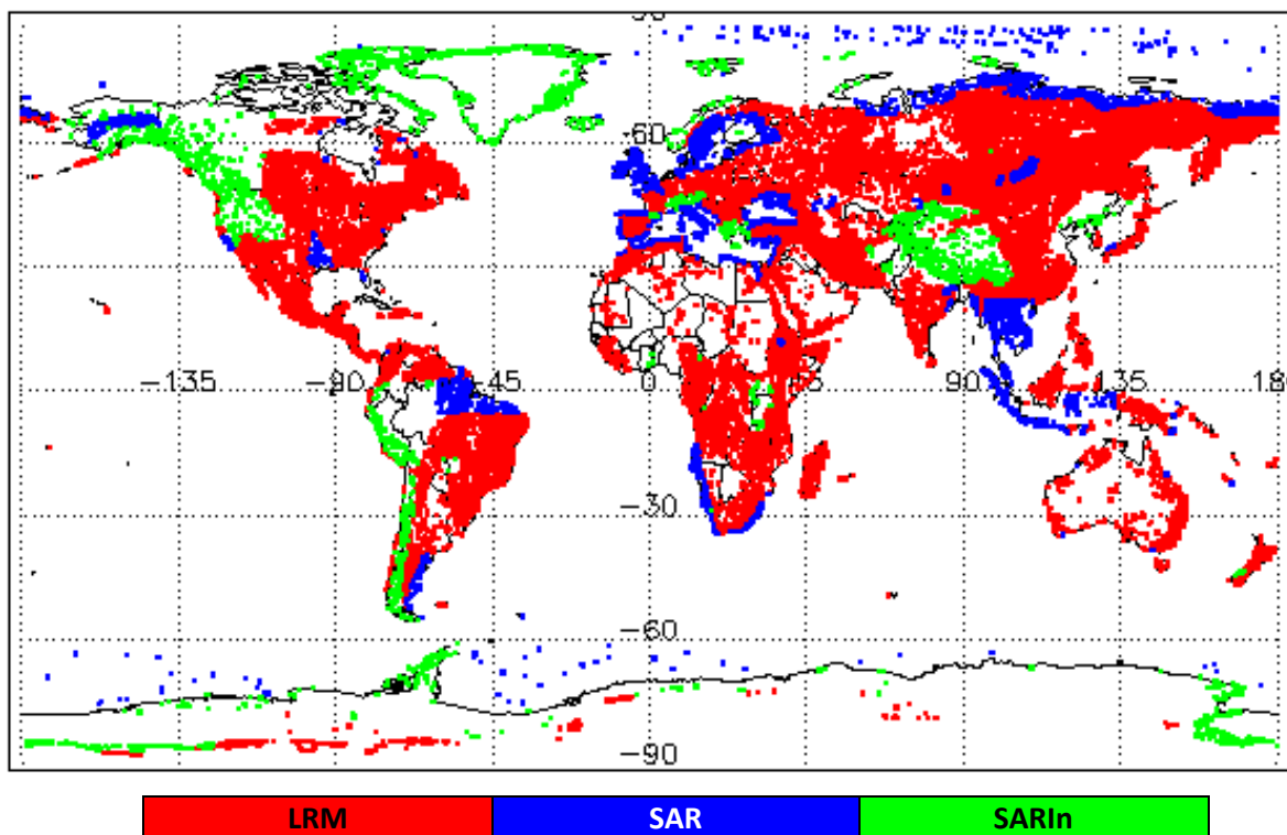
Figure 1 – Global plot showing areas of loss of track in all SIRAL modes L0 data during August 2022
