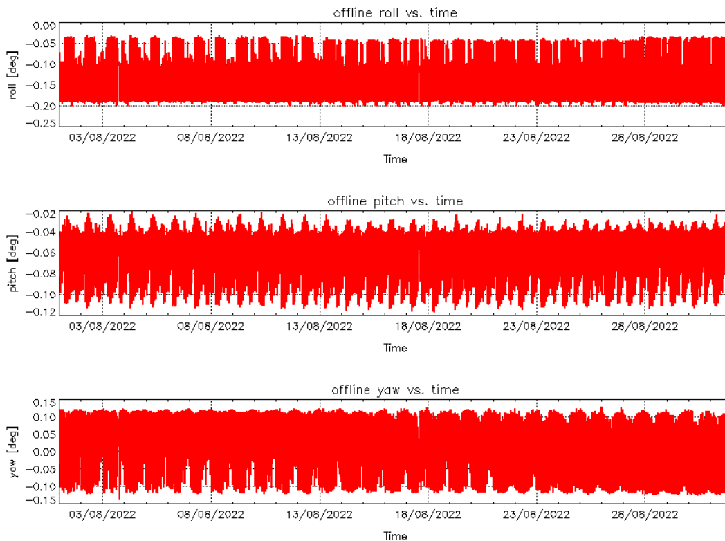
Figure 4 – Roll (top), Pitch (middle) and Yaw (bottom) values for L1B Products during cycle #144.
