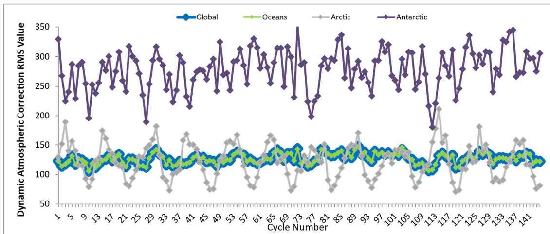
Figure 23 – Dynamic Atmospheric Correction RMS value trend from beginning of mission
