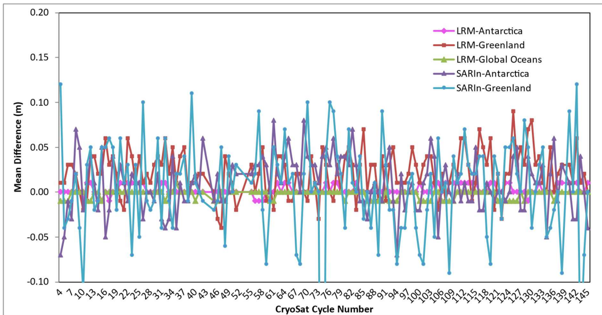
Figure 13 - Time series for Mean Difference in elevation at crossovers from beginning of the mission
