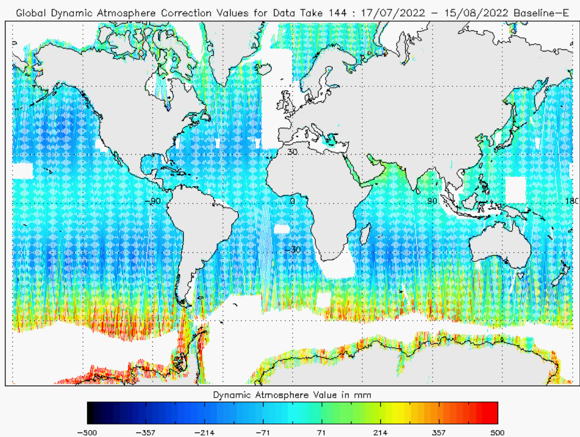
Figure 22 - Global plot of Dynamic Atmospheric Correction for cycle #144
