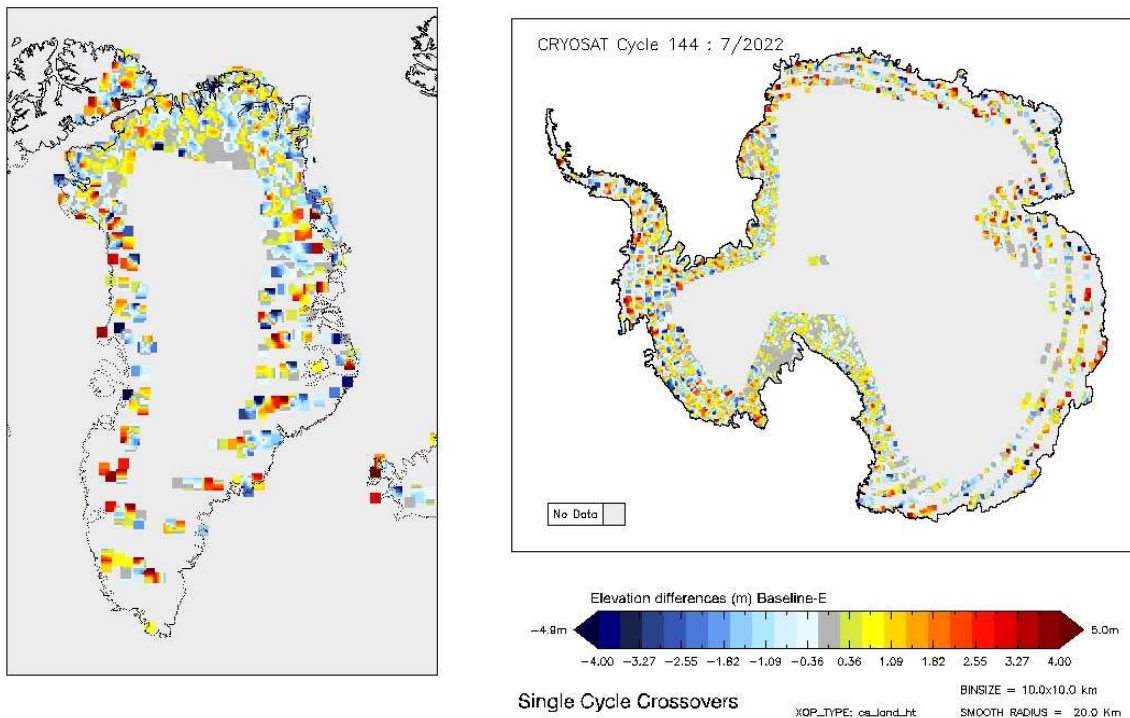
Figure 15 - Greenland and Antarctica maps of SARIn elevation differences for cycle #144.
