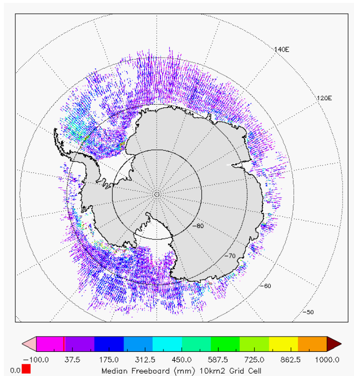
Figure 6 - Polar plots of 10km Gridded Freeboard values from L2 SAR products in cycle #144.
