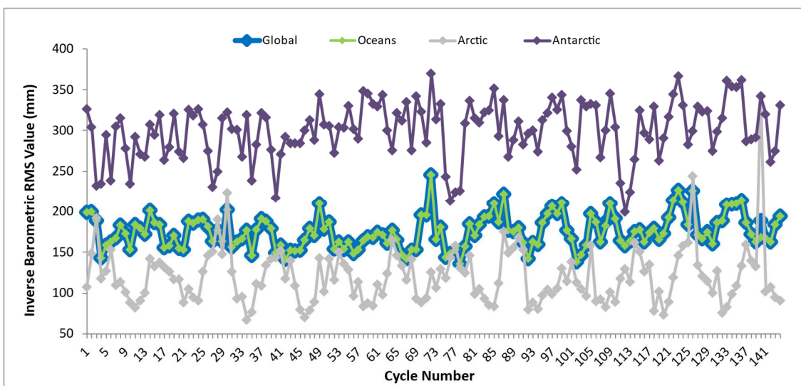
Figure 21 – Inverse Barometric Correction RMS value trend from beginning of mission
