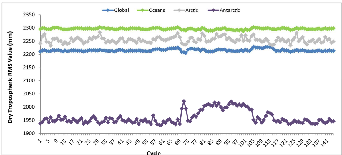
Figure 17 - Dry Tropospheric Correction RMS value trend from beginning of mission
