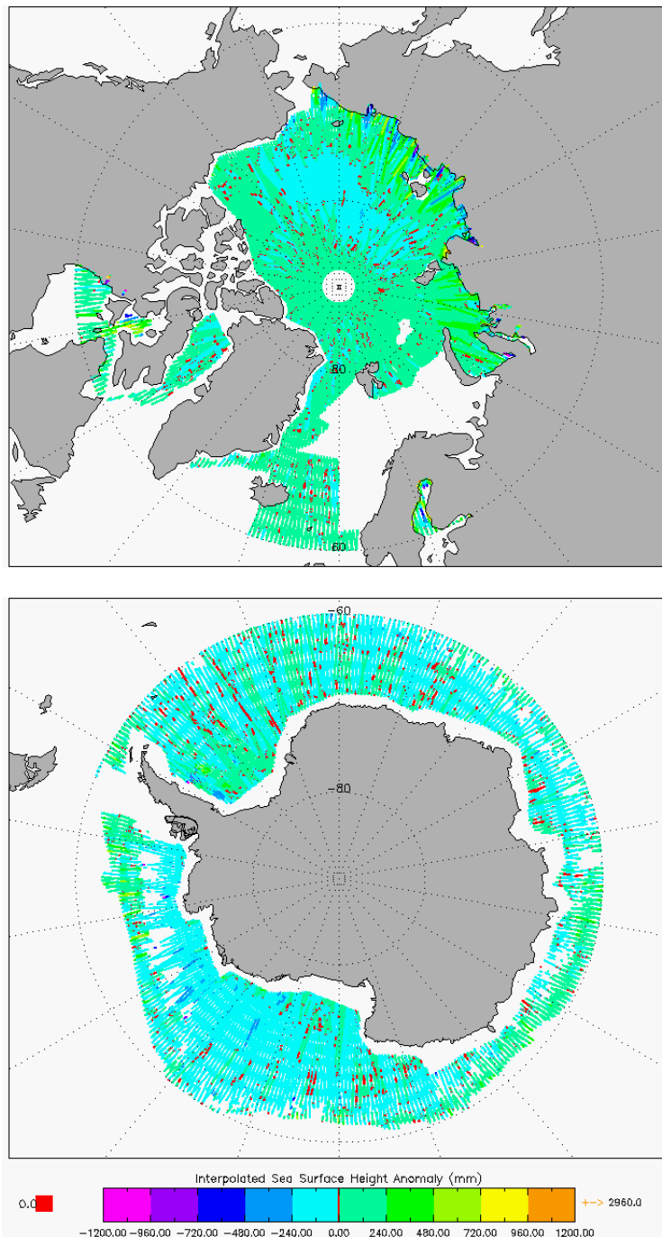
Figure 7 –Polar plots of SSHA for cycle #144.
