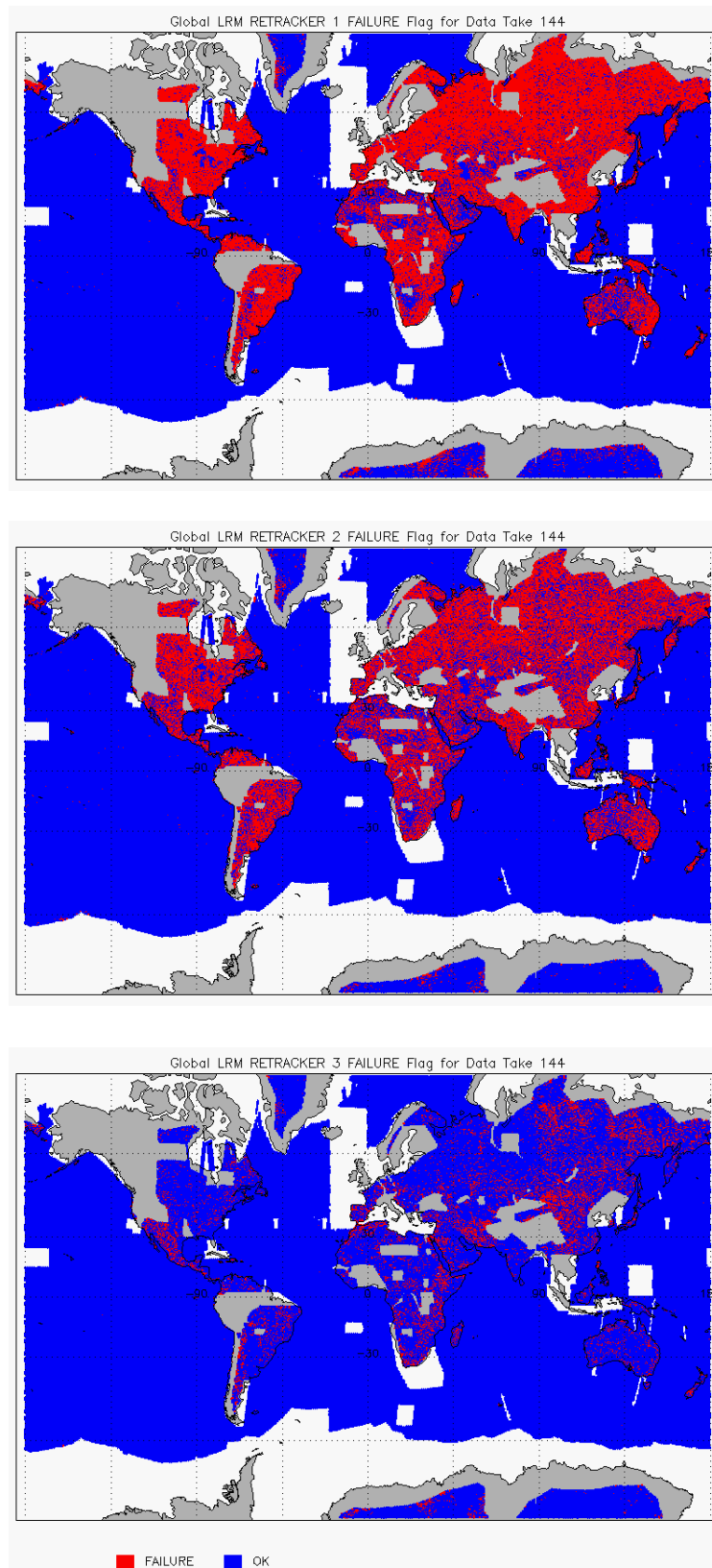
Figure 9 – Global plots showing Retracker Failure Flags for LRM mode for cycle #144: LRM CFI (top), LRM LIRT (middle), LRM OCOG (bottom)
