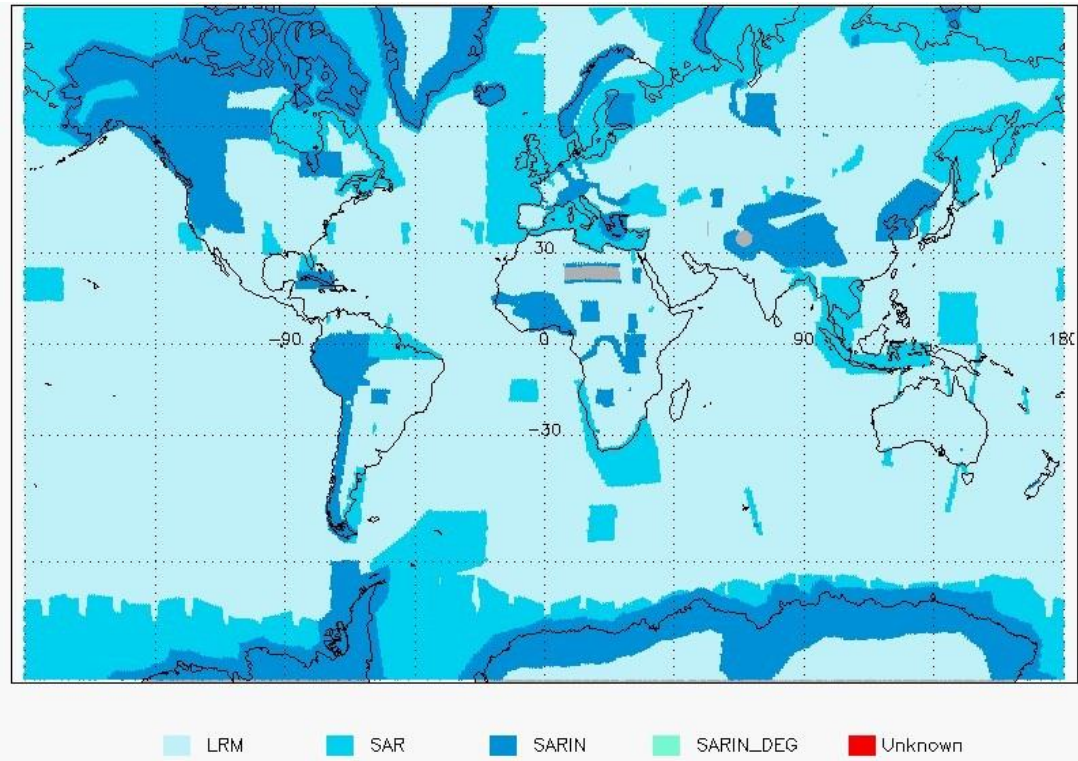
Figure 3 - Global and Polar plots of SIRAL Modes for cycle #143.
