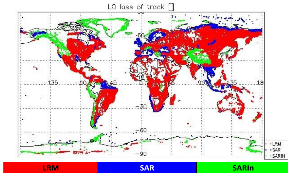
Figure 1 – Global plot showing areas of loss of track in all SIRAL modes L0 data during July 2022
