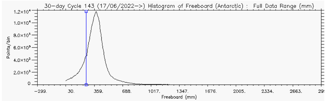
Figure 6 – Histogram of Freeboard for the Antarctic for cycle #143
