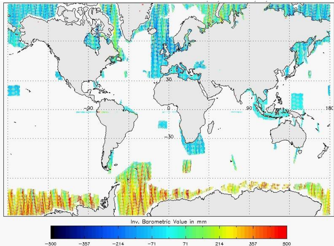
Figure 21 - Global plot of Inverse Barometric Correction for cycle #143
