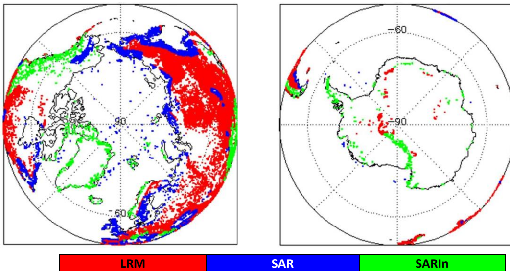
Figure 2 - Polar plots showing areas of loss of track in all SIRAL modes L0 data during July 2022.
