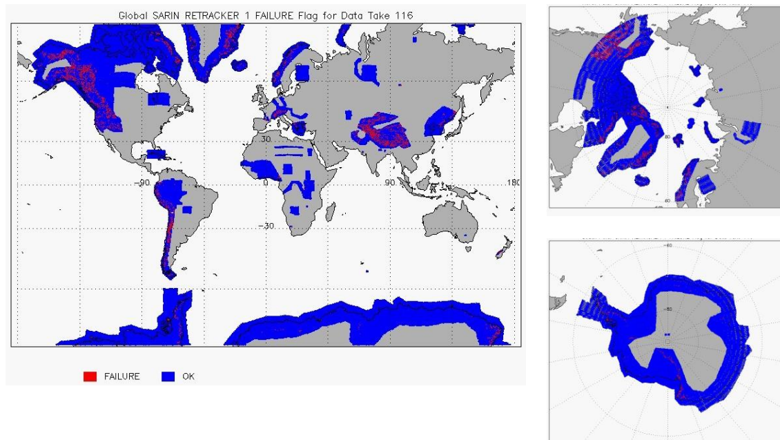
Figure 12 - Global plots showing Retracker Failure Flags for SARIn mode for cycle #143
