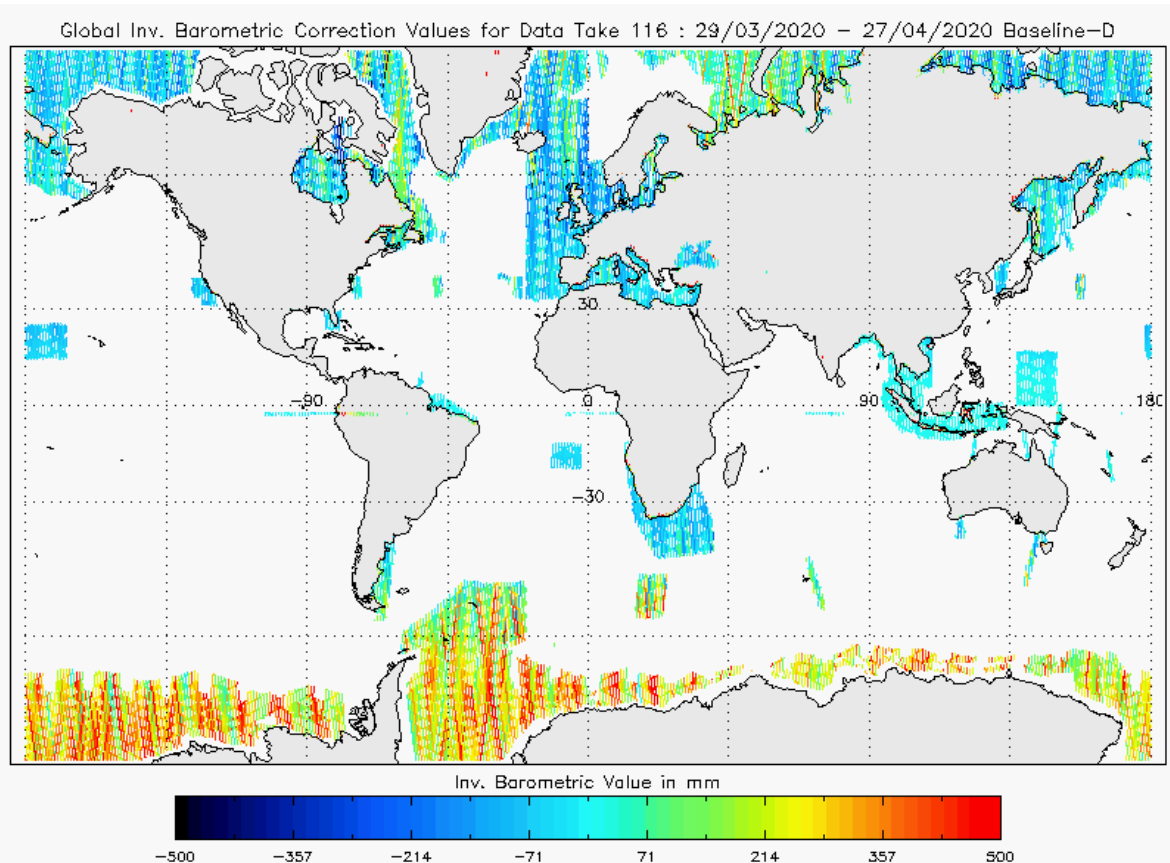
Figure 20 - Global plot of Inverse Barometric Correction for cycle #142
