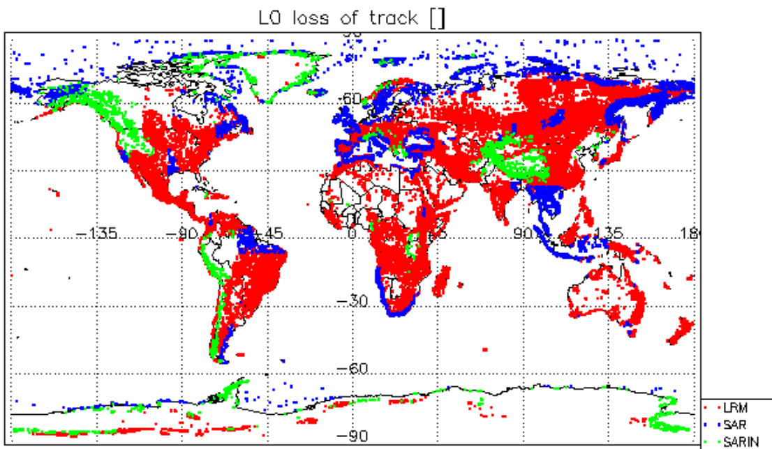
Figure 1 – Global plot showing areas of loss of track in all SIRAL modes L0 data during June 2022, graph is not available and will be ingested when it is available.
