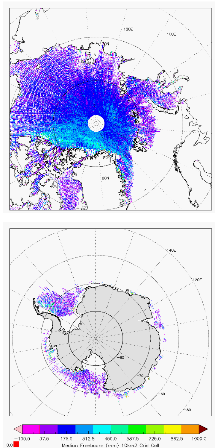
Figure 6 - Polar plots of 10km Gridded Freeboard values from L2 SAR products in cycle #142.
