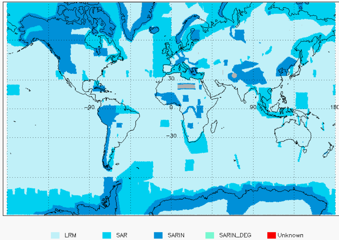
Figure 3 - Global and Polar plots of SIRAL Modes for cycle #142.
