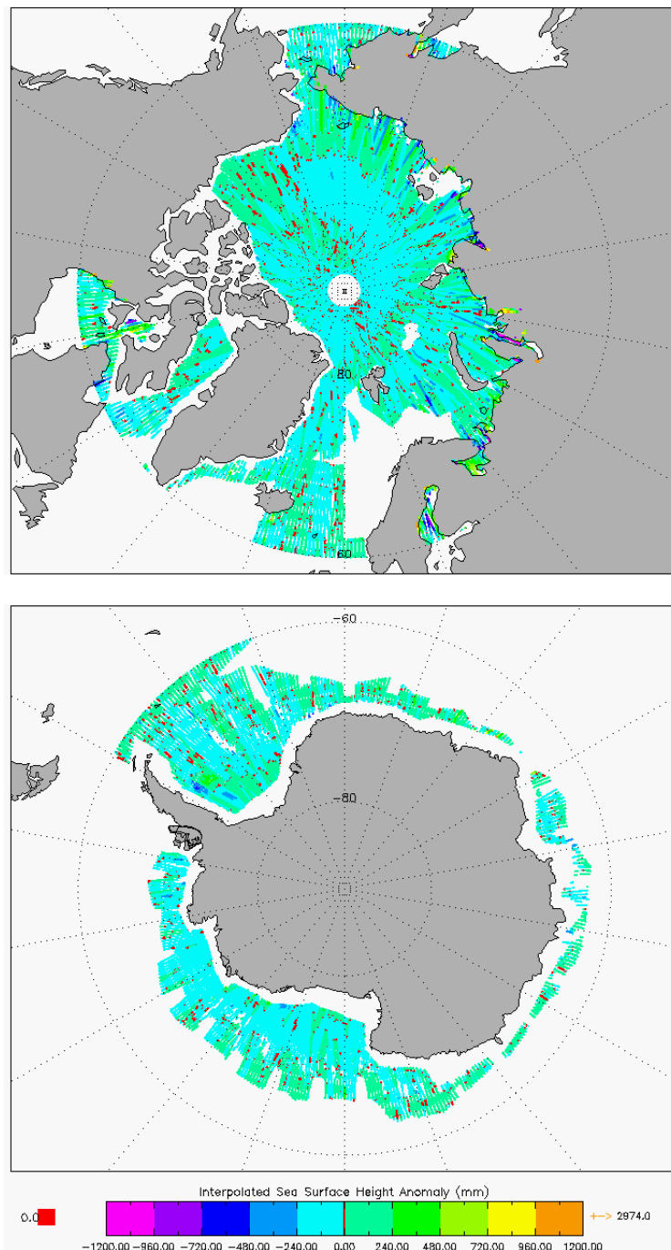
Figure 7 –Polar plots of SSHA for cycle #142.
