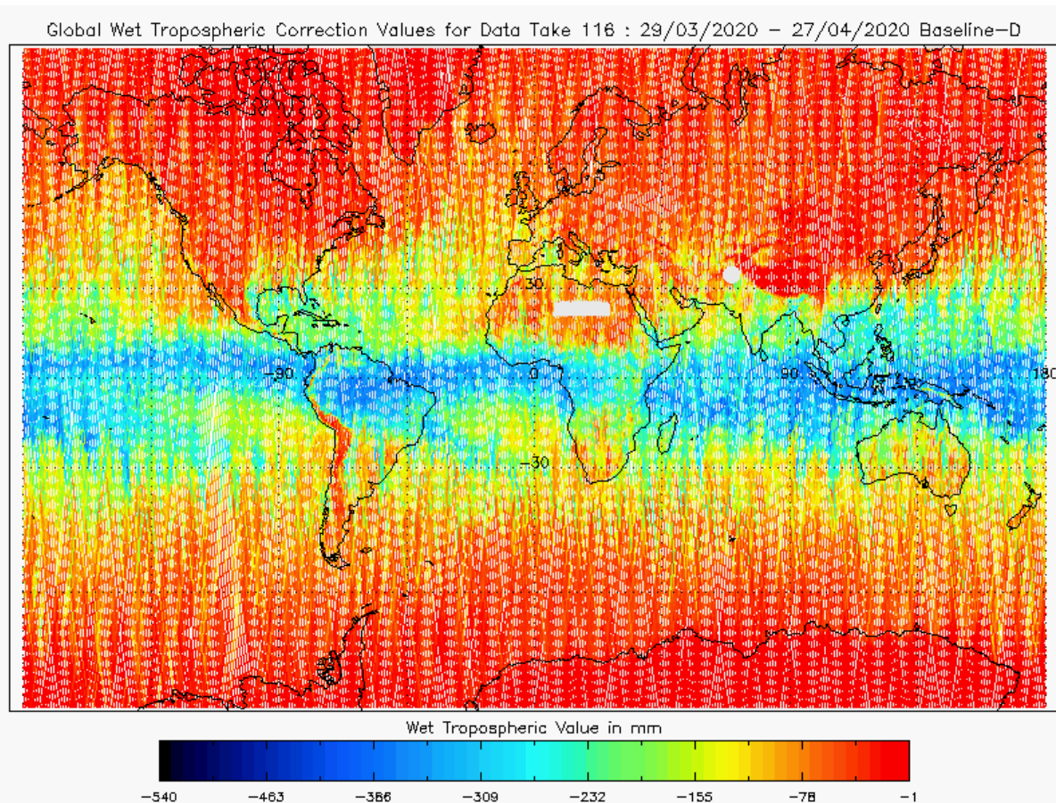
Figure 18 - Global plot of Wet Tropospheric Correction for cycle #142
