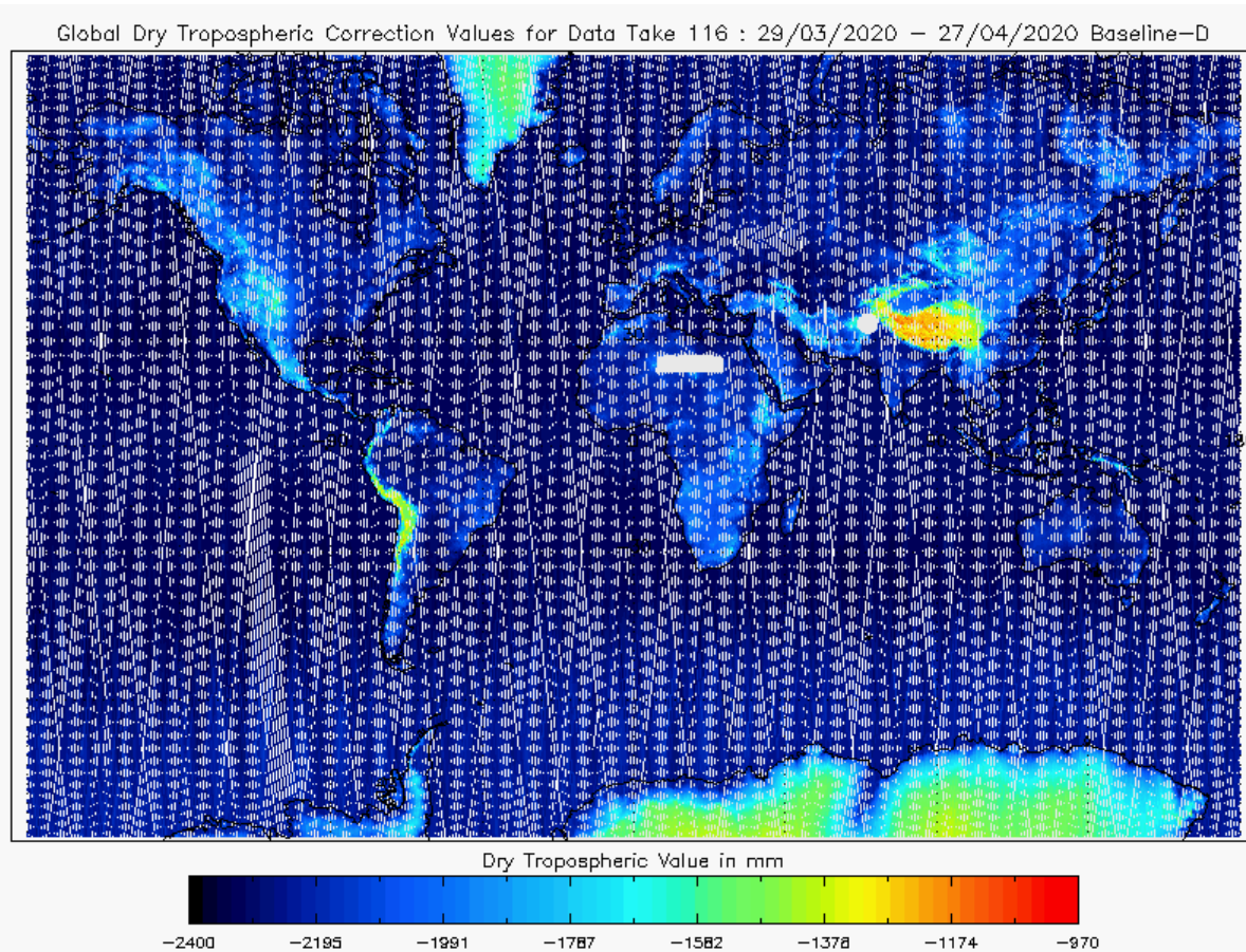
Figure 16 - Global plot of Dry Tropospheric Correction for cycle #142
