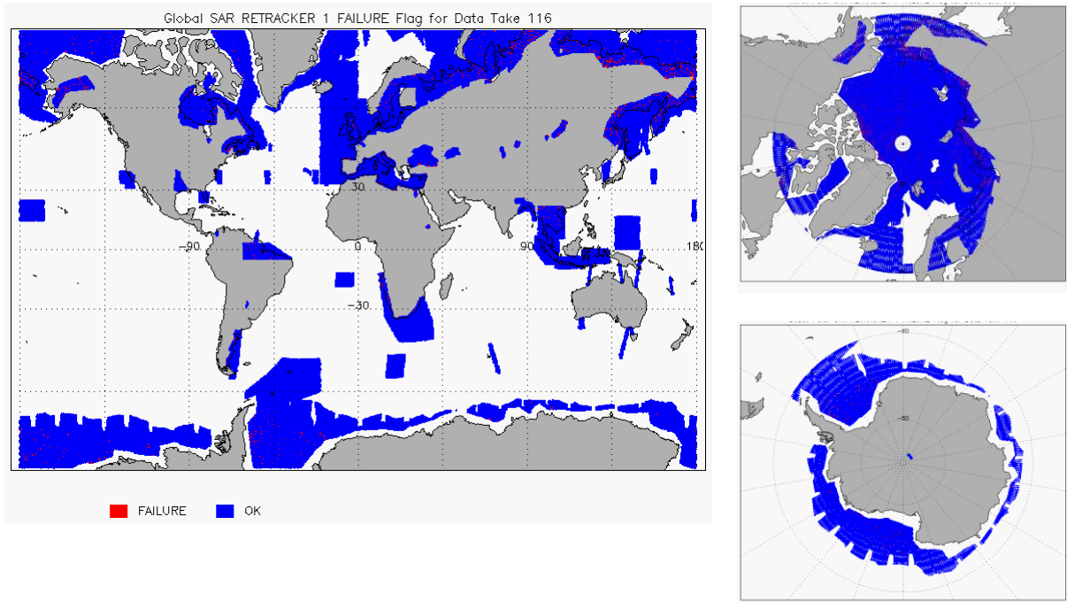
Figure 10 - Global plots showing Retracker Failure Flags for SAR mode for cycle #142
