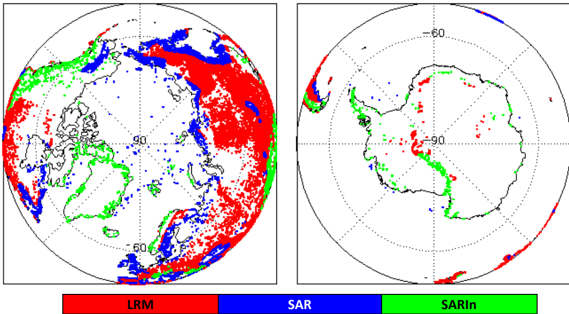
Figure 2 - Polar plots showing areas of loss of track in all SIRAL modes L0 data during June 2022.
