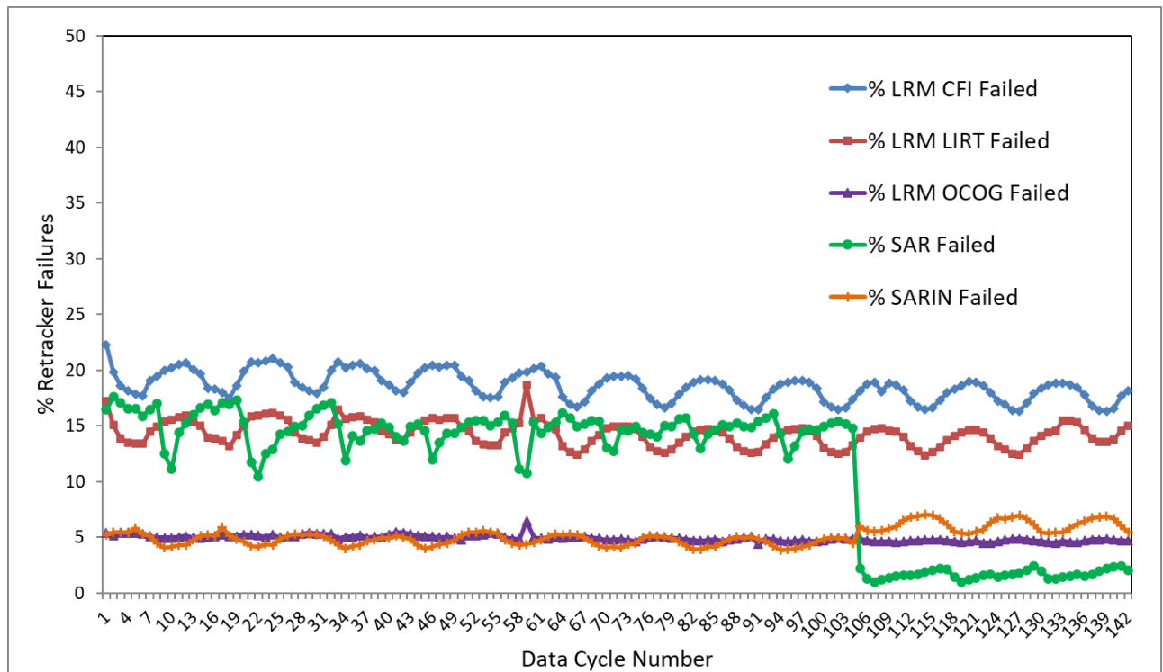
Figure 8 – Time Series for Retracker Failure Flags
