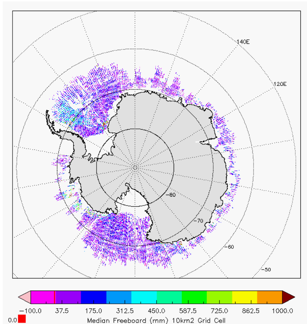
Figure 6 - Polar plot of 10km Gridded Freeboard values from L2 SAR products in cycle #142. Note Freeboard is not calculated for the Arctic during this period.
