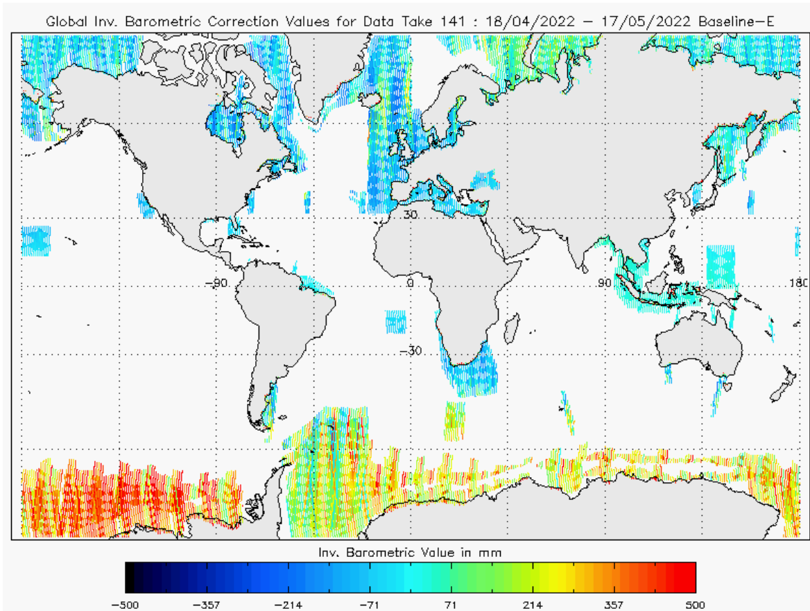
Figure 20 - Global plot of Inverse Barometric Correction for cycle #141
