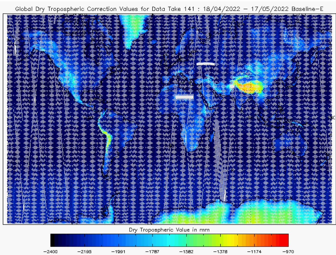
Figure 16 - Global plot of Dry Tropospheric Correction for cycle #141
