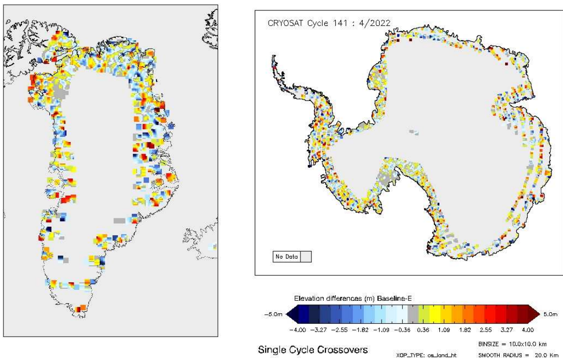
Figure 15 - Greenland and Antarctica maps of SARIn elevation differences for cycle #141.
