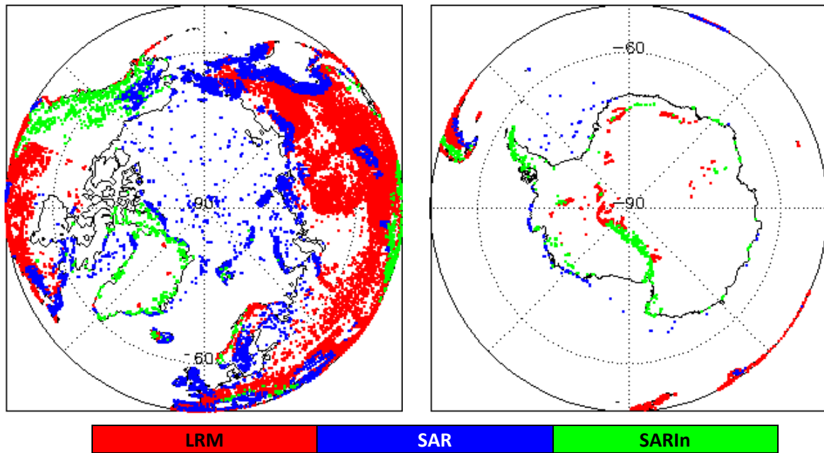
Figure 2 - Polar plots showing areas of loss of track in all SIRAL modes L0 data during May 2022.
