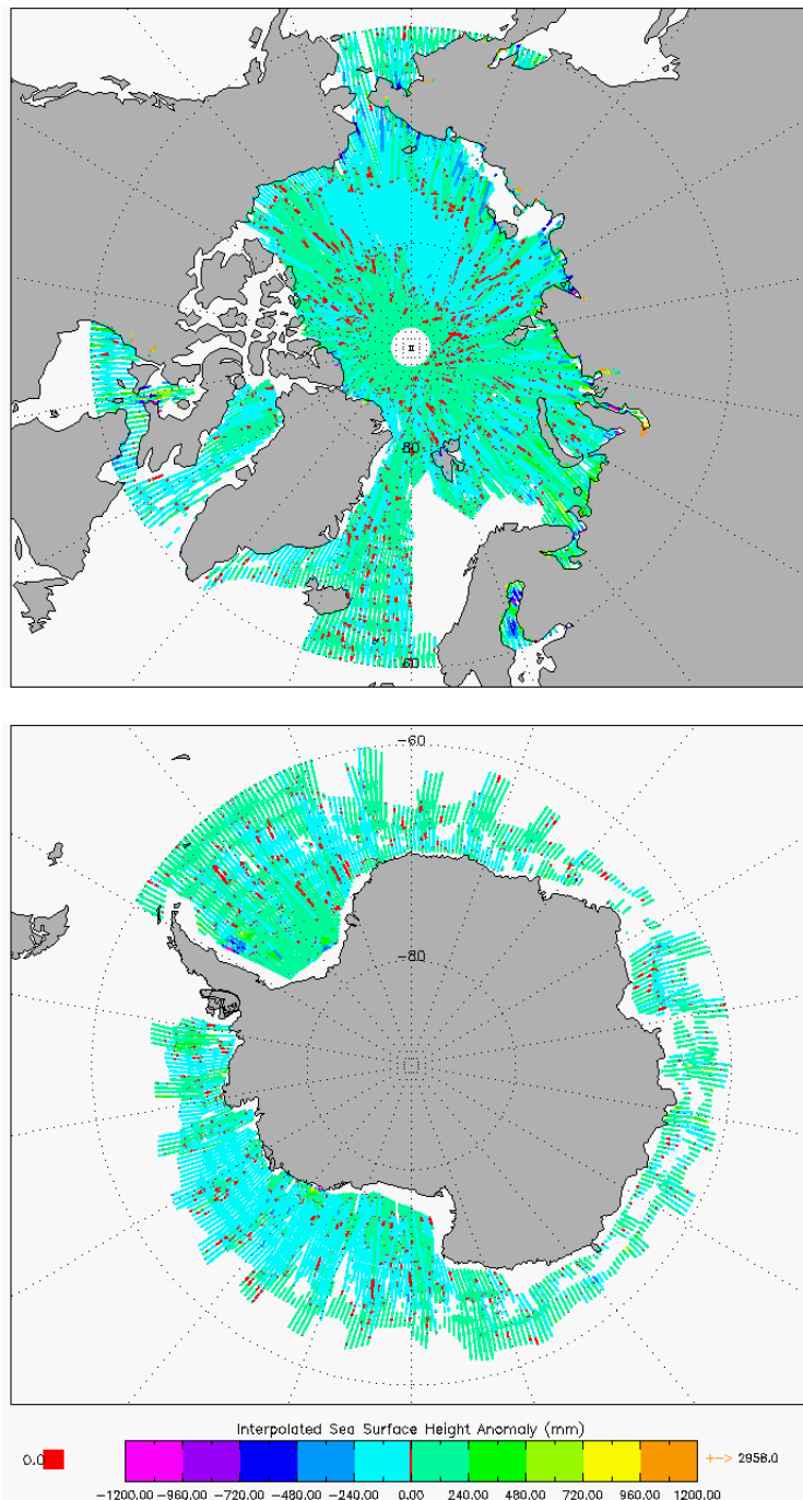
Figure 7 –Polar plots of SSHA for cycle #141.
