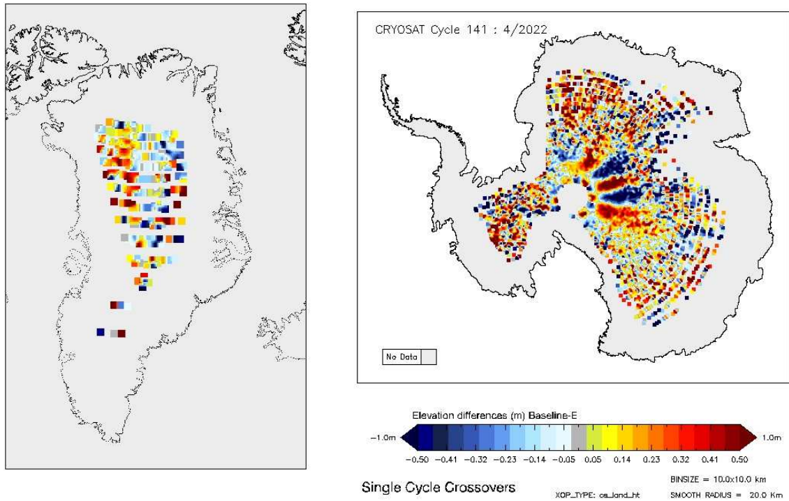
Figure 14 - Greenland and Antarctica maps of LRM elevation differences for cycle #141.
