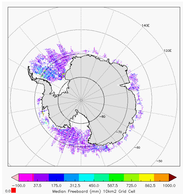
Figure 6 - Polar plots of 10km Gridded Freeboard values from L2 SAR products in cycle #141.
