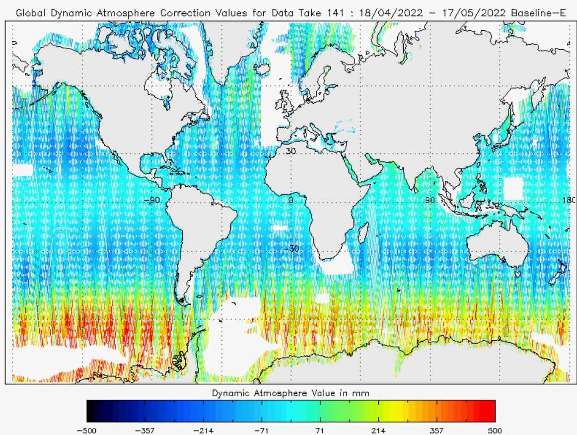
Figure 22 - Global plot of Dynamic Atmospheric Correction for cycle #141
