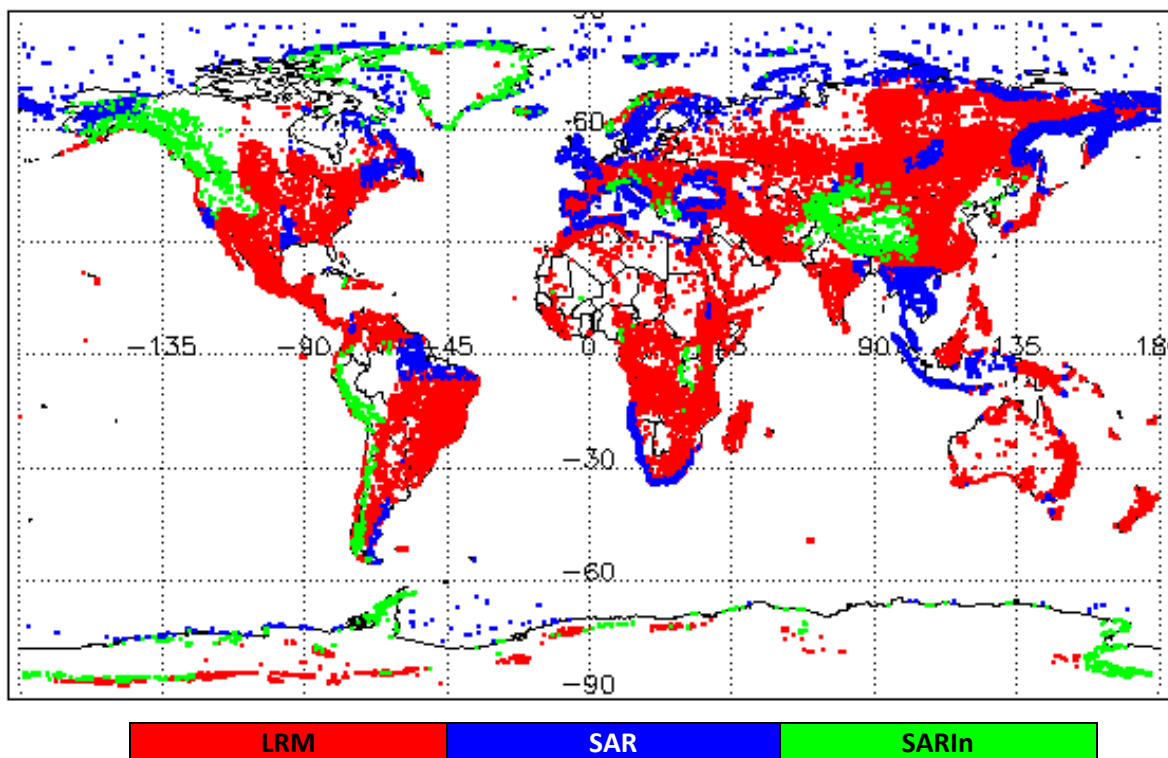
Figure 1 – Global plot showing areas of loss of track in all SIRAL modes L0 data during May 2022
