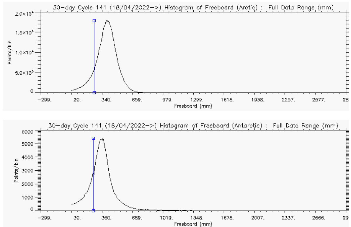
Figure 5 – Histogram of Freeboard for Arctic (above) and Antarctic (below) for cycle #141
