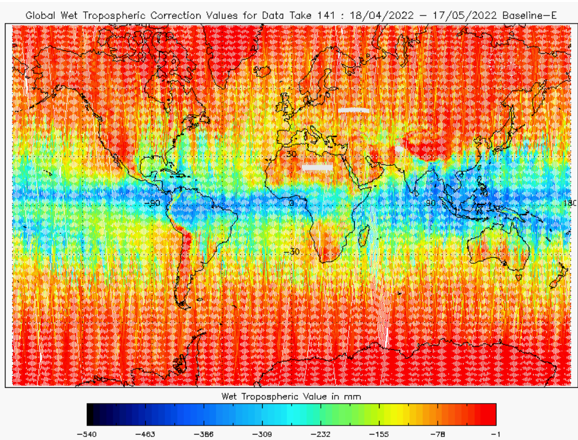
Figure 18 - Global plot of Wet Tropospheric Correction for cycle #141
