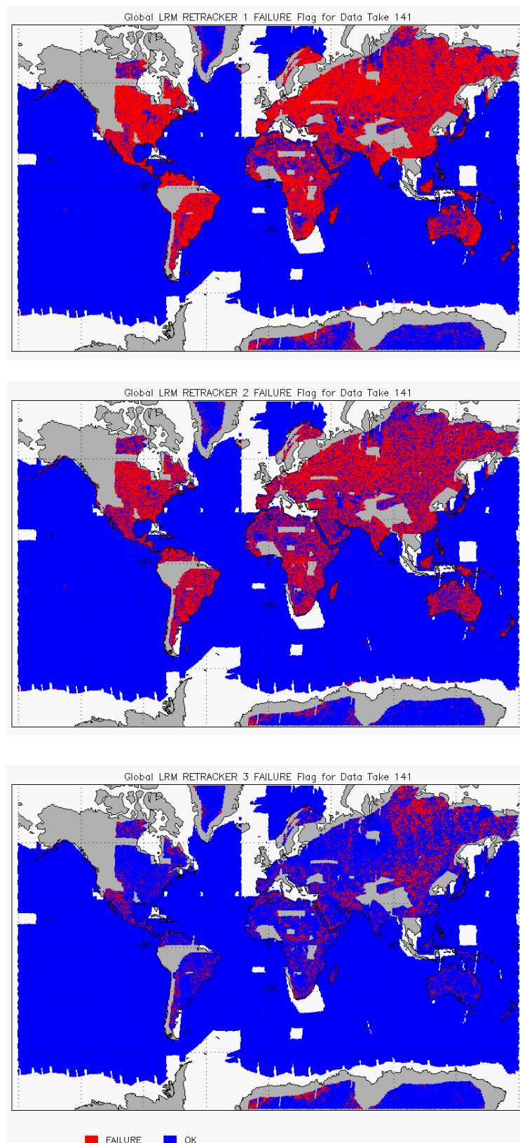
Figure 9 – Global plots showing Retracker Failure Flags for LRM mode for cycle #141:
