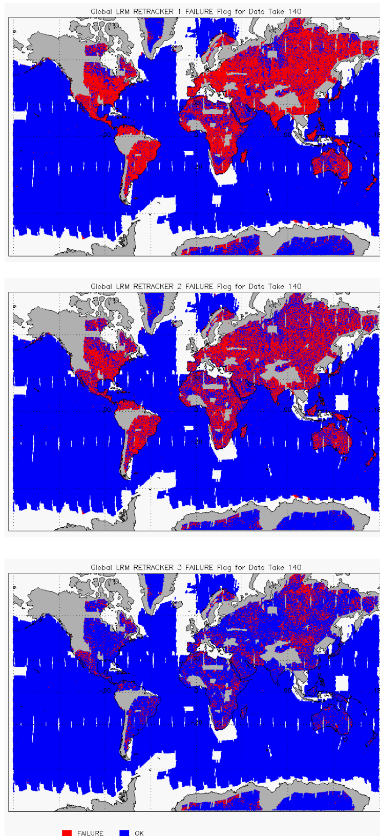
Figure 9 – Global plots showing Retracker Failure Flags for LRM mode for cycle #140: LRM CFI (top), LRM LIRT (middle), LRM OCOG (bottom)
