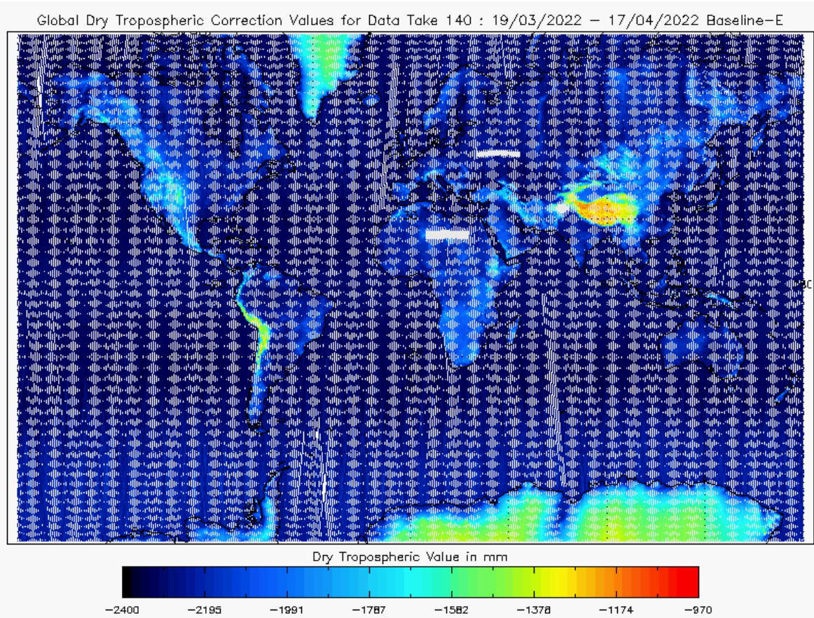
Figure 16 - Global plot of Dry Tropospheric Correction for cycle #140
