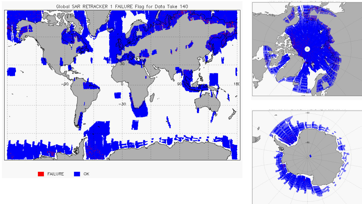
Figure 10 - Global plots showing Retracker Failure Flags for SAR mode for cycle #140
