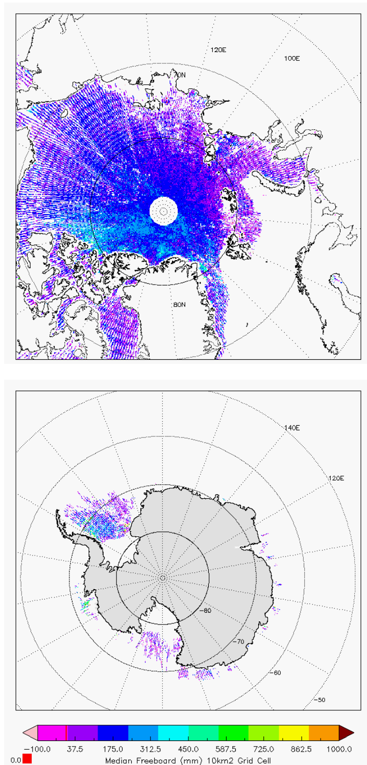
Figure 6 - Polar plots of 10km Gridded Freeboard values from L2 SAR products in cycle #140.
