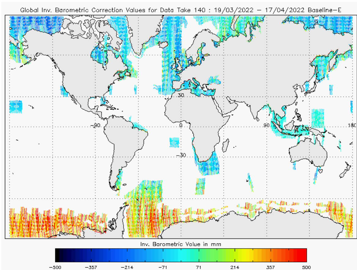
Figure 20 - Global plot of Inverse Barometric Correction for cycle #140
