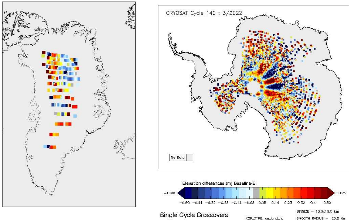
Figure 14 - Greenland and Antarctica maps of LRM elevation differences for cycle #140.
