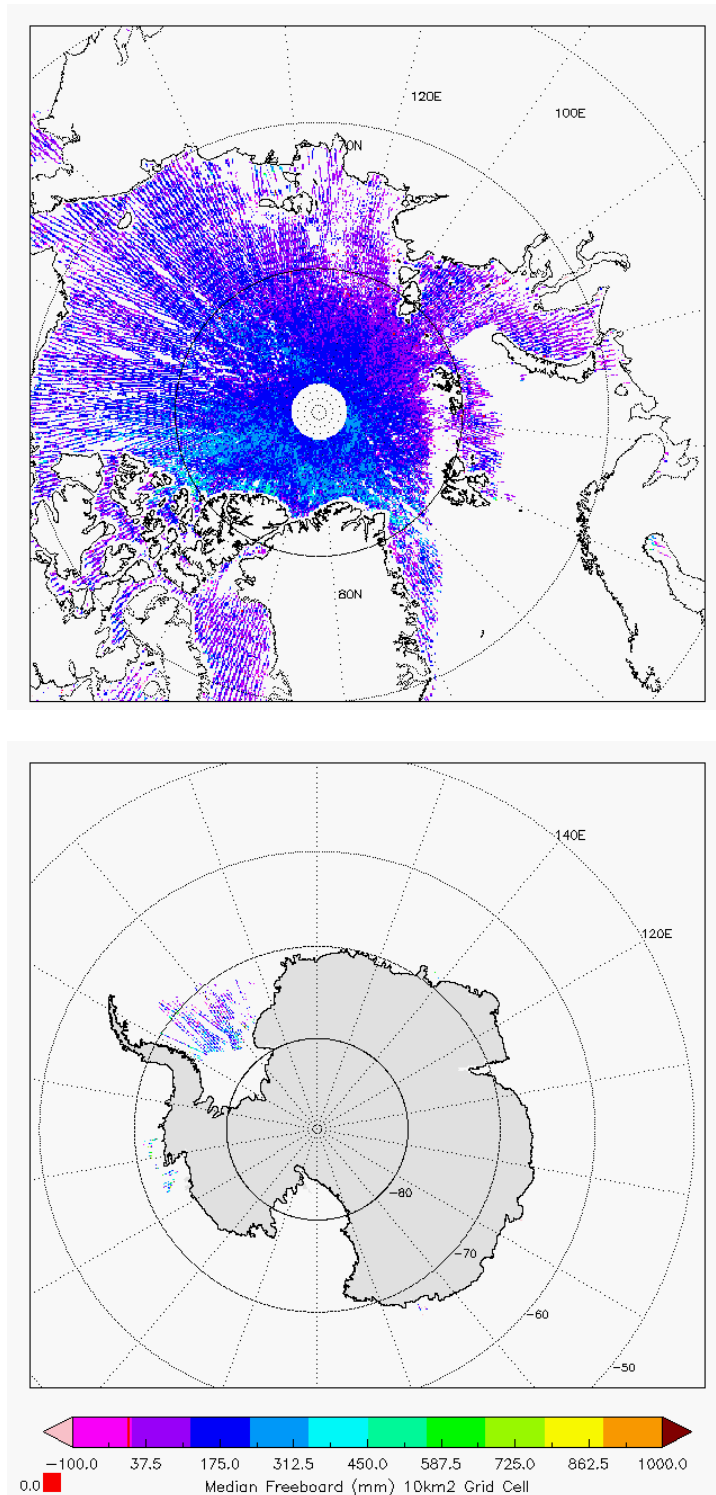
Figure 6 - Polar plots of 10km Gridded Freeboard values from L2 SAR products in cycle #139.
