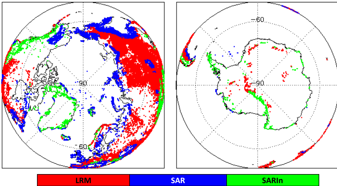
Figure 2 - Polar plots showing areas of loss of track in all SIRAL modes L0 data during March 2022.
