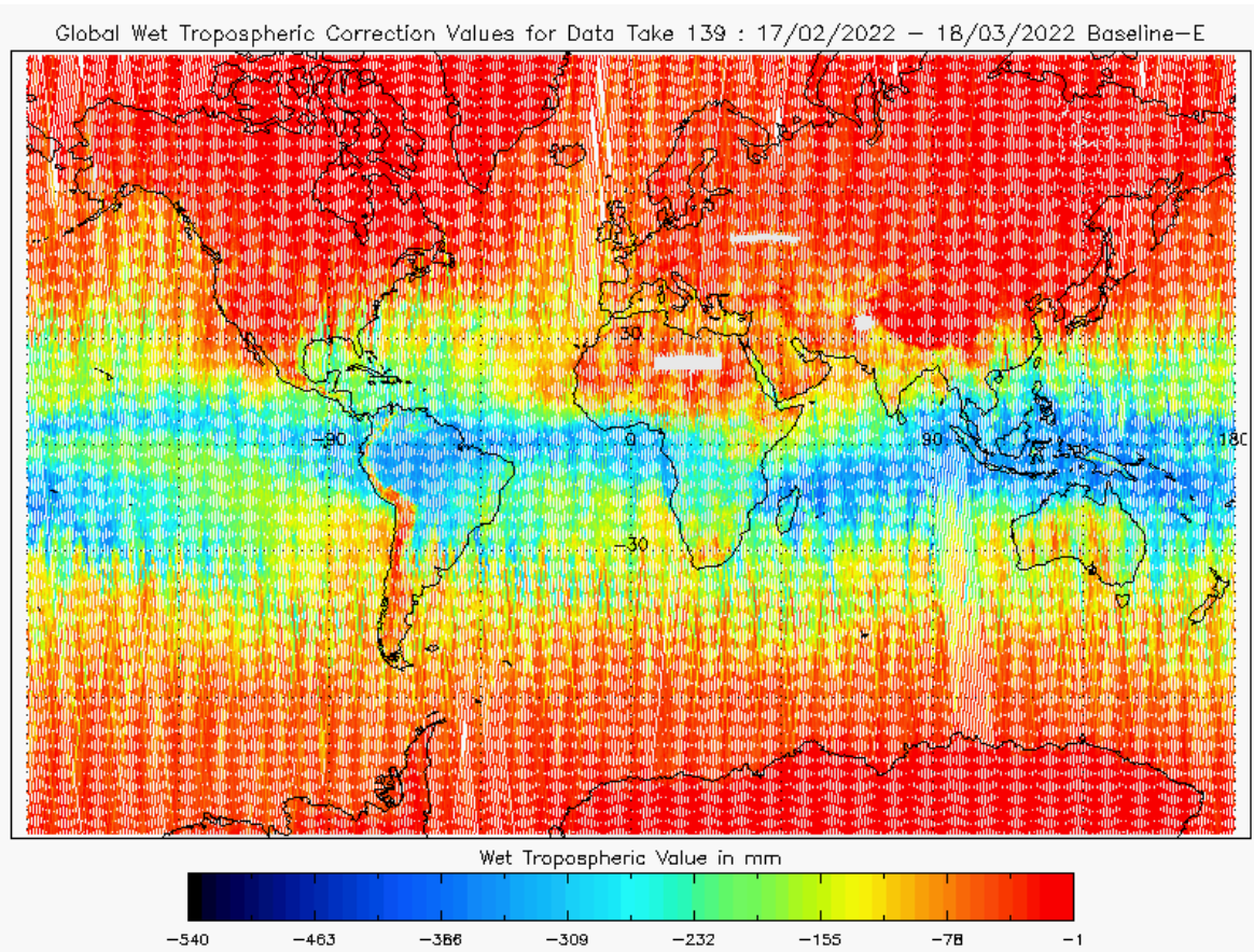
Figure 18 - Global plot of Wet Tropospheric Correction for cycle #139
