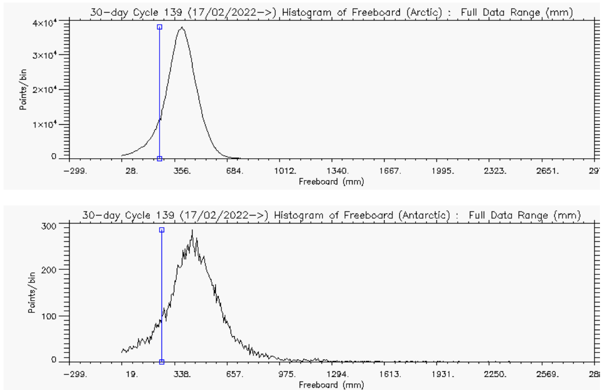
Figure 5 – Histogram of Freeboard for Arctic (above) and Antarctic (below) for cycle #139
