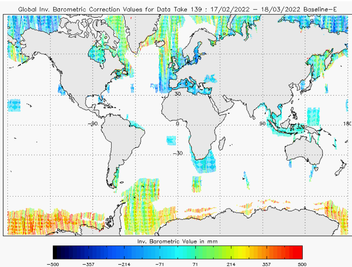
Figure 20 - Global plot of Inverse Barometric Correction for cycle #139
