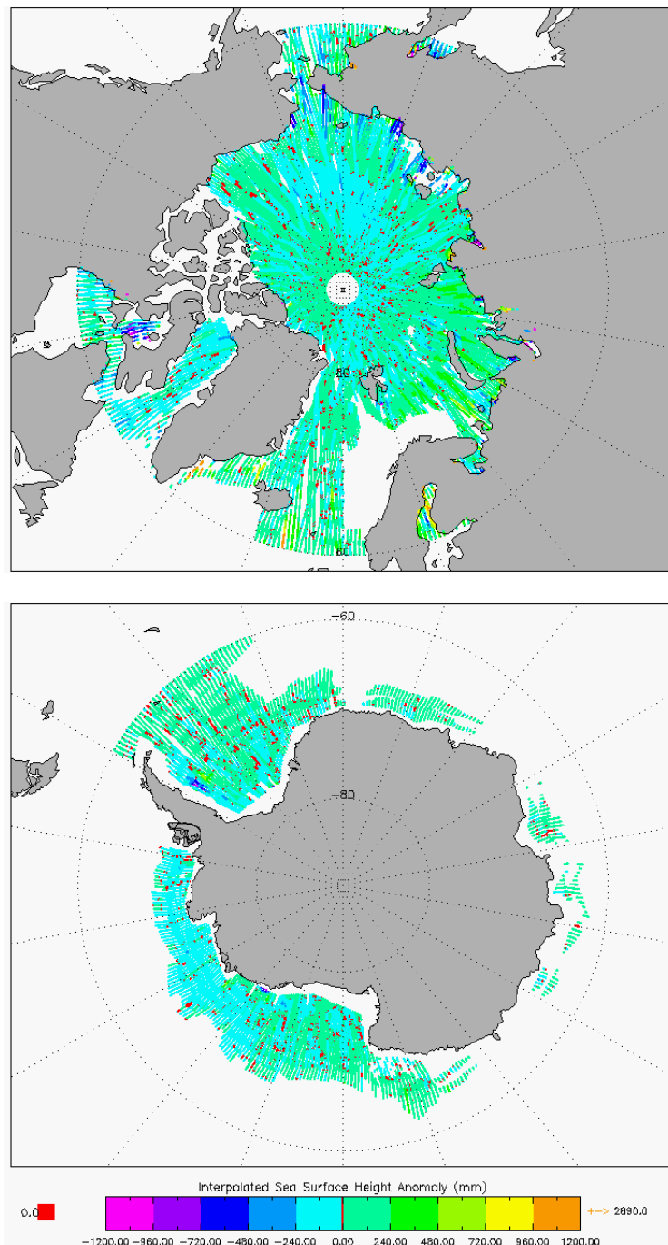
Figure 7 –Polar plots of SSHA for cycle #139.
