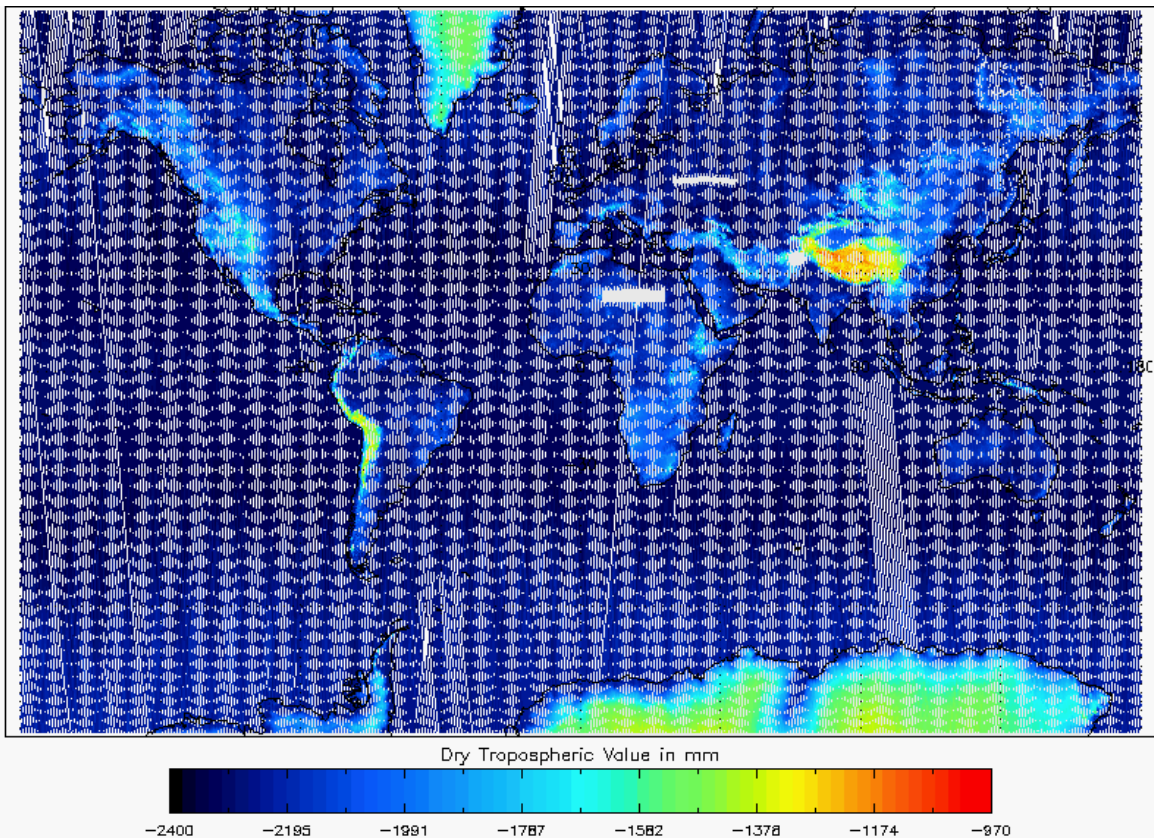
Figure 16 - Global plot of Dry Tropospheric Correction for cycle #139
