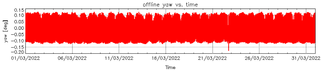
Figure 4 – Roll (top), Pitch (middle) and Yaw (bottom) values for L1B Products during cycle #139.
