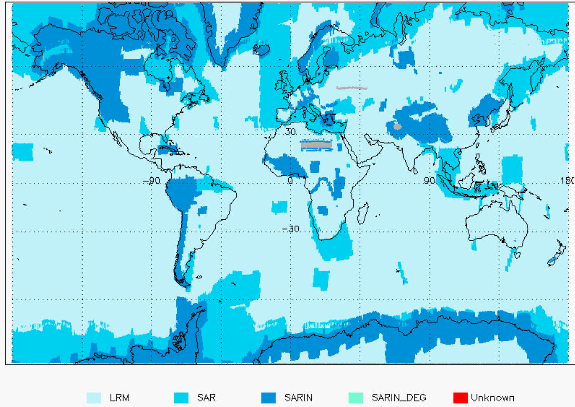
Figure 3 - Global and Polar plots of SIRAL Modes for cycle #139.
