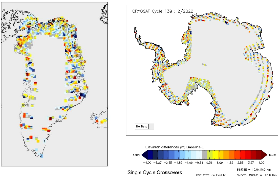
Figure 15 - Greenland and Antarctica maps of SARIn elevation differences for cycle #139.
