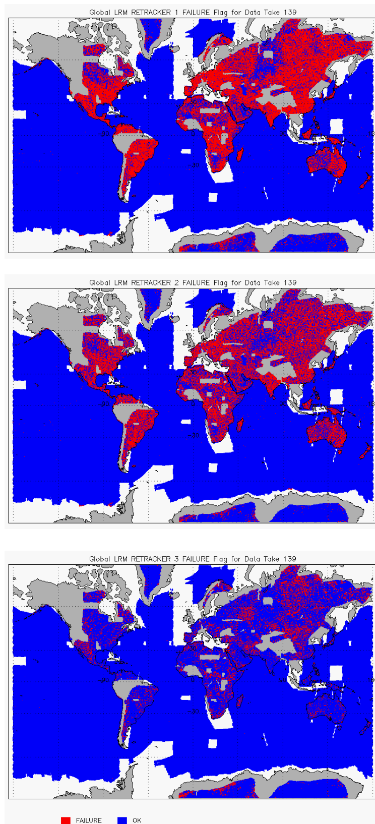
Figure 9 – Global plots showing Retracker Failure Flags for LRM mode for cycle #139:
