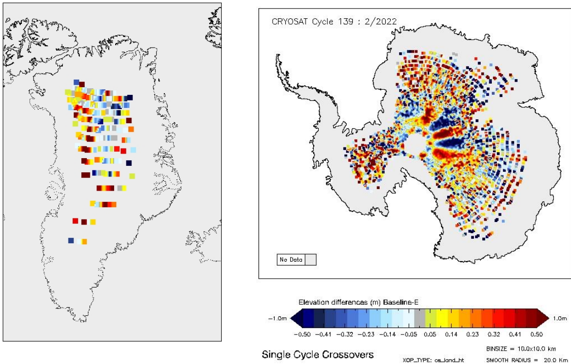
Figure 14 - Greenland and Antarctica maps of LRM elevation differences for cycle #139.
