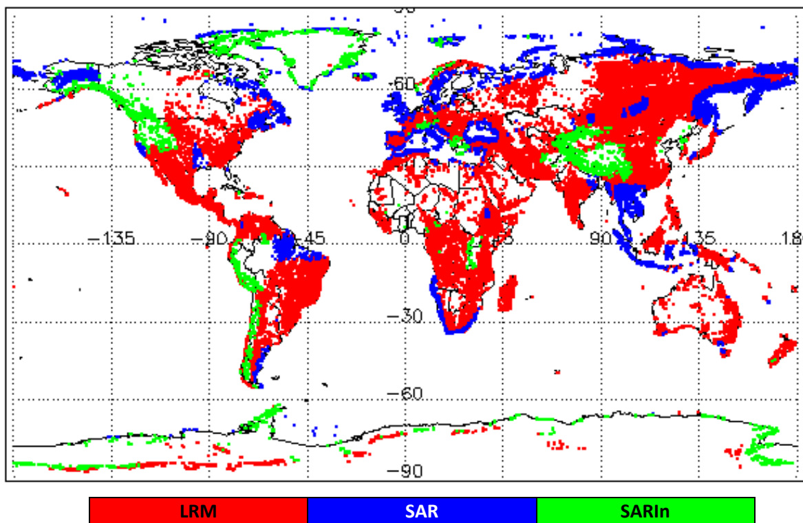
Figure 1 – Global plot showing areas of loss of track in all SIRAL modes L0 data during March 2022
