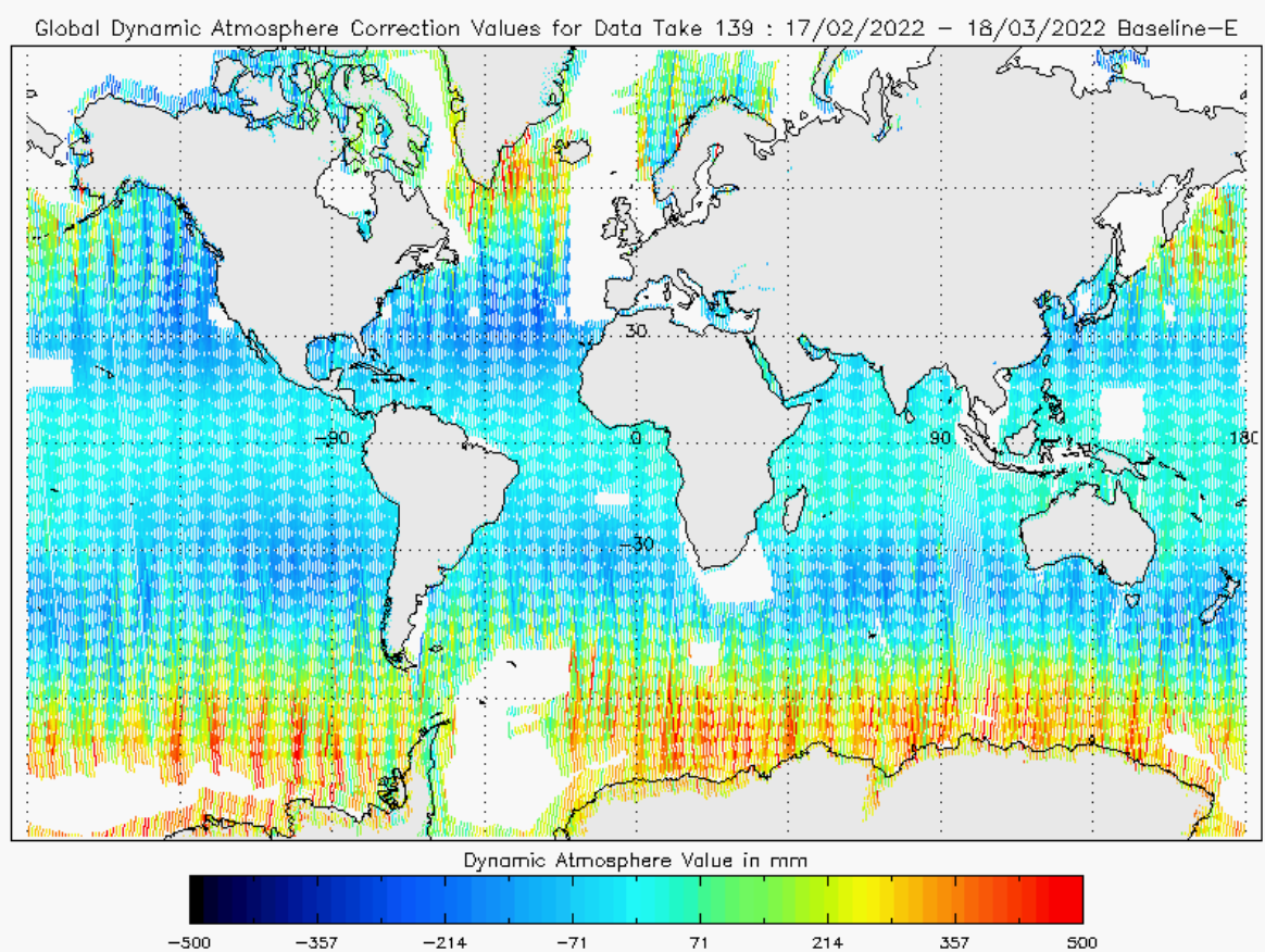
Figure 22 - Global plot of Dynamic Atmospheric Correction for cycle #139
