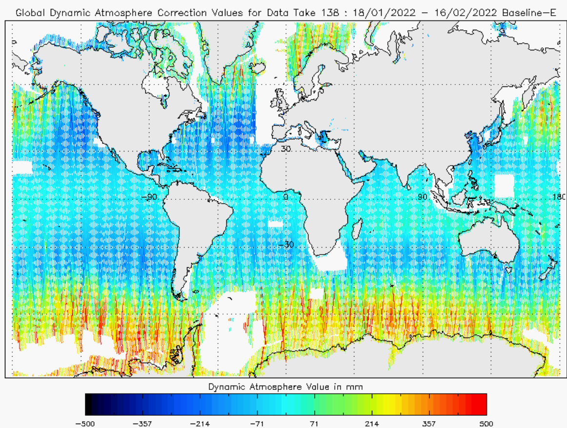
Figure 22 - Global plot of Dynamic Atmospheric Correction for cycle #138
