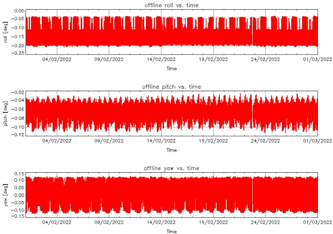
Figure 4 – Roll (top), Pitch (middle) and Yaw (bottom) values for L1B Products during cycle #138.
