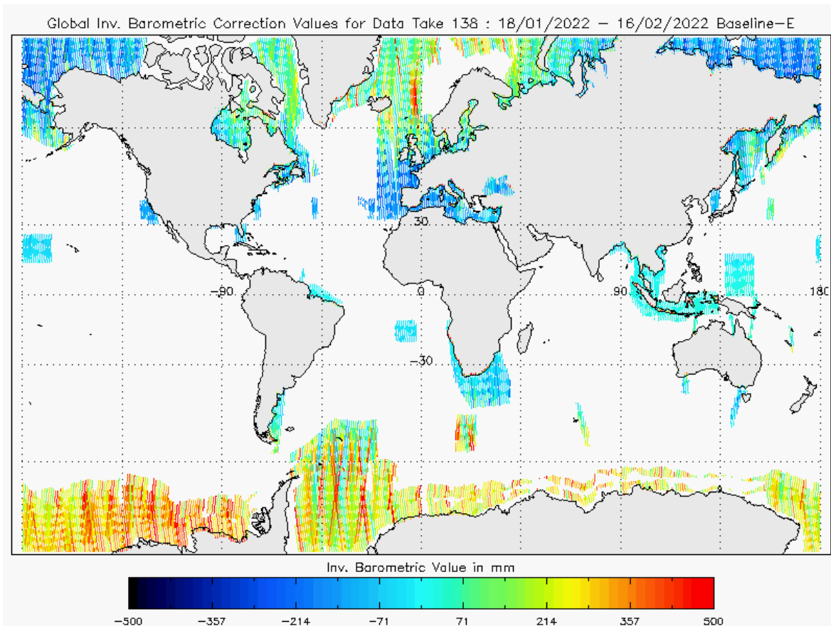
Figure 20 - Global plot of Inverse Barometric Correction for cycle #138
