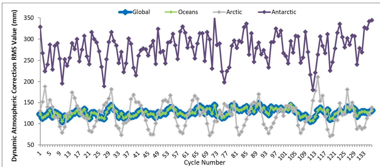
Figure 24 – Dynamic Atmospheric Correction RMS value trend from beginning of mission
