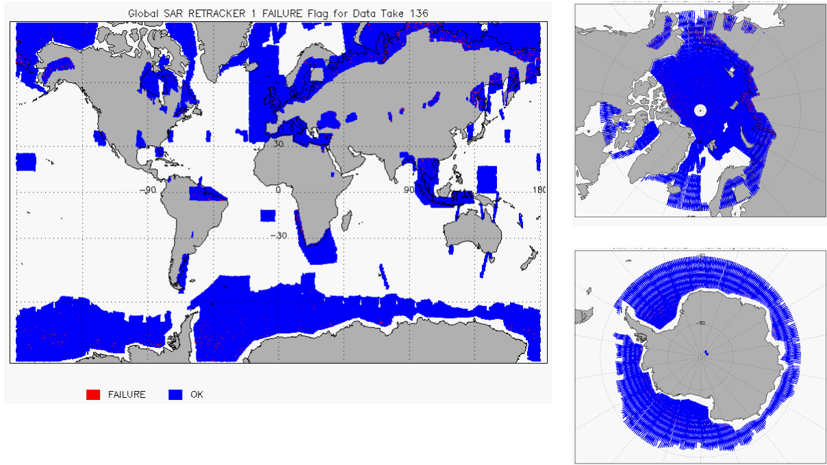
Figure 11 - Global plots showing Retracker Failure Flags for SAR mode for cycle #136
