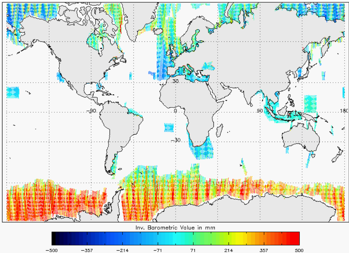
Figure 21 - Global plot of Inverse Barometric Correction for cycle #136
