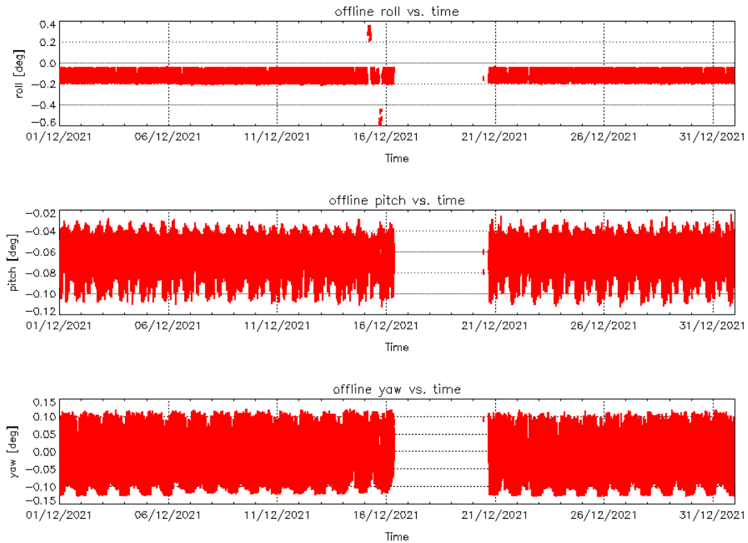
Figure 4 – Roll (top), Pitch (middle) and Yaw (bottom) values for L1B Products during cycle #136.
