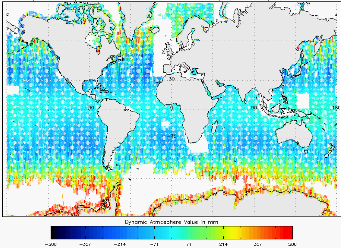
Figure 23 - Global plot of Dynamic Atmospheric Correction for cycle #136
