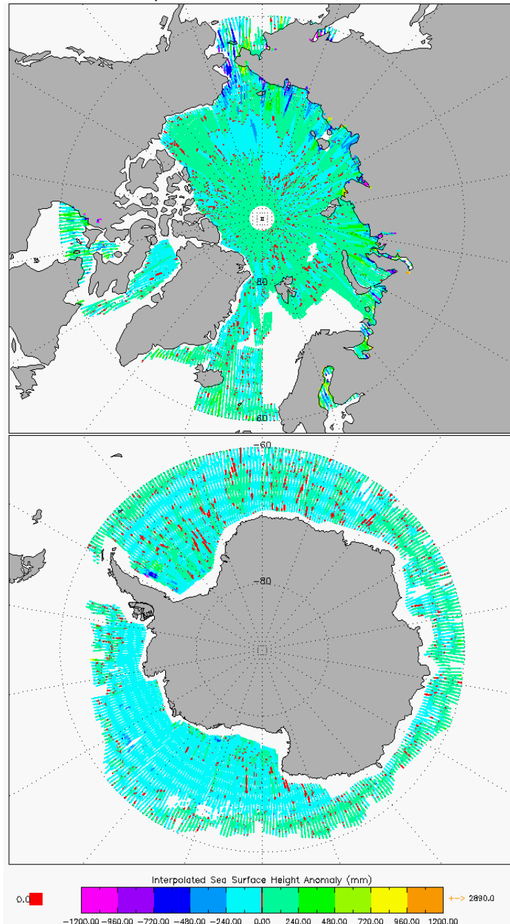
Figure 8 –Polar plots of SSHA for cycle #136.
