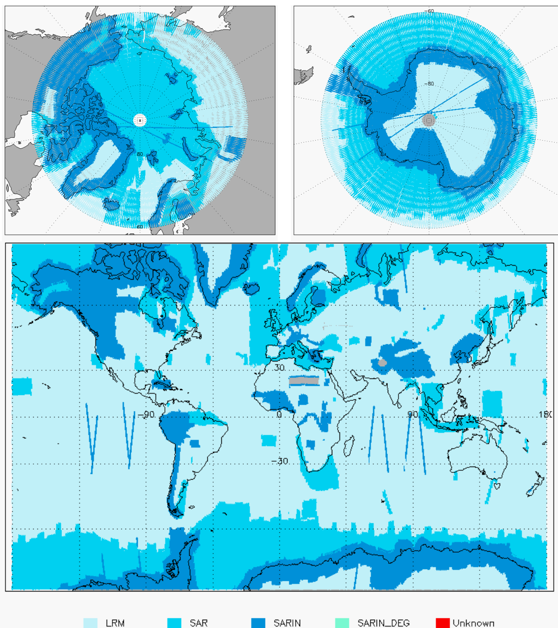
Figure 3 - Global and Polar plots of SIRAL Modes for cycle #136.
