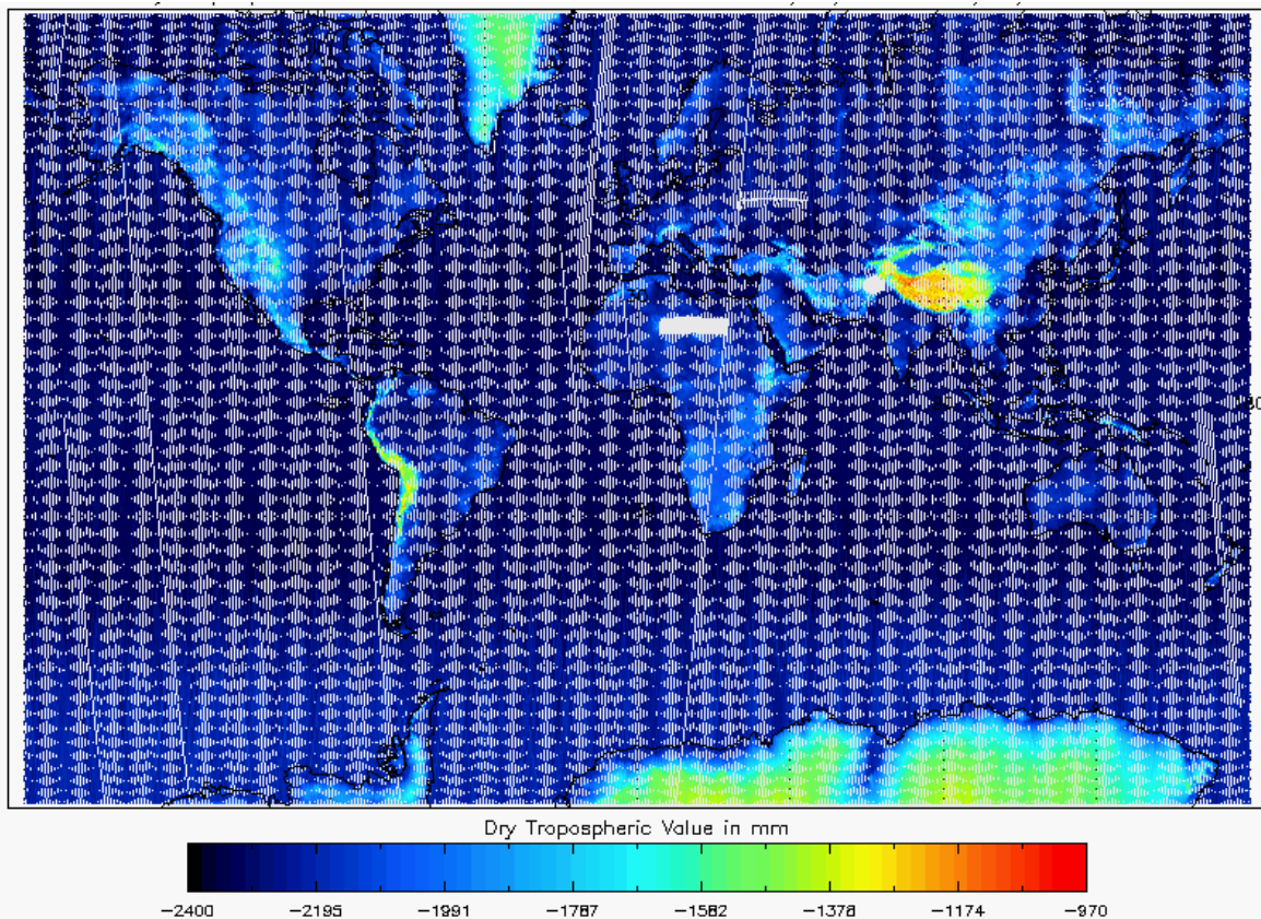
Figure 17 - Global plot of Dry Tropospheric Correction for cycle #136
