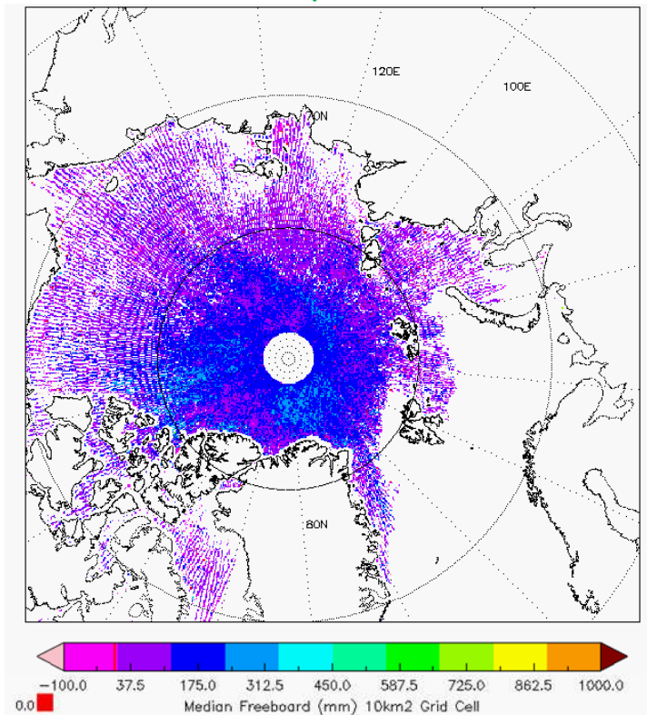
Figure 7 - Polar plots of 10km Gridded Freeboard values from L2 SAR products in cycle #136.
