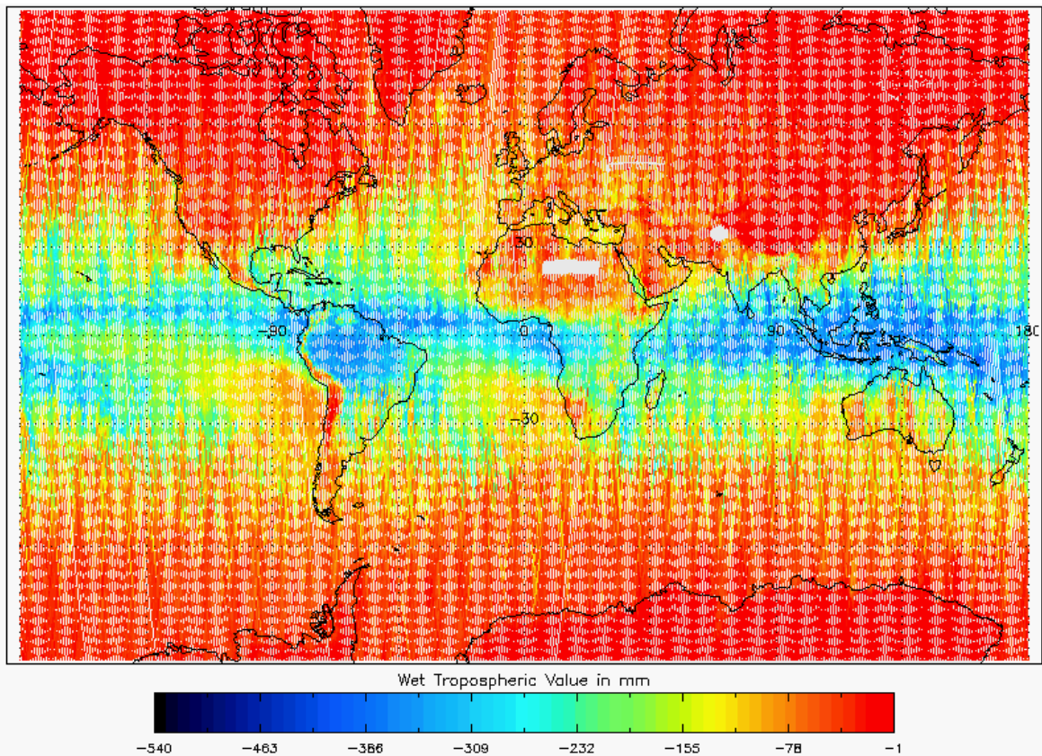
Figure 19 - Global plot of Wet Tropospheric Correction for cycle #136
