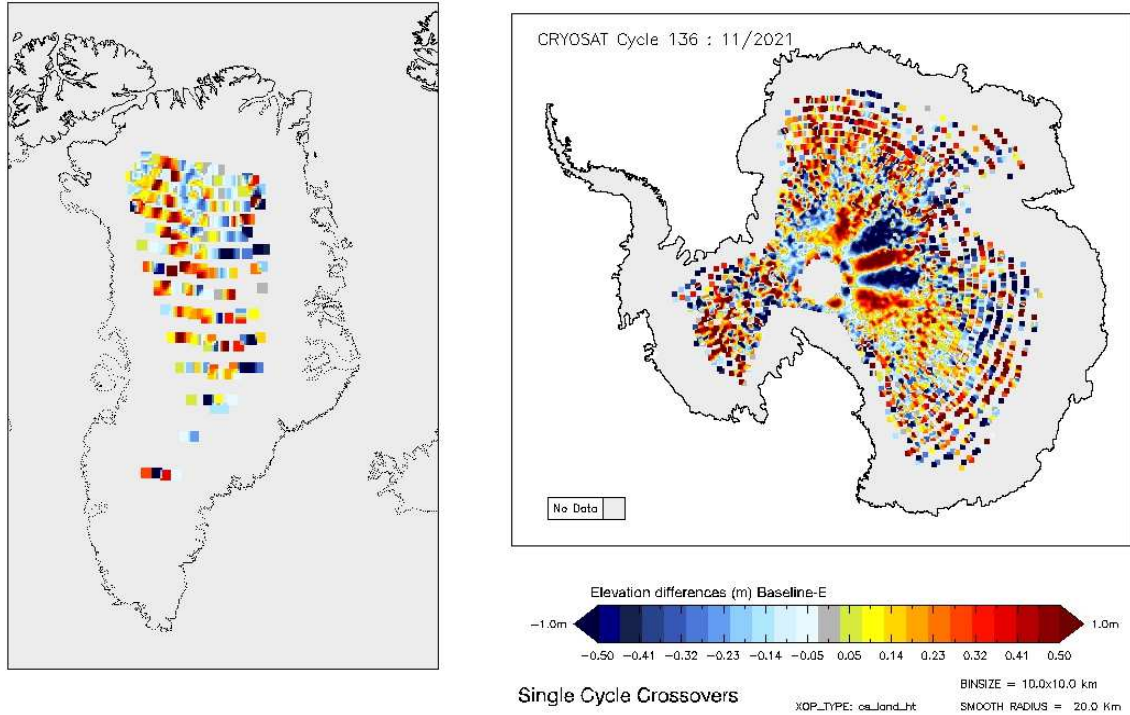
Figure 15 - Greenland and Antarctica maps of LRM elevation differences for cycle #136.
