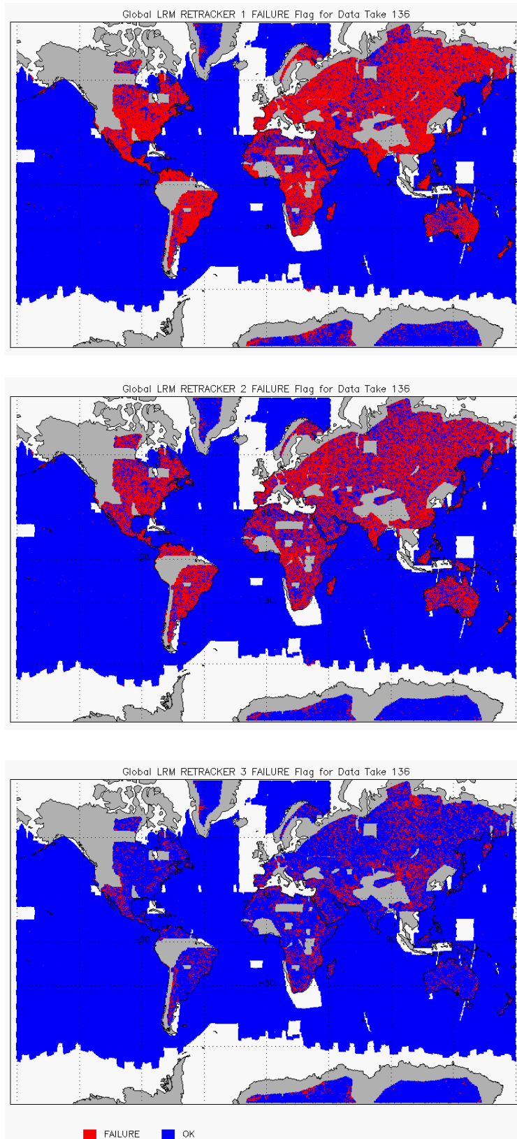
Figure 10 – Global plots showing Retracker Failure Flags for LRM mode for cycle #136: LRM CFI (top), LRM LIRT (middle), LRM OCOG (bottom)
