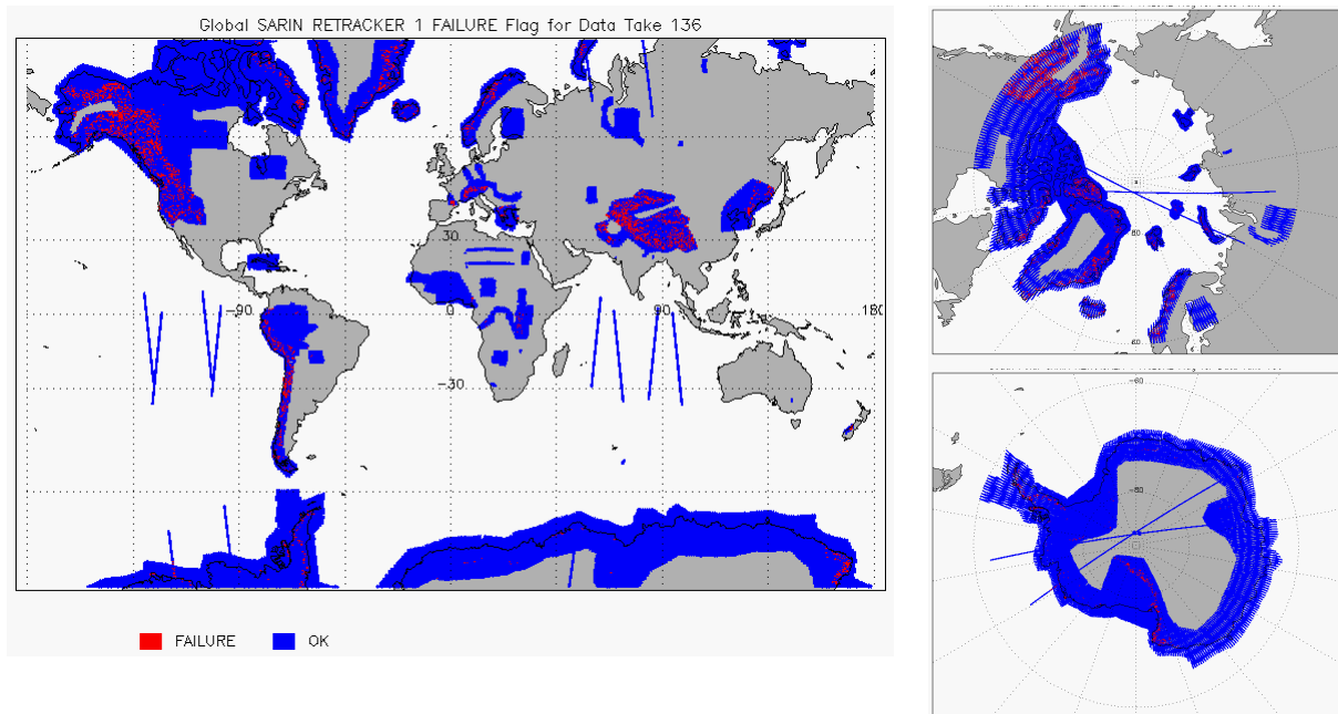
Figure 12 – Global plots showing Retracker Failure Flags for SARIn mode for cycle #136
