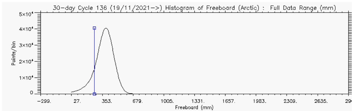
Figure 6 – Histogram of Freeboard for Arctic (above) and Antarctic (below) for cycle #136
