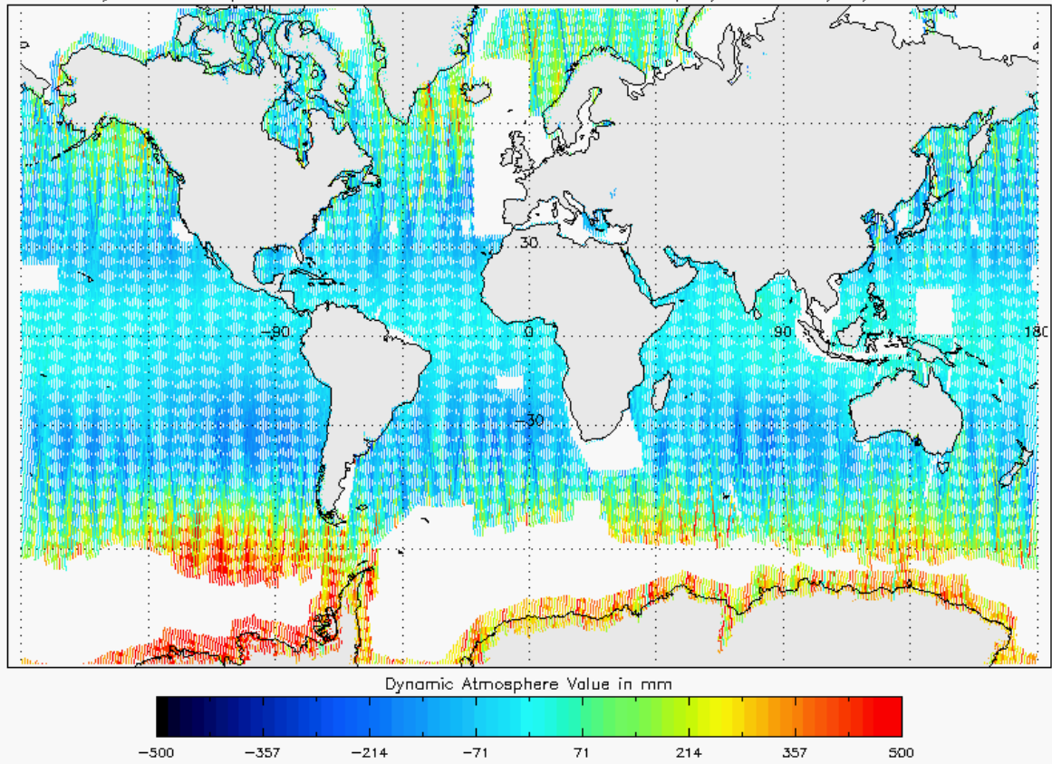
Figure 22 - Global plot of Dynamic Atmospheric Correction for cycle #135
