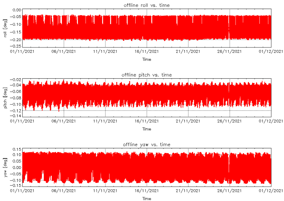
Figure 4 – Roll (top), Pitch (middle) and Yaw (bottom) values for L1B Products during cycle #135.
