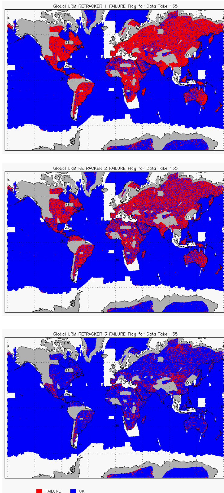
Figure 9 – Global plots showing Retracker Failure Flags for LRM mode for cycle #135: LRM CFI (top), LRM LIRT (middle), LRM OCOG (bottom)
