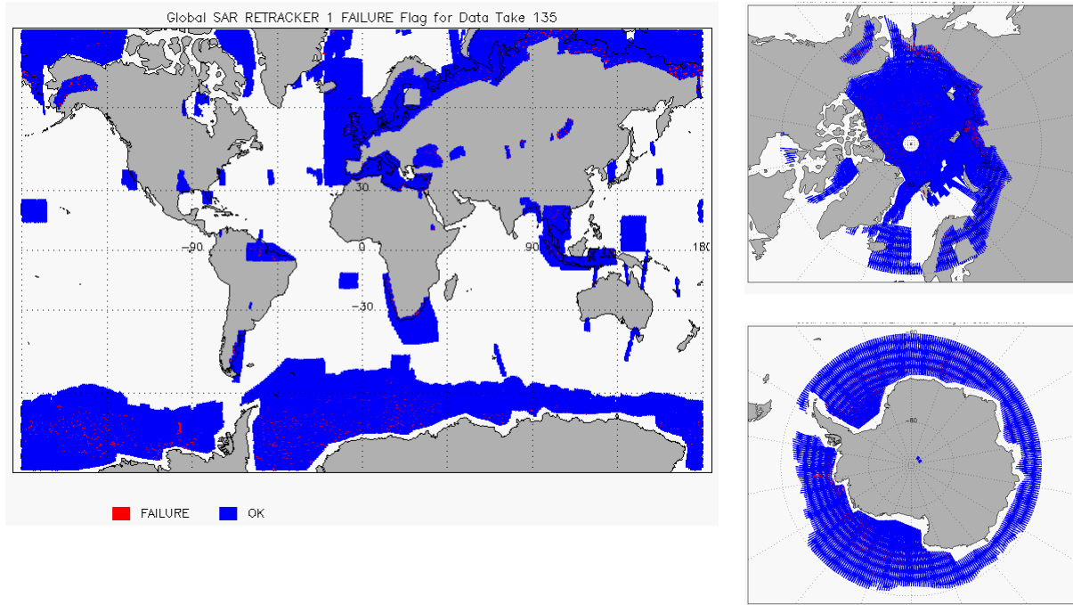
Figure 10 - Global plots showing Retracker Failure Flags for SAR mode for cycle #135
