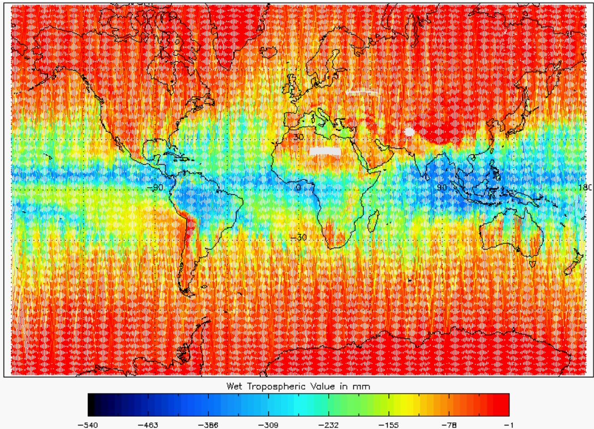
Figure 18 - Global plot of Wet Tropospheric Correction for cycle #135
