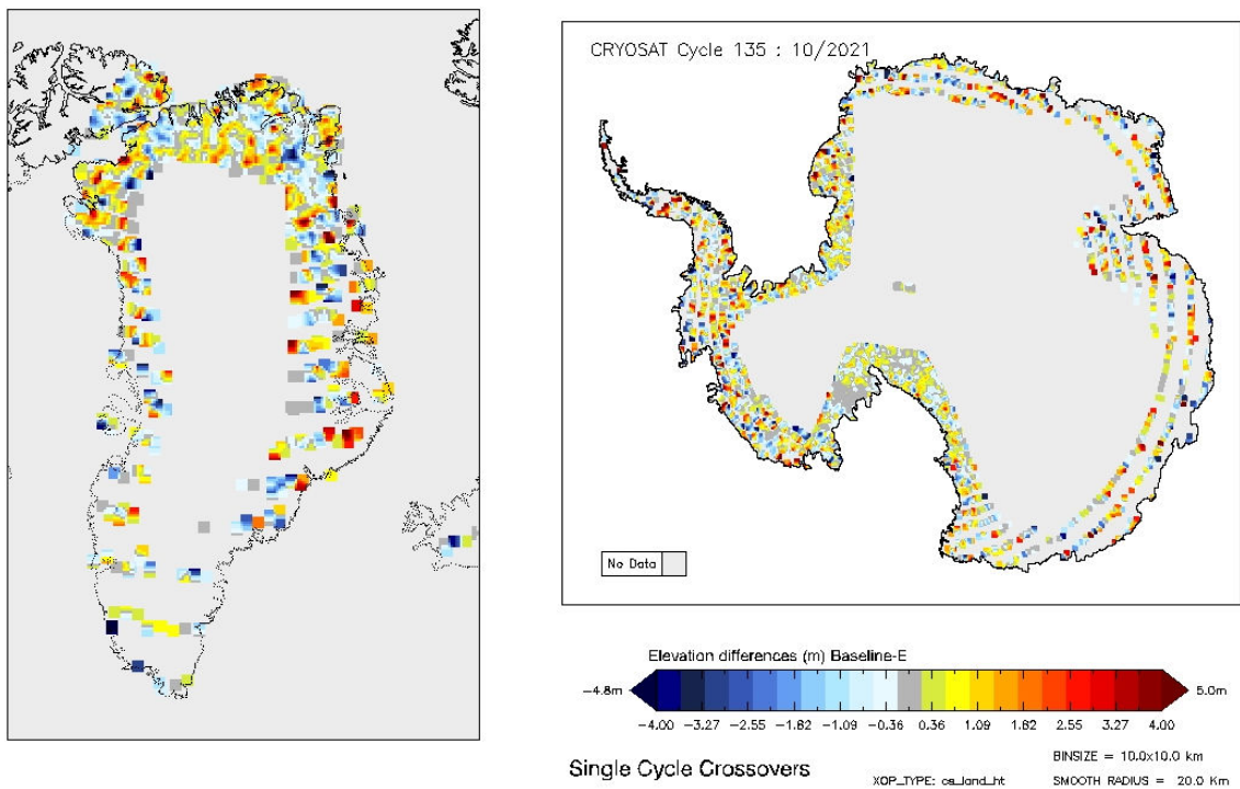
Figure 15 - Greenland and Antarctica maps of SARIn elevation differences for cycle #135.
