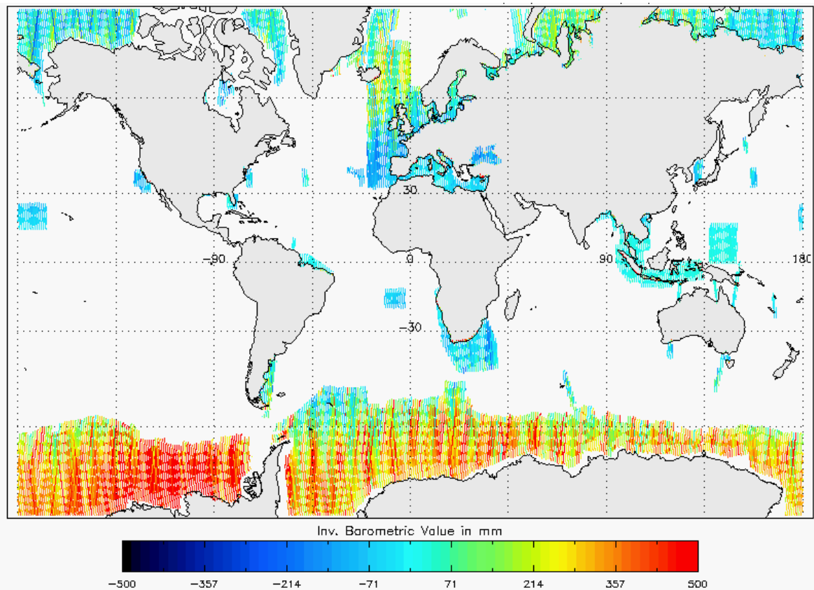
Figure 20 - Global plot of Inverse Barometric Correction for cycle #135
