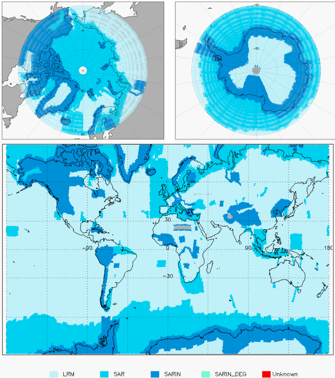
Figure 3 - Global and Polar plots of SIRAL Modes for cycle #135.
