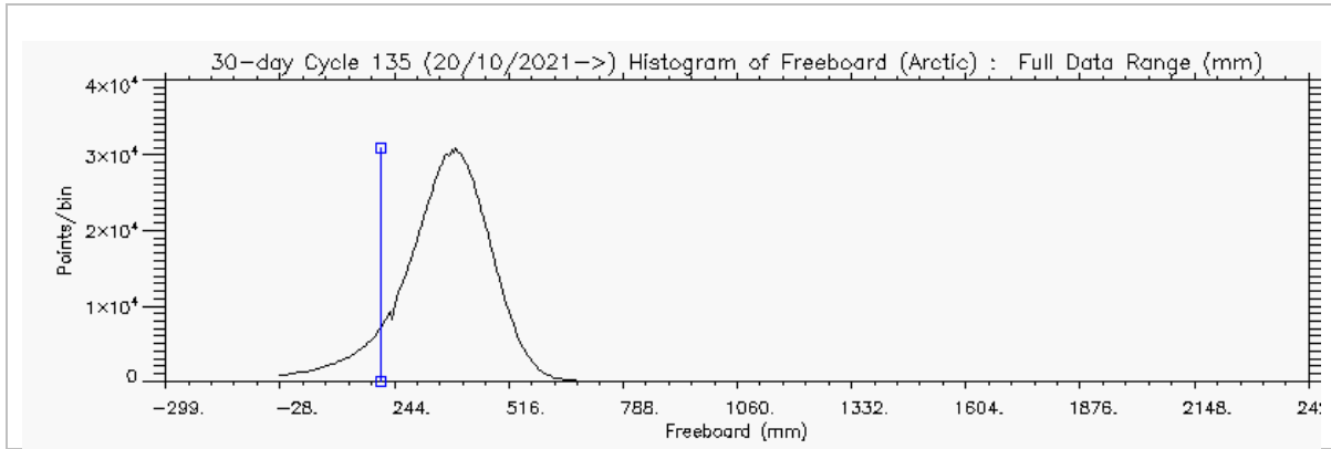
Figure 5 – Histogram of Freeboard for Arctic (above) and Antarctic (below) for cycle #135
