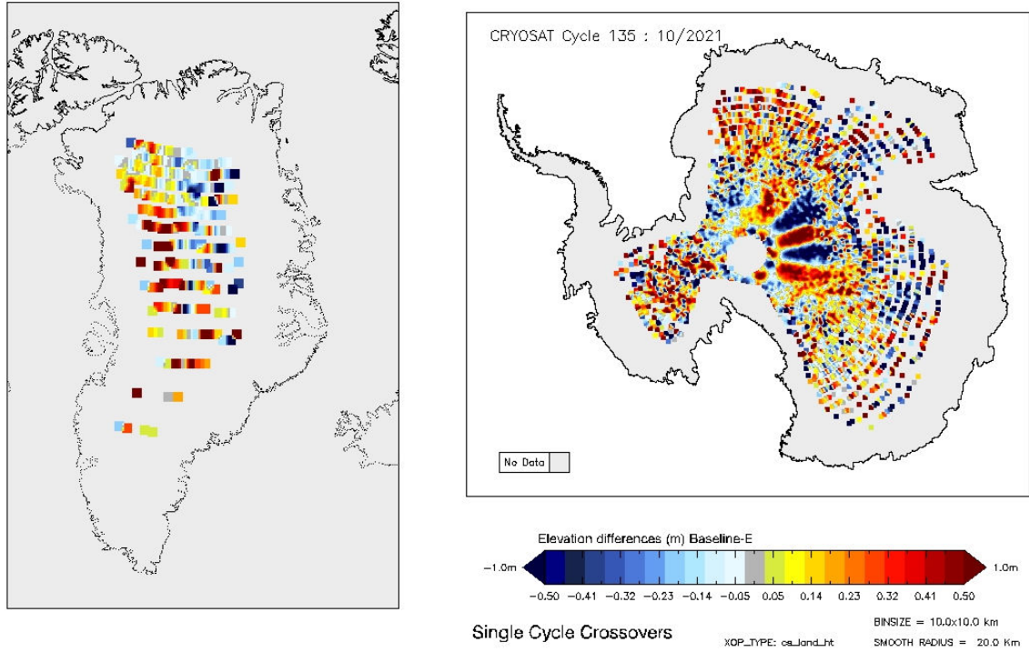
Figure 14 - Greenland and Antarctica maps of LRM elevation differences for cycle #135.
