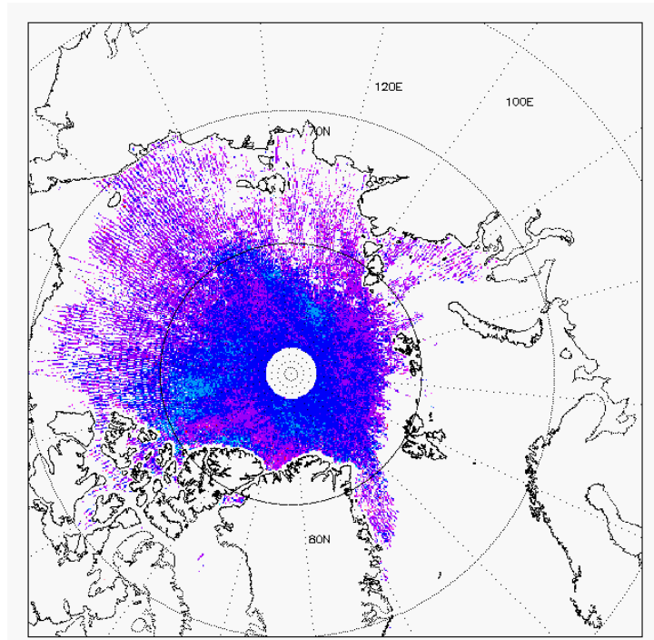
Figure 6 - Polar plots of 10km Gridded Freeboard values from L2 SAR products in cycle #135.
