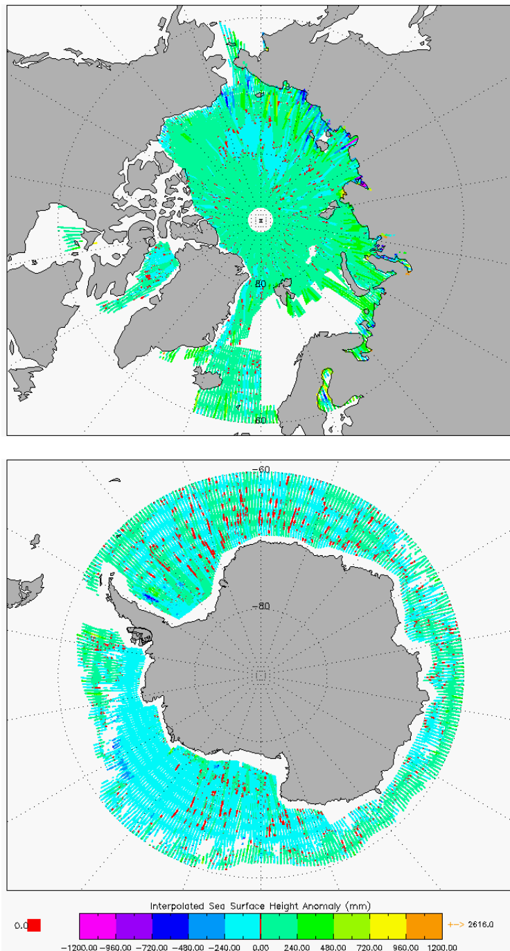
Figure 7 –Polar plots of SSHA for cycle #135.
