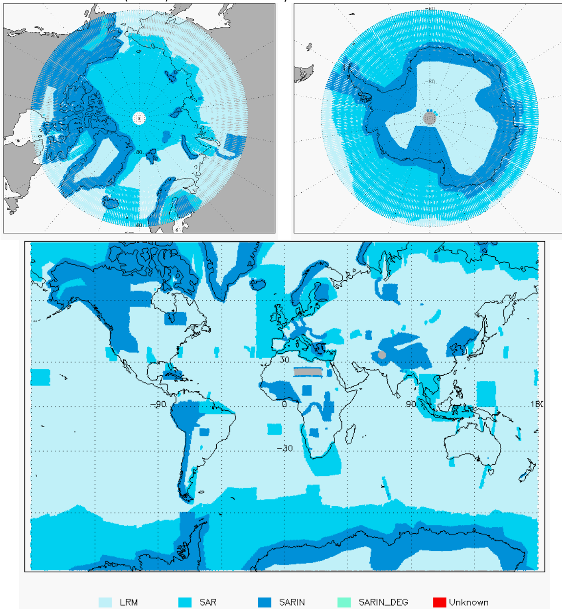
Figure 3 - Global and Polar plots of SIRAL Modes for cycle #133.
