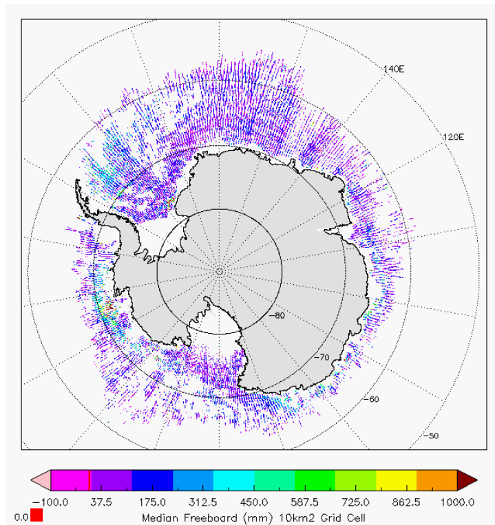
Figure 6 - Polar plots of 10km Gridded Freeboard values from L2 SAR products in cycle #133.
