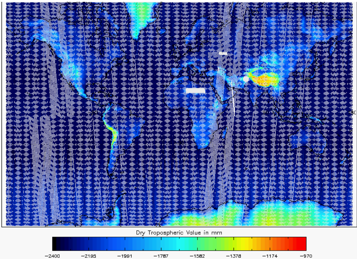
Figure 16 - Global plot of Dry Tropospheric Correction for cycle #133
