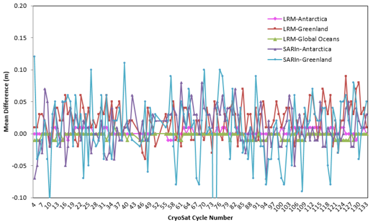
Figure 13 - Time series for Mean Difference in elevation at crossovers from beginning of the mission
