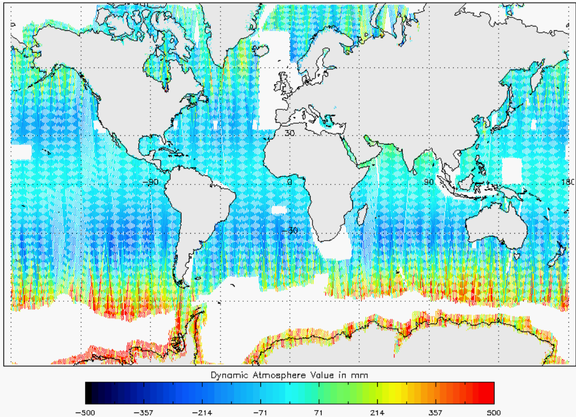
Figure 22 - Global plot of Dynamic Atmospheric Correction for cycle #133
