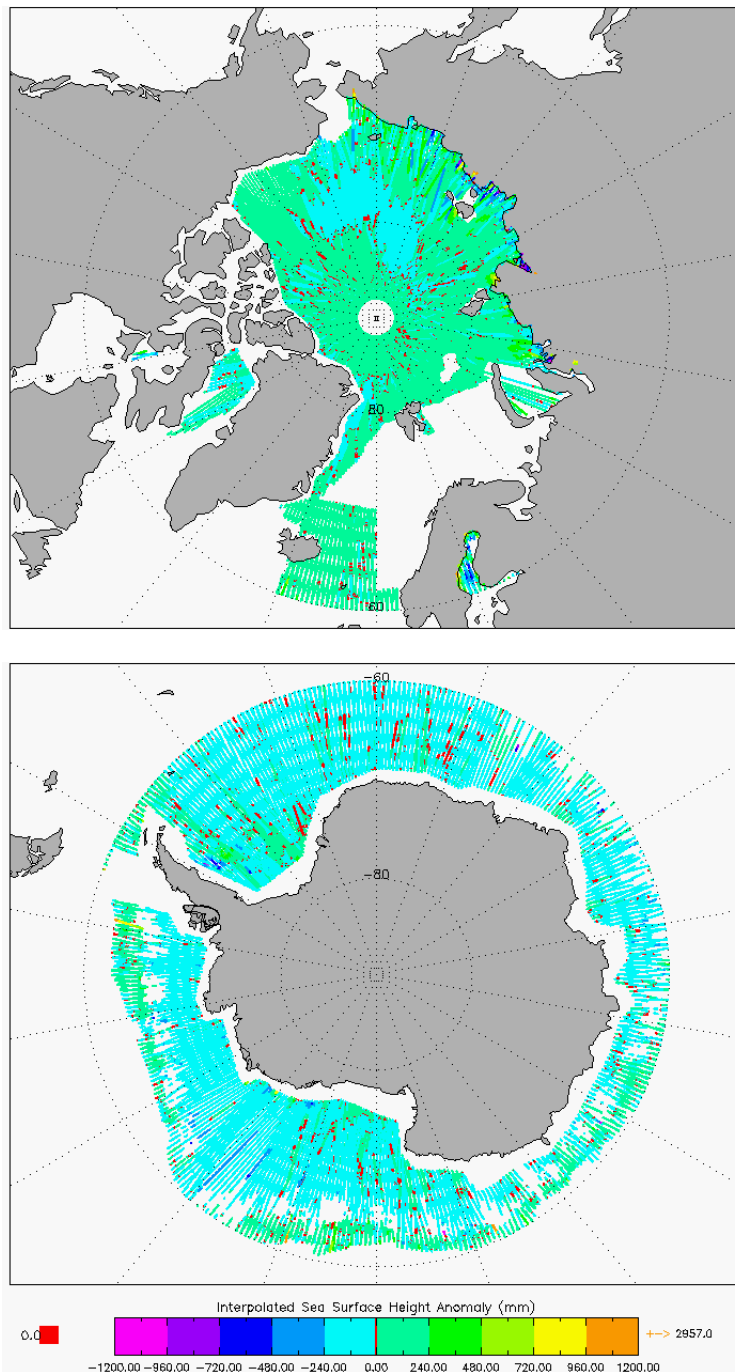
Figure 7 –Polar plots of SSHA for cycle #133.
