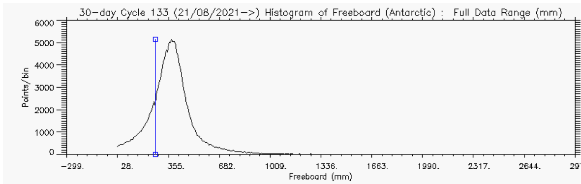
Figure 5 – Histogram of Freeboard for Antarctic for cycle #133
