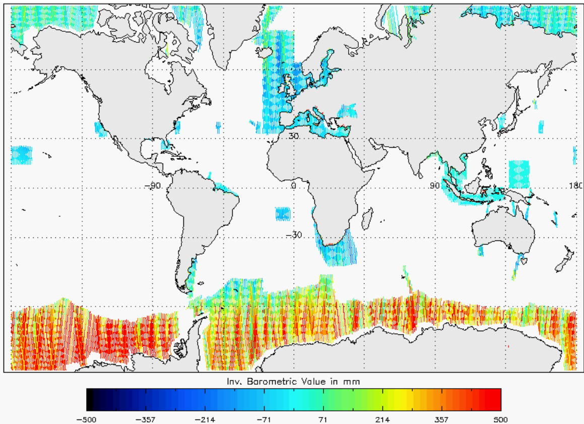
Figure 20 - Global plot of Inverse Barometric Correction for cycle #133
