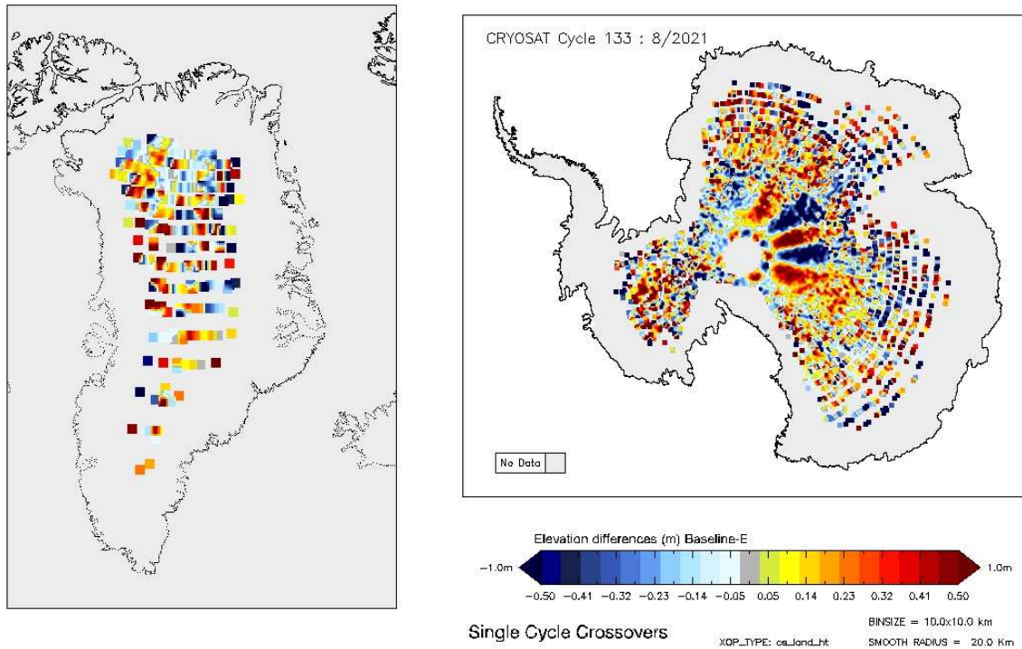
Figure 14 - Greenland and Antarctica maps of LRM elevation differences for cycle #133.
