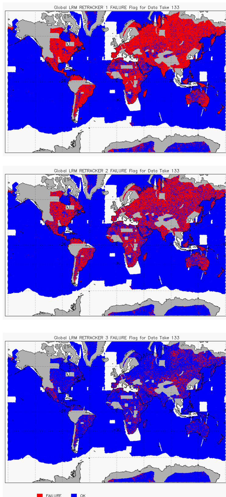
Figure 9 – Global plots showing Retracker Failure Flags for LRM mode for cycle #133:
