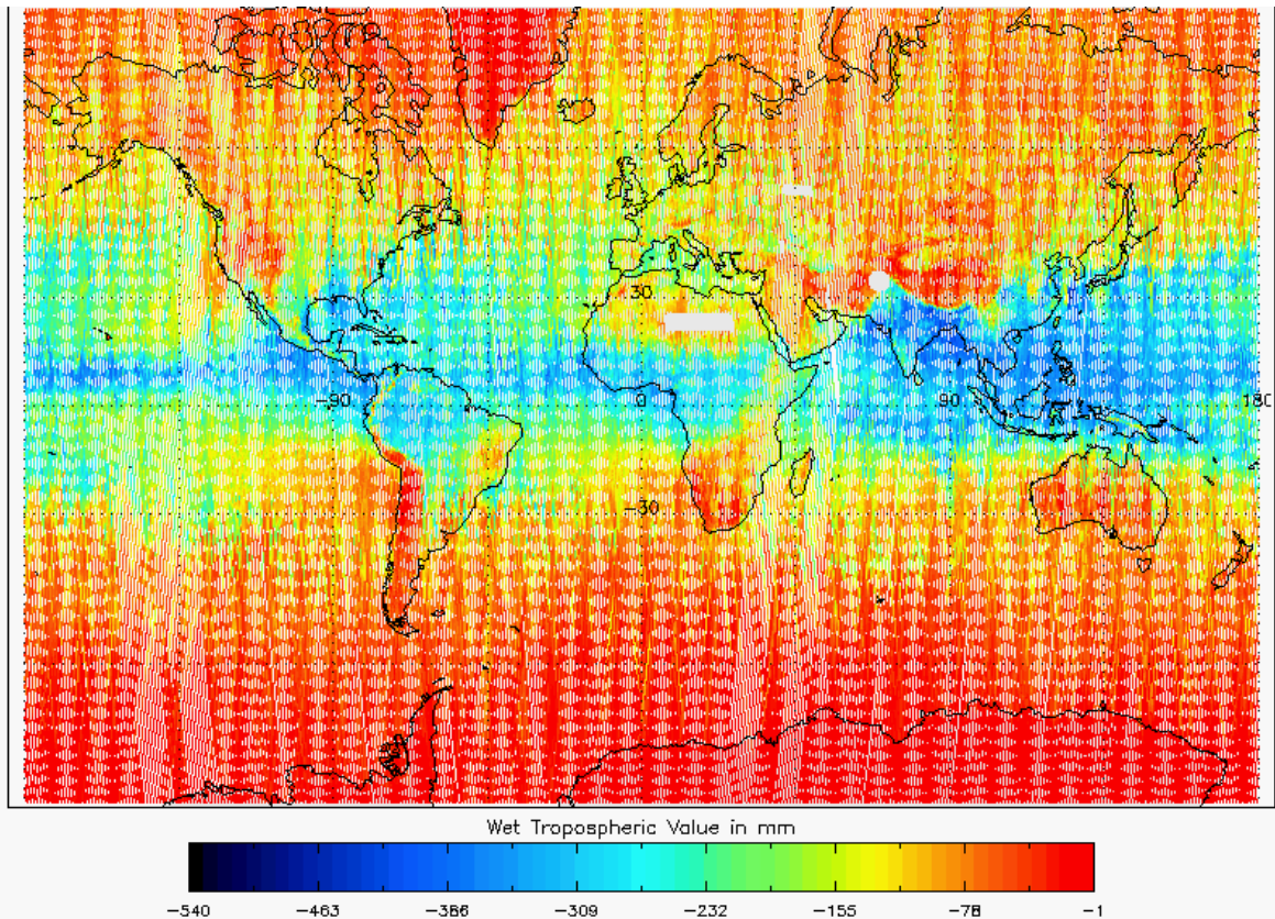
Figure 18 - Global plot of Wet Tropospheric Correction for cycle #133
