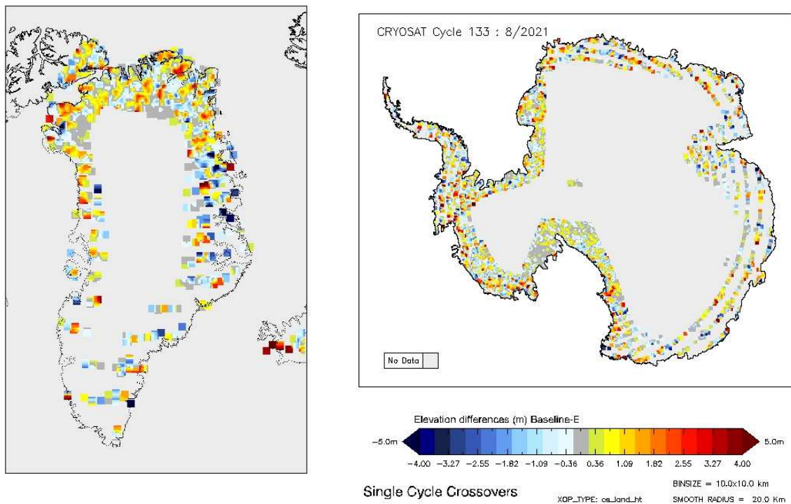
Figure 15 - Greenland and Antarctica maps of SARIn elevation differences for cycle #133.
