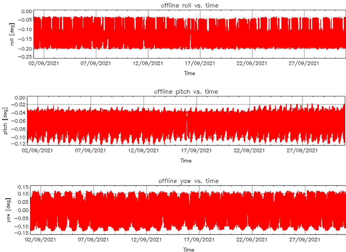
Figure 4 – Roll (top), Pitch (middle) and Yaw (bottom) values for L1B Products during cycle #133.
