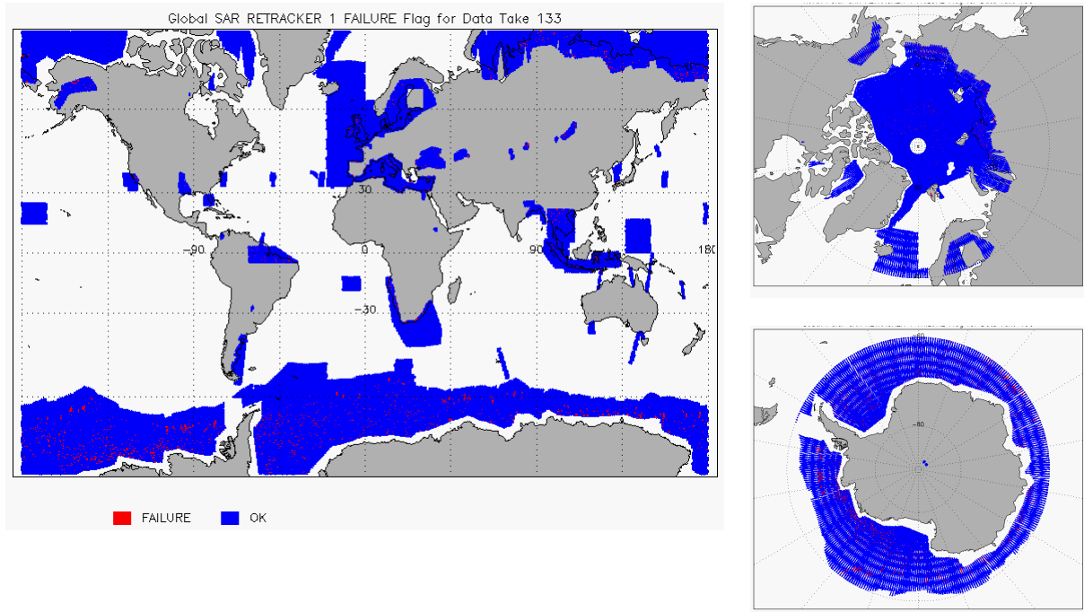
Figure 10 - Global plots showing Retracker Failure Flags for SAR mode for cycle #133
