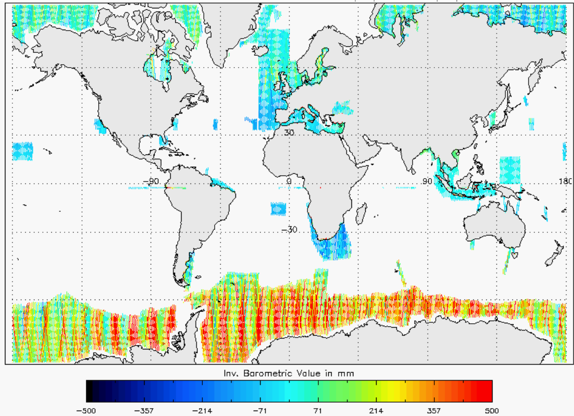
Figure 20 - Global plot of Inverse Barometric Correction for cycle #132
