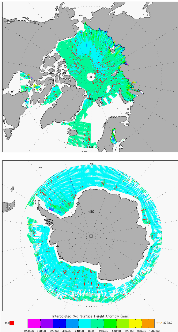
Figure 7 –Polar plots of SSHA for cycle #132.
