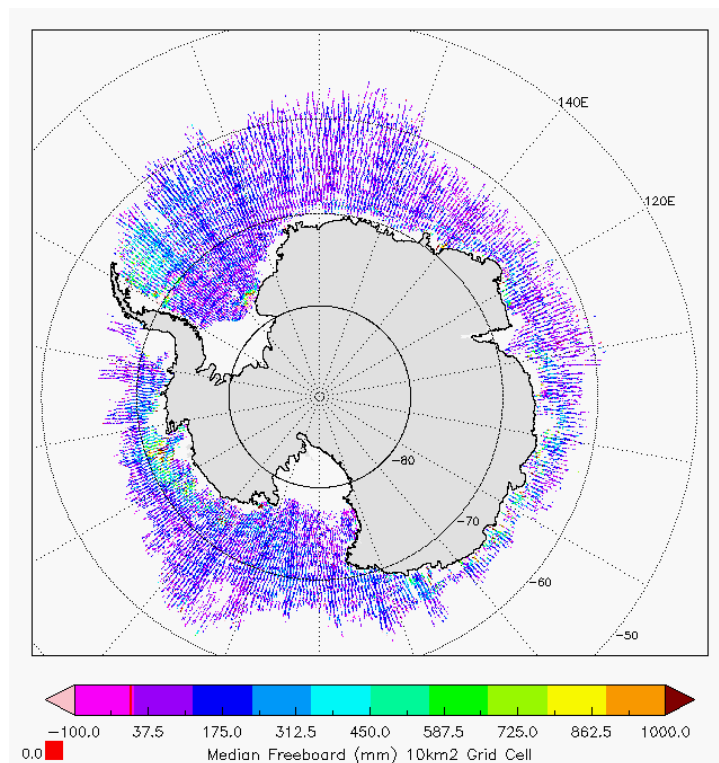
Figure 6 - Polar plots of 10km Gridded Freeboard values from L2 SAR products in cycle #132.
