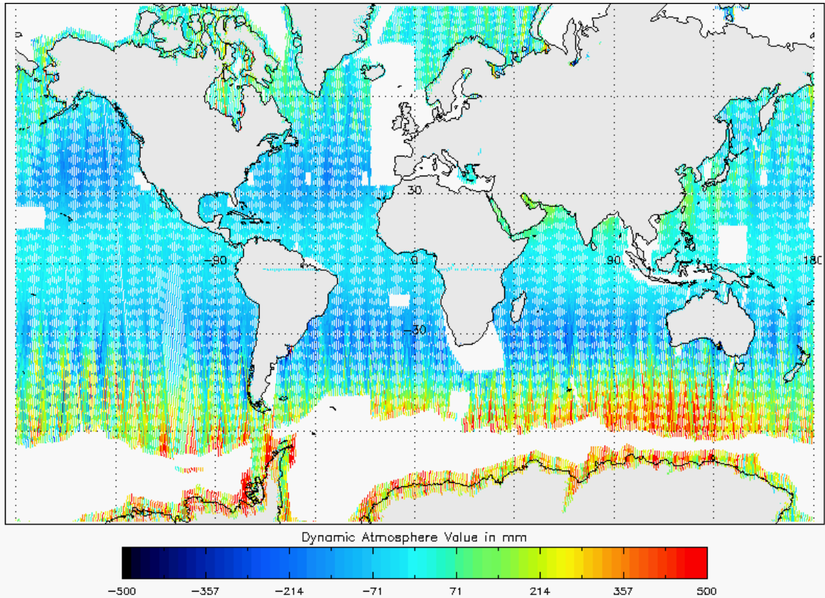
Figure 22 - Global plot of Dynamic Atmospheric Correction for cycle #132
