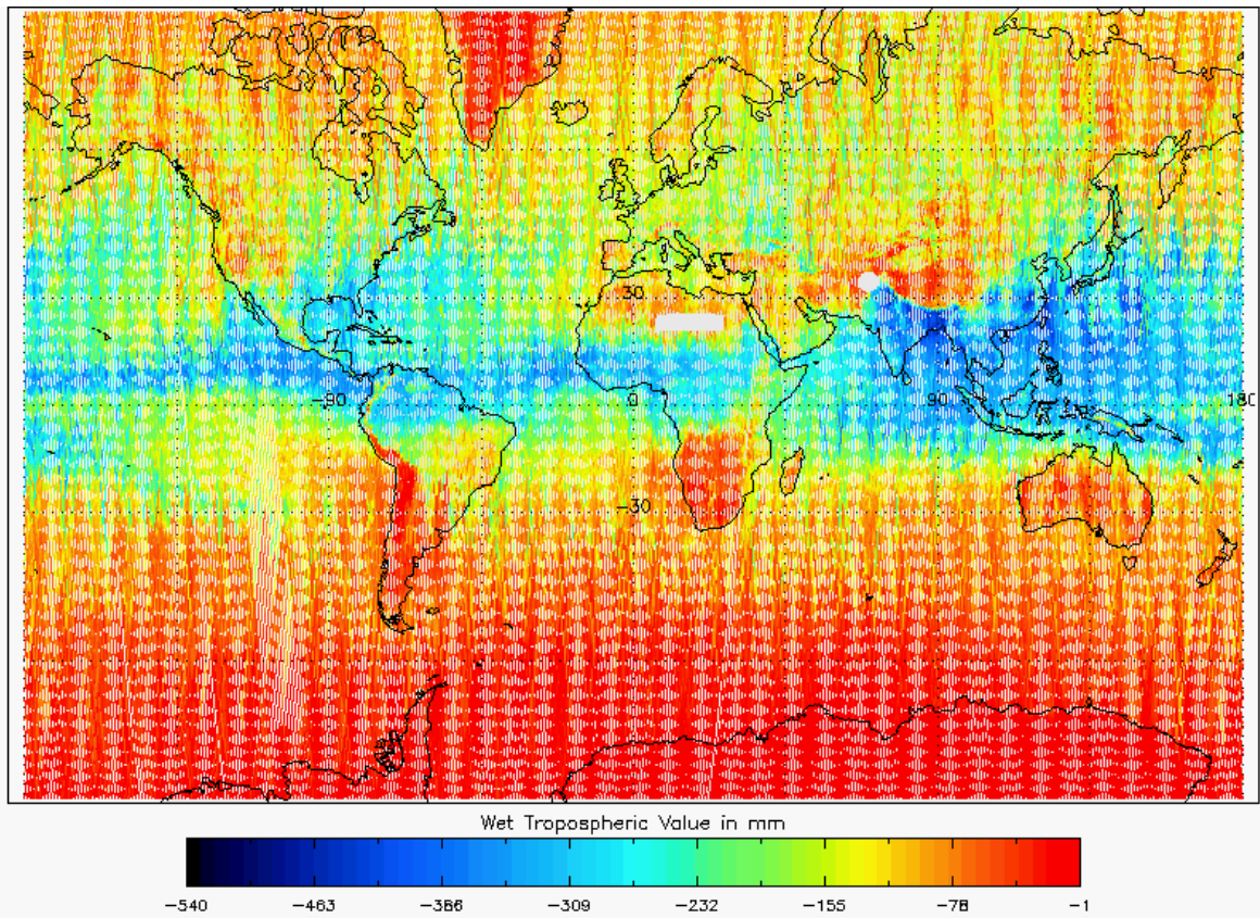
Figure 18 - Global plot of Wet Tropospheric Correction for cycle #132
