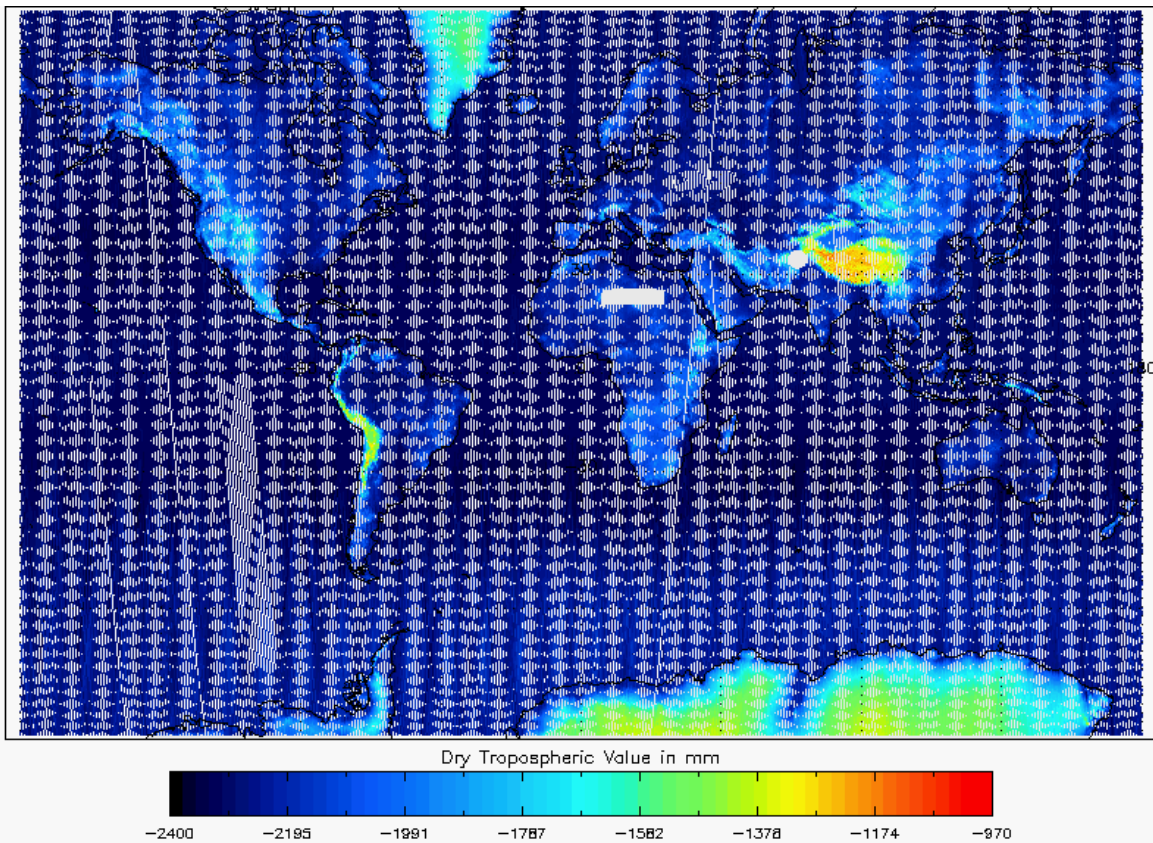
Figure 16 - Global plot of Dry Tropospheric Correction for cycle #132
