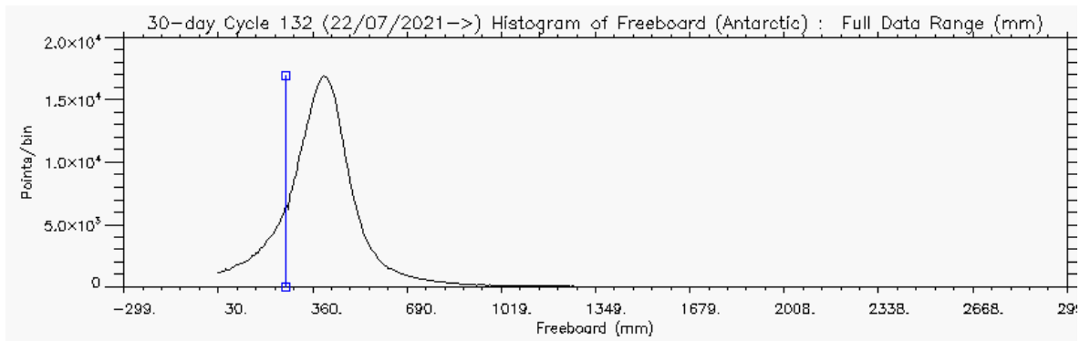
Figure 5 – Histogram of Freeboard for Arctic (above) and Antarctic (below) for cycle #132
