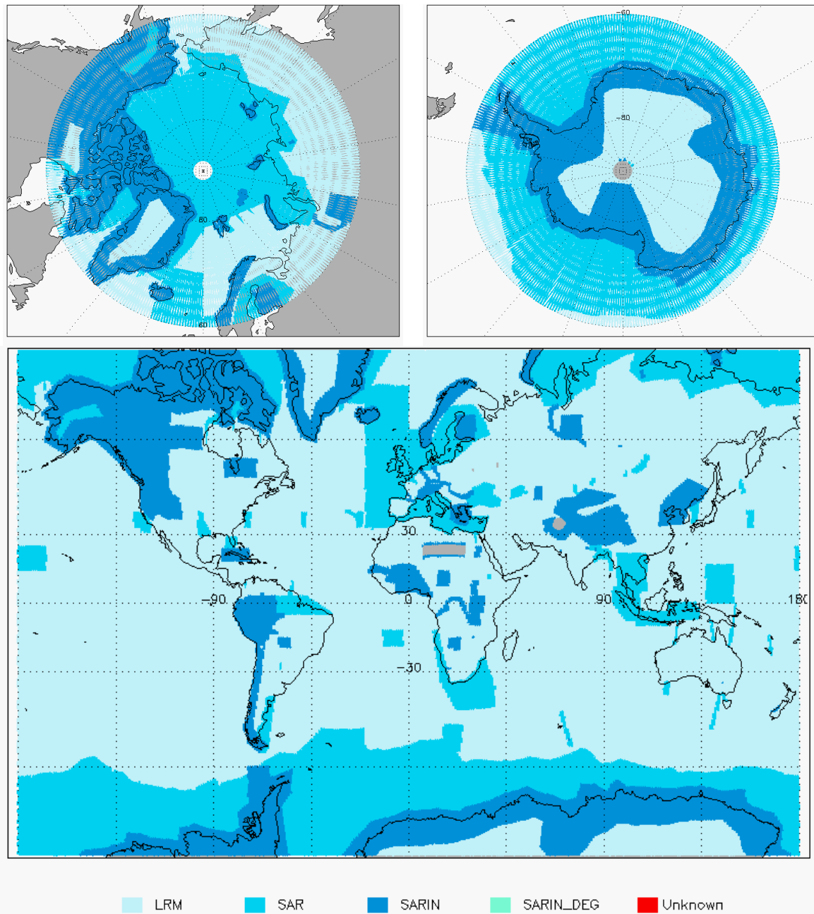
Figure 3 - Global and Polar plots of SIRAL Modes for cycle #132.
