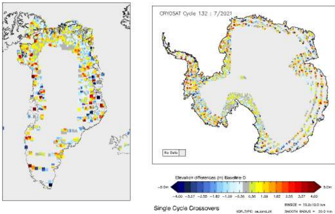
Figure 15 - Greenland and Antarctica maps of SARIn elevation differences for cycle #132.
