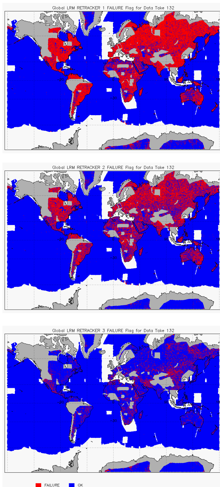
Figure 9 – Global plots showing Retracker Failure Flags for LRM mode for cycle #132:
