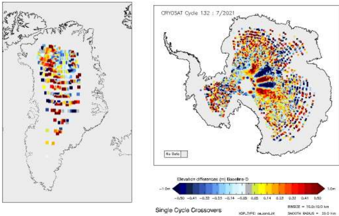
Figure 14 - Greenland and Antarctica maps of LRM elevation differences for cycle #132.
