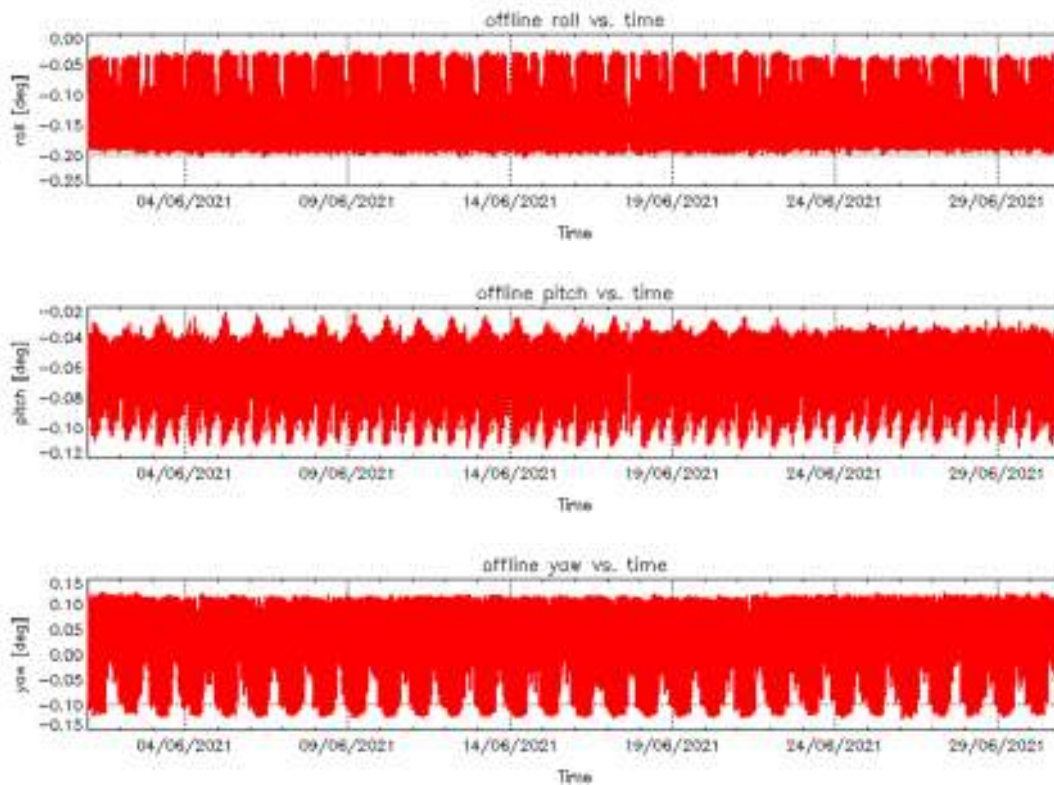
Figure 4 – Roll (top), Pitch (middle) and Yaw (bottom) values for L1B Products during cycle #130.
