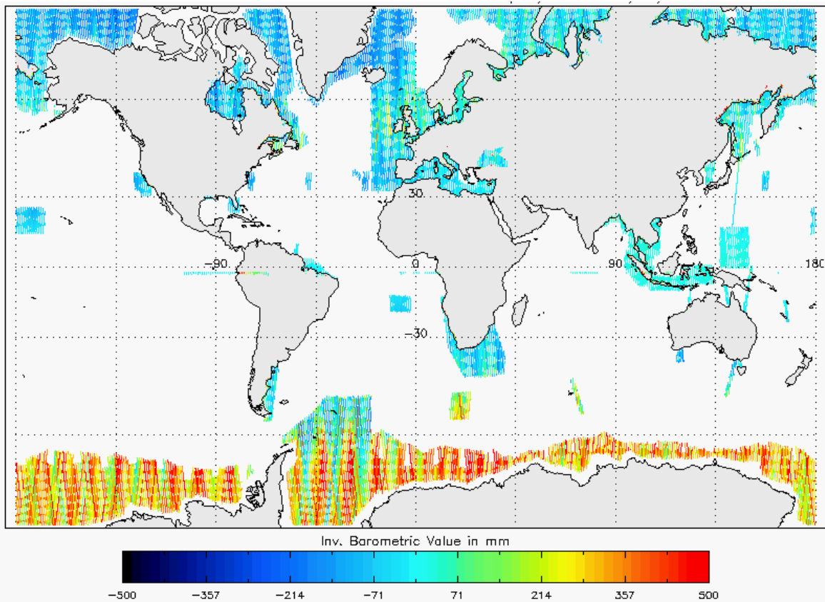
Figure 20 - Global plot of Inverse Barometric Correction for cycle #129
