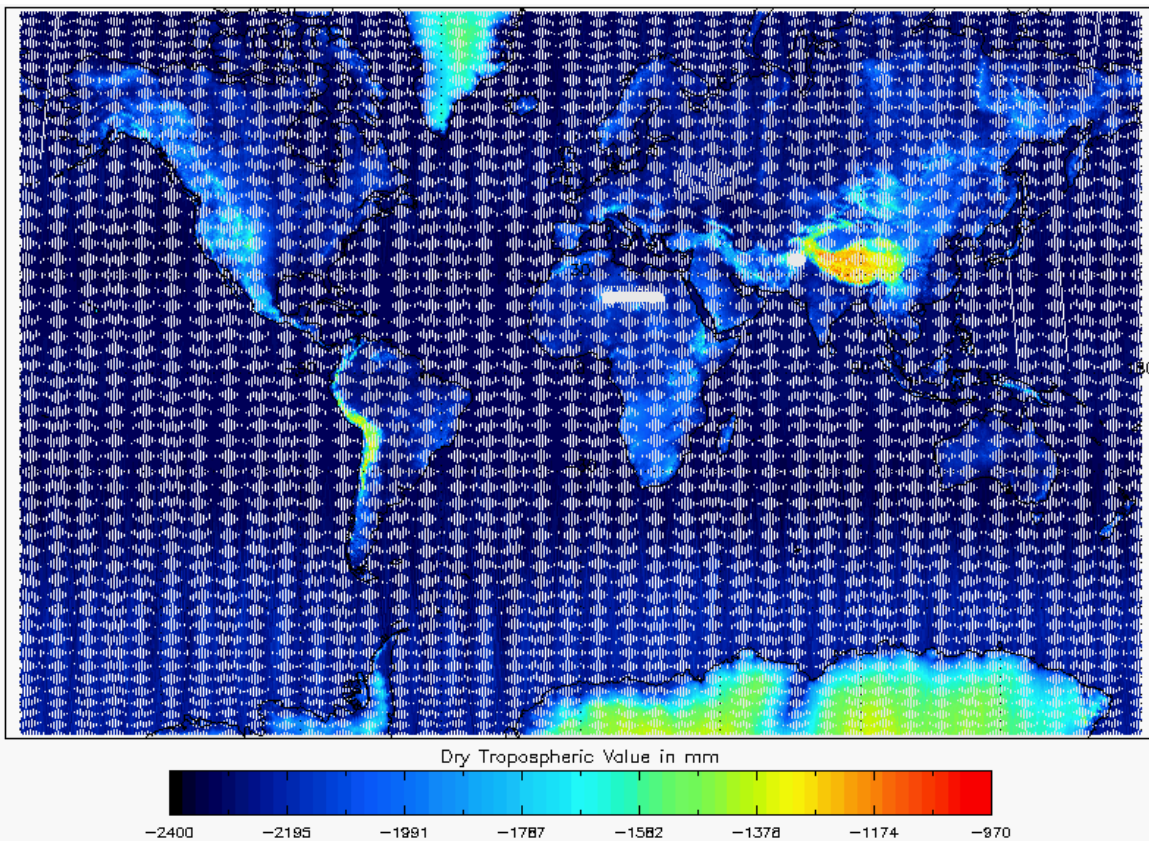
Figure 16 - Global plot of Dry Tropospheric Correction for cycle #129
