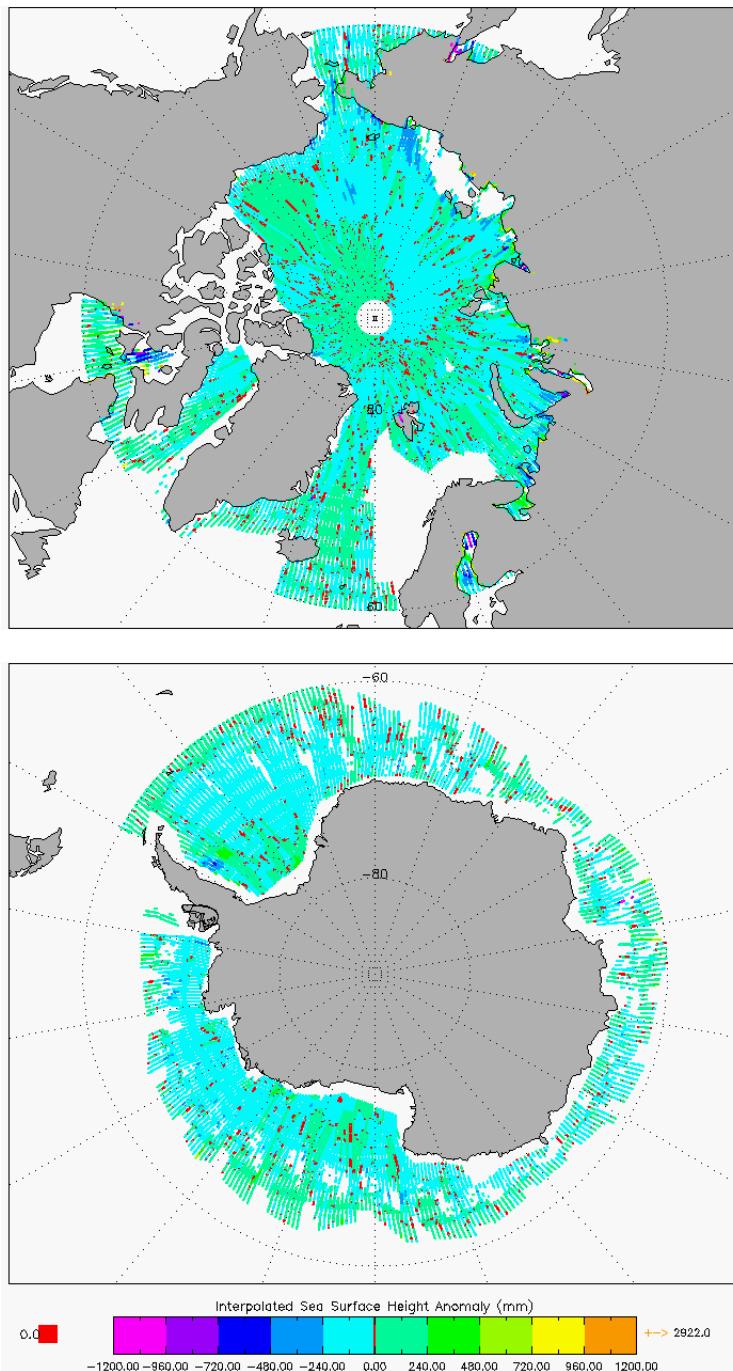
Figure 7 –Polar plots of SSHA for cycle #129.
