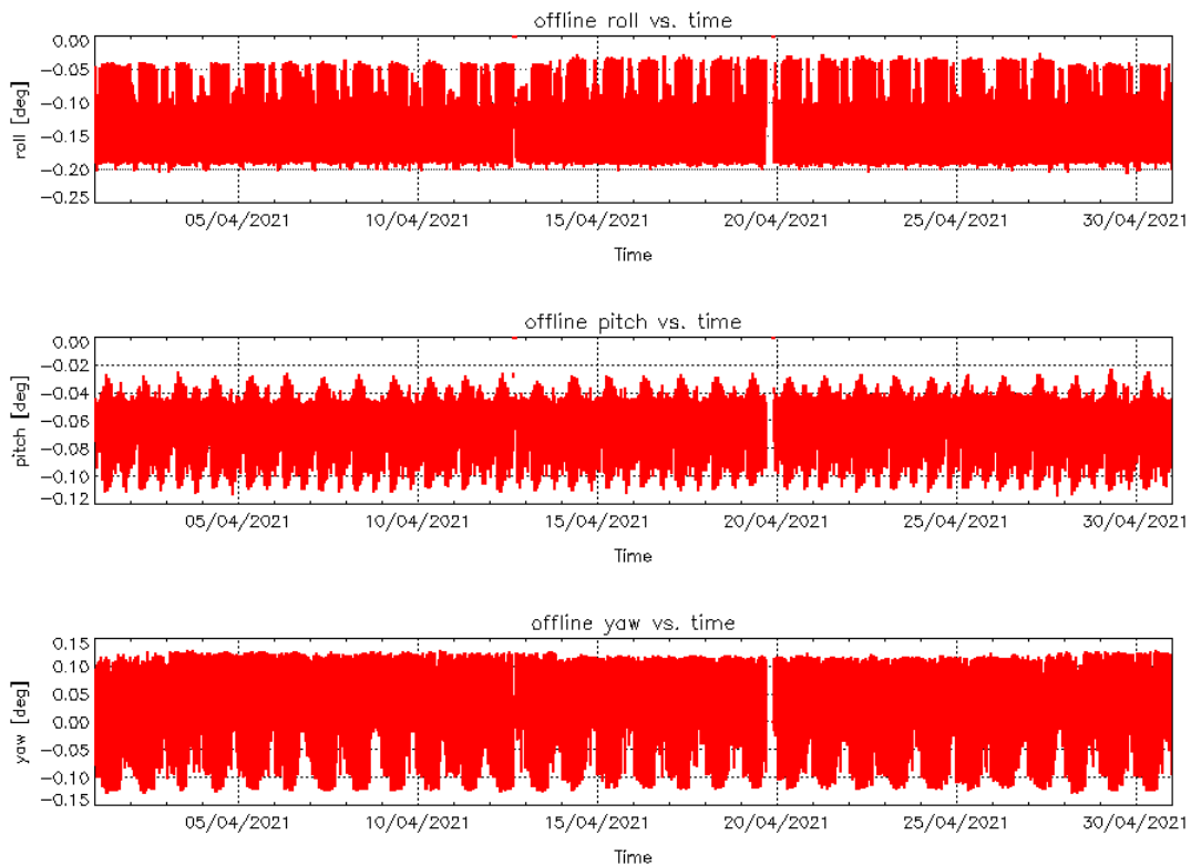
Figure 4 – Roll (top), Pitch (middle) and Yaw (bottom) values for L1B Products during cycle #129.
