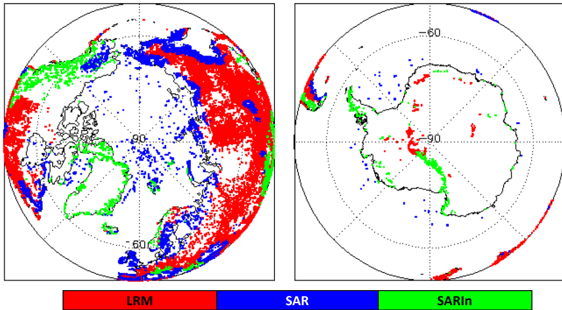
Figure 2 - Polar plots showing areas of loss of track in all SIRAL modes L0 data during May 2021.
