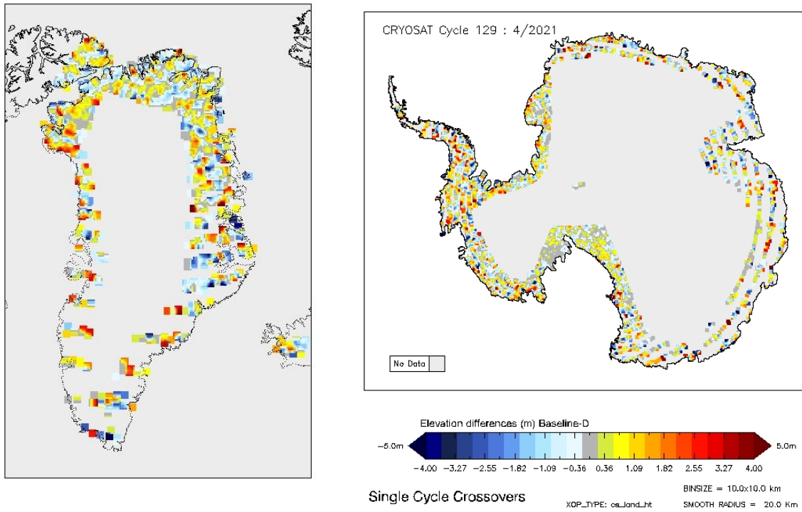
Figure 15 - Greenland and Antarctica maps of SARIn elevation differences for cycle #129.
