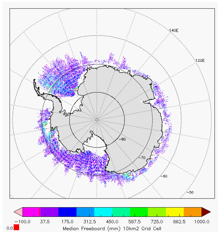
Figure 6 - Polar plots of 10km Gridded Freeboard values from L2 SAR products in cycle #129.
