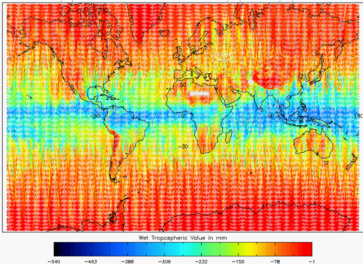
Figure 18 - Global plot of Wet Tropospheric Correction for cycle #129
