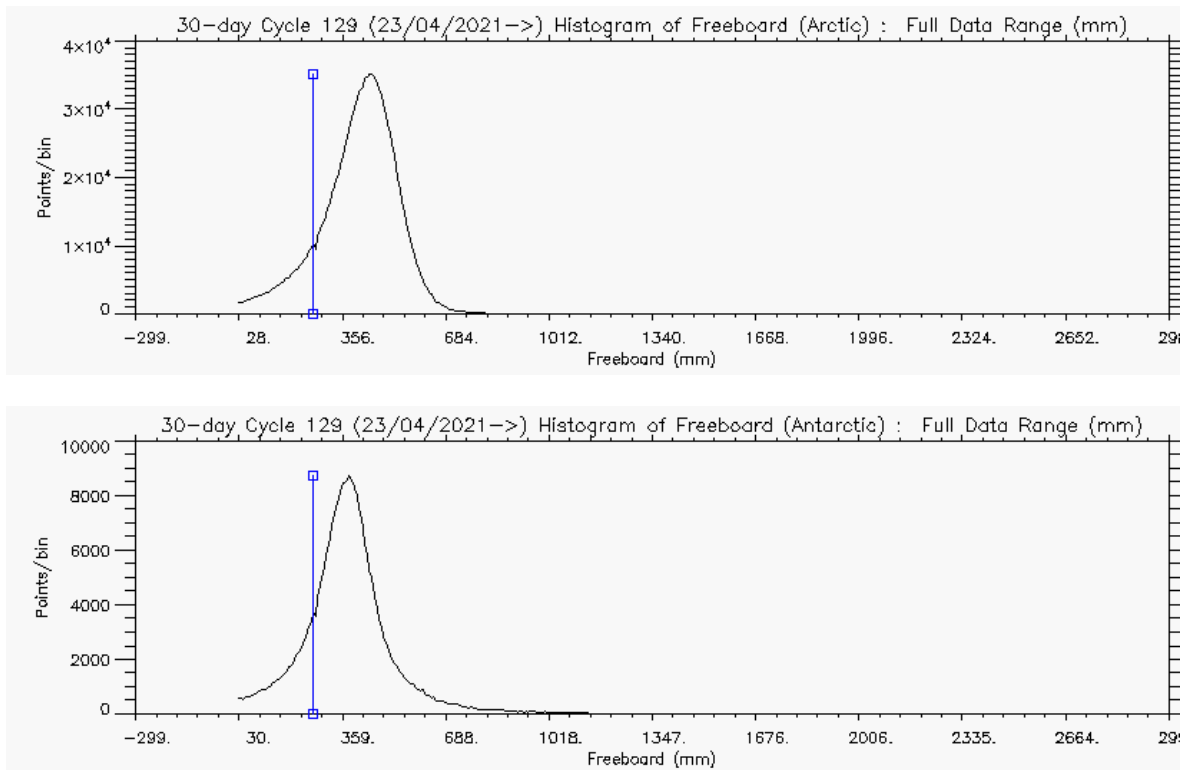
Figure 5 – Histogram of Freeboard for Arctic (above) and Antarctic (below) for cycle #129
