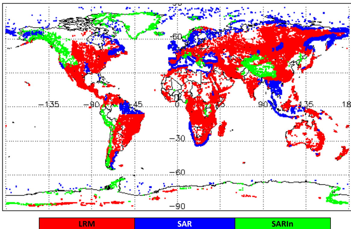
Figure 1 – Global plot showing areas of loss of track in all SIRAL modes L0 data during May 2021
