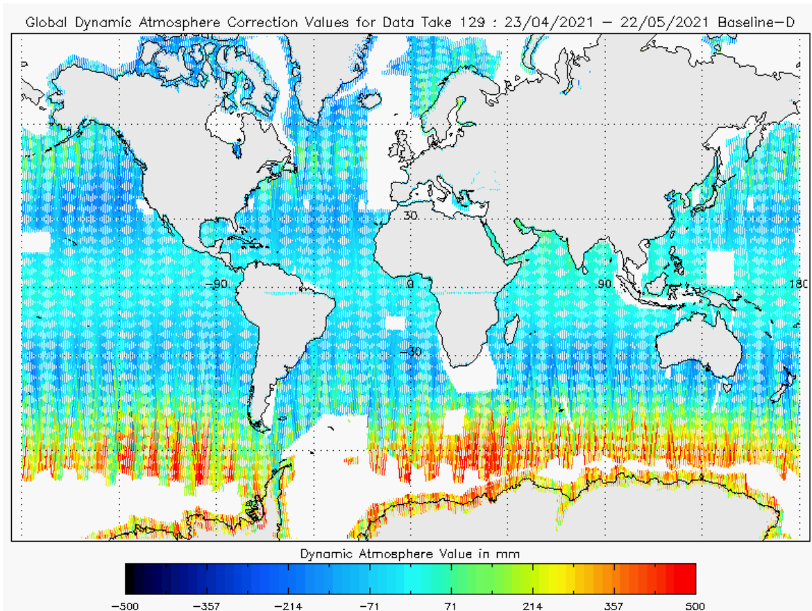
Figure 22 - Global plot of Dynamic Atmospheric Correction for cycle #129
