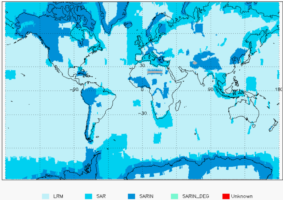
Figure 3 - Global and Polar plots of SIRAL Modes for cycle #128.
