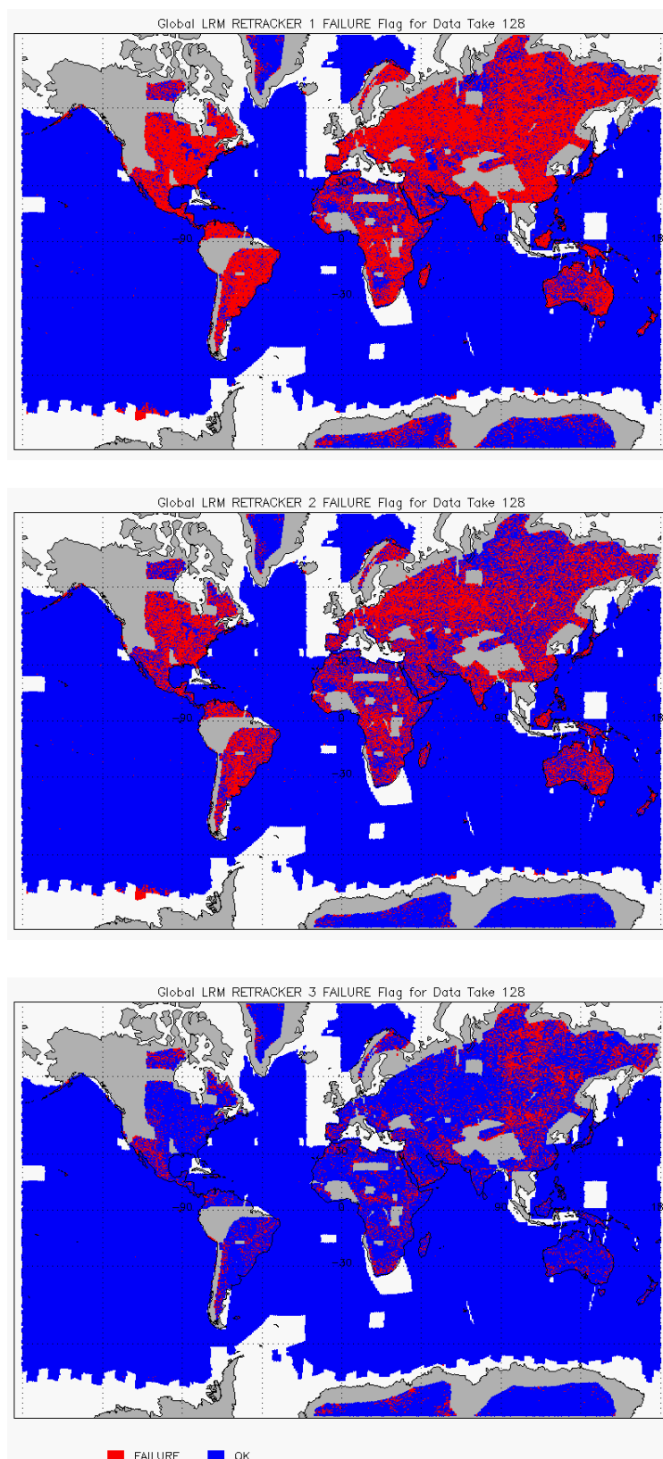
Figure 9 – Global plots showing Retracker Failure Flags for LRM mode for cycle #128: LRM CFI (top), LRM LIRT (middle), LRM OCOG (bottom)
