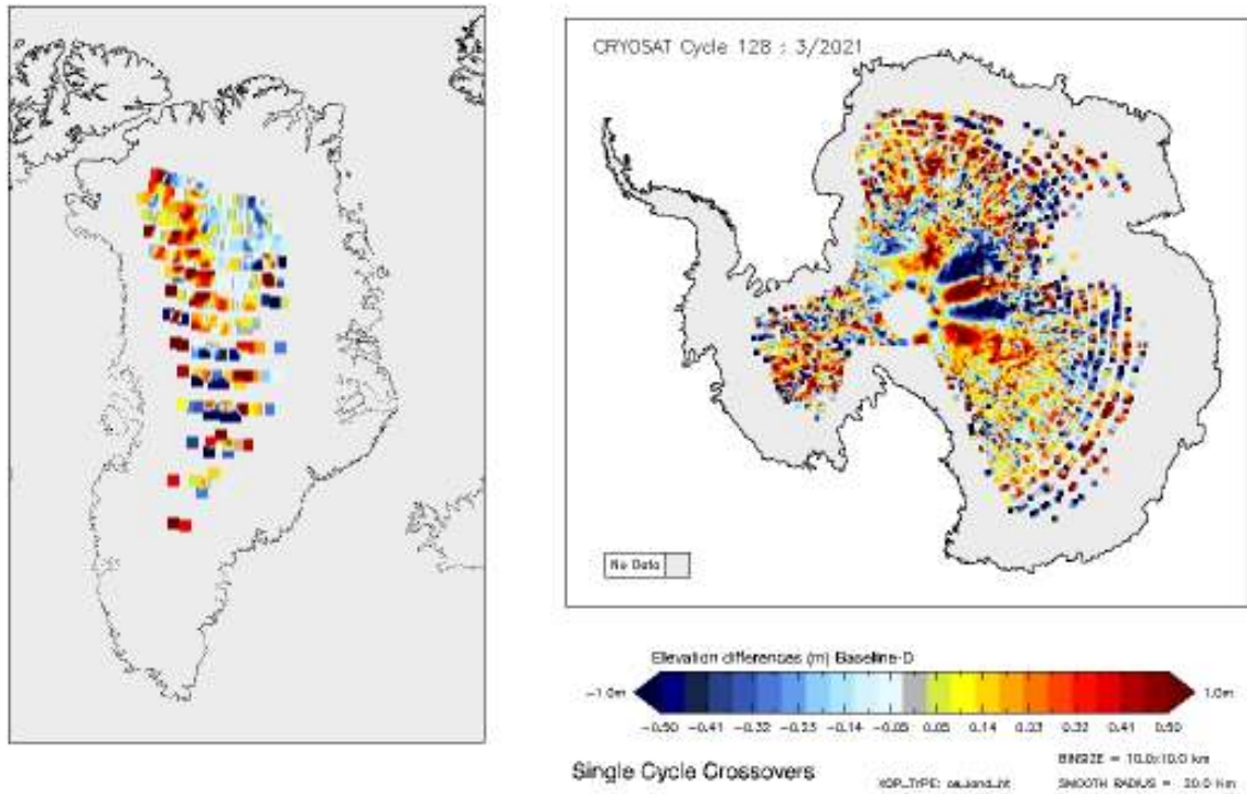
Figure 14 - Greenland and Antarctica maps of LRM elevation differences for cycle #128.
