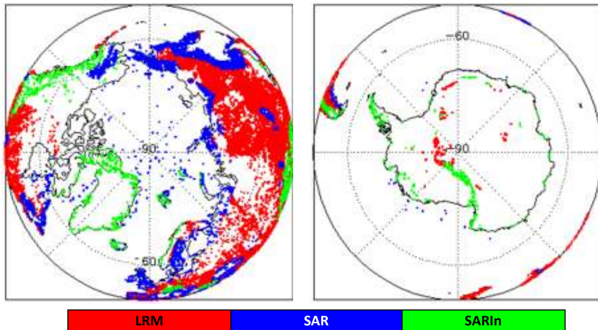
Figure 2 - Polar plots showing areas of loss of track in all SIRAL modes L0 data during April 2021.
