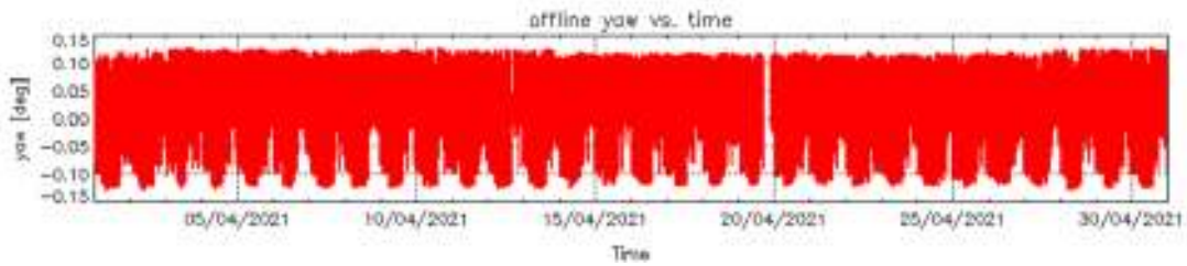
Figure 4 – Roll (top), Pitch (middle) and Yaw (bottom) values for L1B Products during cycle #128.
