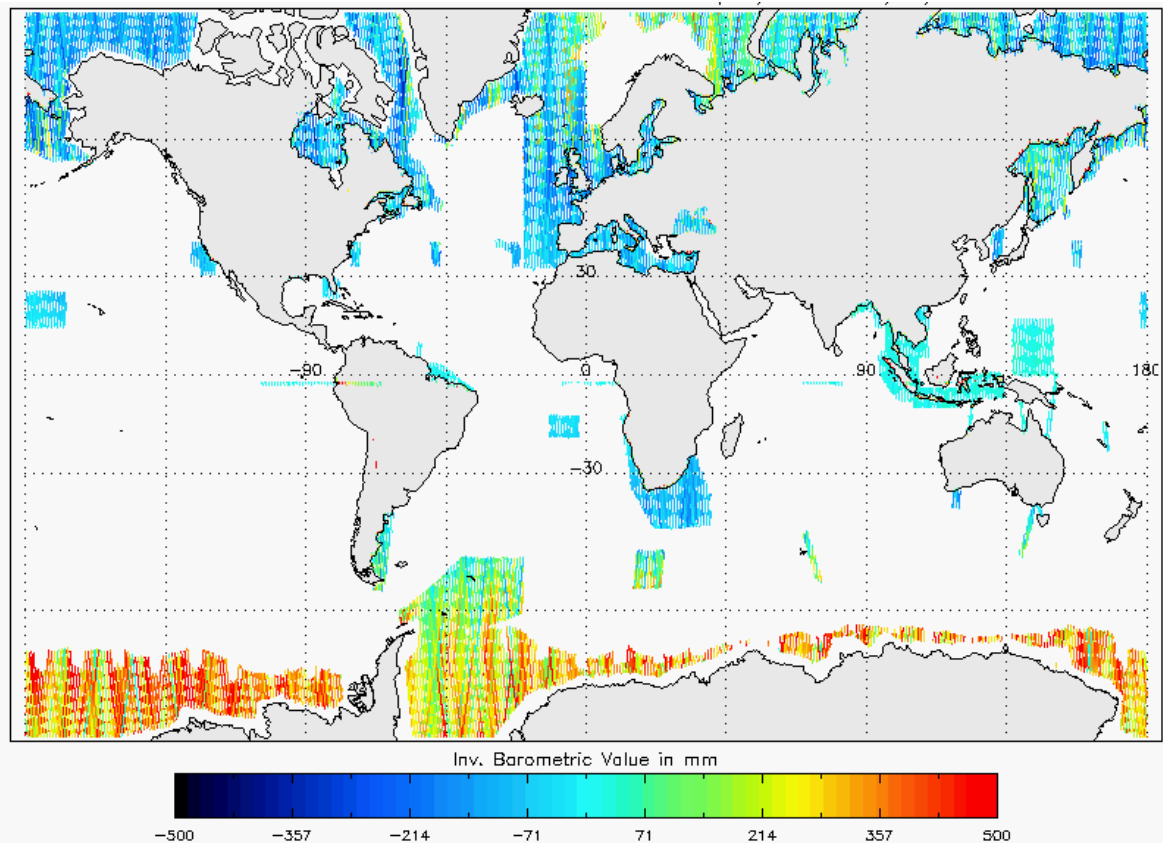
Figure 20 - Global plot of Inverse Barometric Correction for cycle #128
