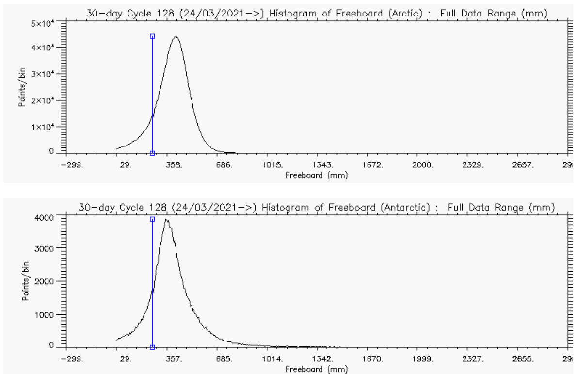
Figure 5 – Histogram of Freeboard for Arctic (above) and Antarctic (below) for cycle #128
