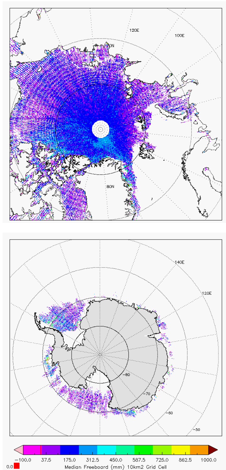
Figure 6 - Polar plots of 10km Gridded Freeboard values from L2 SAR products in cycle #128.
