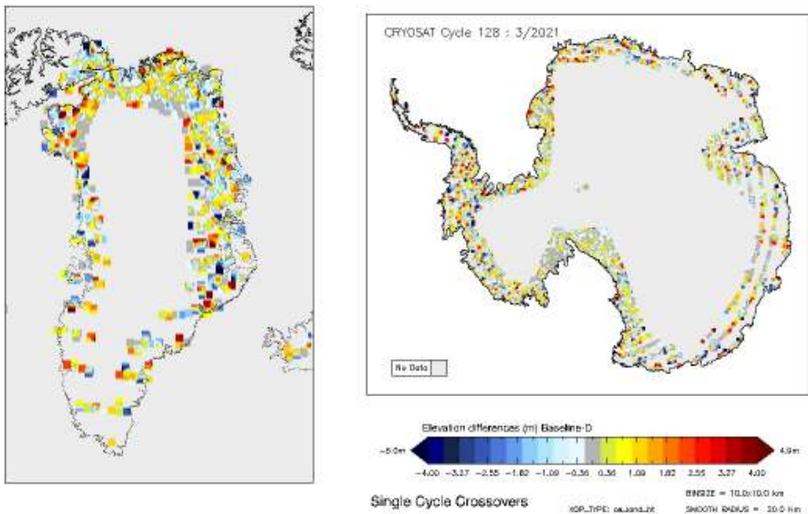
Figure 15 - Greenland and Antarctica maps of SARIn elevation differences for cycle #128.
