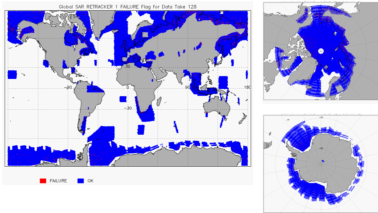
Figure 10 - Global plots showing Retracker Failure Flags for SAR mode for cycle #128
