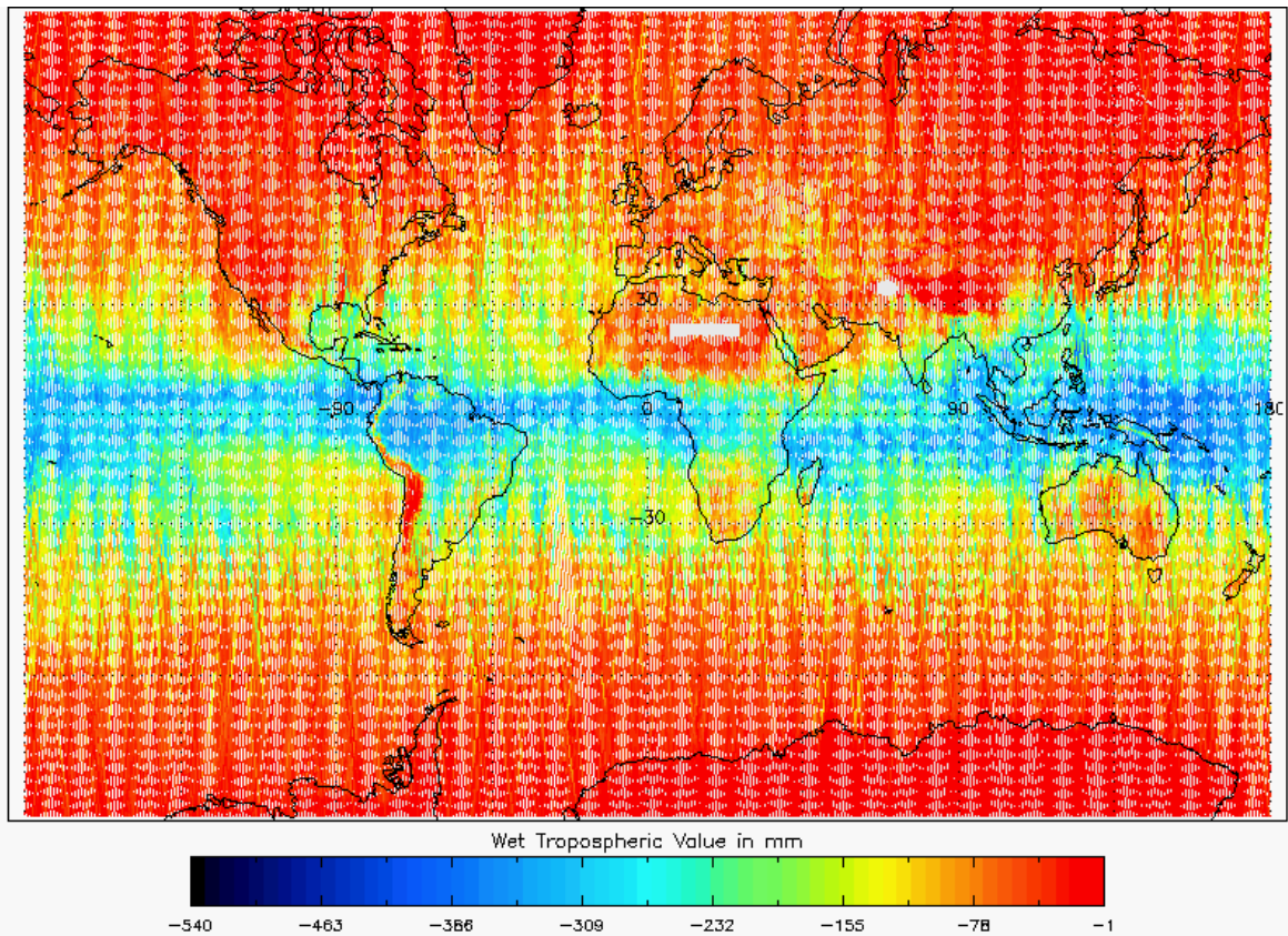
Figure 18 - Global plot of Wet Tropospheric Correction for cycle #128
