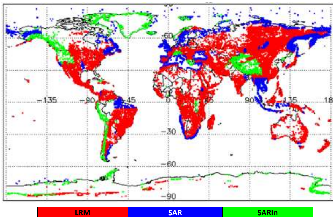
Figure 1 – Global plot showing areas of loss of track in all SIRAL modes L0 data during April 2021
