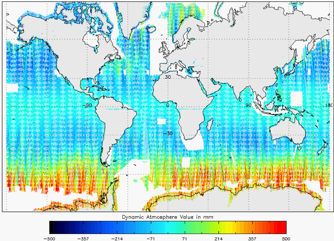
Figure 22 - Global plot of Dynamic Atmospheric Correction for cycle #128
