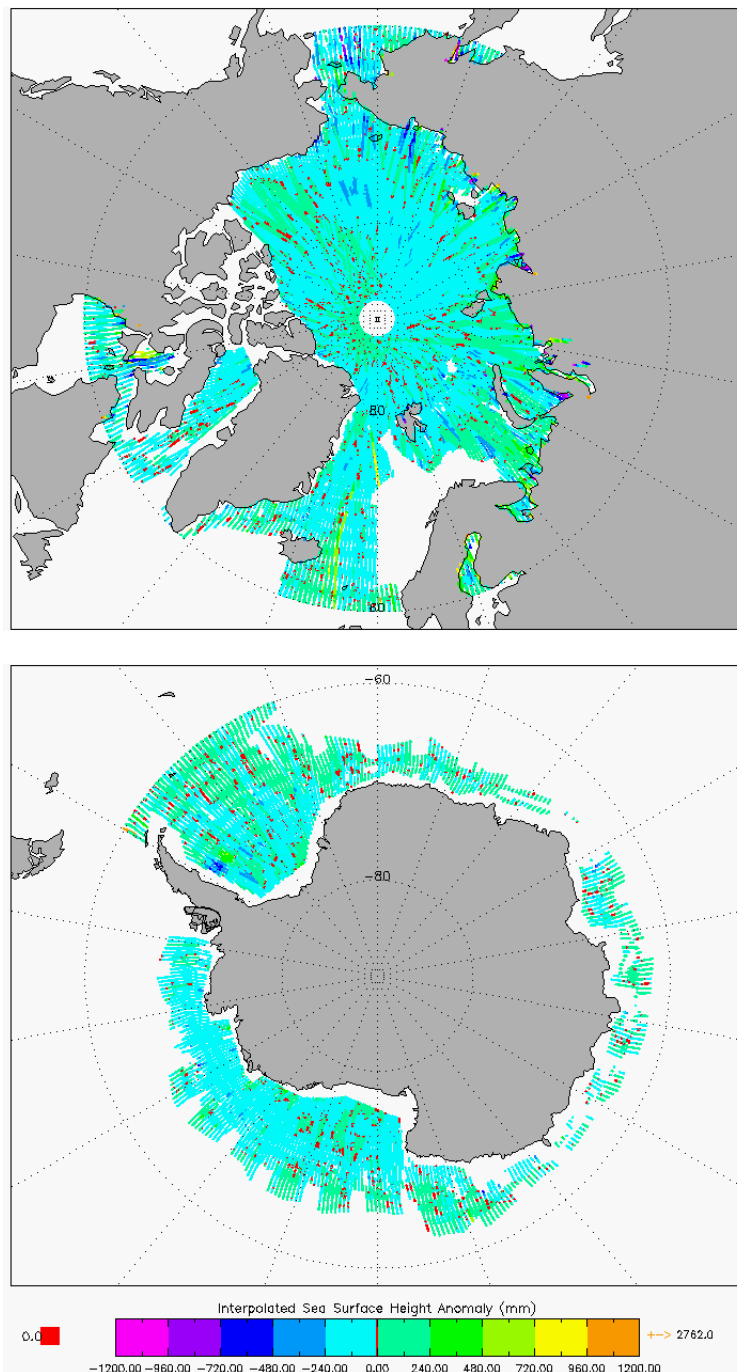
Figure 7 –Polar plots of SSHA for cycle #128.
