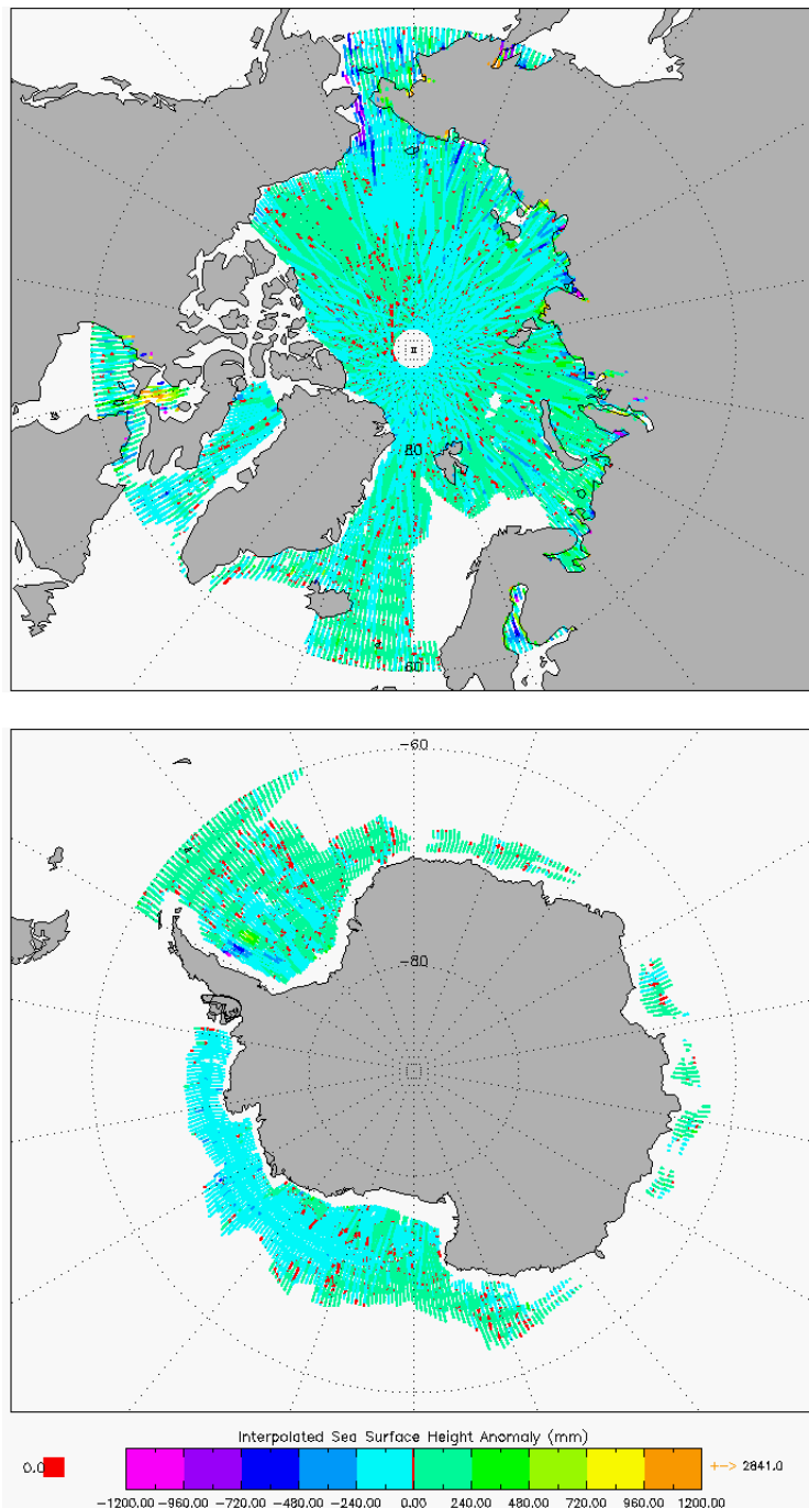
Figure 7 –Polar plots of SSHA for cycle #127.
