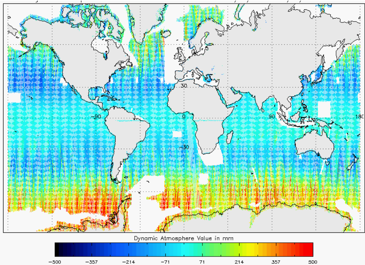
Figure 22 - Global plot of Dynamic Atmospheric Correction for cycle #127
