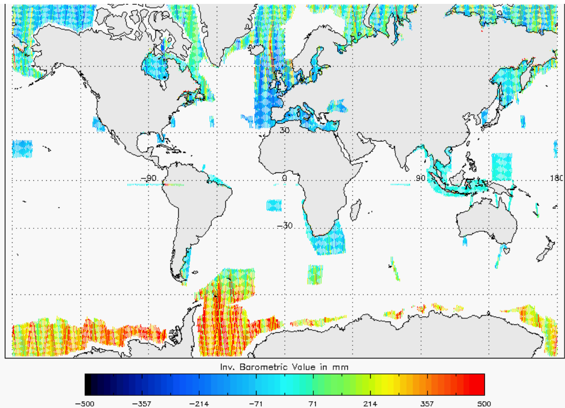
Figure 20 - Global plot of Inverse Barometric Correction for cycle #127
