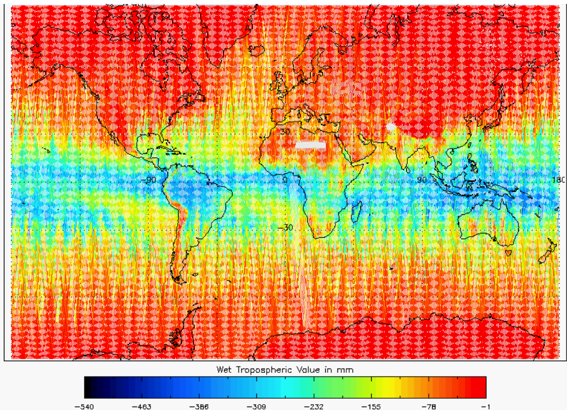
Figure 18 - Global plot of Wet Tropospheric Correction for cycle #127
