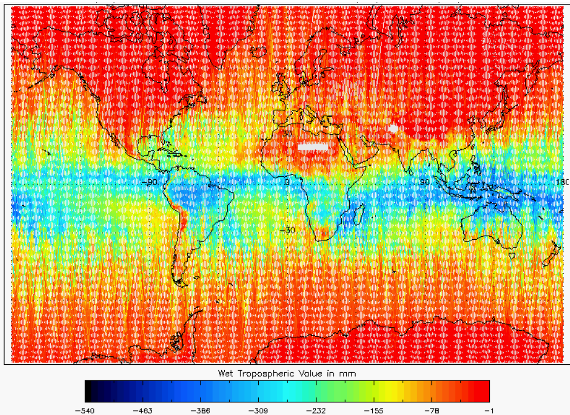
Figure 18 - Global plot of Wet Tropospheric Correction for cycle #126
