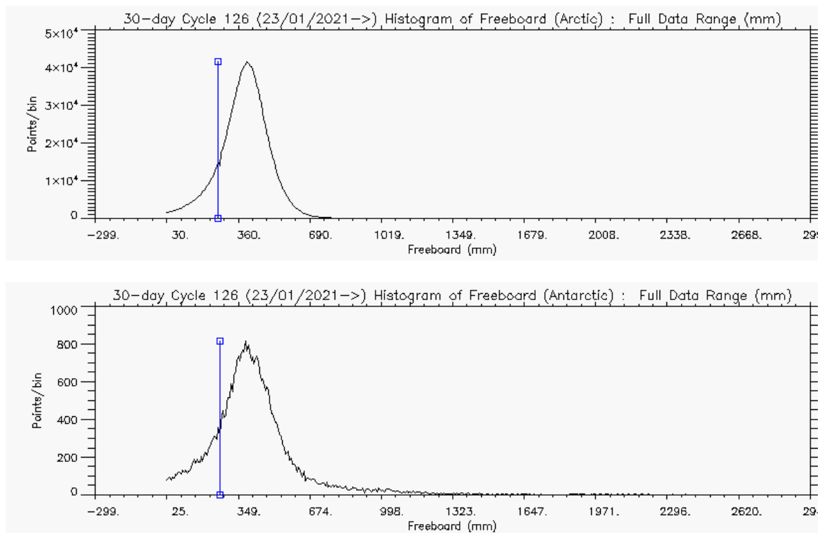
Figure 5 – Histogram of Freeboard for Arctic (above) and Antarctic (below) for cycle #126
