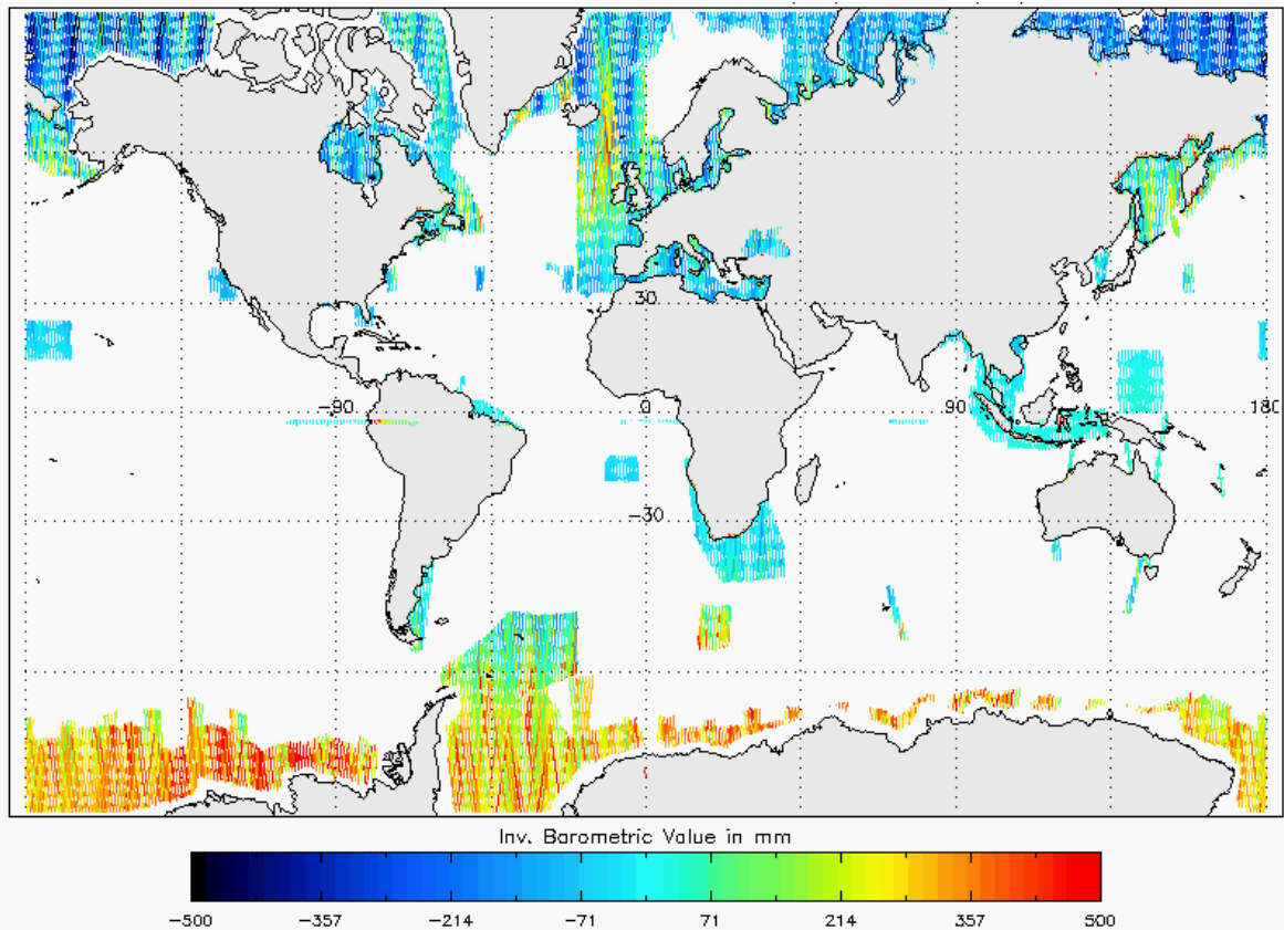
Figure 20 - Global plot of Inverse Barometric Correction for cycle #126
