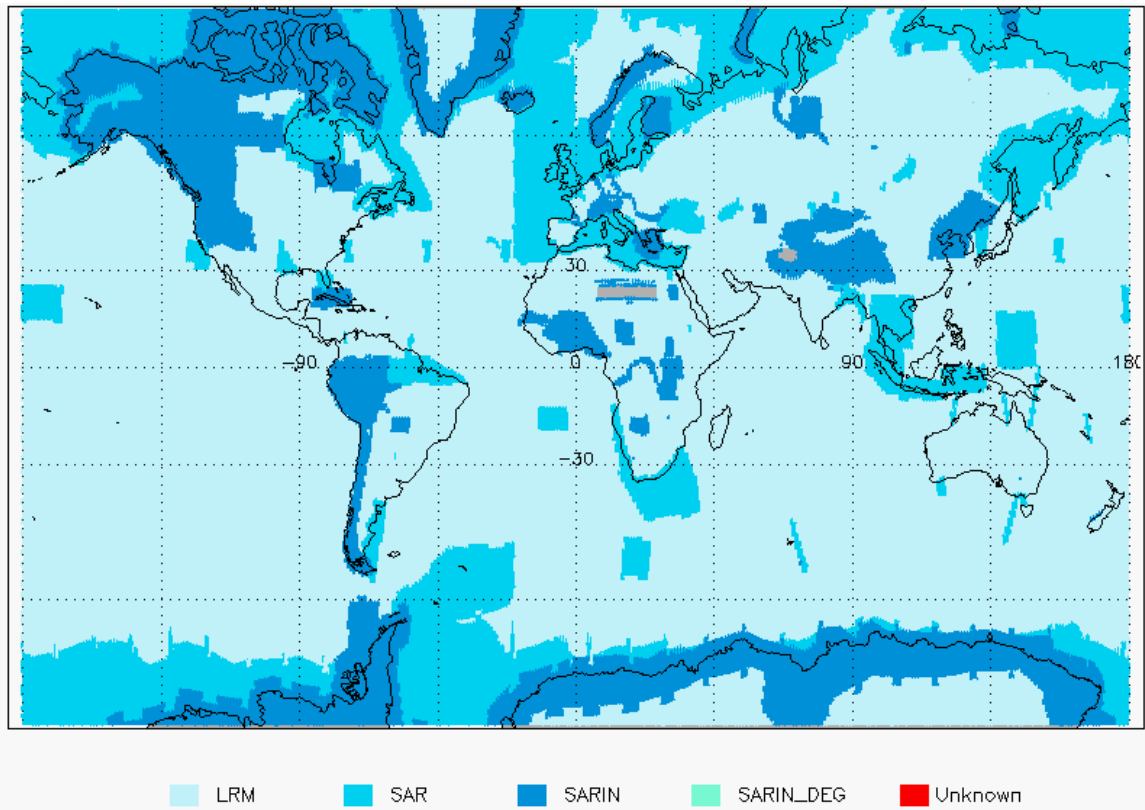
Figure 3 - Global and Polar plots of SIRAL Modes for cycle #126.
