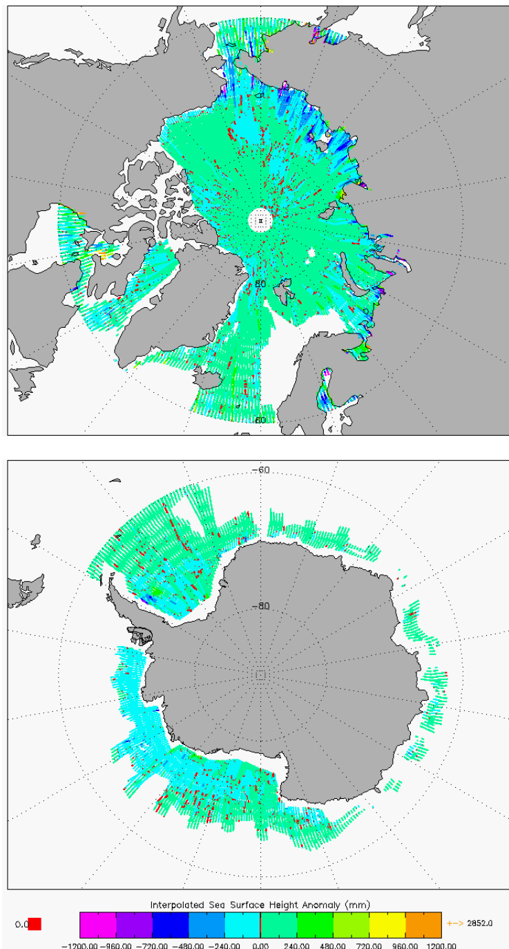
Figure 7 –Polar plots of SSHA for cycle #126.
