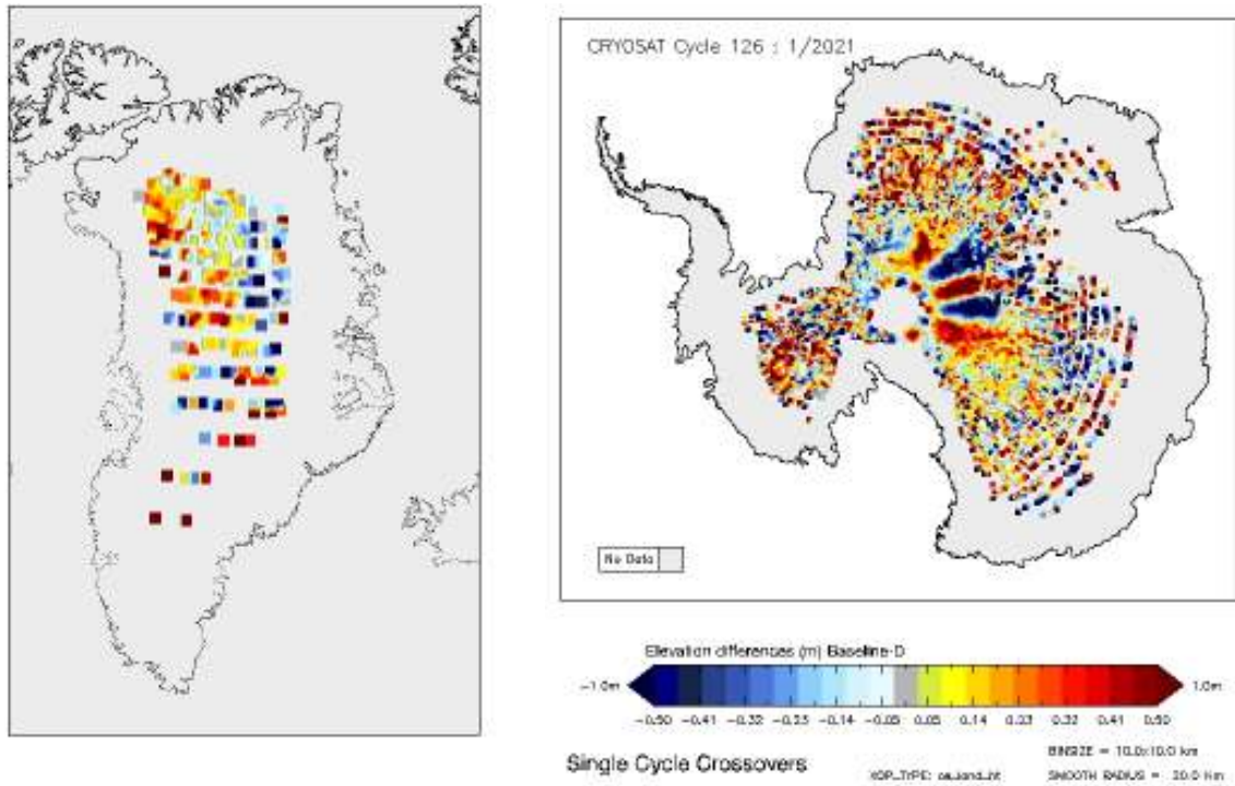
Figure 14 - Greenland and Antarctica maps of LRM elevation differences for cycle #126.
