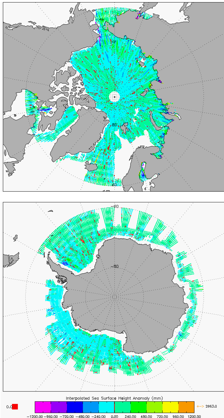
Figure 7 –Polar plots of SSHA for cycle #125.
