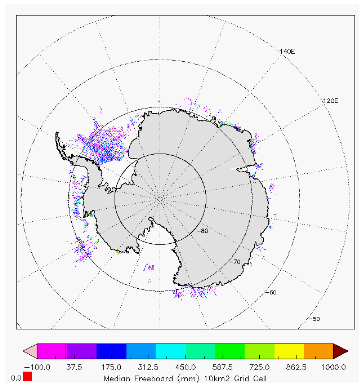
Figure 6 - Polar plots of 10km Gridded Freeboard values from L2 SAR products in cycle #125.
