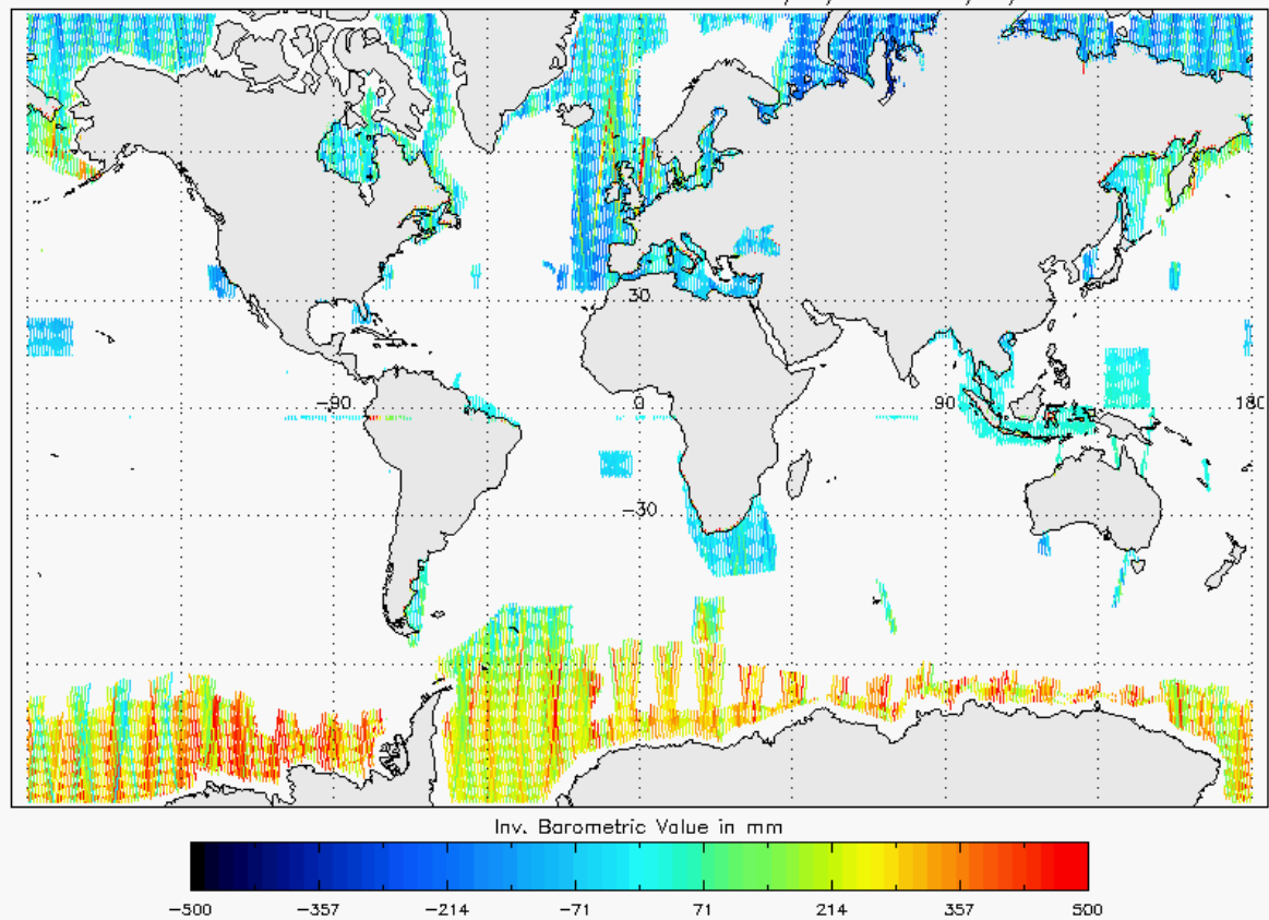
Figure 20 - Global plot of Inverse Barometric Correction for cycle #125
