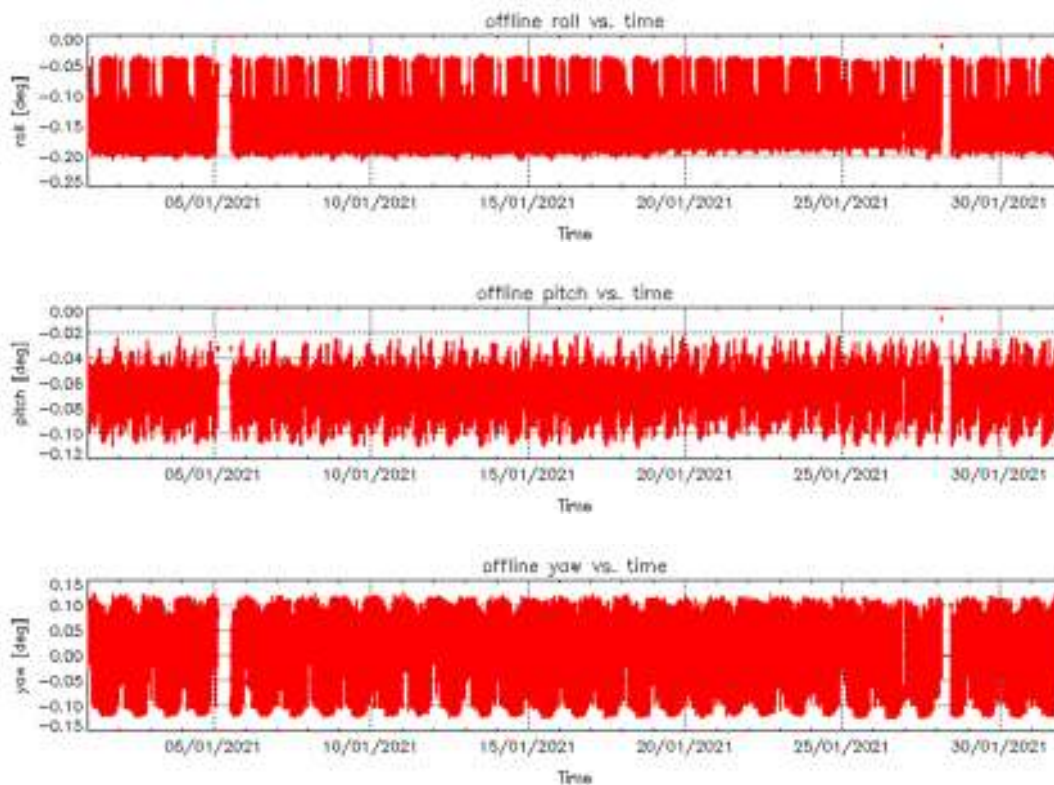
Figure 4 – Roll (top), Pitch (middle) and Yaw (bottom) values for L1B Products during cycle #125.
