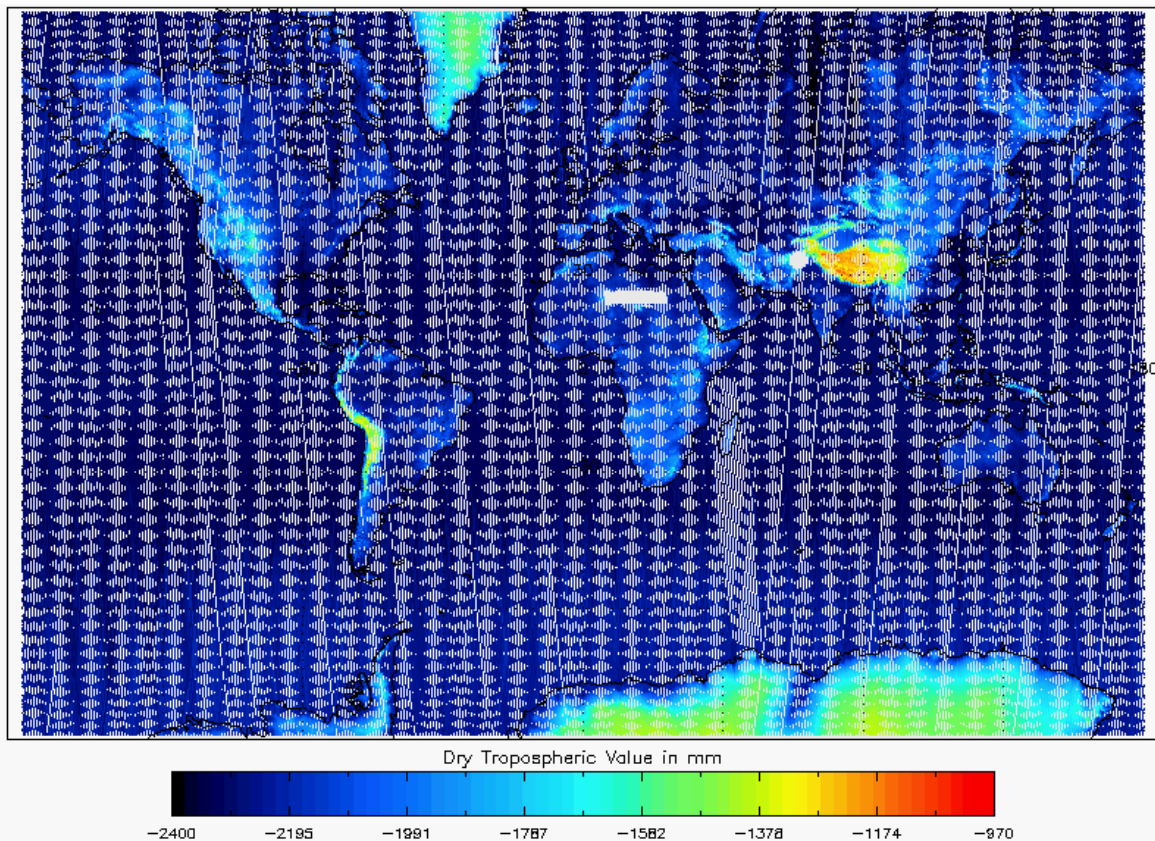
Figure 16 - Global plot of Dry Tropospheric Correction for cycle #125
