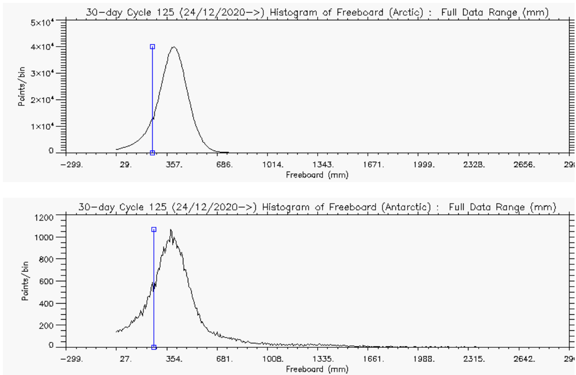
Figure 5 – Histogram of Freeboard for Arctic (above) and Antarctic (below) for cycle #125
