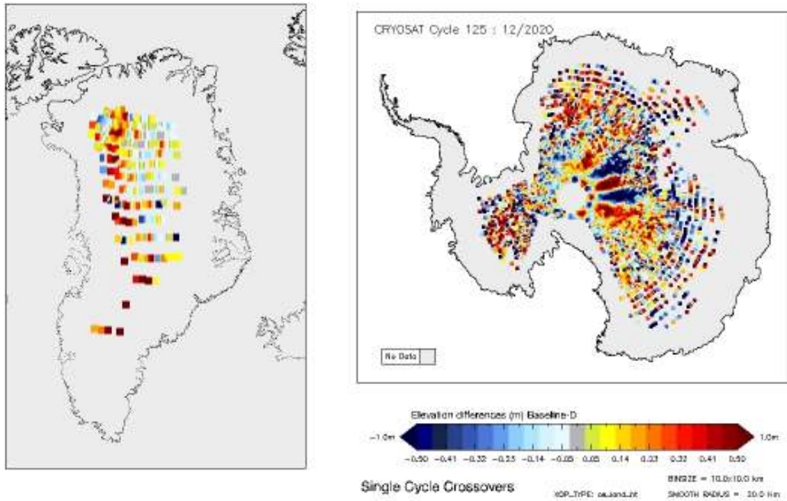
Figure 14 - Greenland and Antarctica maps of LRM elevation differences for cycle #125.
