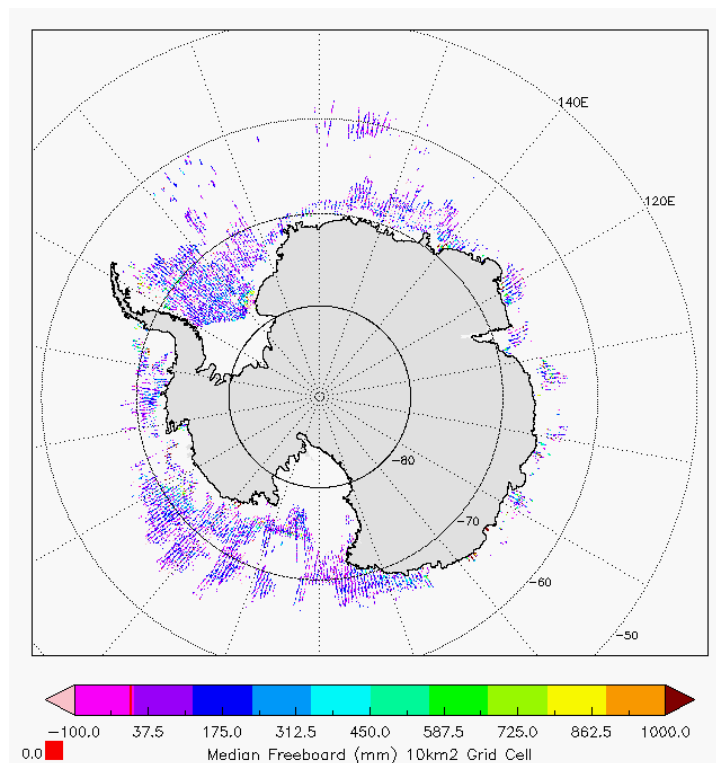
Figure 6 - Polar plots of 10km Gridded Freeboard values from L2 SAR products in cycle #124.
