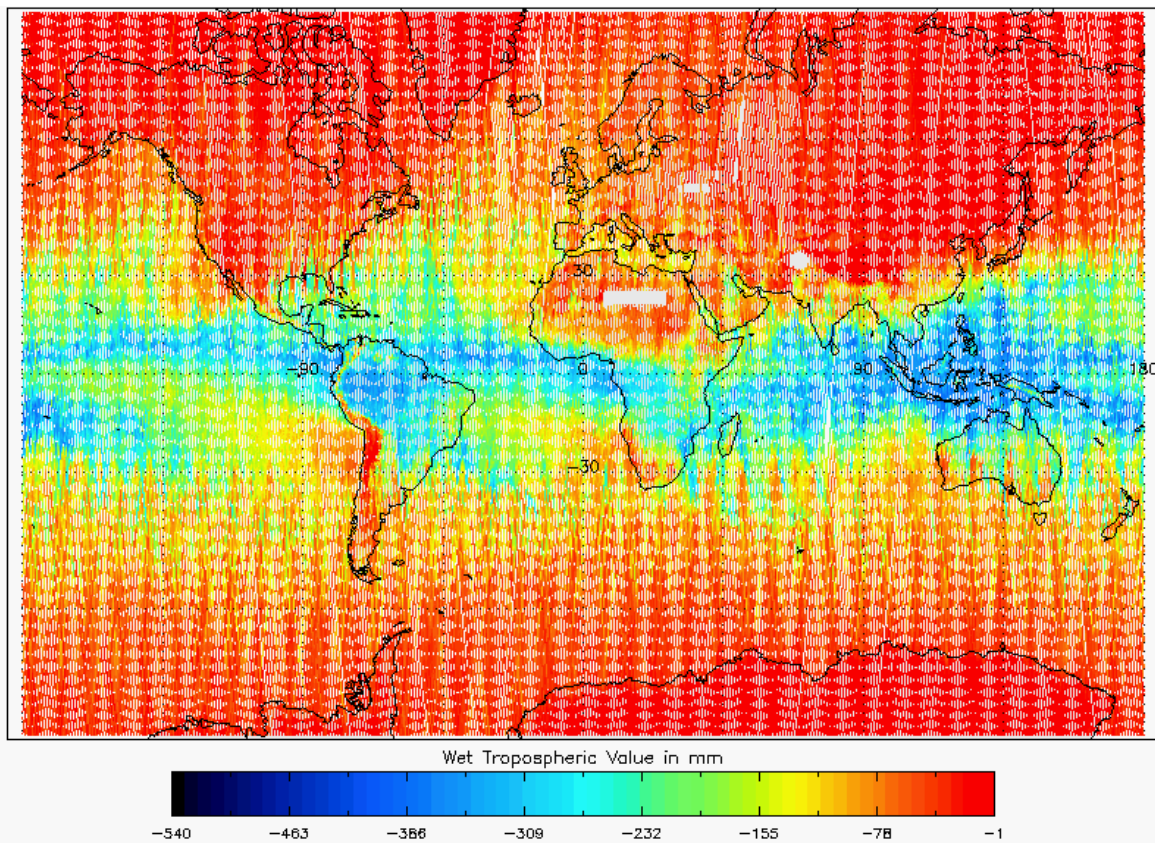
Figure 18 - Global plot of Wet Tropospheric Correction for cycle #124
