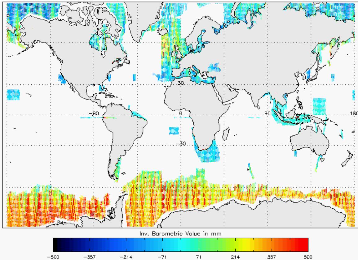
Figure 20 - Global plot of Inverse Barometric Correction for cycle #124
