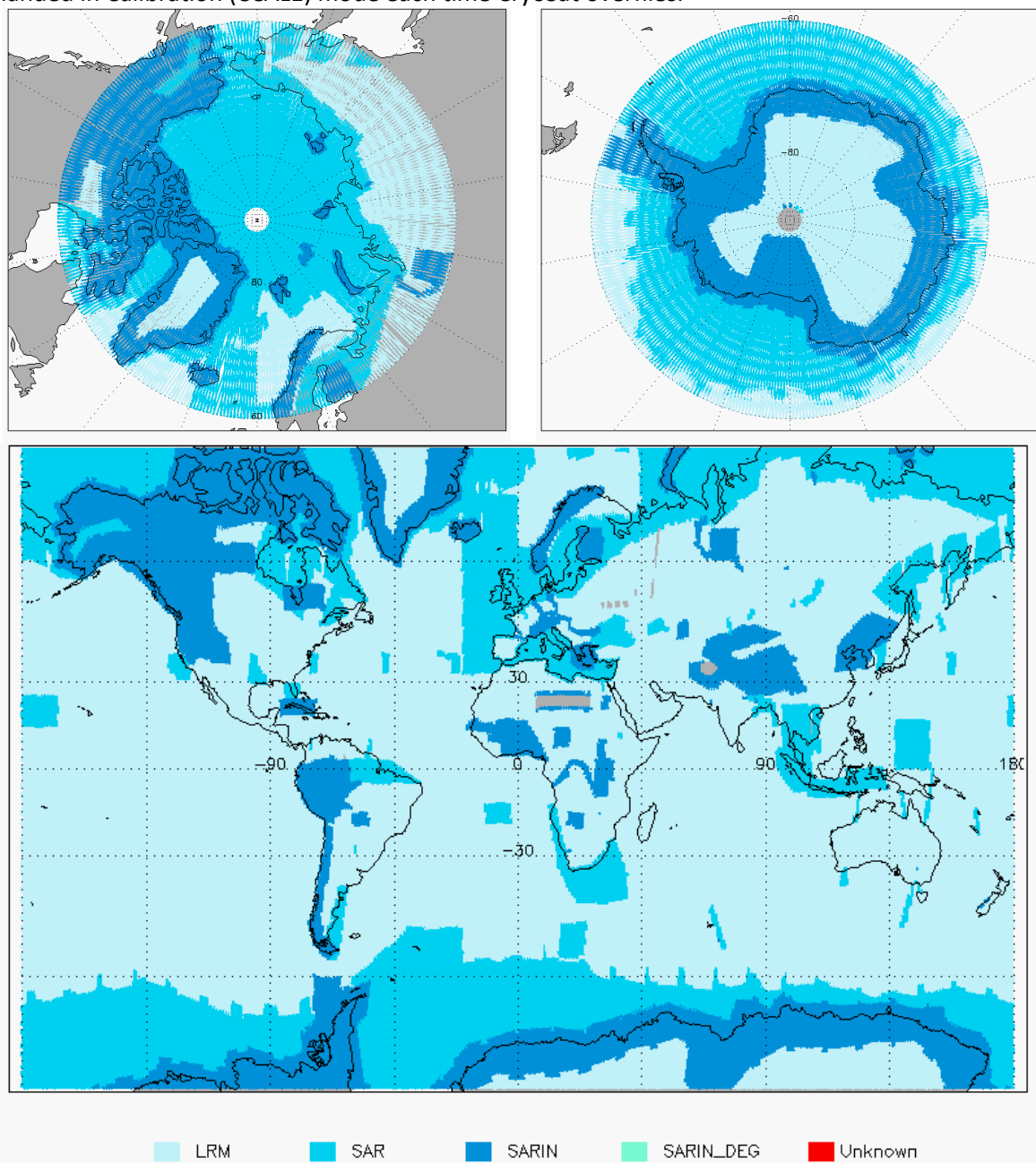
Figure 3 - Global and Polar plots of SIRAL Modes for cycle #124.
