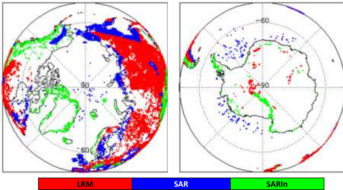
Figure 2 - Polar plots showing areas of loss of track in all SIRAL modes L0 data during December 2020.
