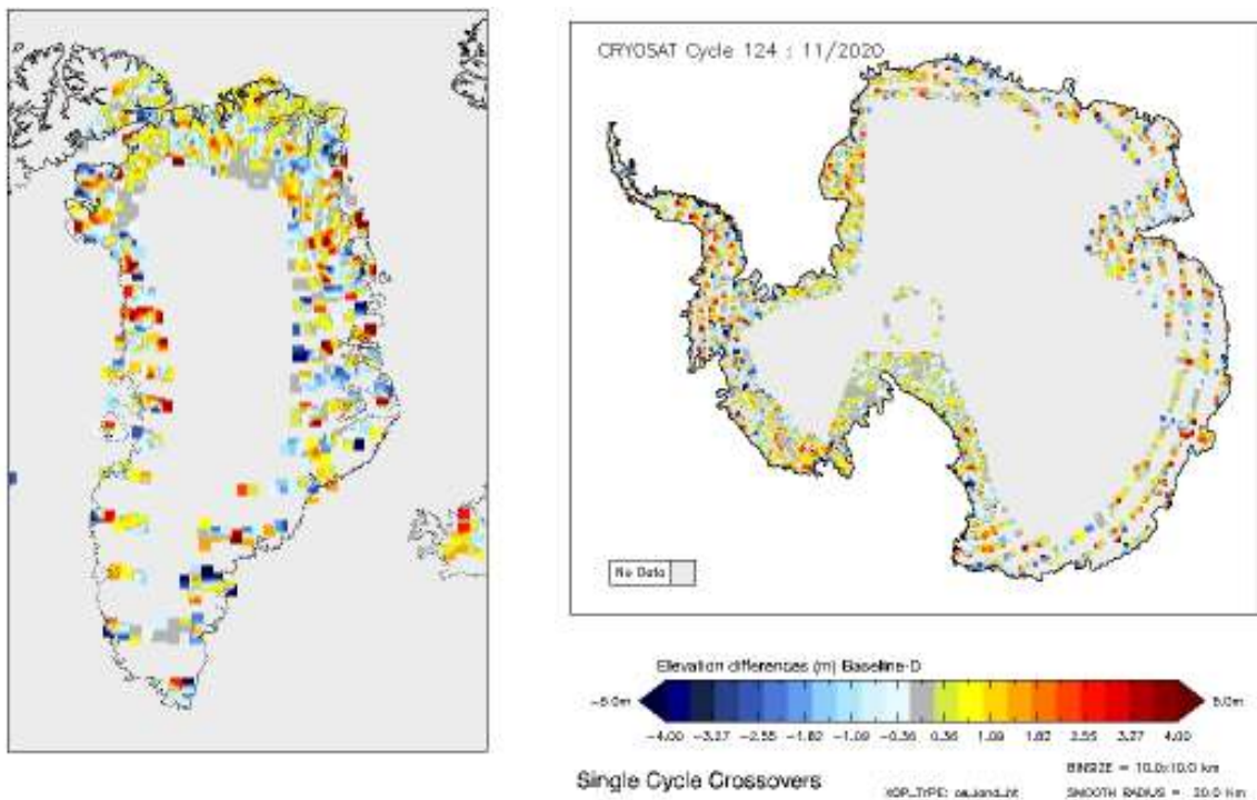
Figure 15 - Greenland and Antarctica maps of SARIn elevation differences for cycle #124.
