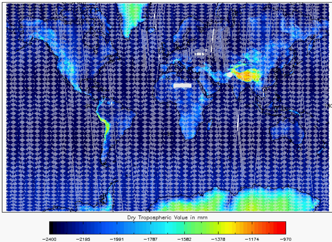
Figure 16 - Global plot of Dry Tropospheric Correction for cycle #124
