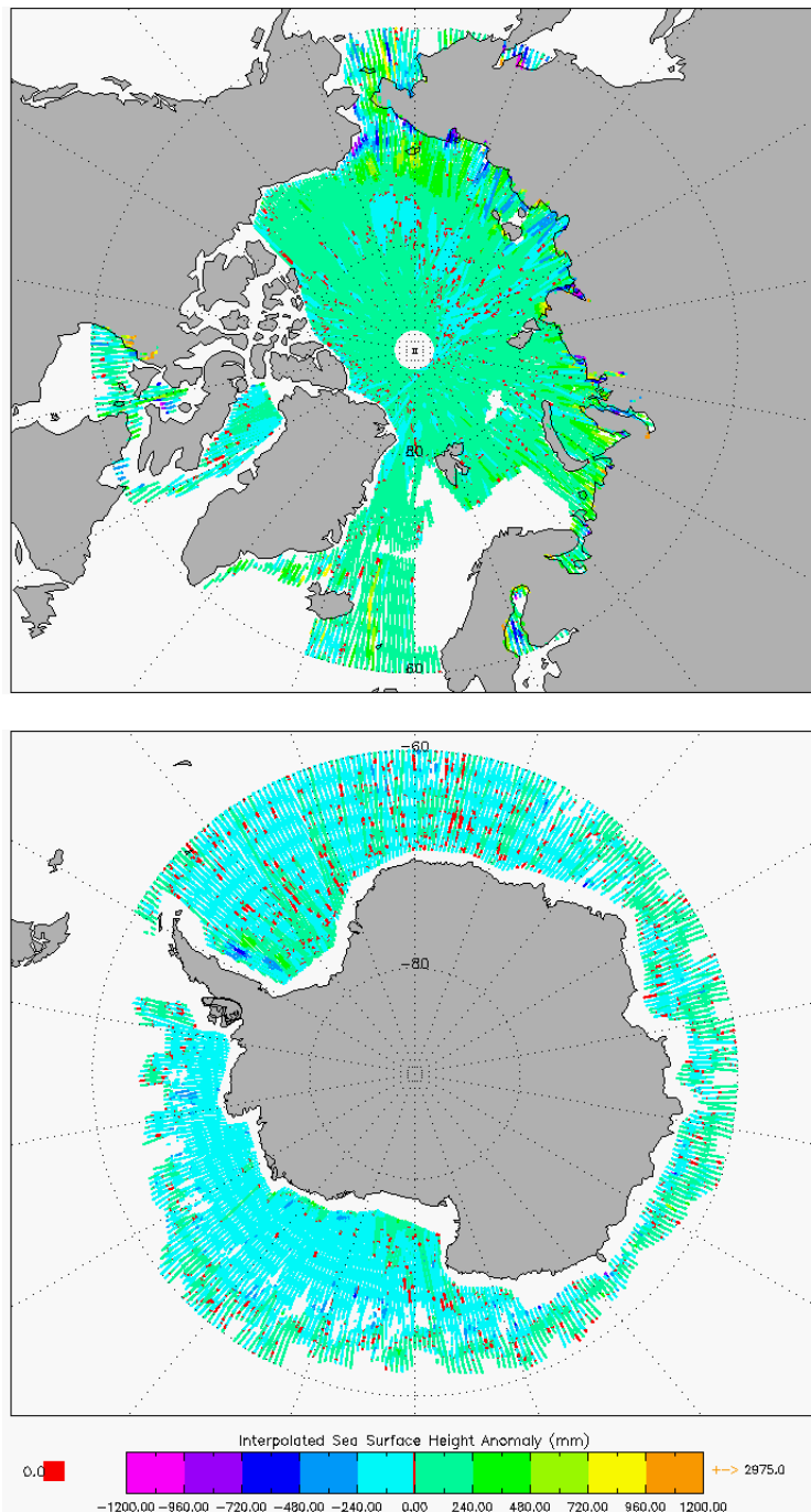
Figure 7 –Polar plots of SSHA for cycle #124.
