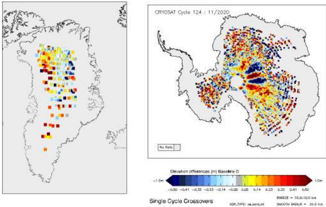
Figure 14 - Greenland and Antarctica maps of LRM elevation differences for cycle #124.
