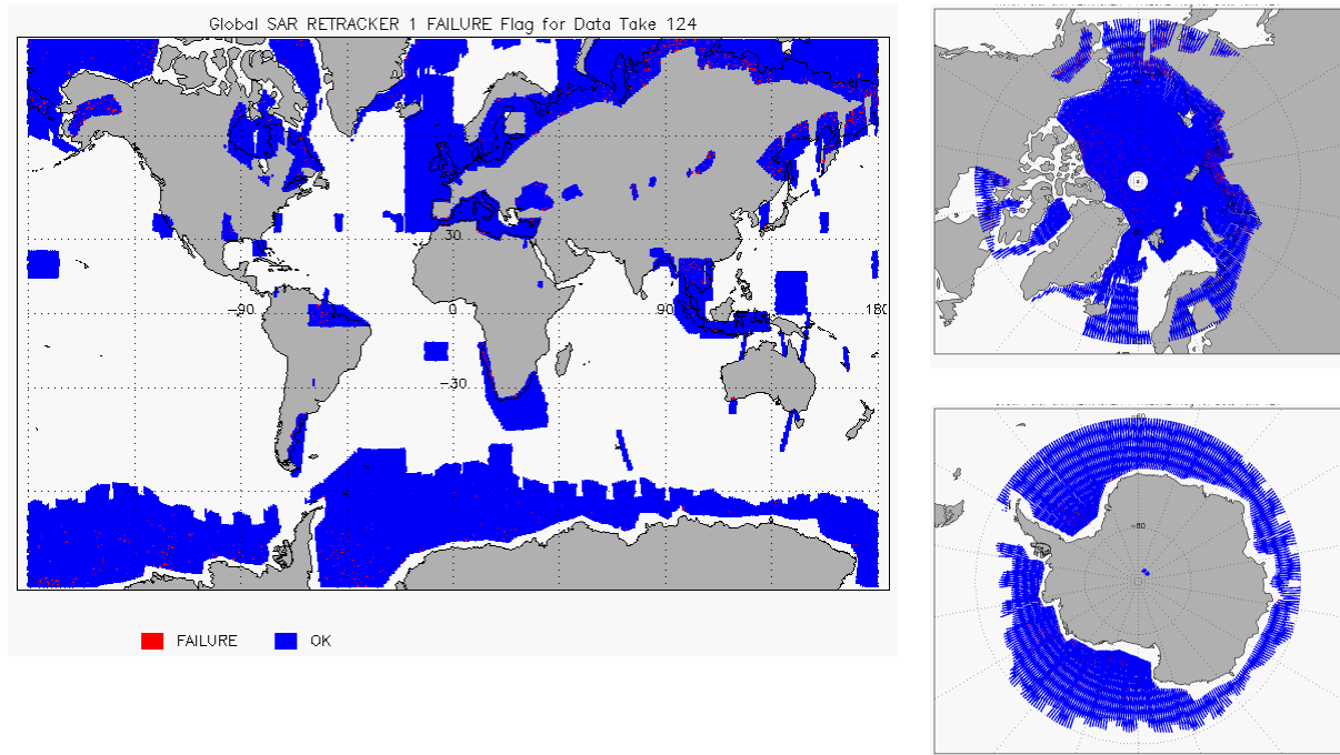
Figure 10 - Global plots showing Retracker Failure Flags for SAR mode for cycle #124
