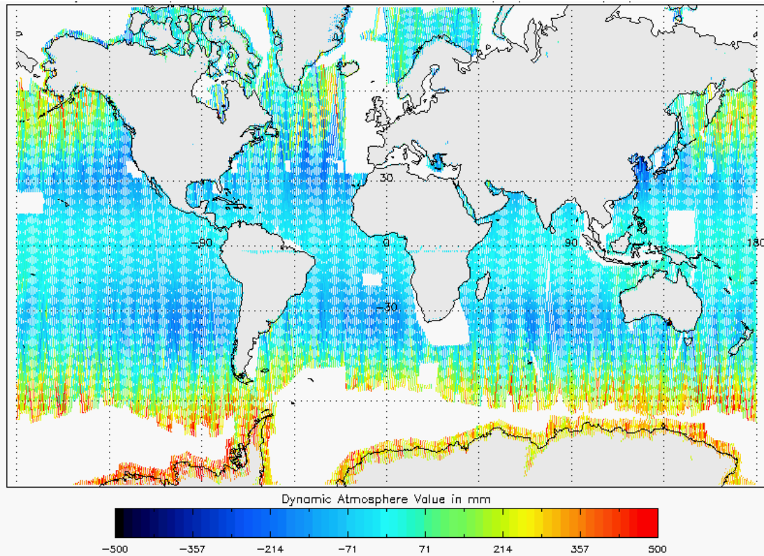
Figure 22 - Global plot of Dynamic Atmospheric Correction for cycle #124
