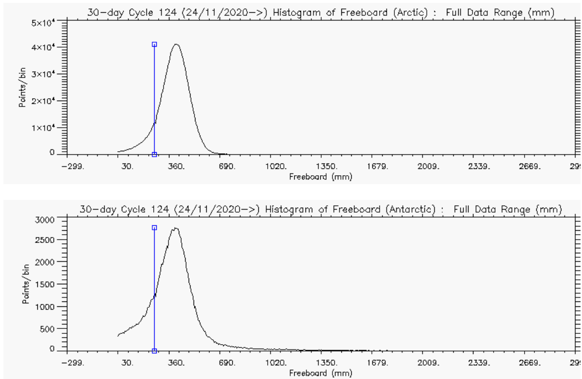
Figure 5 – Histogram of Freeboard for Arctic (above) and Antarctic (below) for cycle #124
