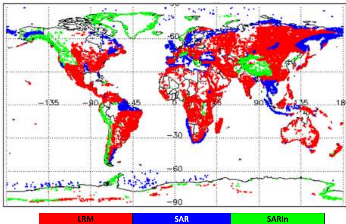
Figure 1 – Global plot showing areas of loss of track in all SIRAL modes L0 data during December 2020
