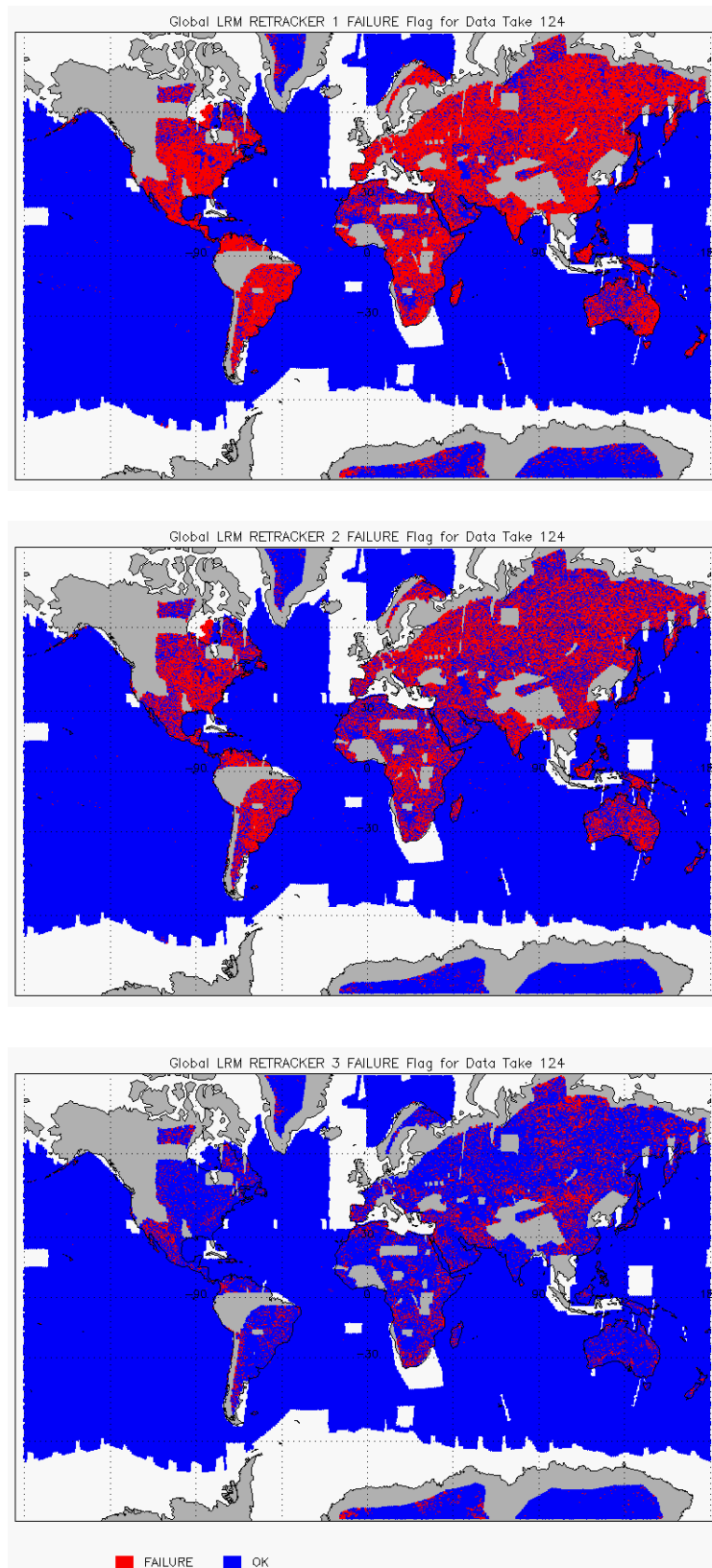
Figure 9 – Global plots showing Retracker Failure Flags for LRM mode for cycle #124:
