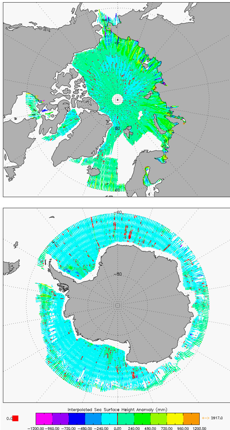
Figure 7 –Polar plots of SSHA for cycle #123.
