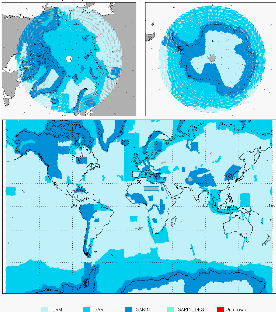
Figure 3 - Global and Polar plots of SIRAL Modes for cycle #123.
