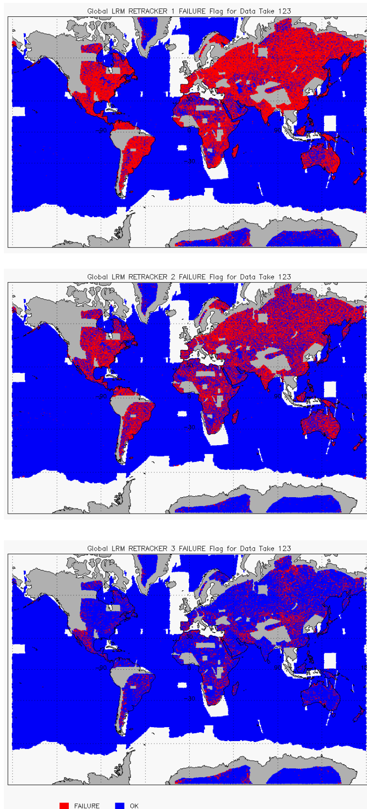
Figure 9 – Global plots showing Retracker Failure Flags for LRM mode for cycle #123:
