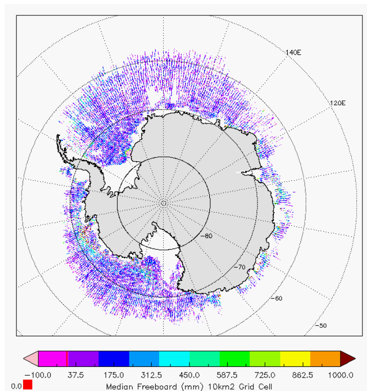
Figure 6 - Polar plots of 10km Gridded Freeboard values from L2 SAR products in cycle #123.
