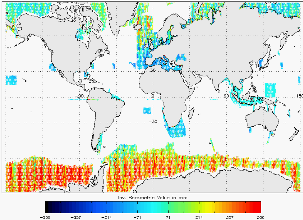
Figure 20 - Global plot of Inverse Barometric Correction for cycle #123
