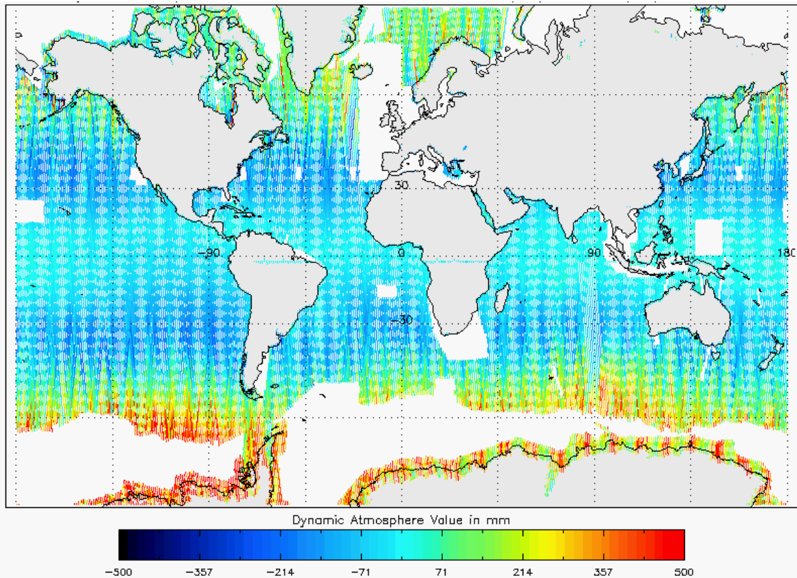
Figure 22 - Global plot of Dynamic Atmospheric Correction for cycle #123
