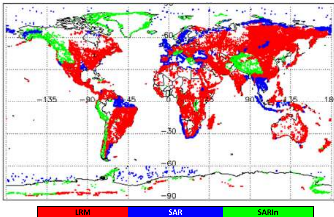
Figure 1 – Global plot showing areas of loss of track in all SIRAL modes L0 data during November 2020
