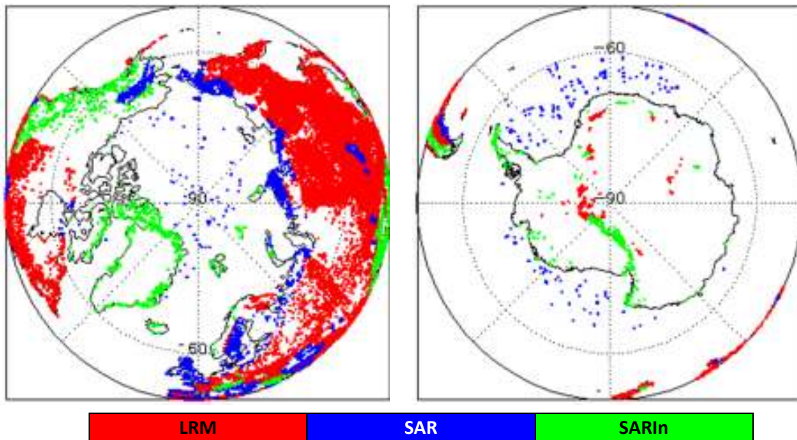
Figure 2 - Polar plots showing areas of loss of track in all SIRAL modes L0 data during November 2020.
