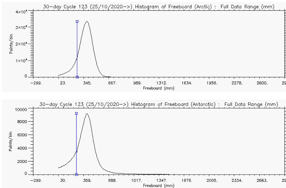
Figure 5 – Histogram of Freeboard for Arctic (above) and Antarctic (below) for cycle #123
