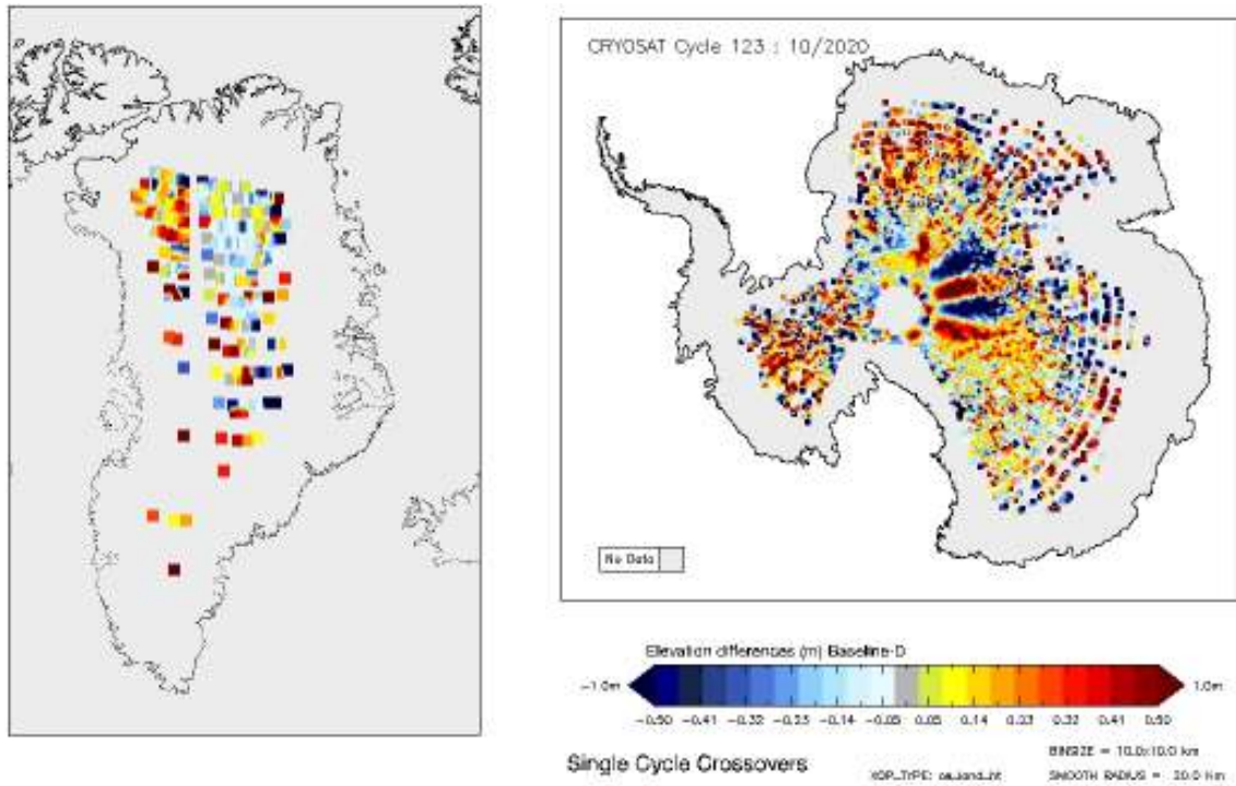
Figure 14 - Greenland and Antarctica maps of LRM elevation differences for cycle #123.
