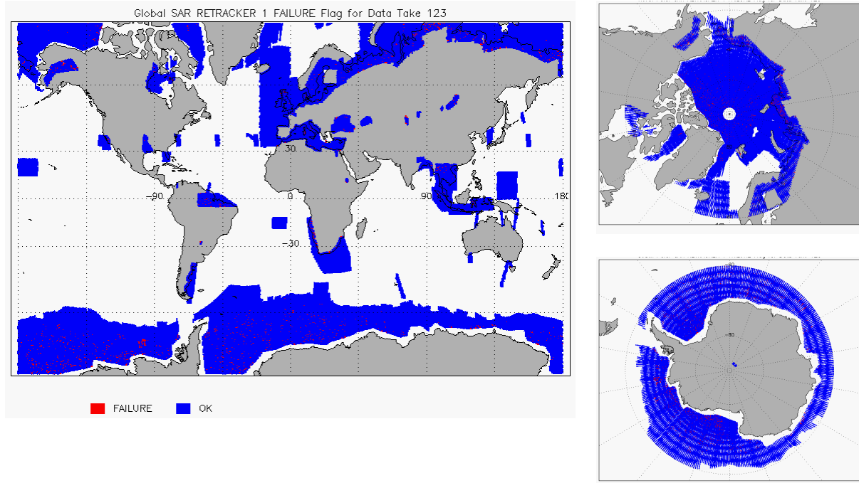
Figure 10 - Global plots showing Retracker Failure Flags for SAR mode for cycle #123
