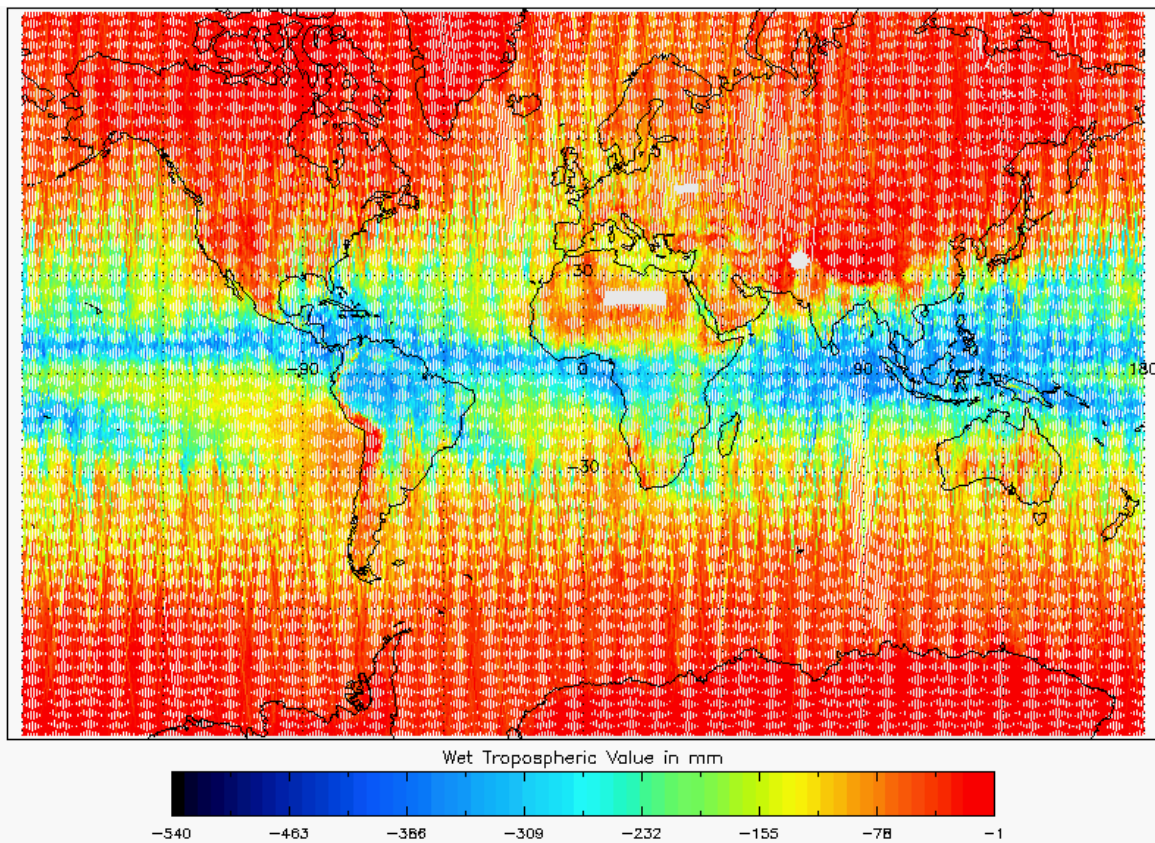
Figure 18 - Global plot of Wet Tropospheric Correction for cycle #123
