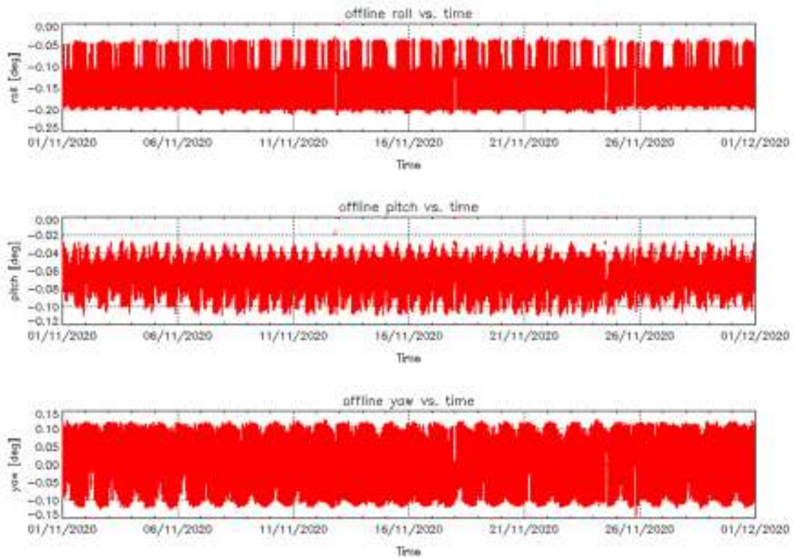
Figure 4 – Roll (top), Pitch (middle) and Yaw (bottom) values for L1B Products during cycle #123.
