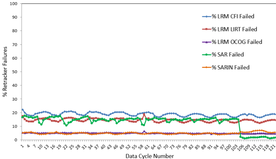
Figure 9 – Time Series for Retracker Failure Flags
