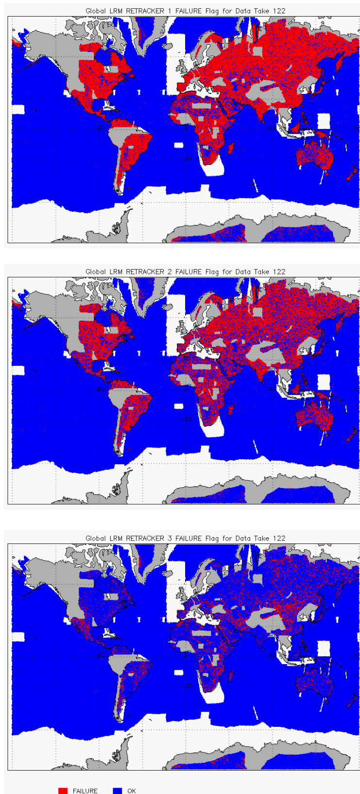
Figure 10 – Global plots showing Retracker Failure Flags for LRM mode for cycle #122: LRM CFI (top), LRM LIRT (middle), LRM OCOG (bottom)
