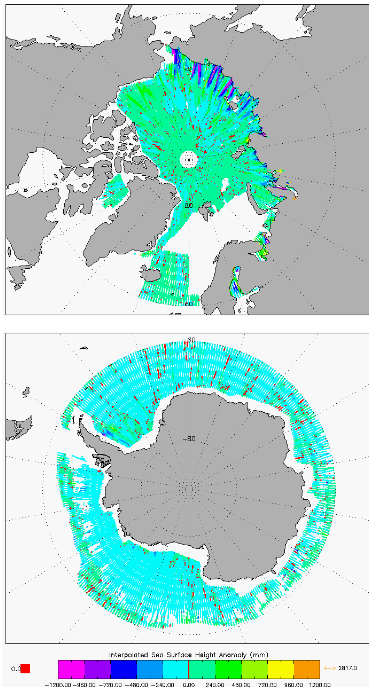
Figure 8 –Polar plots of SSHA for cycle #122.
