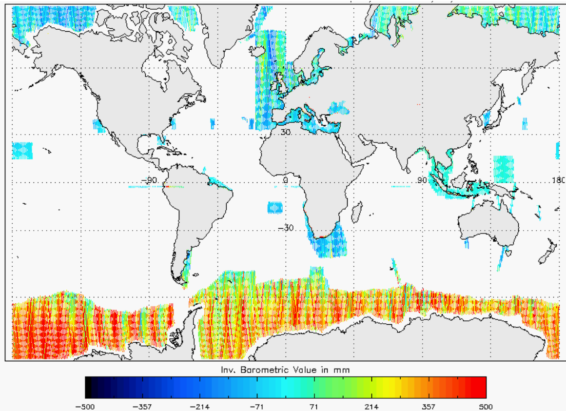
Figure 21 - Global plot of Inverse Barometric Correction for cycle #122
