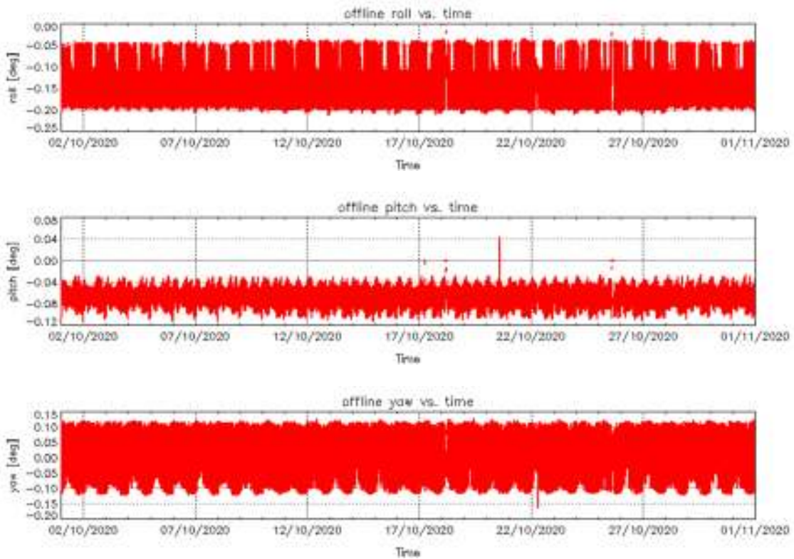
Figure 4 – Roll (top), Pitch (middle) and Yaw (bottom) values for L1B Products during cycle #122.
