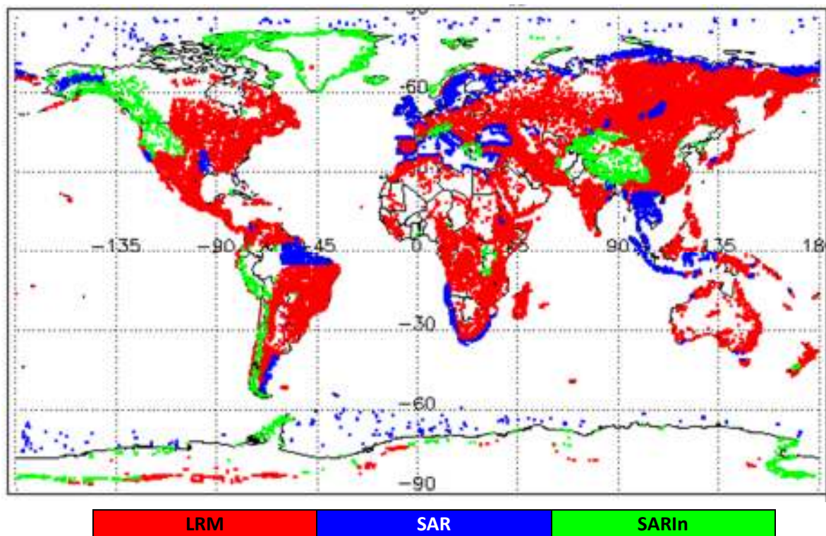
Figure 1 – Global plot showing areas of loss of track in all SIRAL modes L0 data during October 2020
