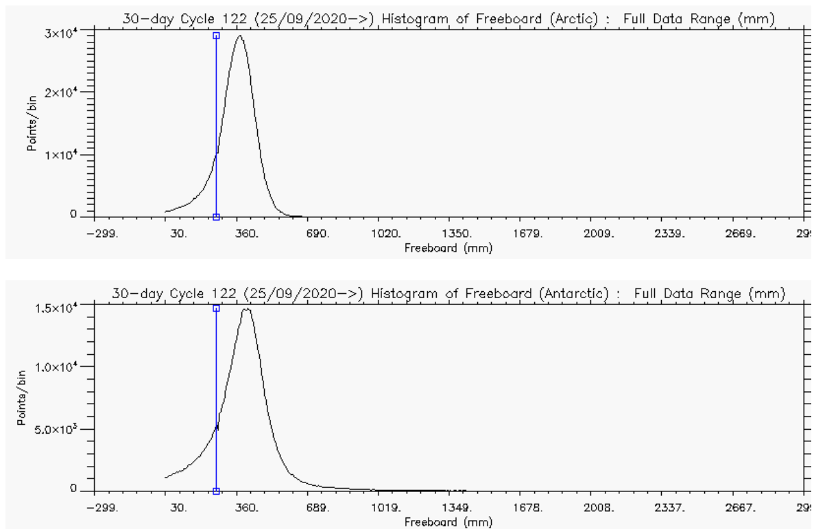
Figure 6 – Histogram of Freeboard for Arctic (above) and Antarctic (below) for cycle #122
