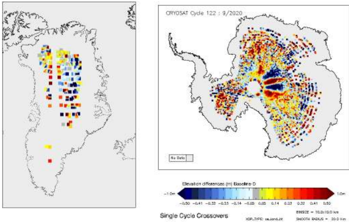
Figure 15 - Greenland and Antarctica maps of LRM elevation differences for cycle #122.
