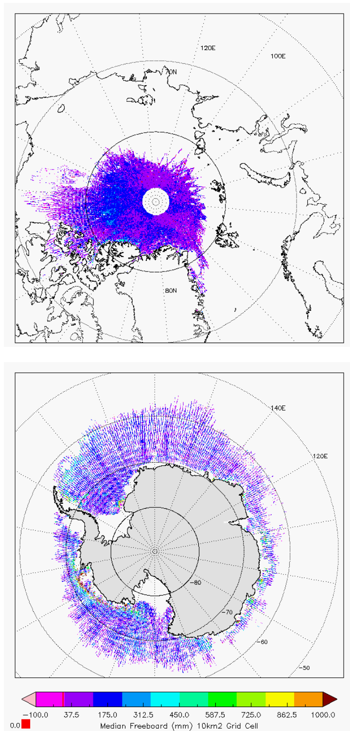
Figure 7 - Polar plots of 10km Gridded Freeboard values from L2 SAR products in cycle #122.
