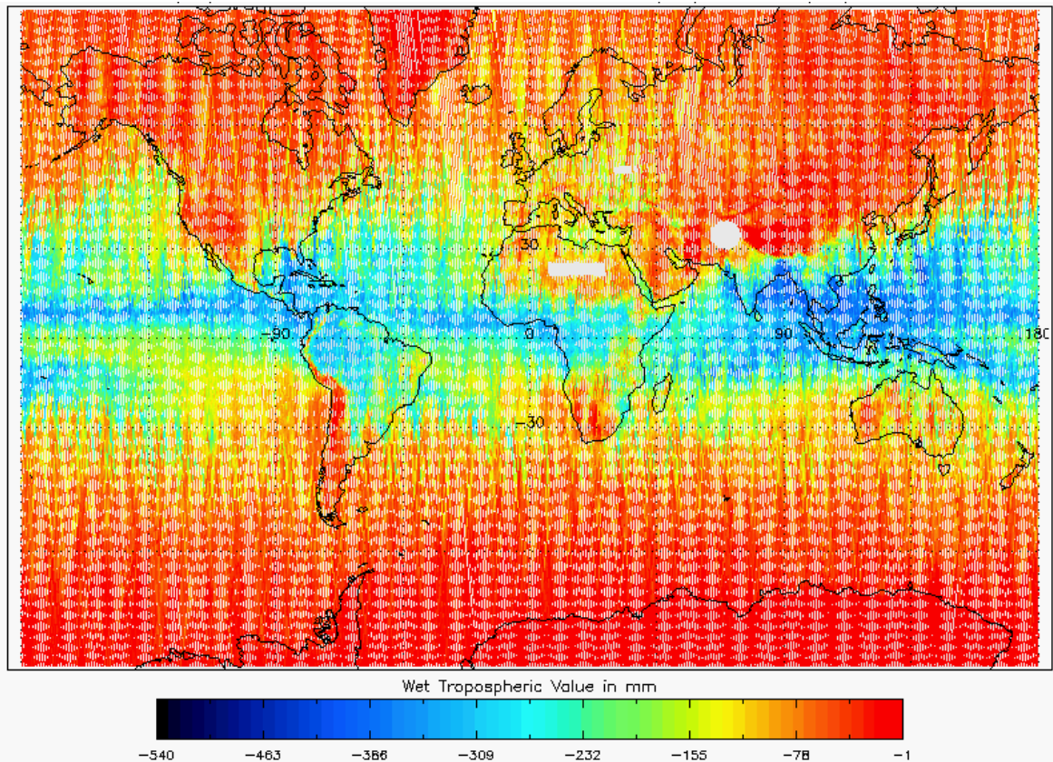
Figure 19 - Global plot of Wet Tropospheric Correction for cycle #122
