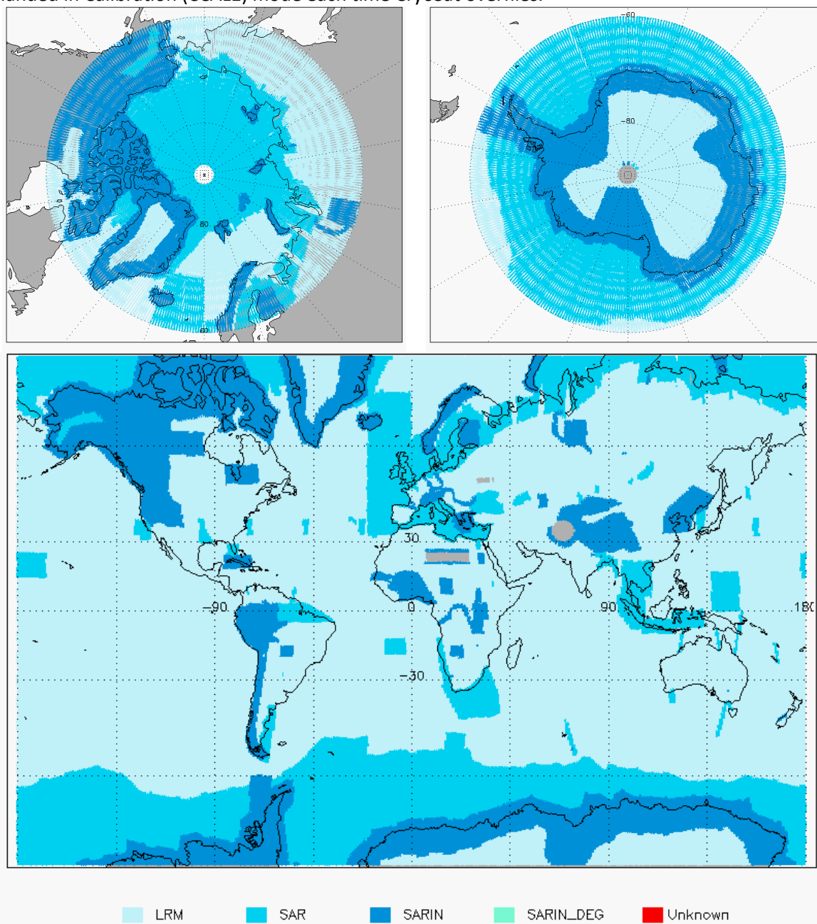
Figure 3 - Global and Polar plots of SIRAL Modes for cycle #122.
