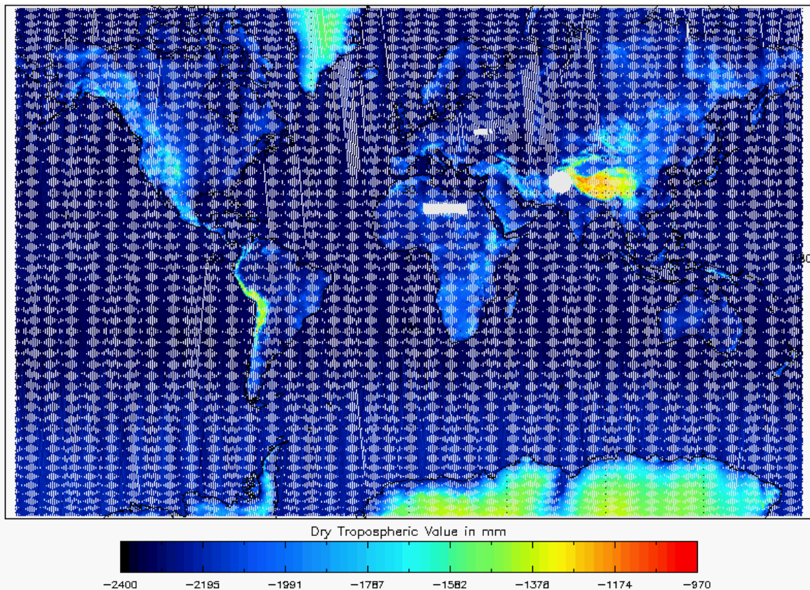
Figure 17 - Global plot of Dry Tropospheric Correction for cycle #122
