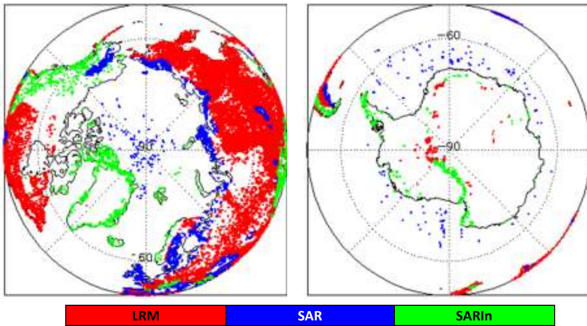
Figure 2 - Polar plots showing areas of loss of track in all SIRAL modes L0 data during October 2020.
