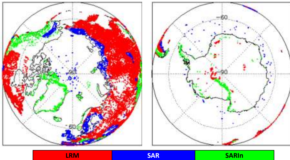
Figure 2 - Polar plots showing areas of loss of track in all SIRAL modes L0 data during September 2020.
