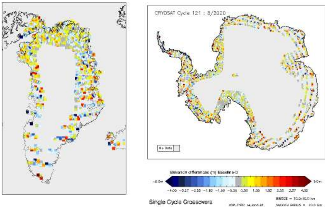
Figure 15 - Greenland and Antarctica maps of SARIn elevation differences for cycle #121.
