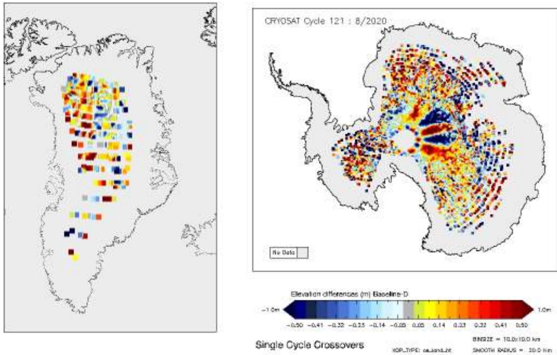
Figure 14 - Greenland and Antarctica maps of LRM elevation differences for cycle #121.
