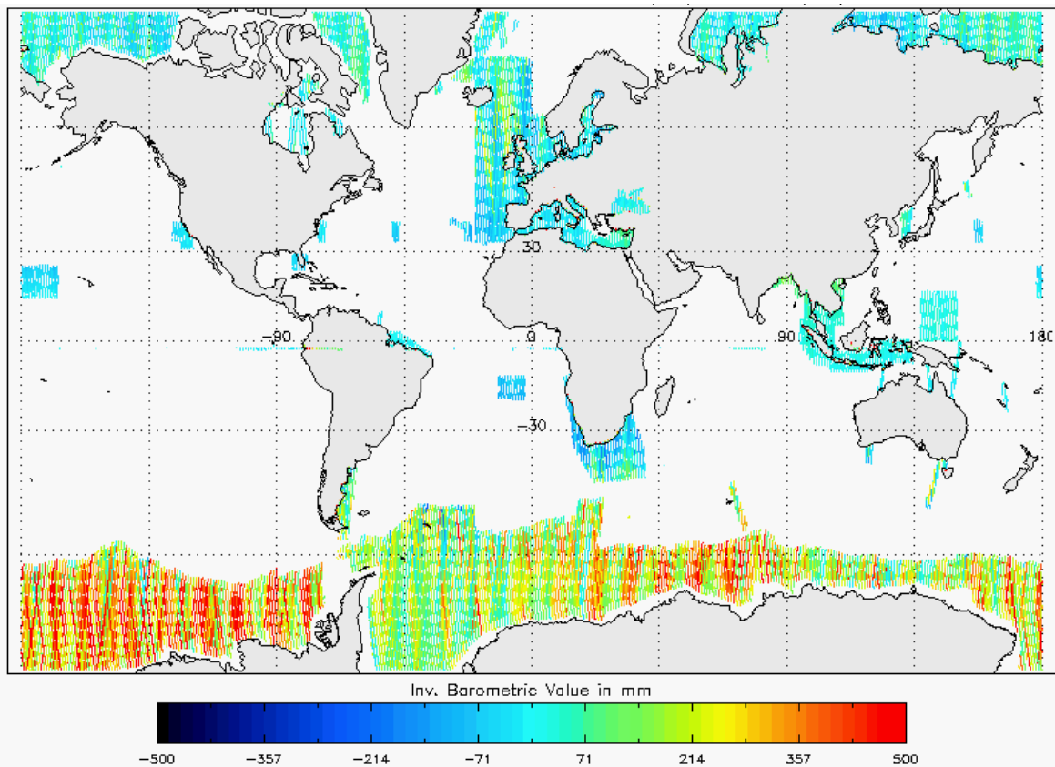
Figure 21 - Global plot of Inverse Barometric Correction for cycle #120
