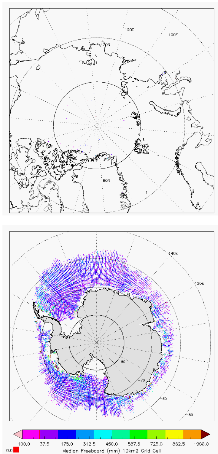
Figure 7 - Polar plots of 10km Gridded Freeboard values from L2 SAR products in cycle #120.
