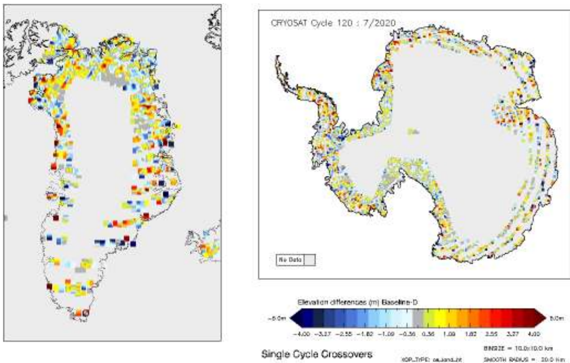
Figure 16 - Greenland and Antarctica maps of SARIn elevation differences for cycle #120.
