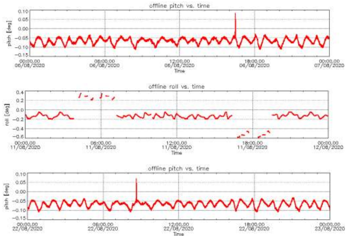
Figure 5 – Spike in pitch due to processing errors on 06/08/2020 (top), Anomaly in roll due to roll manoeuvre on 11/08/2020 (middle), Spike in pitch due to processing errors on 22/08/2020 (bottom).
