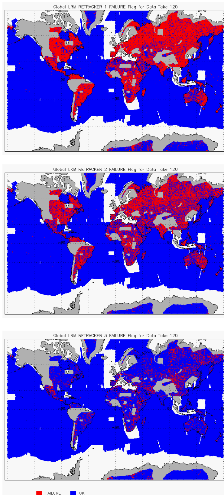
Figure 10 – Global plots showing Retracker Failure Flags for LRM mode for cycle #120: LRM CFI (top), LRM LIRT (middle), LRM OCOG (bottom)
