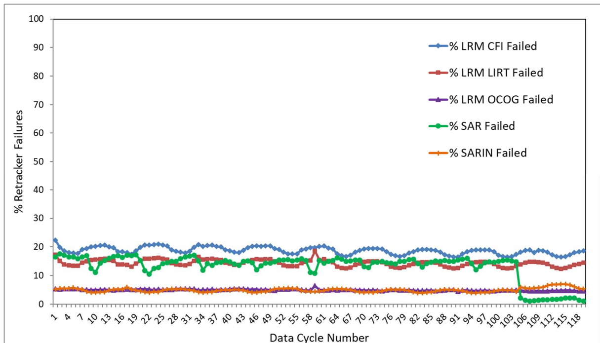
Figure 9 – Time Series for Retracker Failure Flags
