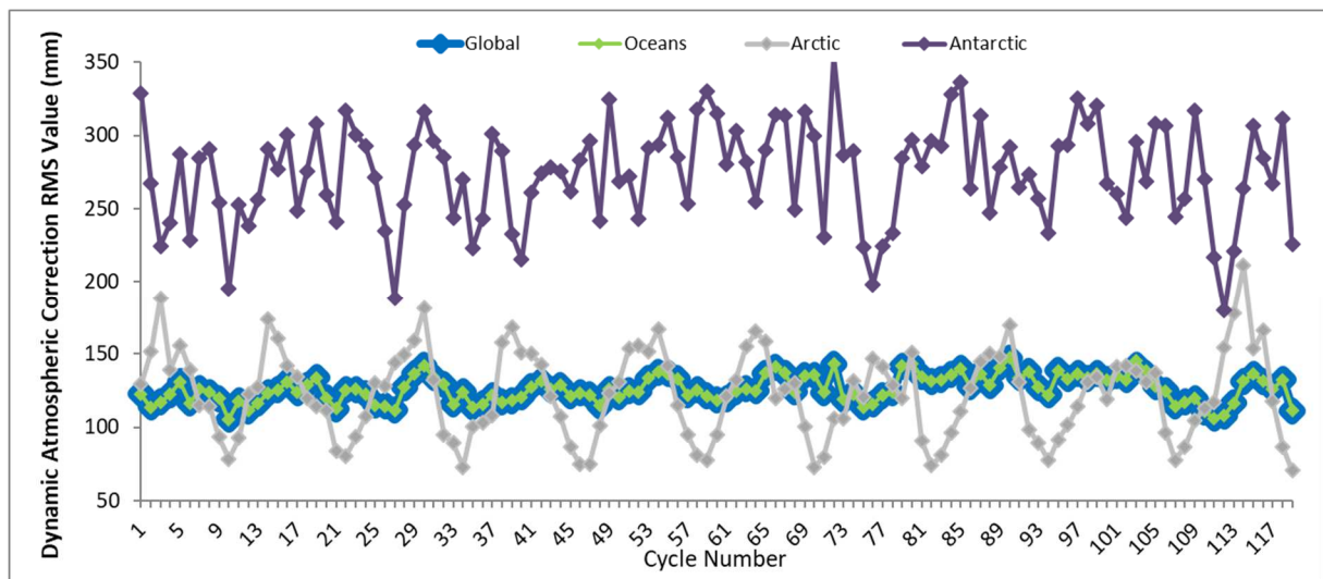
Figure 24 – Dynamic Atmospheric Correction RMS value trend from beginning of mission
