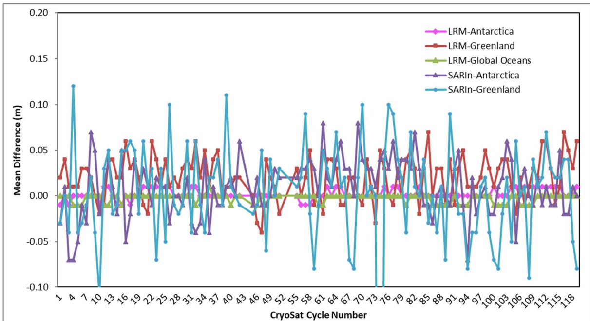
Figure 14 - Time series for Mean Difference in elevation at crossovers from beginning of the mission
