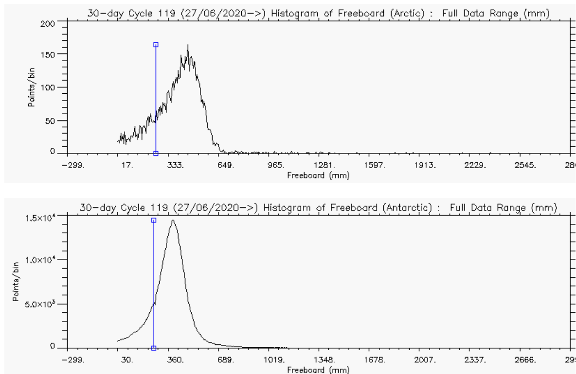
Figure 6 – Histogram of Freeboard for Arctic (above) and Antarctic (below) for cycle #119
