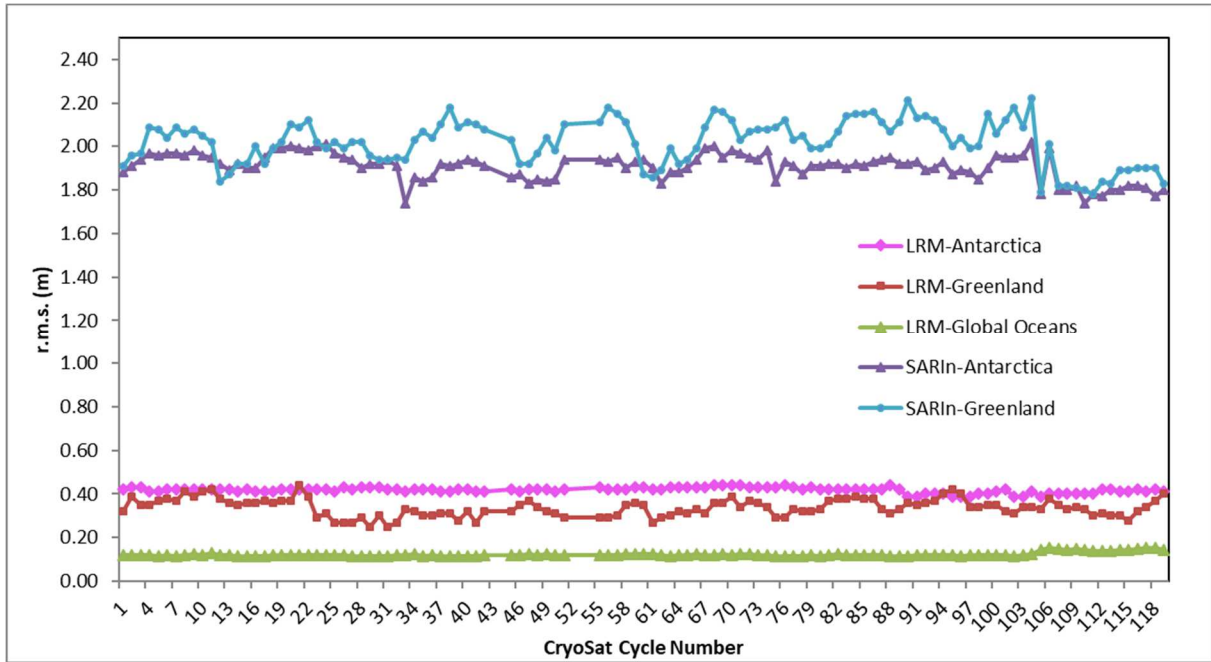
Figure 13 - Time series for crossover elevation r.m.s values from beginning of the mission
