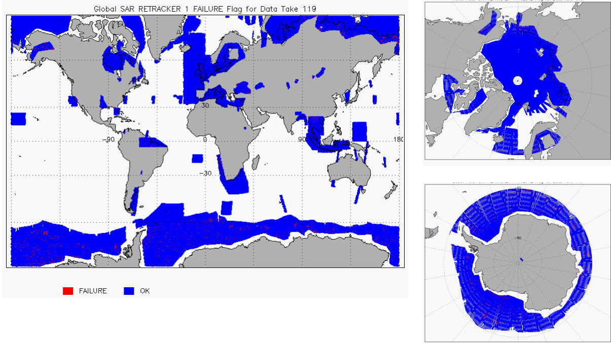
Figure 11 - Global plots showing Retracker Failure Flags for SAR mode for cycle #119
