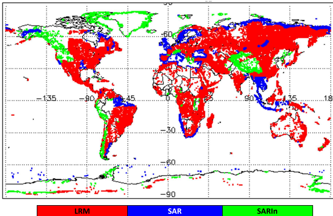
Figure 1 – Global plot showing areas of loss of track in all SIRAL modes L0 data during July 2020
