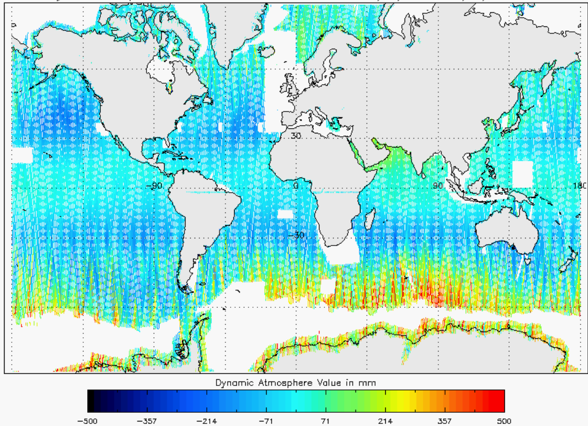
Figure 23 - Global plot of Dynamic Atmospheric Correction for cycle #119
