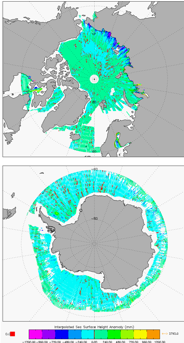
Figure 8 –Polar plots of SSHA for cycle #119.
