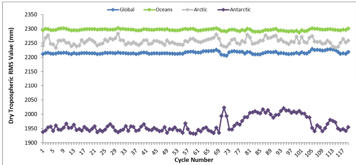
Figure 18 - Dry Tropospheric Correction RMS value trend from beginning of mission
