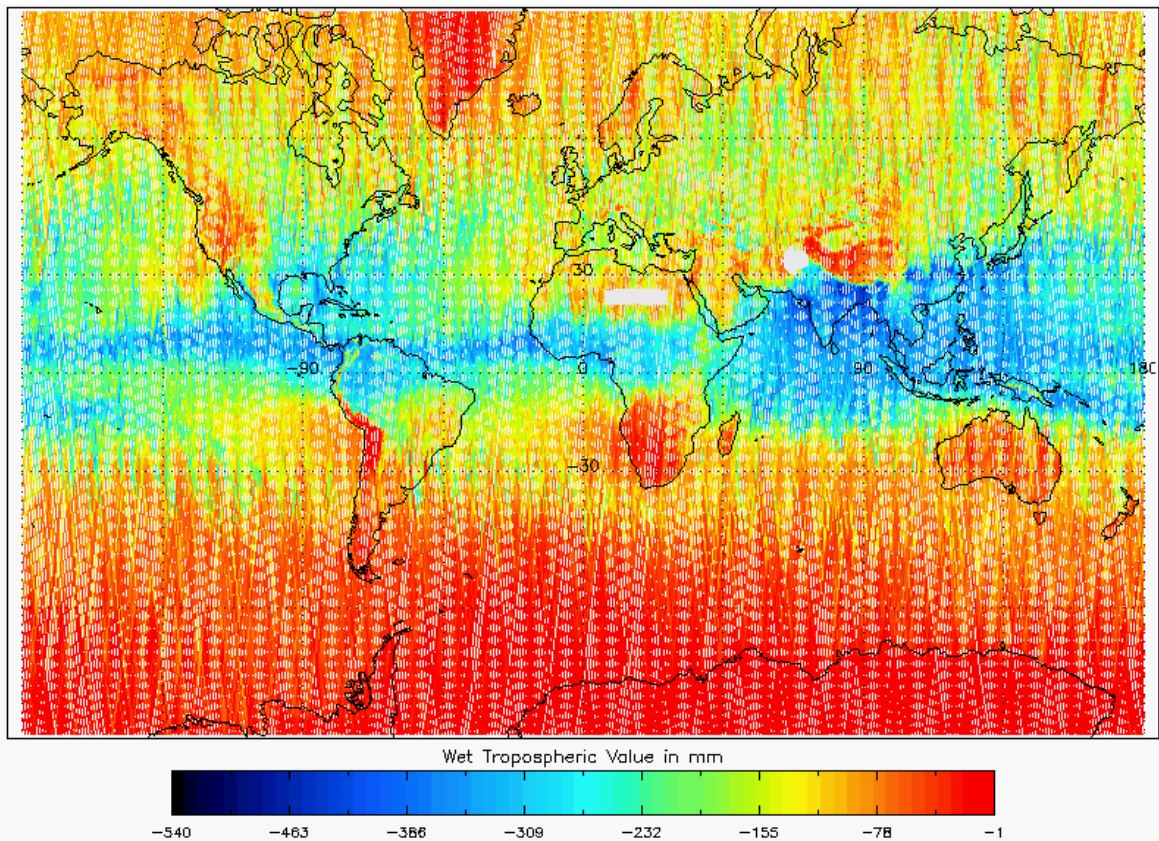
Figure 19 - Global plot of Wet Tropospheric Correction for cycle #119
