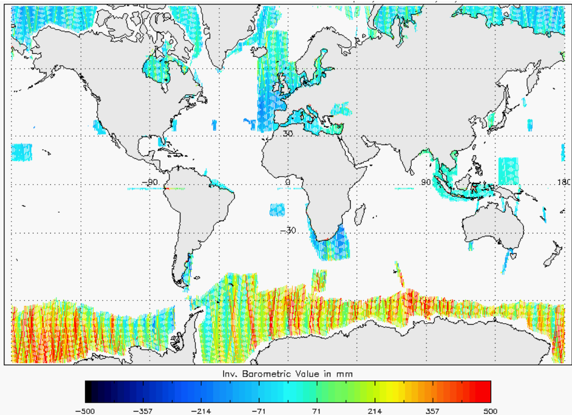
Figure 21 - Global plot of Inverse Barometric Correction for cycle #119
