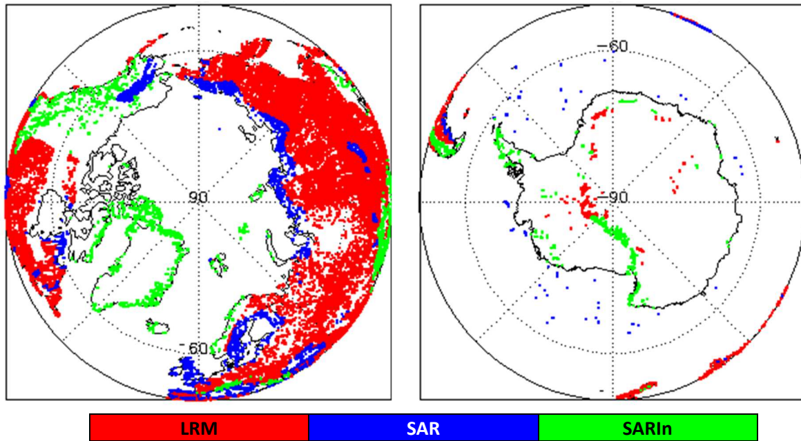
Figure 2 - Polar plots showing areas of loss of track in all SIRAL modes L0 data during July 2020.
