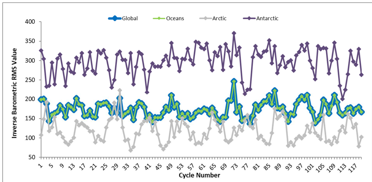
Figure 22 – Inverse Barometric Correction RMS value trend from beginning of mission
