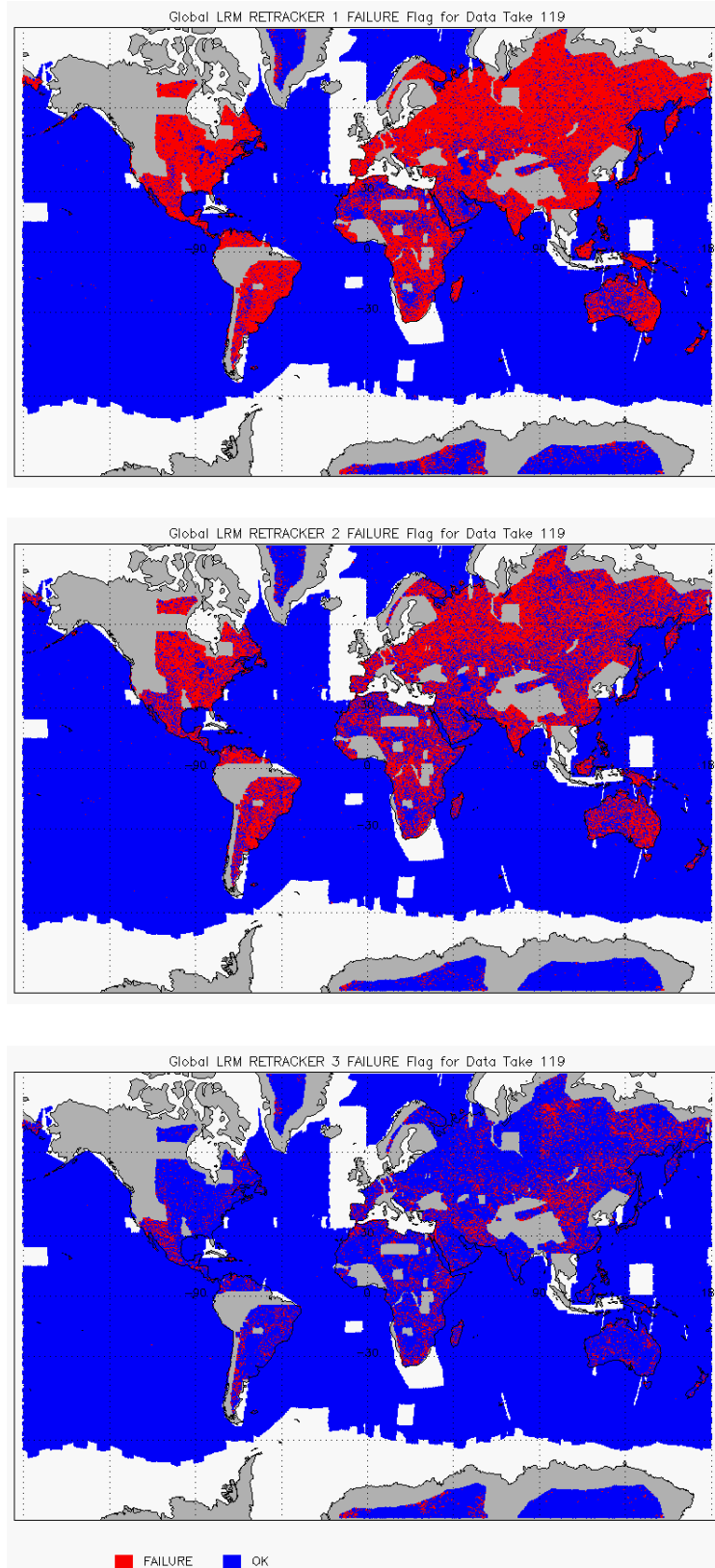
Figure 10 – Global plots showing Retracker Failure Flags for LRM mode for cycle #119: LRM CFI (top), LRM LIRT (middle), LRM OCOG (bottom)
