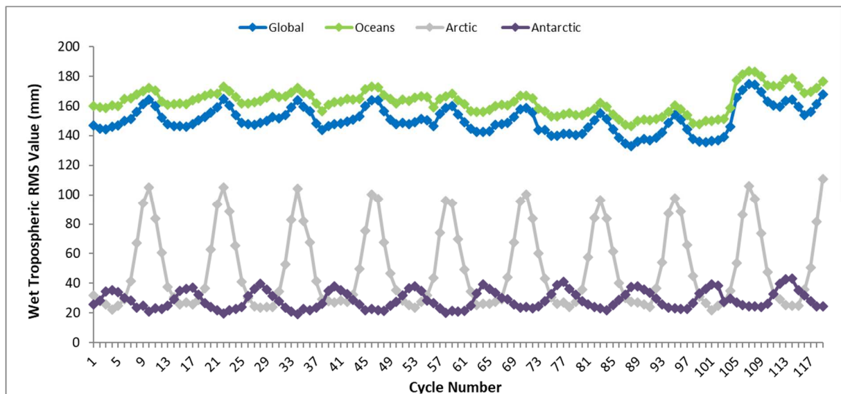
Figure 20 – Wet Tropospheric Correction RMS value trend from beginning of mission
