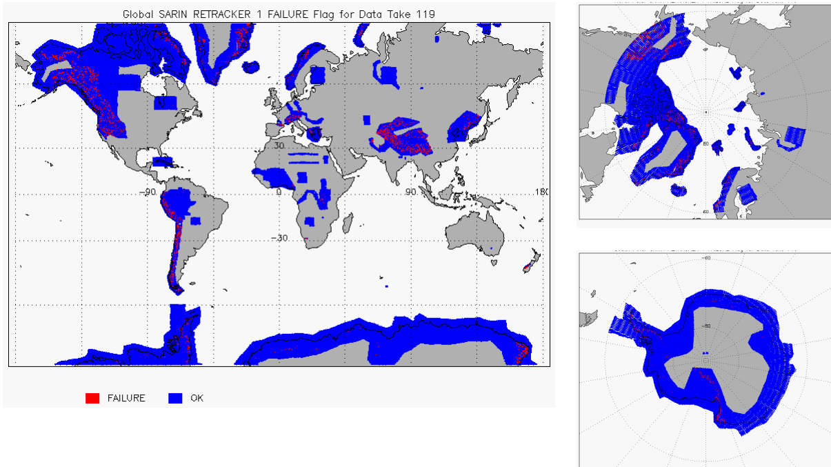
Figure 12 – Global plots showing Retracker Failure Flags for SARIn mode for cycle #119
