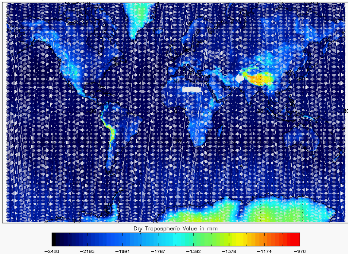
Figure 17 - Global plot of Dry Tropospheric Correction for cycle #119
