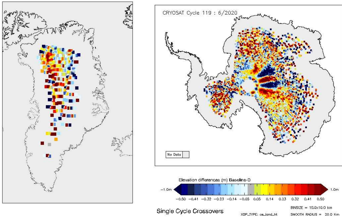
Figure 15 - Greenland and Antarctica maps of LRM elevation differences for cycle #119.
