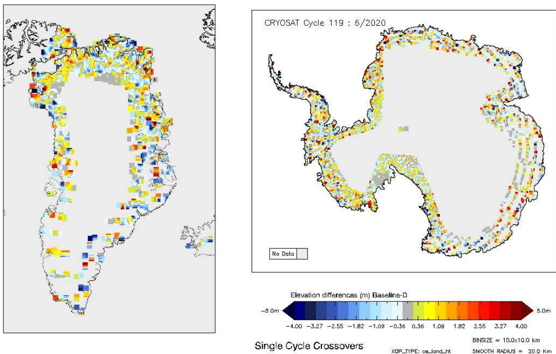
Figure 16 - Greenland and Antarctica maps of SARIn elevation differences for cycle #119.
