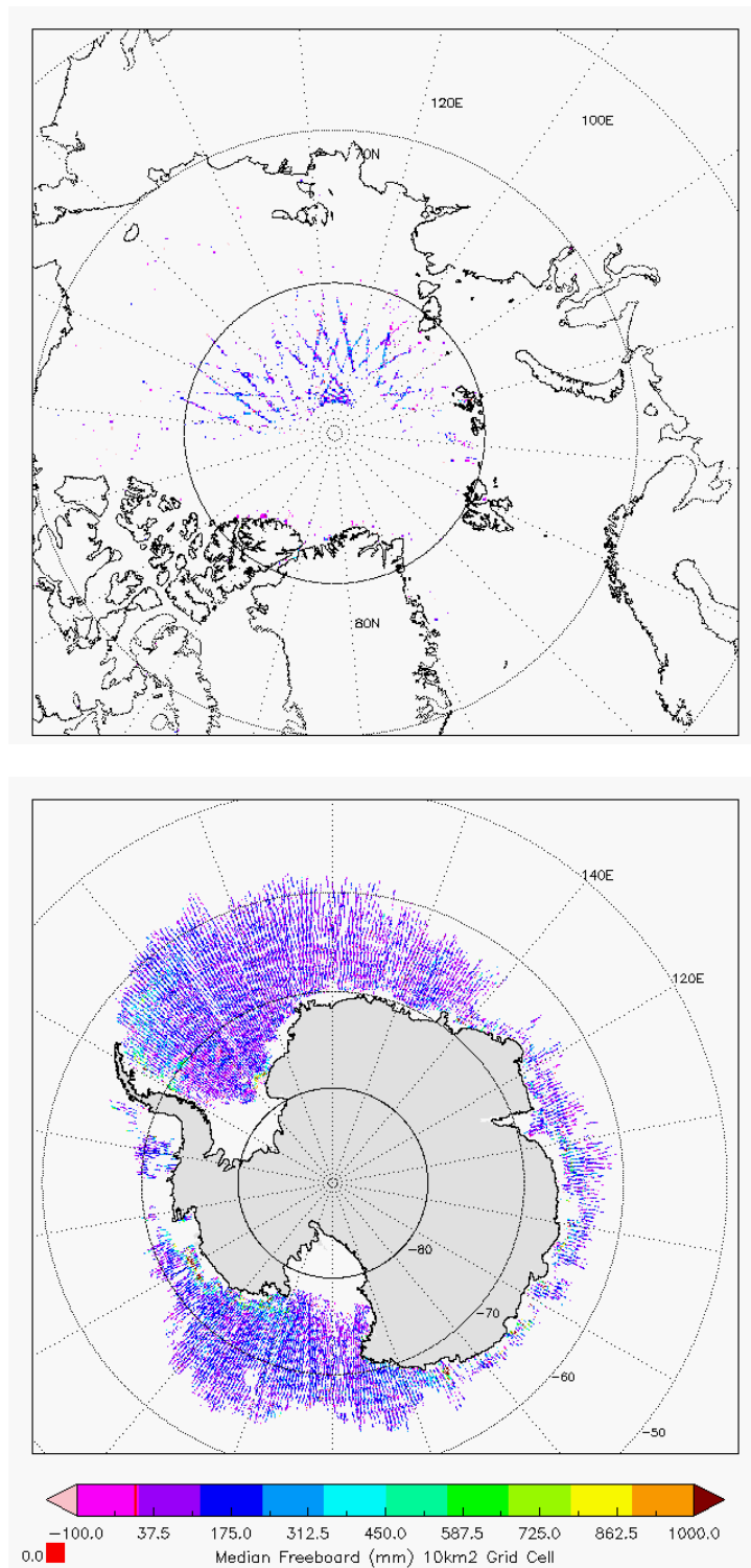
Figure 7 - Polar plots of 10km Gridded Freeboard values from L2 SAR products in cycle #119.
