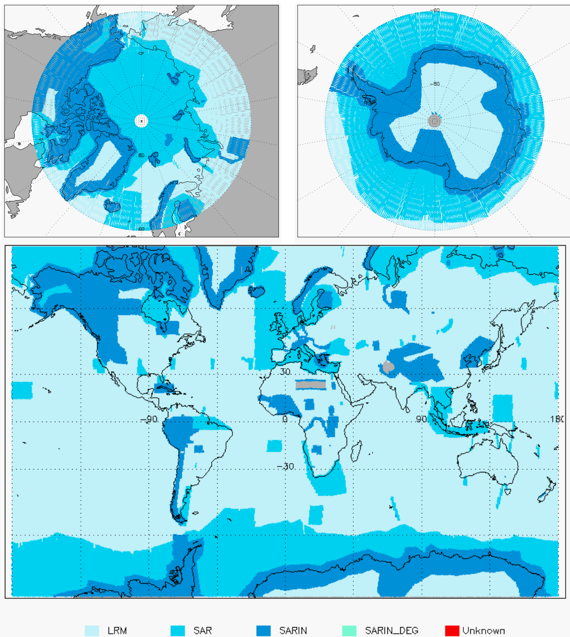
Figure 3 - Global and Polar plots of SIRAL Modes for cycle #119.
