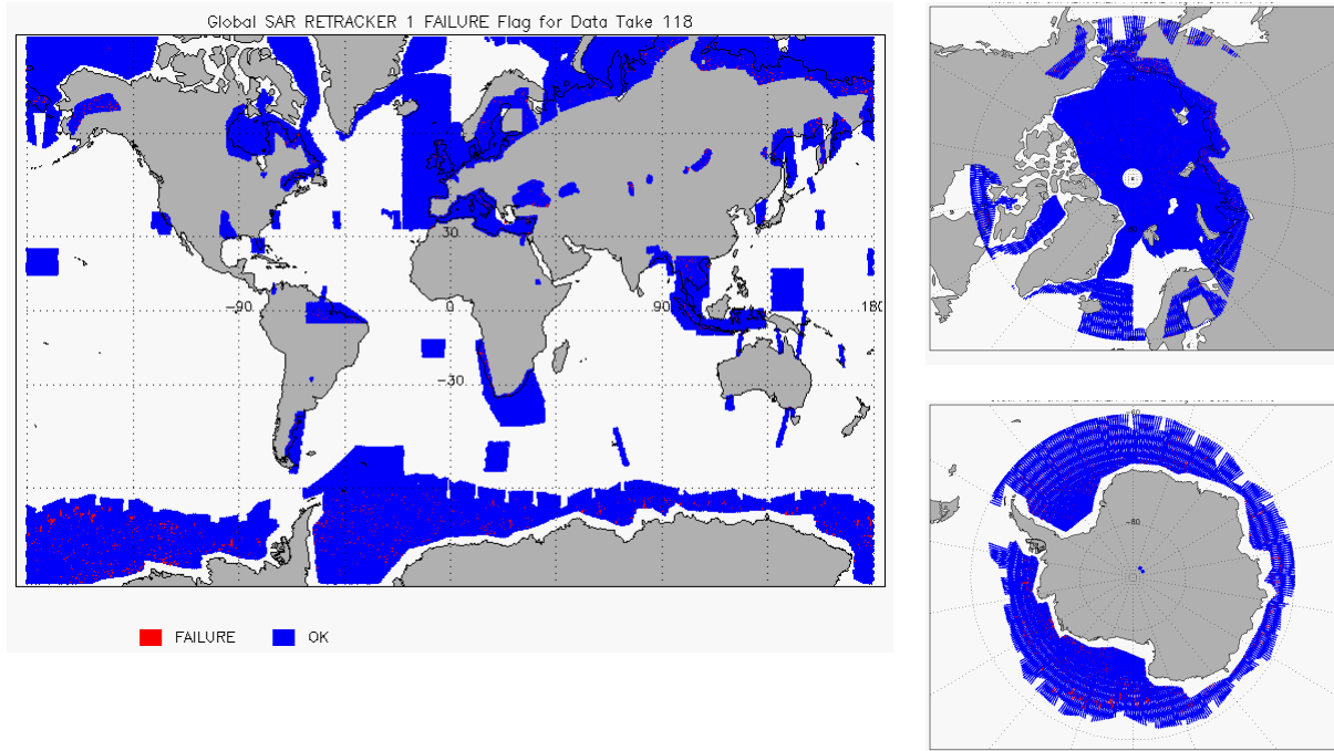
Figure 10 - Global plots showing Retracker Failure Flags for SAR mode for cycle #118
