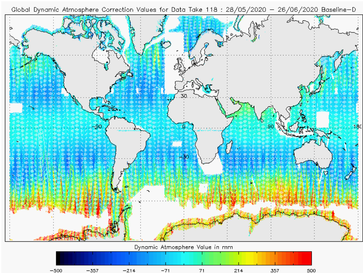
Figure 22 - Global plot of Dynamic Atmospheric Correction for cycle #118
