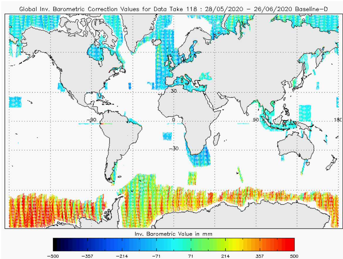
Figure 20 - Global plot of Inverse Barometric Correction for cycle #118
