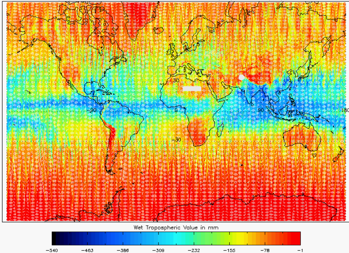
Figure 18 - Global plot of Wet Tropospheric Correction for cycle #118
