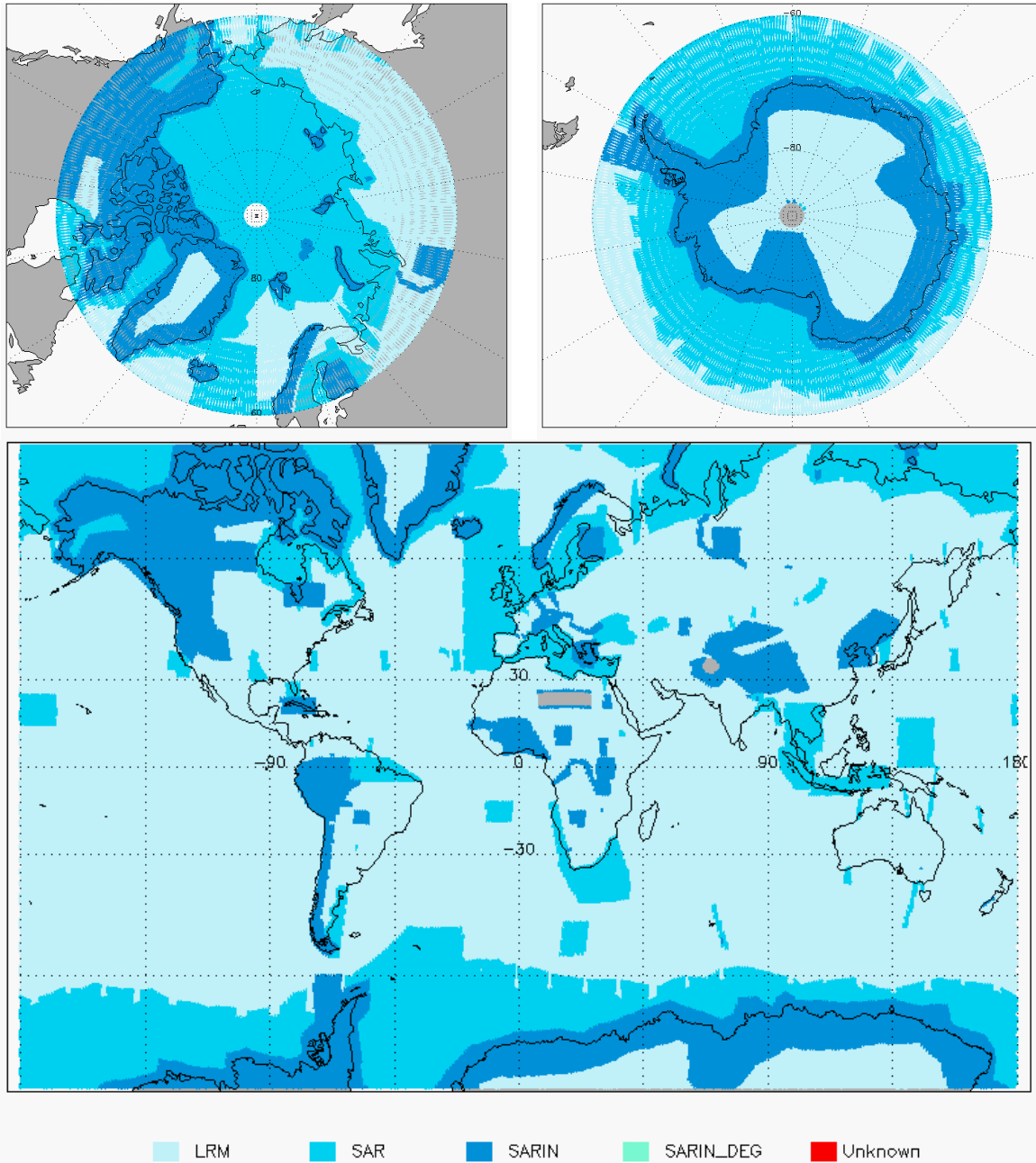
Figure 3 - Global and Polar plots of SIRAL Modes for cycle #118.
