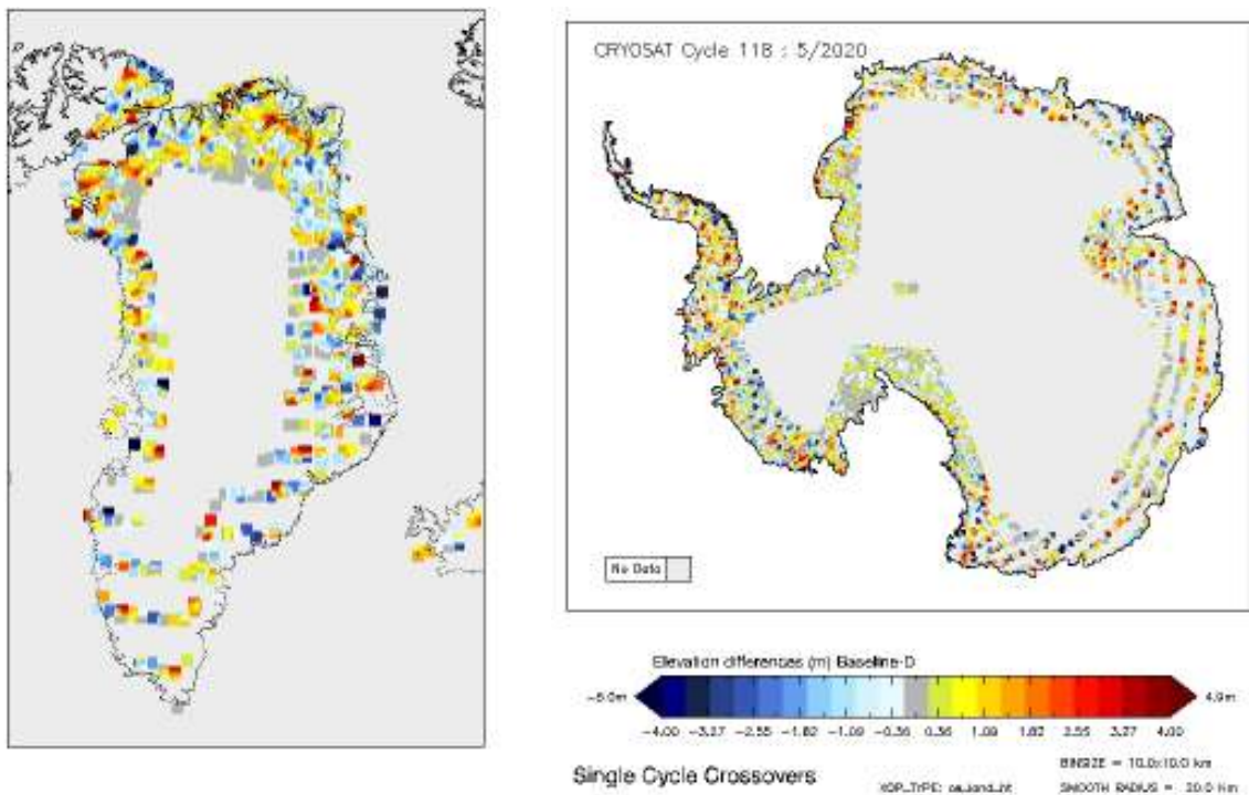
Figure 15 - Greenland and Antarctica maps of SARIn elevation differences for cycle #118.
