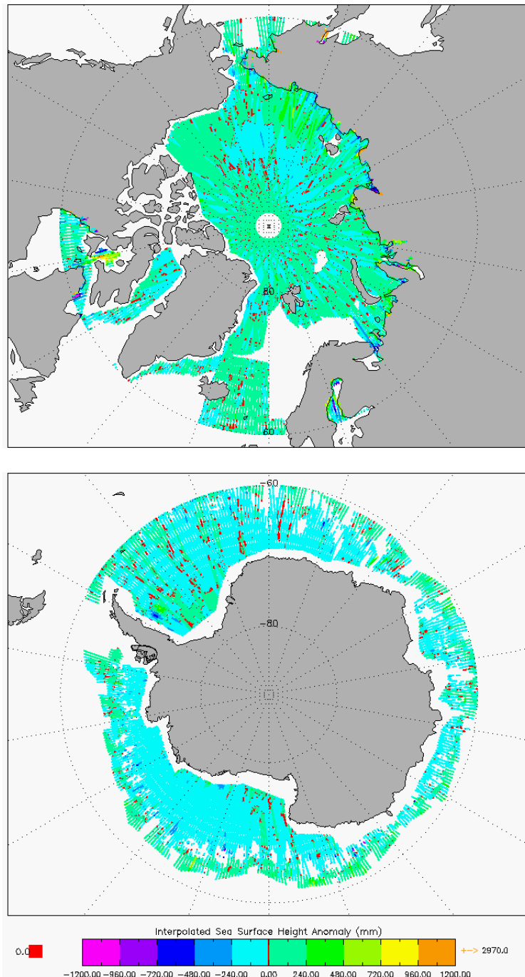
Figure 7 –Polar plots of SSHA for cycle #118.
