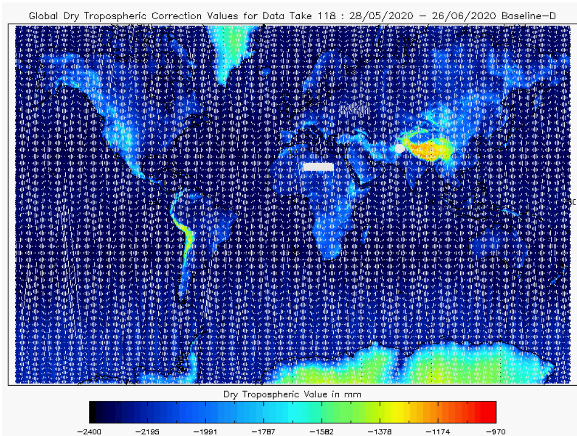
Figure 16 - Global plot of Dry Tropospheric Correction for cycle #118
