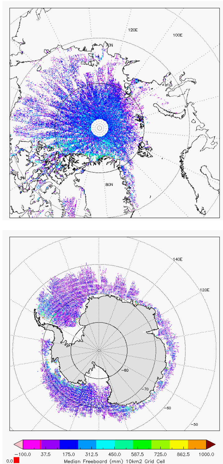
Figure 6 - Polar plots of 10km Gridded Freeboard values from L2 SAR products in cycle #118.
