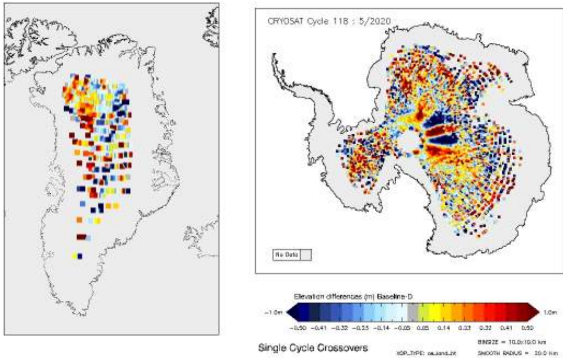
Figure 14 - Greenland and Antarctica maps of LRM elevation differences for cycle #118.
