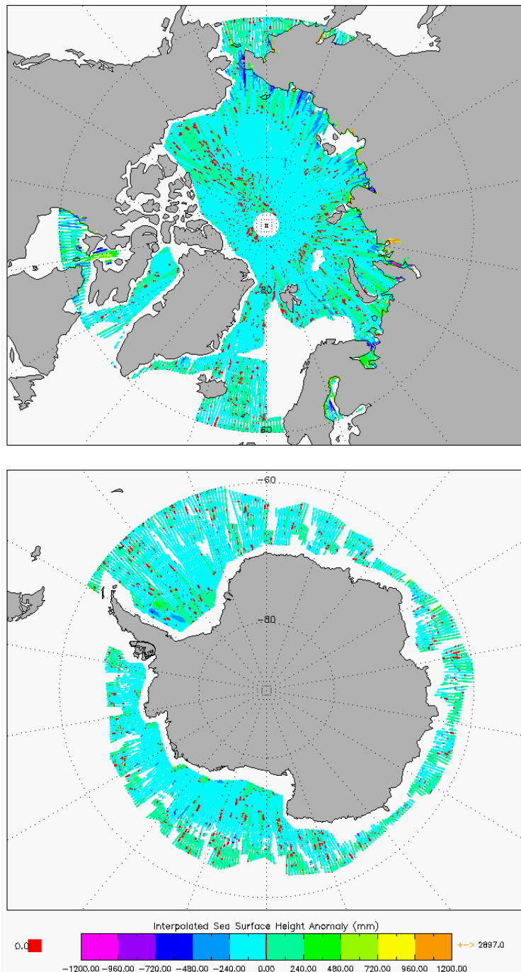
Figure 7 –Polar plots of SSHA for cycle #117.
