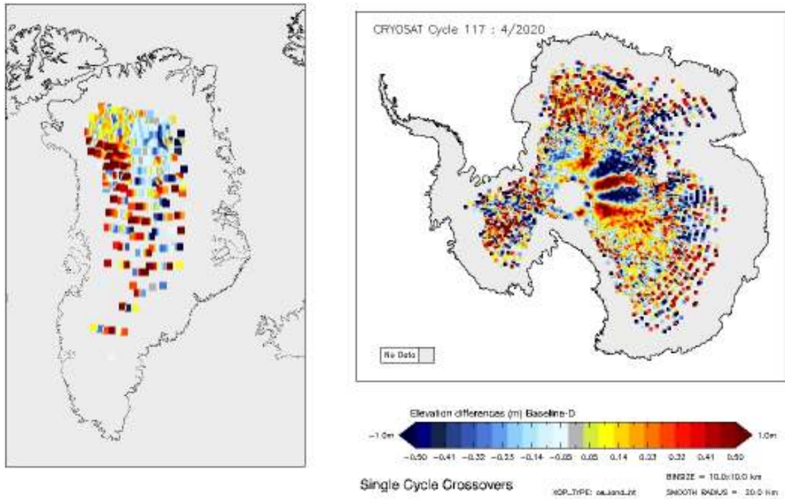
Figure 14 - Greenland and Antarctica maps of LRM elevation differences for cycle #117.
