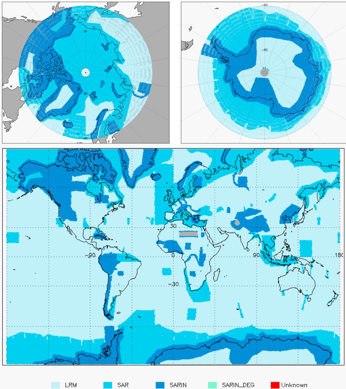
Figure 3 - Global and Polar plots of SIRAL Modes for cycle #117.
