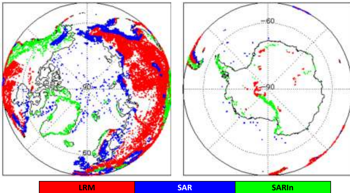
Figure 2 - Polar plots showing areas of loss of track in all SIRAL modes L0 data during May 2020.
