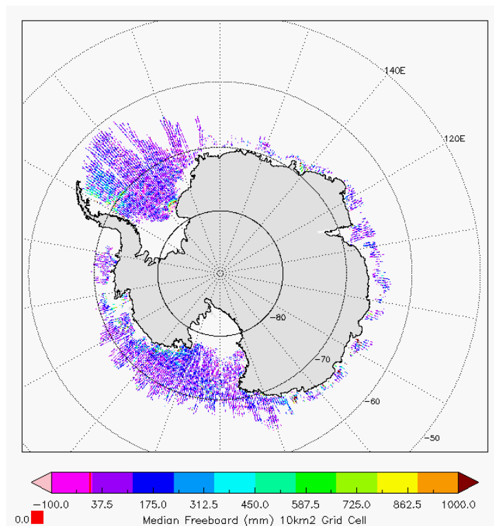
Figure 6 - Polar plots of 10km Gridded Freeboard values from L2 SAR products in cycle #117.
