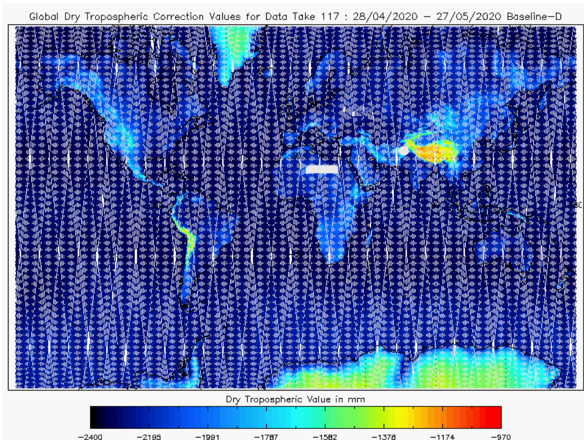
Figure 16 - Global plot of Dry Tropospheric Correction for cycle #117
