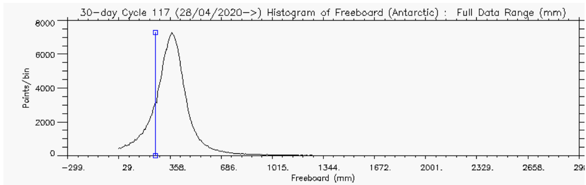
Figure 5 – Histogram of Freeboard for Arctic (above) and Antarctic (below) for cycle #117
