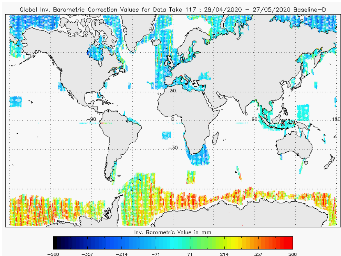
Figure 20 - Global plot of Inverse Barometric Correction for cycle #117
