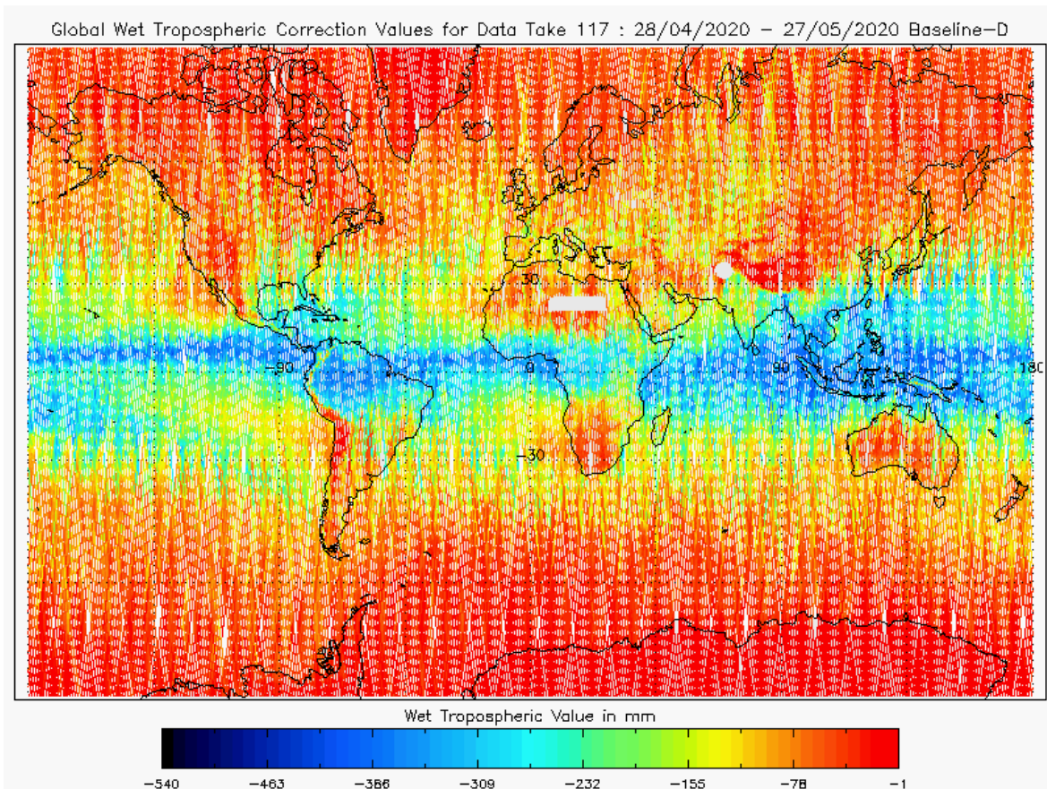
Figure 18 - Global plot of Wet Tropospheric Correction for cycle #117
