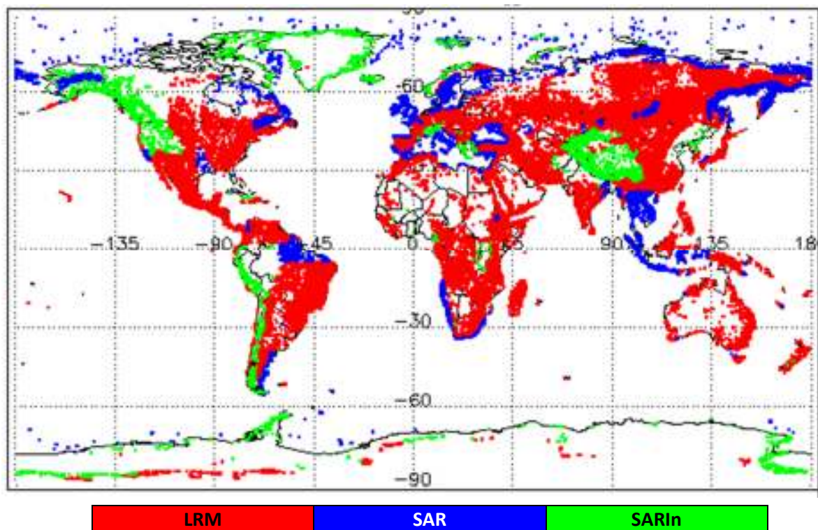
Figure 1 – Global plot showing areas of loss of track in all SIRAL modes L0 data during May 2020
