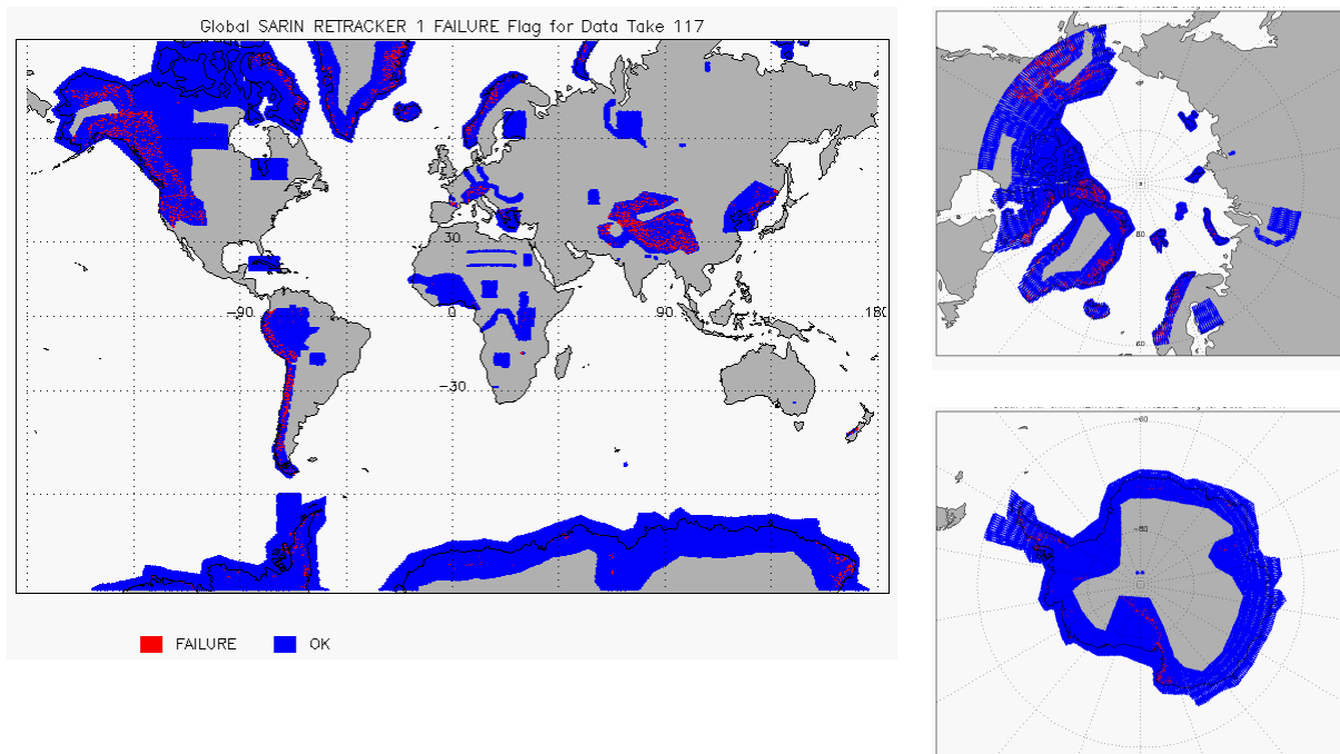
Figure 10 - Global plots showing Retracker Failure Flags for SAR mode for cycle #117
