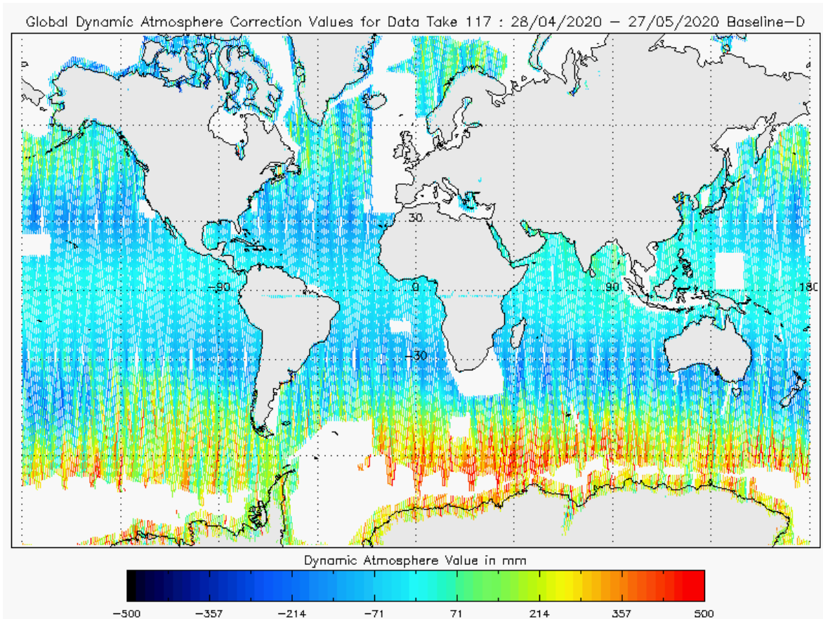
Figure 22 - Global plot of Dynamic Atmospheric Correction for cycle #117
