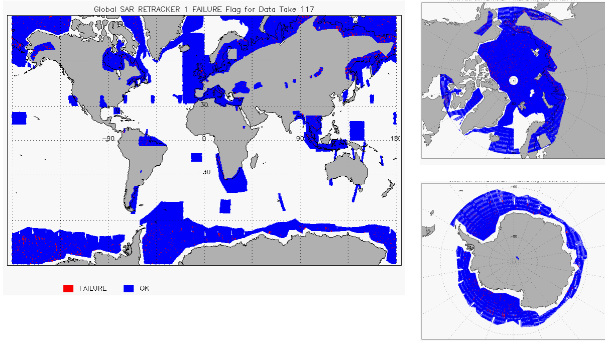
Figure 10 - Global plots showing Retracker Failure Flags for SAR mode for cycle #117
