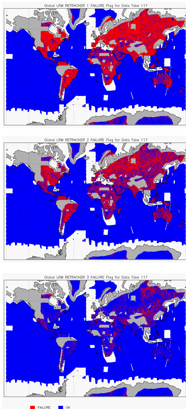
Figure 9 – Global plots showing Retracker Failure Flags for LRM mode for cycle #117:
