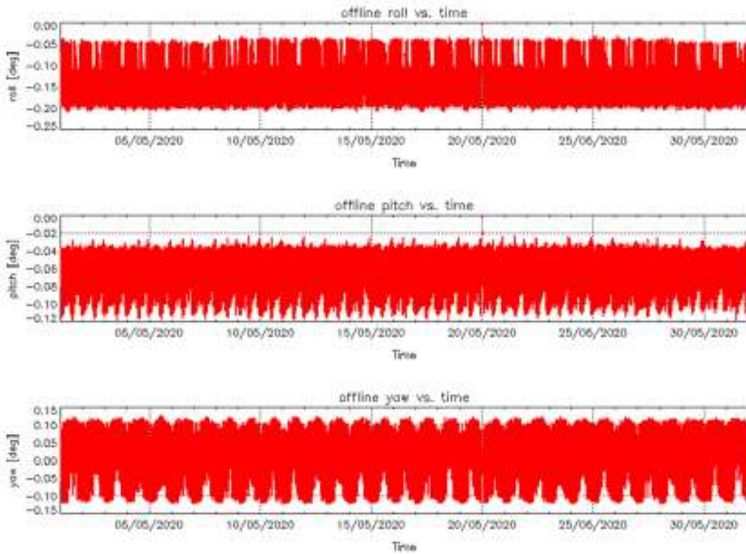
Figure 4 – Roll (top), Pitch (middle) and Yaw (bottom) values for L1B Products during cycle #117.
