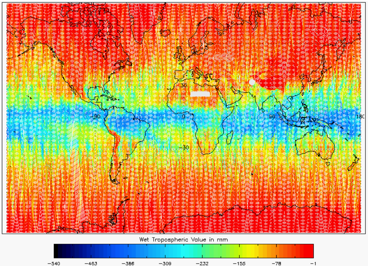
Figure 19 - Global plot of Wet Tropospheric Correction for cycle #116
