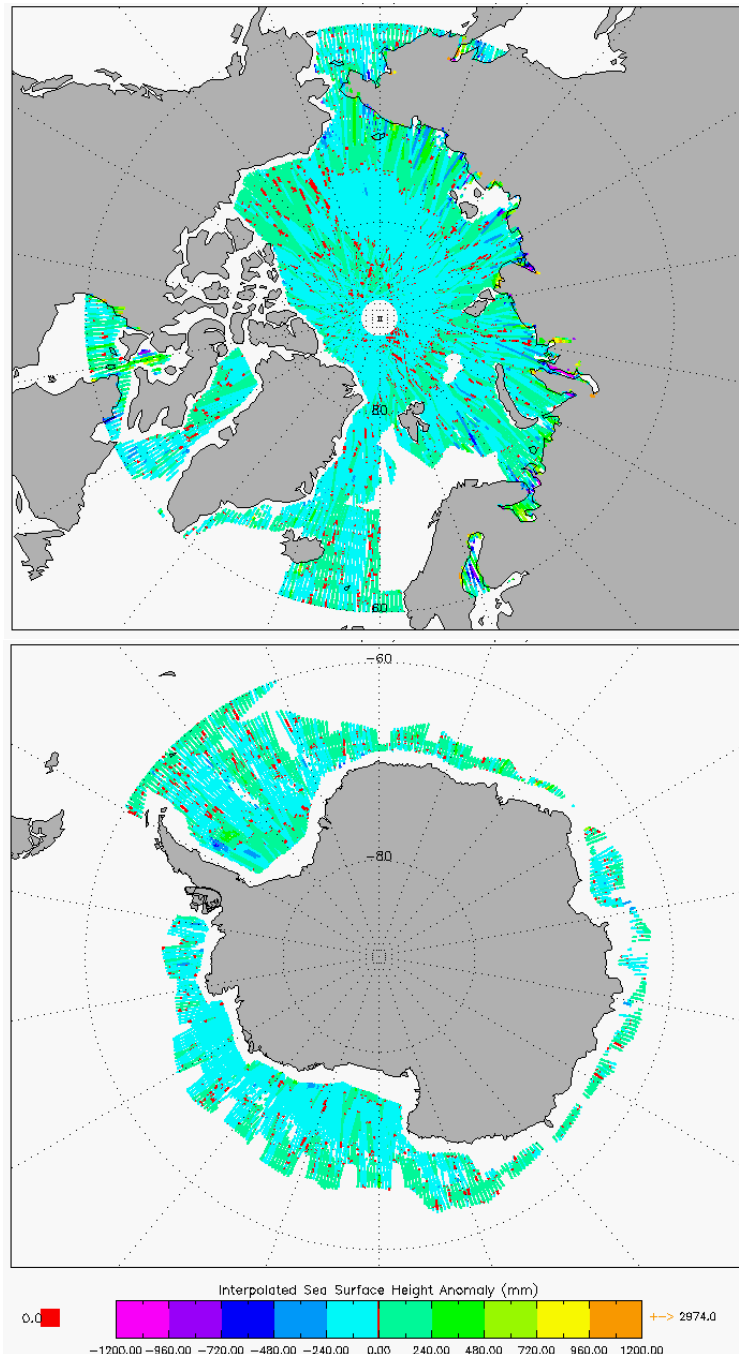
Figure 8 –Polar plots of SSHA for cycle #116.
