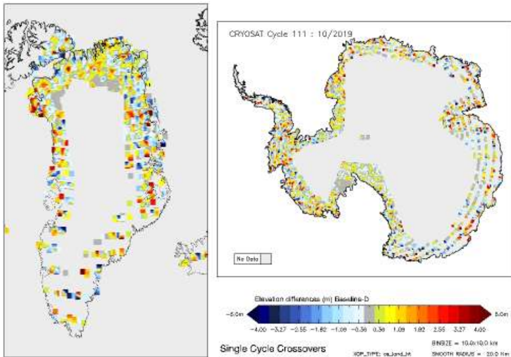
Figure 16 - Greenland and Antarctica maps of SARIn elevation differences for cycle #116.
