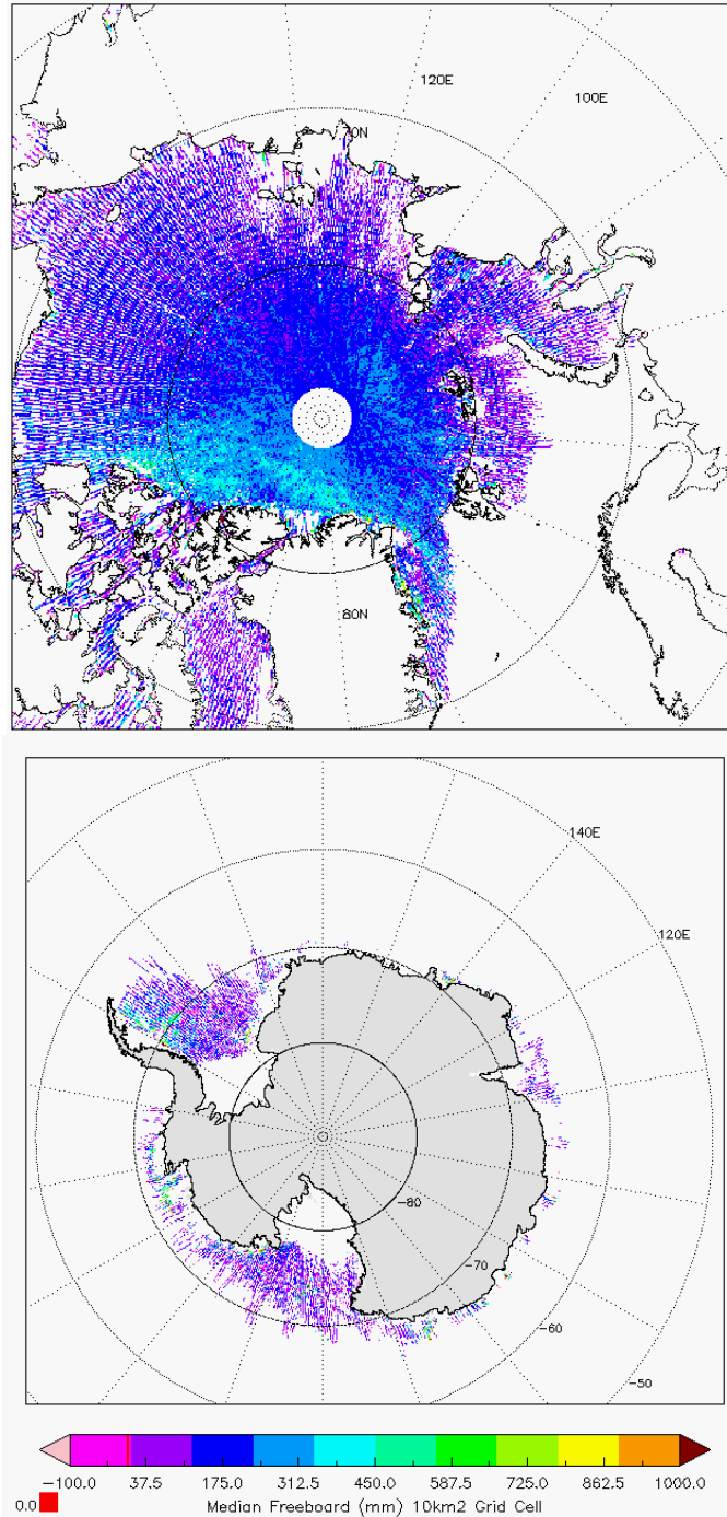
Figure 7 - Polar plots of 10km Gridded Freeboard values from L2 SAR products in cycle #116.
