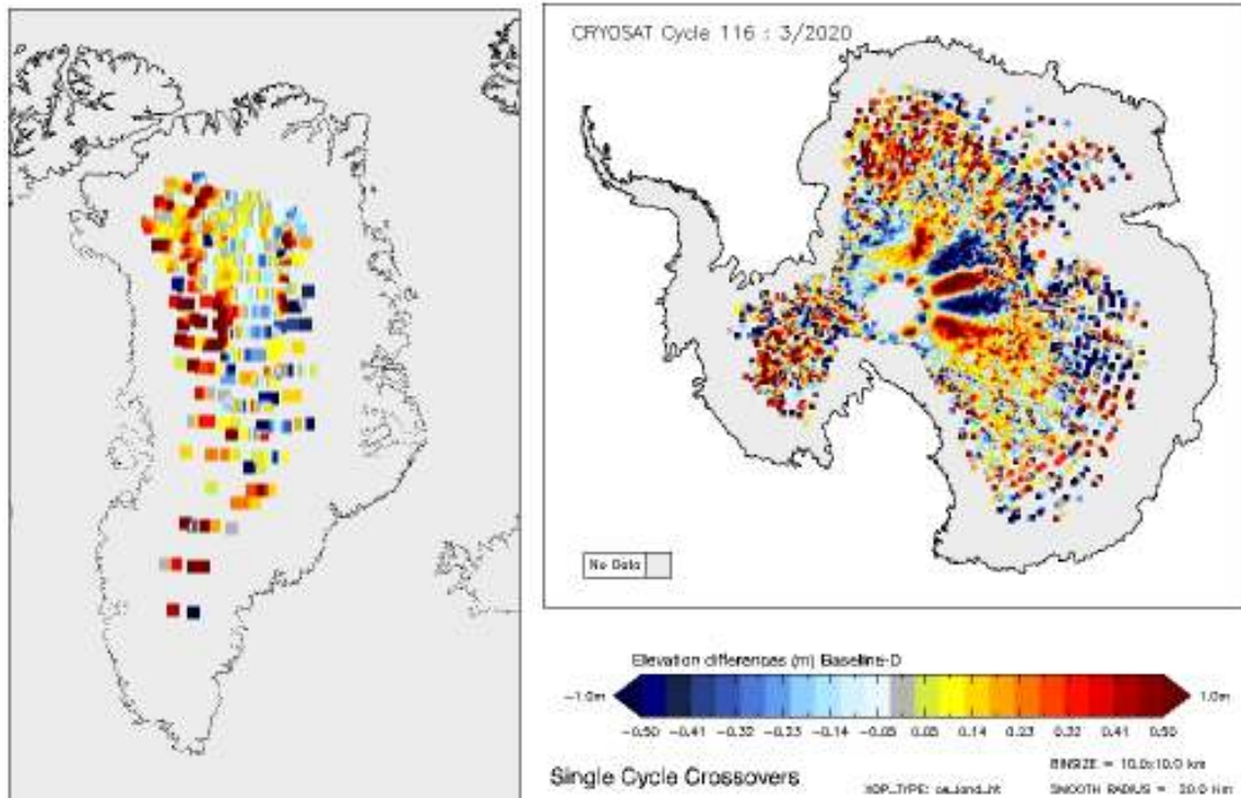
Figure 15 - Greenland and Antarctica maps of LRM elevation differences for cycle #116.
