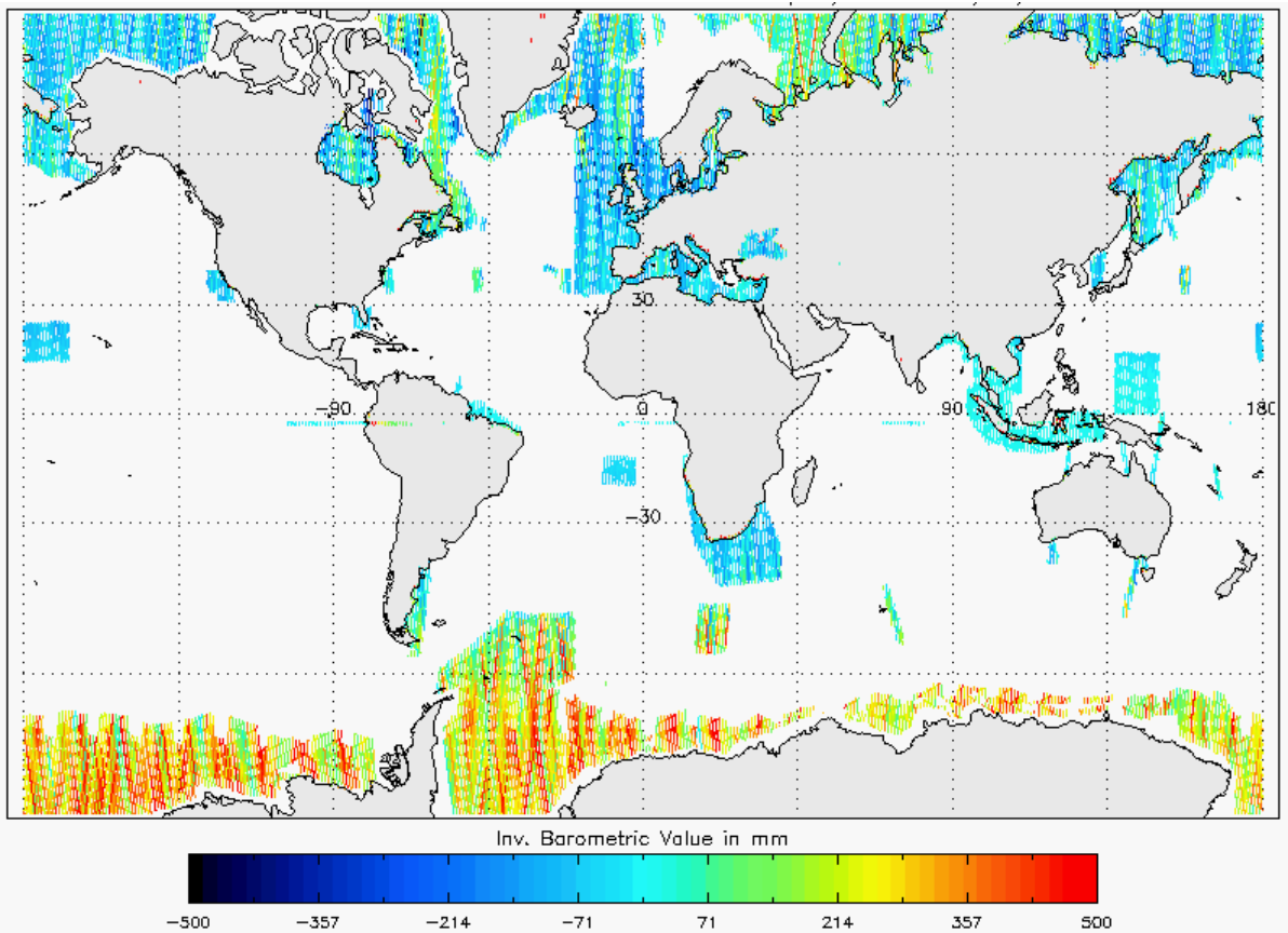
Figure 21 - Global plot of Inverse Barometric Correction for cycle #116
