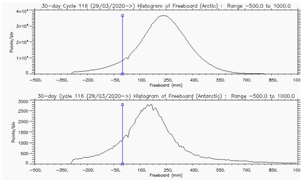
Figure 6 – Histogram of Freeboard for Arctic (above) and Antarctic (below) for cycle #116
