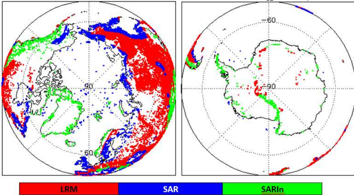
Figure 2 - Polar plots showing areas of loss of track in all SIRAL modes L0 data during April 2020.
