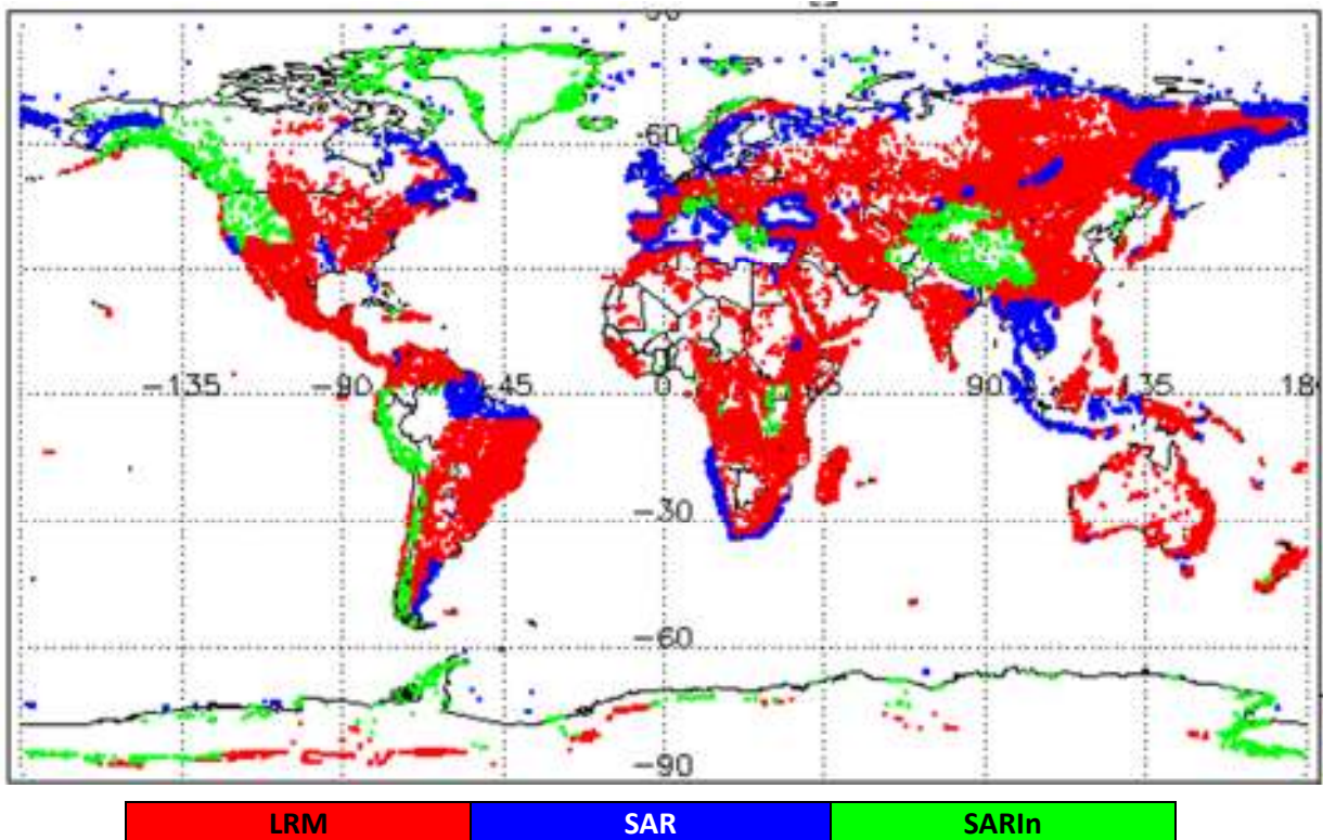
Figure 1 - Global plot showing areas of loss of track in all SIRAL modes L0 data during April 2020.
