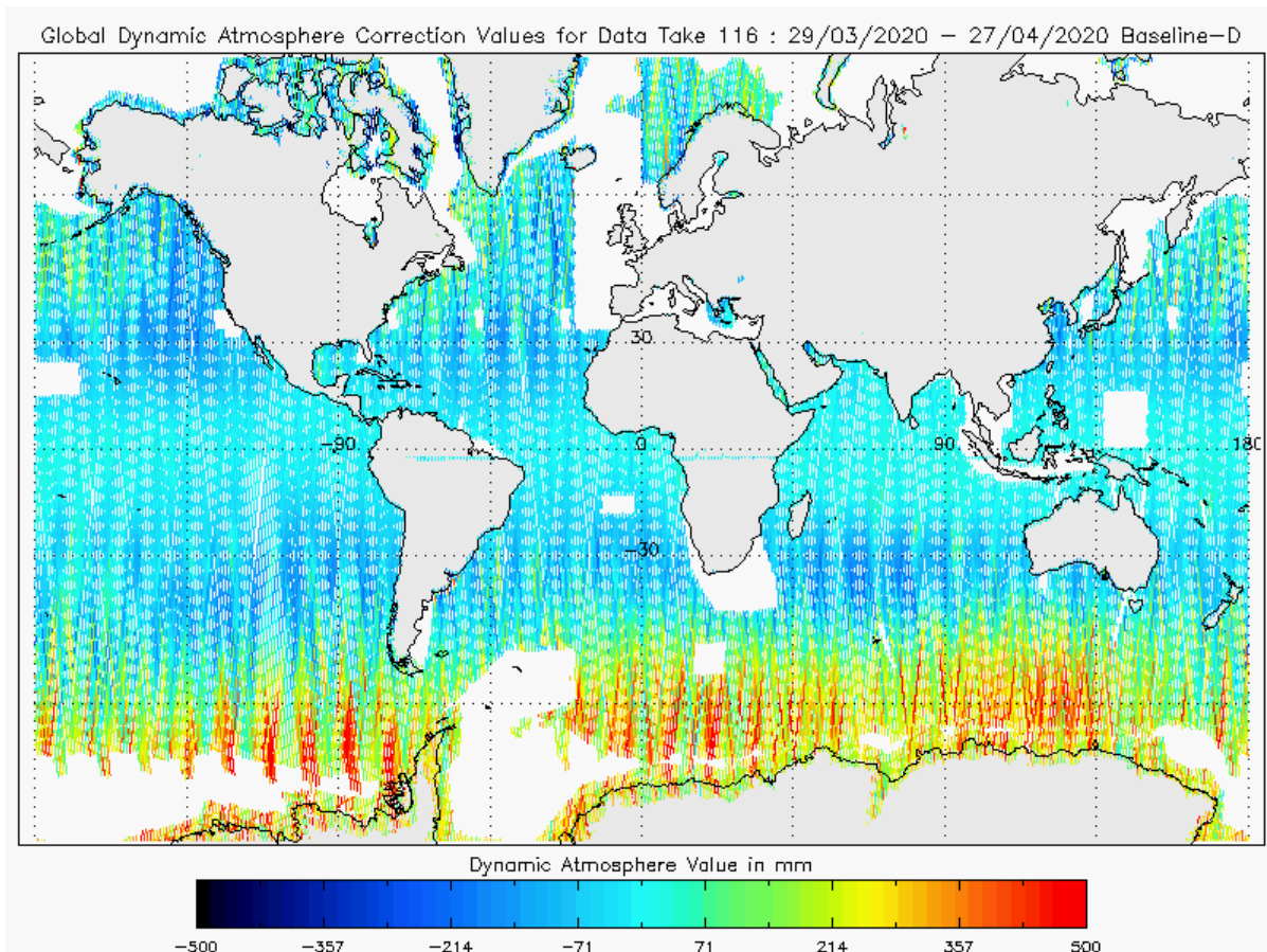
Figure 23 - Global plot of Dynamic Atmospheric Correction for cycle #116
