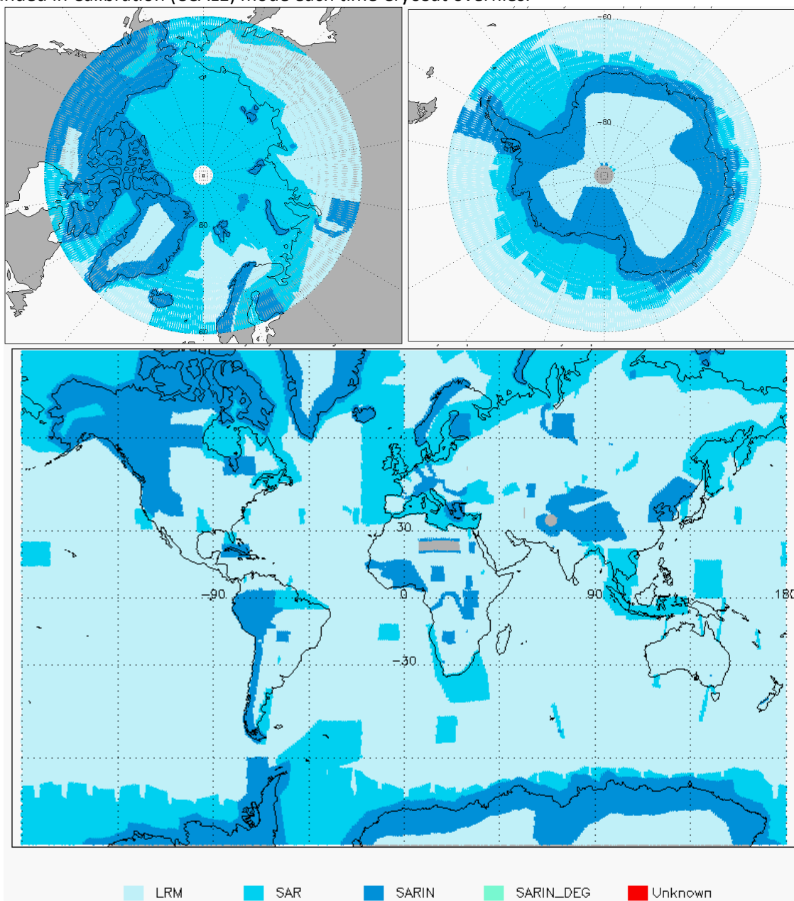
Figure 3 - Global and Polar plots of SIRAL Modes for cycle #116.
