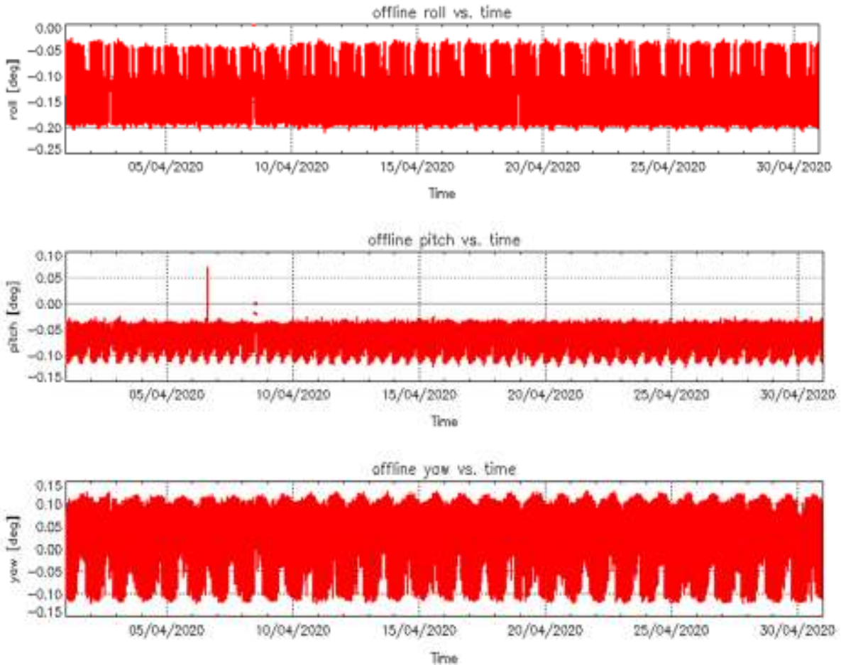
Figure 4 – Roll (top), Pitch (middle) and Yaw (bottom) values for L1B Products during cycle #116.
