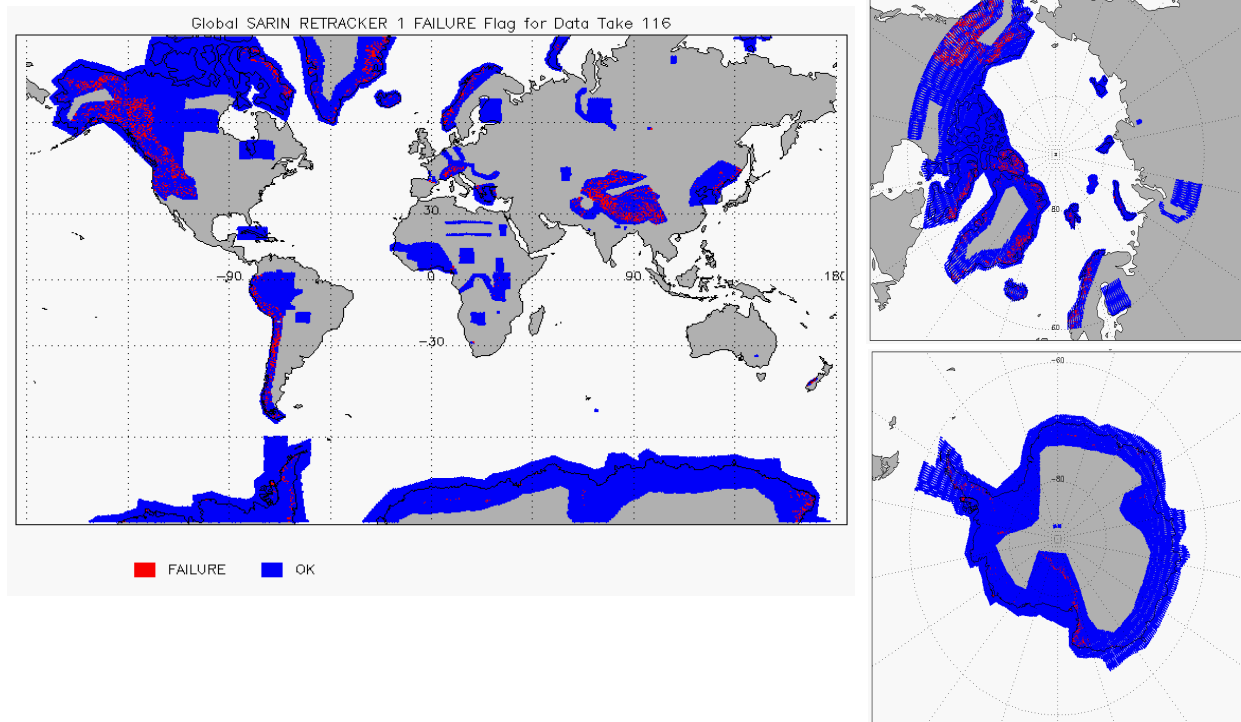
Figure 12 – Global plots showing Retracker Failure Flags for SARIn mode for cycle #116
