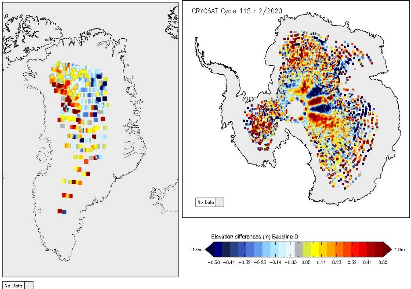
Figure 14 - Greenland and Antarctica maps of LRM elevation differences for cycle #115.
