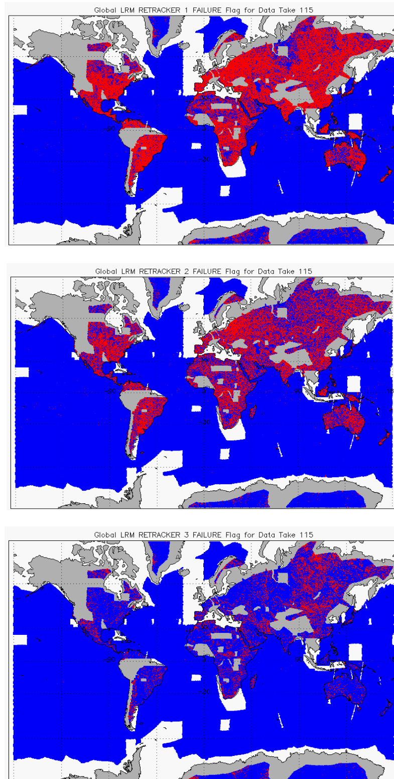
Figure 9 – Global plots showing Retracker Failure Flags for LRM mode for cycle #115: LRM CFI (top), LRM LIRT (middle), LRM OCOG (bottom)
