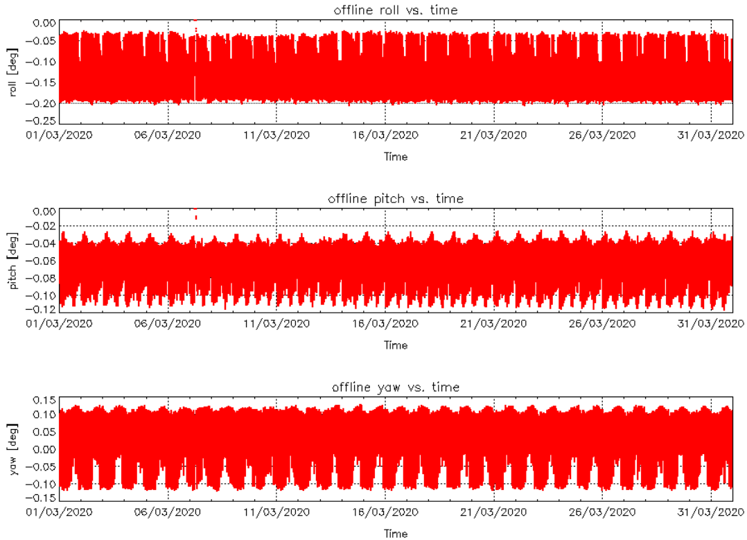
Figure 4 – Roll (top), Pitch (middle) and Yaw (bottom) values for L1B Products during cycle #115.
