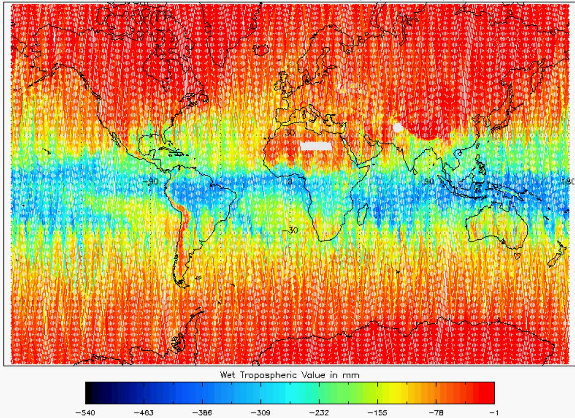
Figure 18 - Global plot of Wet Tropospheric Correction for cycle #115
