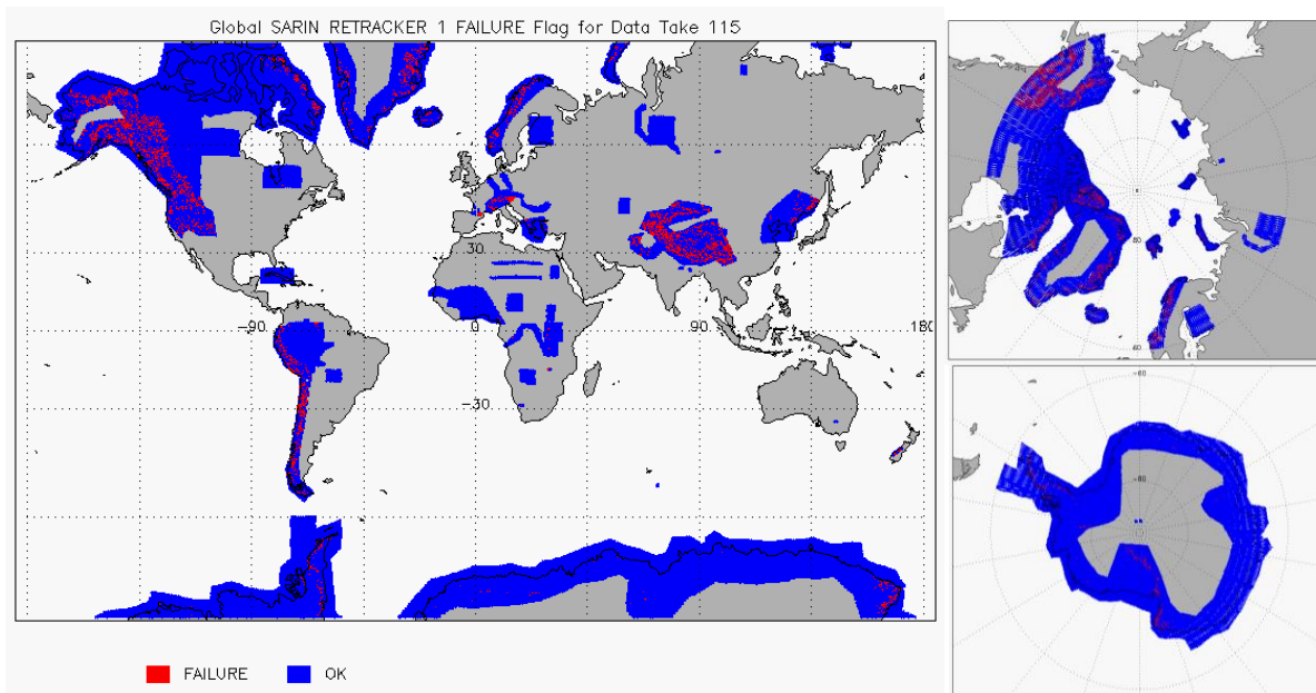
Figure 11 – Global plots showing Retracker Failure Flags for SARIn mode for cycle #115
