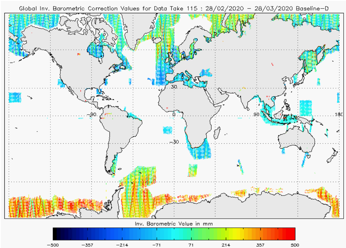
Figure 20 shows, geographically, the value of the Inverse Barometric Correction, applied to the L2 data during cycle #115 and Figure 21 shows the trends in r.m.s values since the beginning of the mission.
