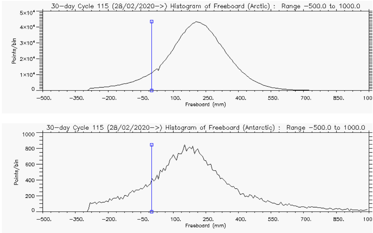
Figure 5 – Histogram of Freeboard for Arctic (above) and Antarctic (below) for cycle #115
