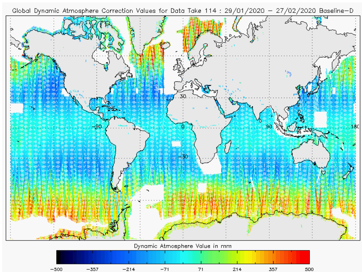
Figure 23 - Global plot of Dynamic Atmospheric Correction for cycle #114
