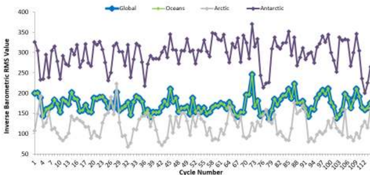
Figure 22 – Inverse Barometric Correction RMS value trend from beginning of mission
