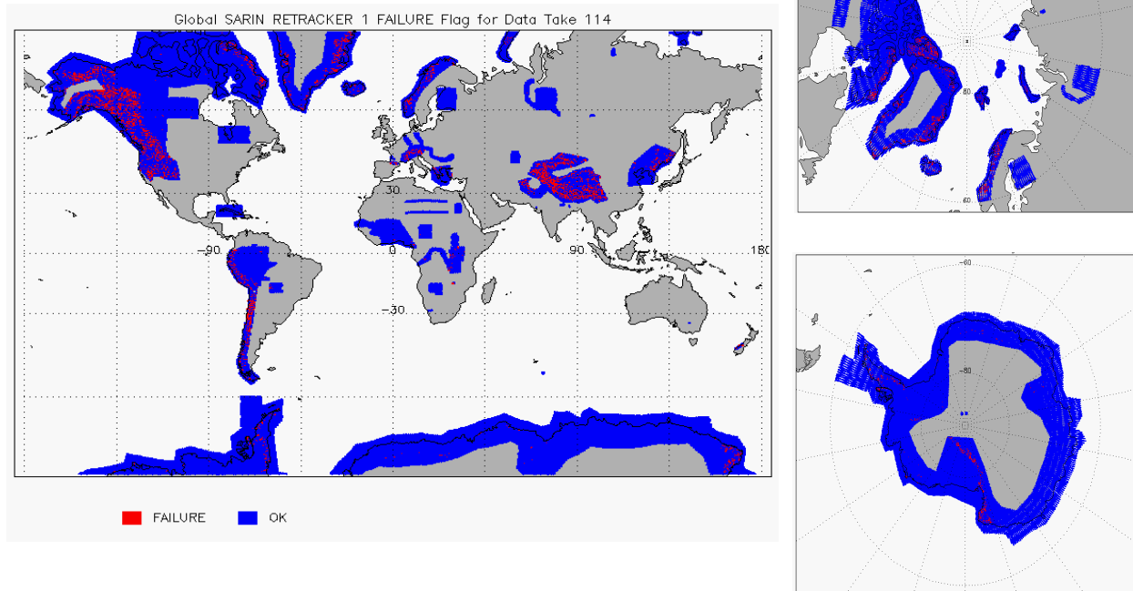
Figure 12 – Global plots showing Retracker Failure Flags for SARIn mode for cycle #114
