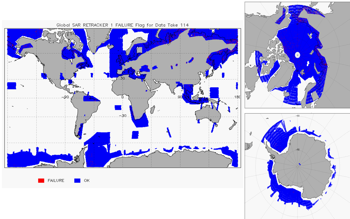
Figure 11 – Global plots showing Retracker Failure Flags for SAR mode for cycle #114
