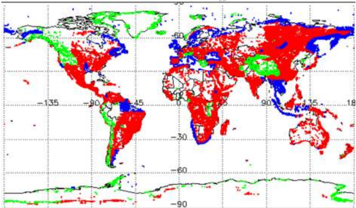
Figure 1 - Global plot showing areas of loss of track in all SIRAL modes L0 data during February 2020.
