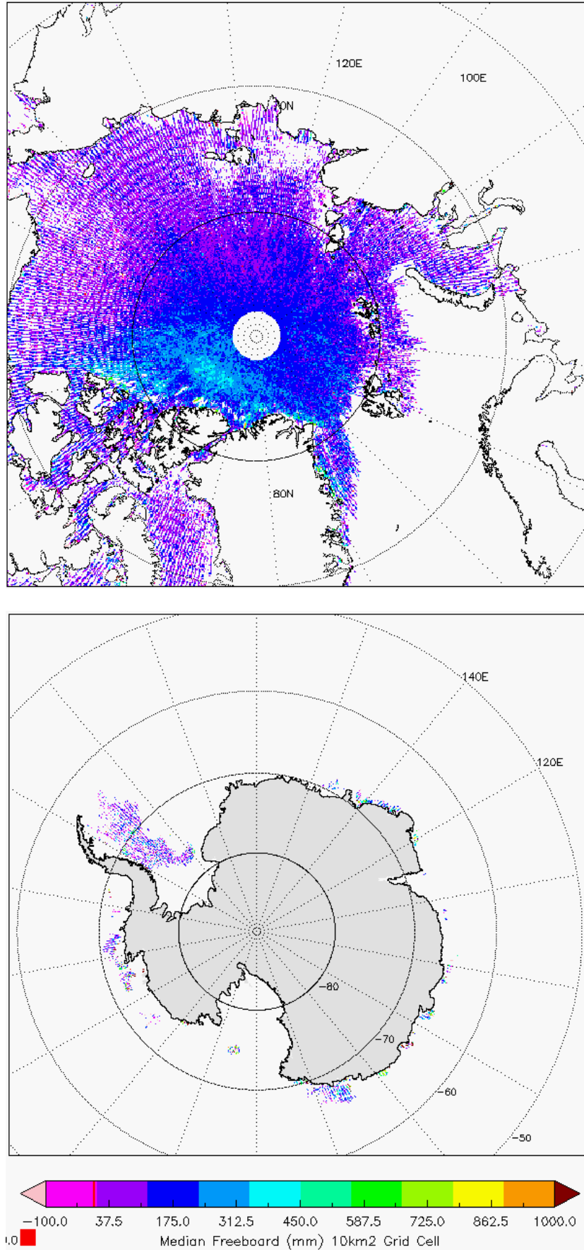
Figure 7 - Polar plots of 10km Gridded Freeboard values from L2 SAR products in cycle #114.
