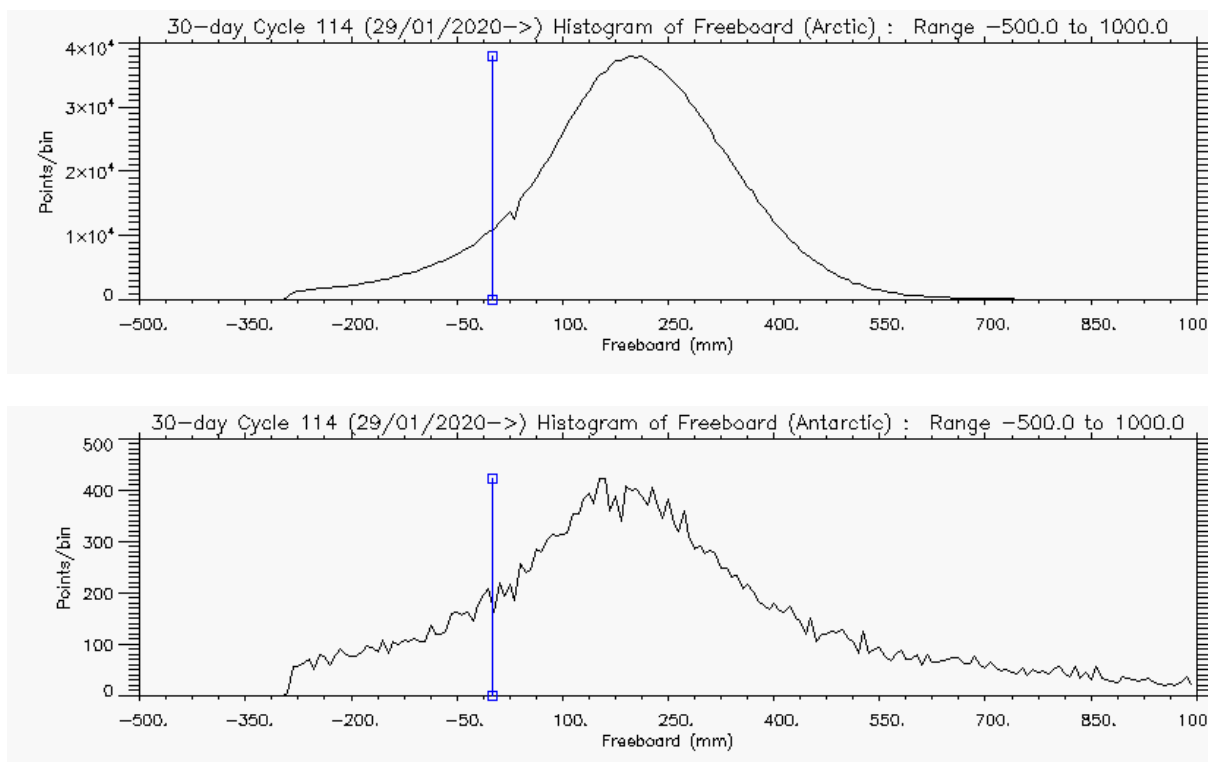
Figure 6 – Histogram of Freeboard for Arctic (above) and Antarctic (below) for cycle #114
