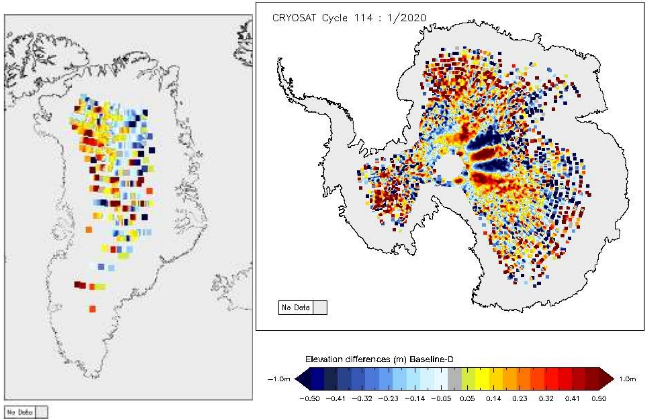
Figure 15 - Greenland and Antarctica maps of LRM elevation differences for cycle #114.
