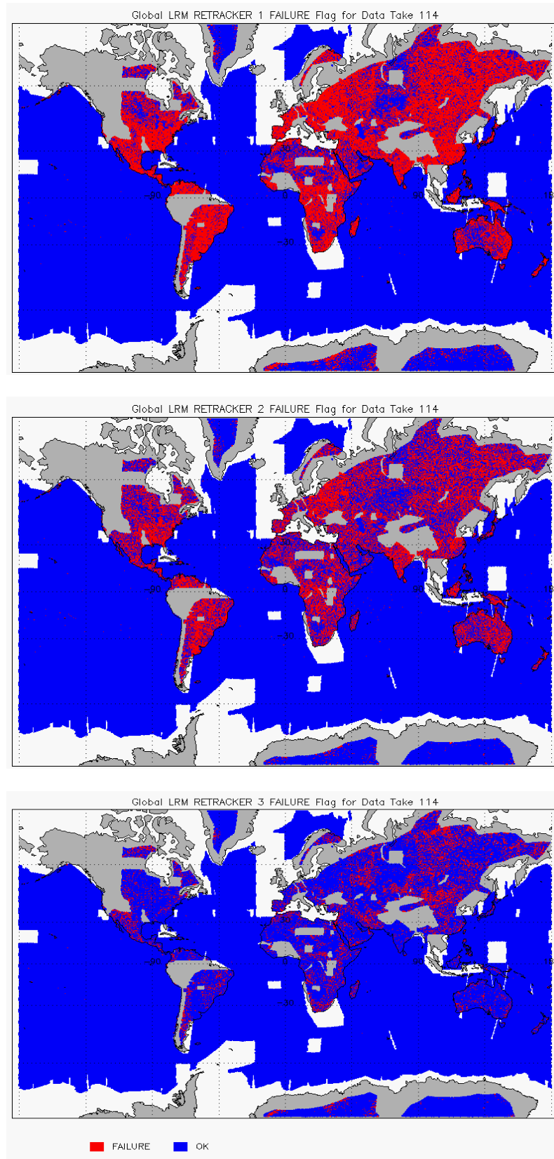
Figure 10 – Global plots showing Retracker Failure Flags for LRM mode for cycle #114: LRM CFI (top), LRM LIRT (middle), LRM OCOG (bottom)
