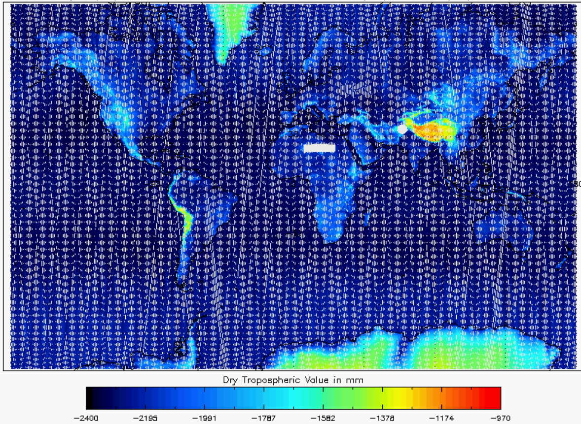
Figure 17 - Global plot of Dry Tropospheric Correction for cycle #114
