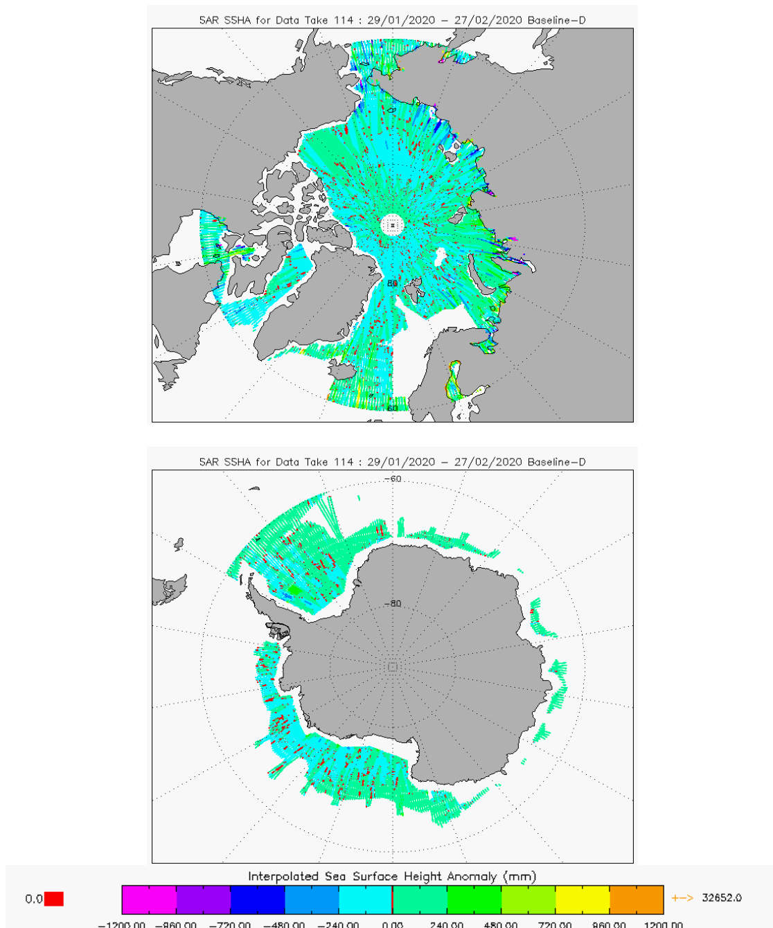
Figure 8 –Polar plots of SSHA for cycle #114.
