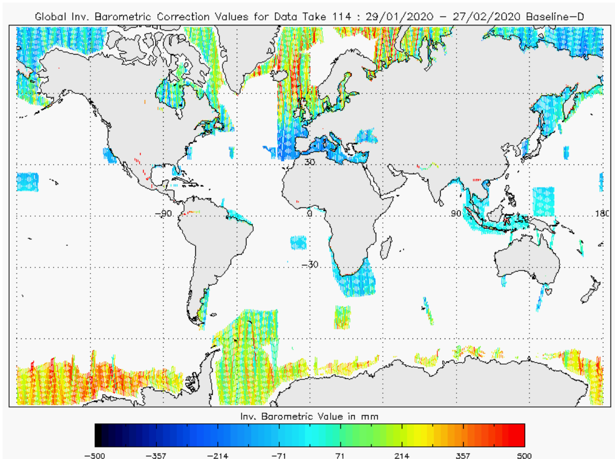
Figure 21 - Global plot of Inverse Barometric Correction for cycle #114
