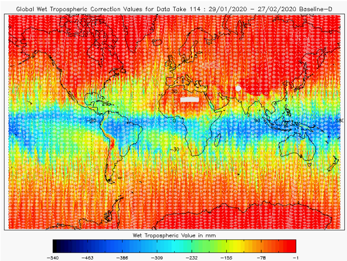
Figure 19 - Global plot of Wet Tropospheric Correction for cycle #114
