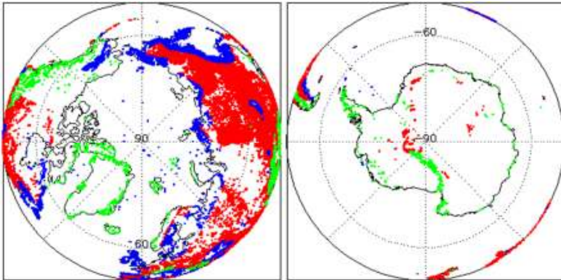
Figure 2 - Polar plots showing areas of loss of track in all SIRAL modes L0 data during February 2020.
