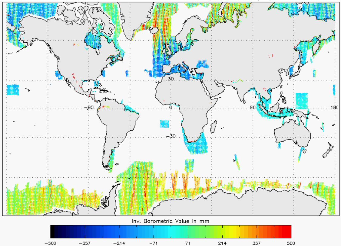
Figure 20 - Global plot of Inverse Barometric Correction for cycle #113
