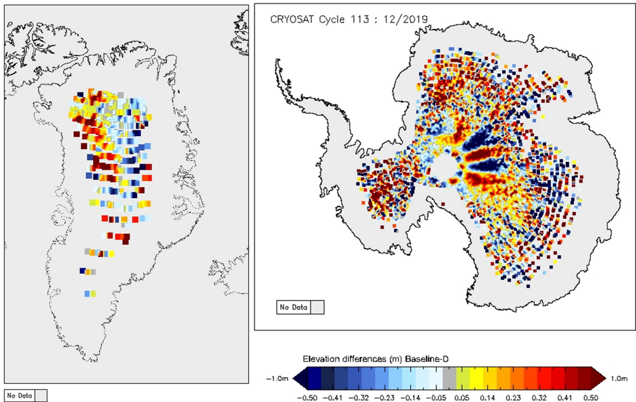
Figure 14 - Greenland and Antarctica maps of LRM elevation differences for cycle #113.
