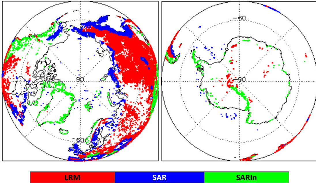
Figure 2 - Polar plots showing areas of loss of track in all SIRAL modes L0 data during January 2020.
