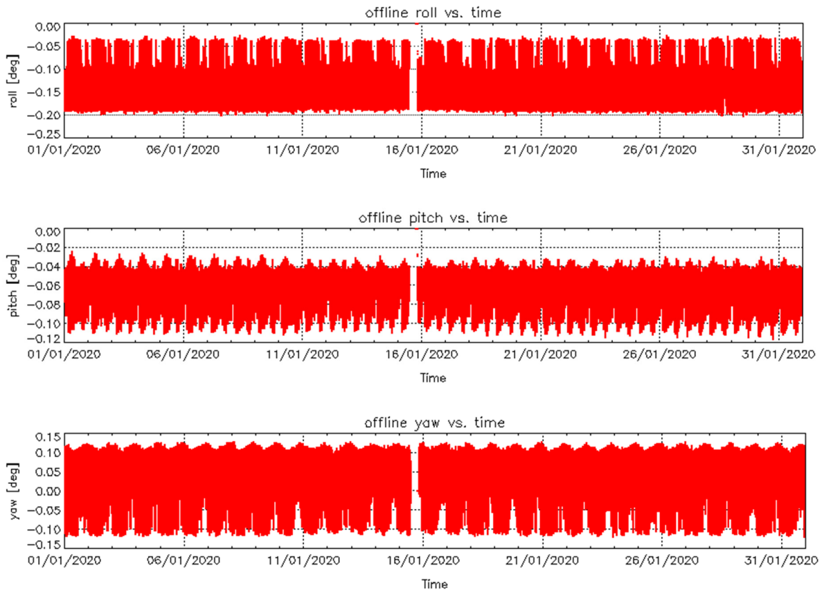
Figure 4 – Roll (top), Pitch (middle) and Yaw (bottom) values for L1B Products during cycle #113.
