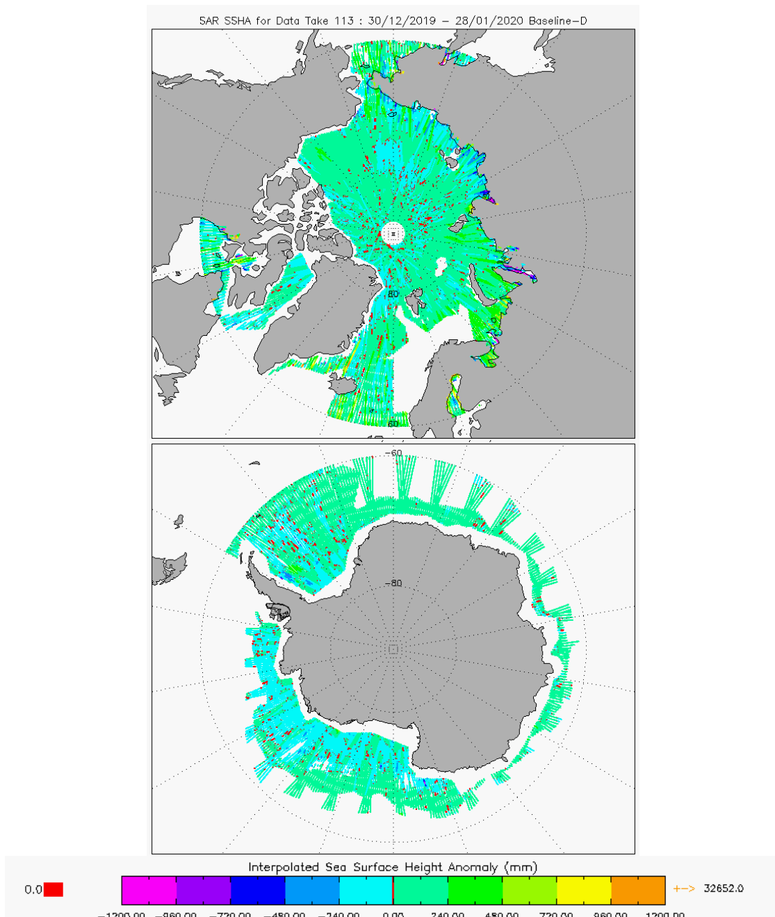
Figure 7 –Polar plots of SSHA for cycle #113.
