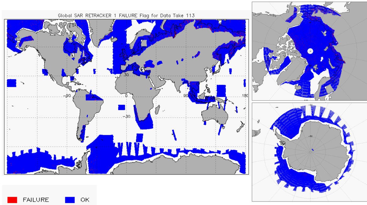
Figure 10 – Global plots showing Retracker Failure Flags for SAR mode for cycle #113
