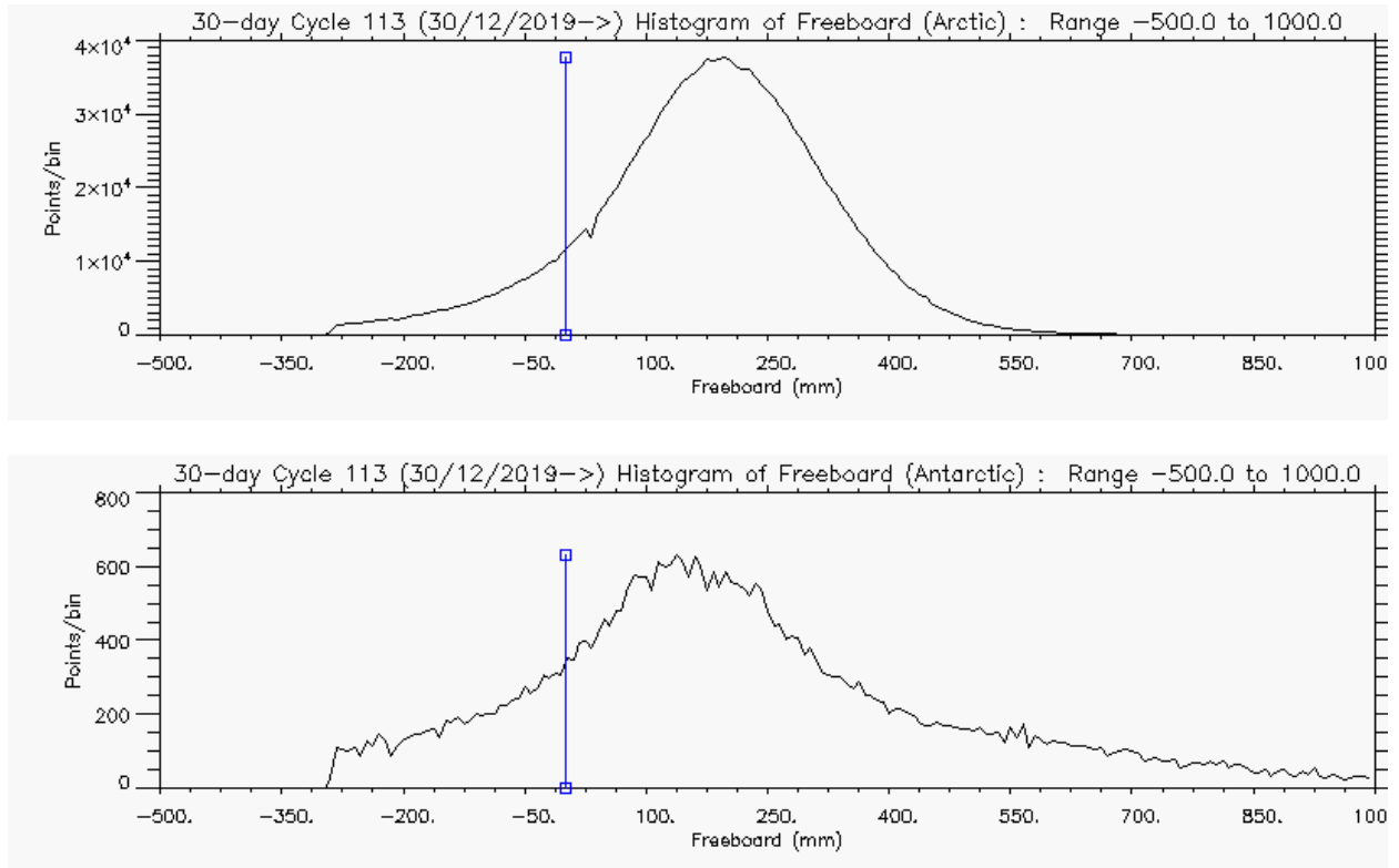
Figure 5 – Histogram of Freeboard for Arctic (above) and Antarctic (below) for cycle #113
