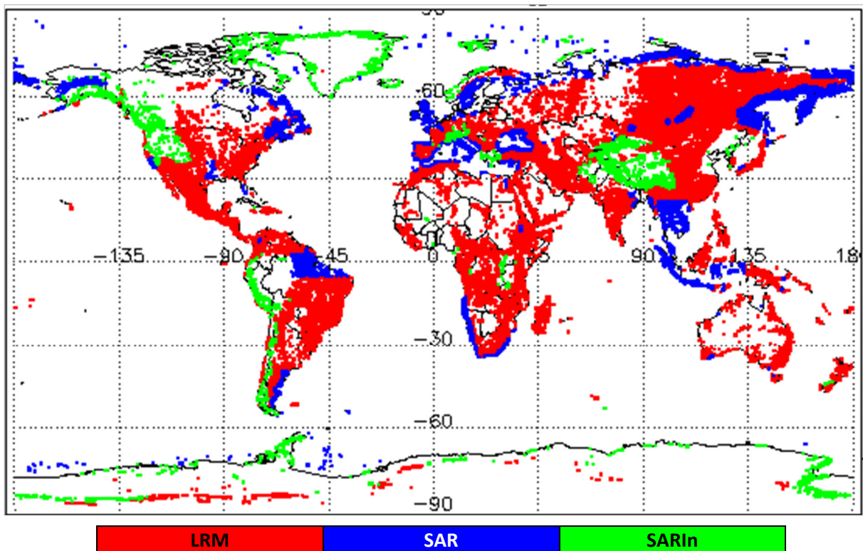
Figure 1 - Global plot showing areas of loss of track in all SIRAL modes L0 data during January 2020.
