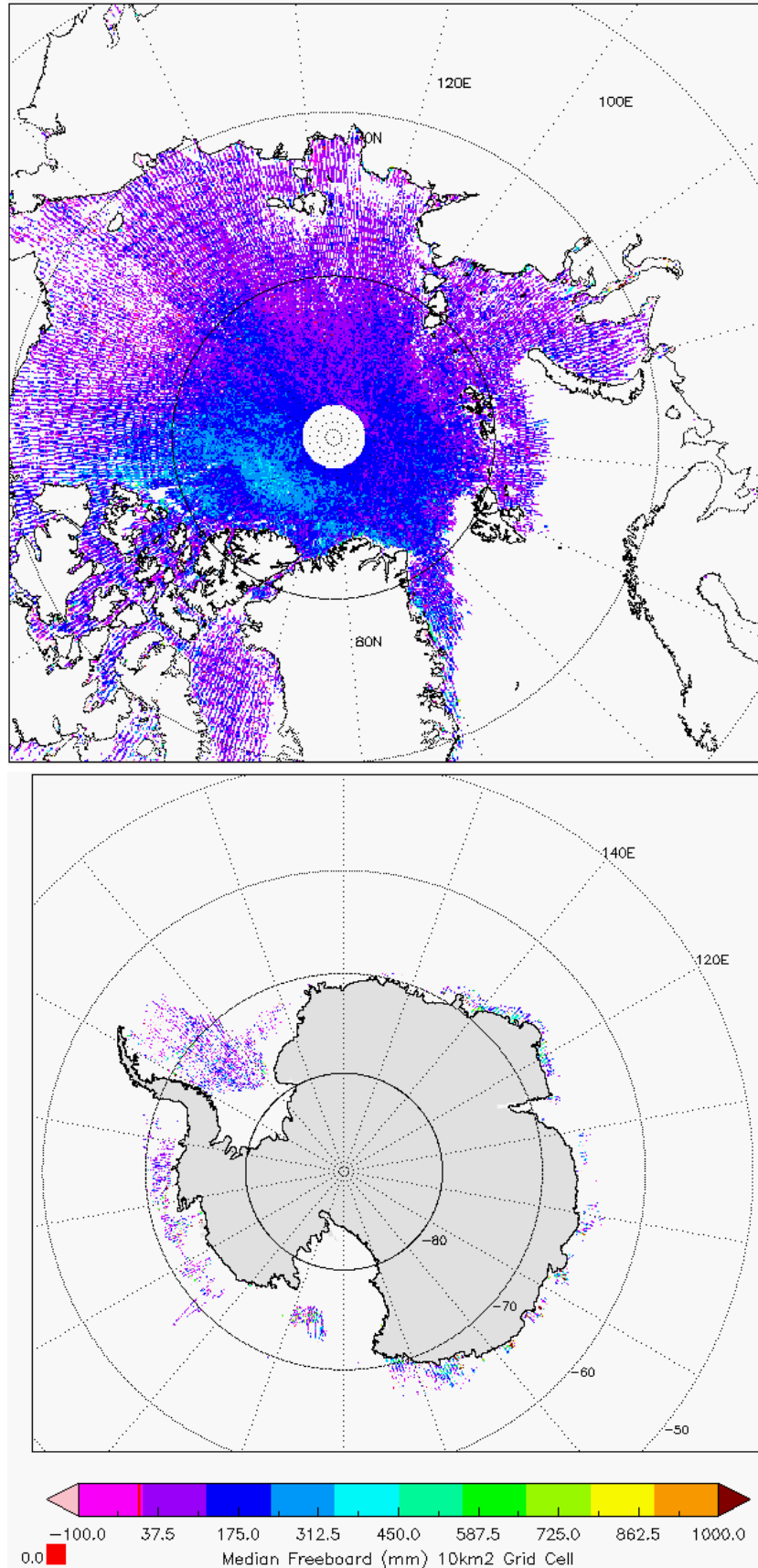
Figure 6 - Polar plots of 10km Gridded Freeboard values from L2 SAR products in cycle #113.
