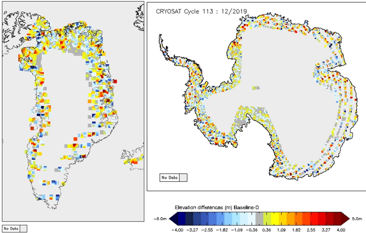
Figure 15 - Greenland and Antarctica maps of SARIn elevation differences for cycle #113
