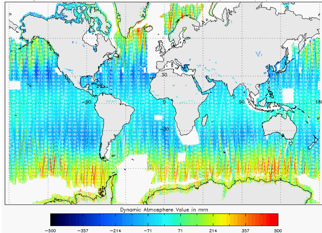
Figure 22 - Global plot of Dynamic Atmospheric Correction for cycle #113
