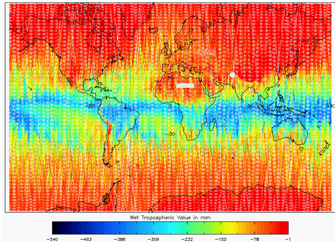
Figure 18 - Global plot of Wet Tropospheric Correction for cycle #113
