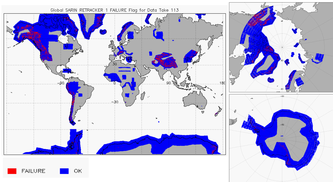
Figure 11 – Global plots showing Retracker Failure Flags for SARIn mode for cycle #113
