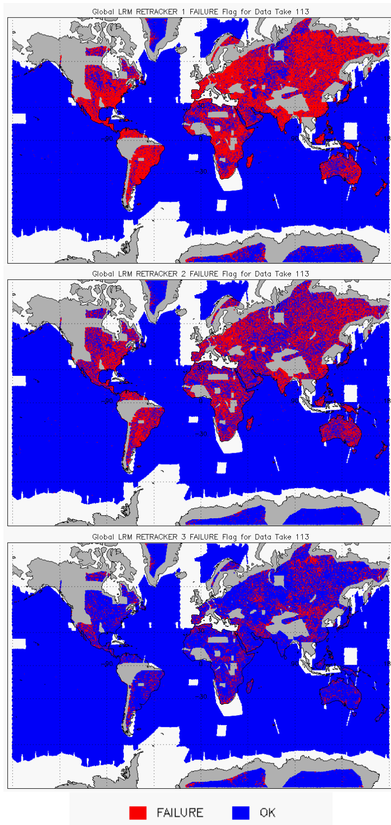
Figure 9 – Global plots showing Retracker Failure Flags for LRM mode for cycle #113: LRM CFI (top), LRM LIRT (middle), LRM OCOG (bottom)
