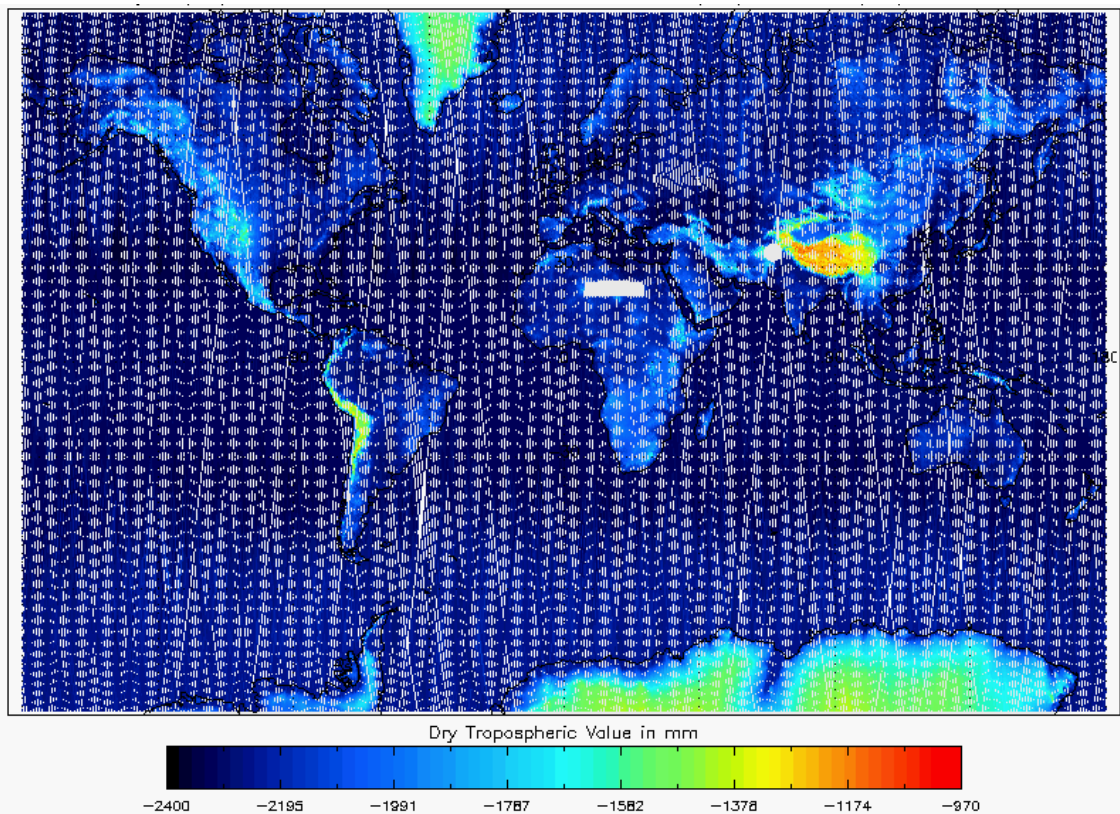
Figure 16 - Global plot of Dry Tropospheric Correction for cycle #113
