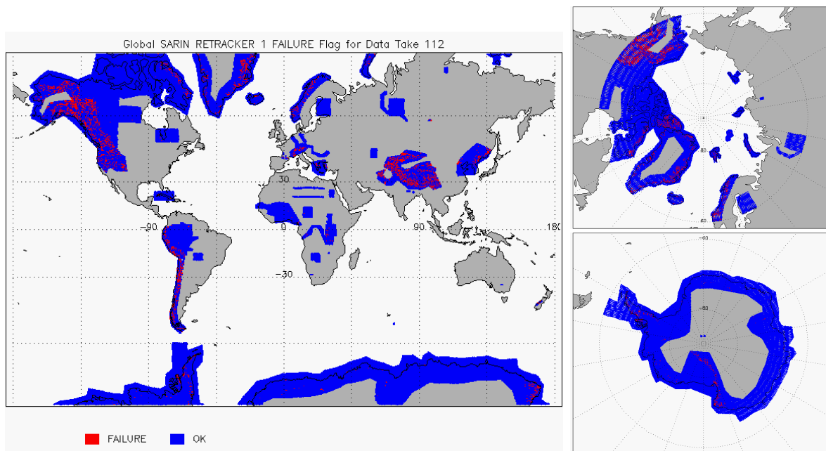
Figure 12 – Global plots showing Retracker Failure Flags for SARIn mode for cycle #112
