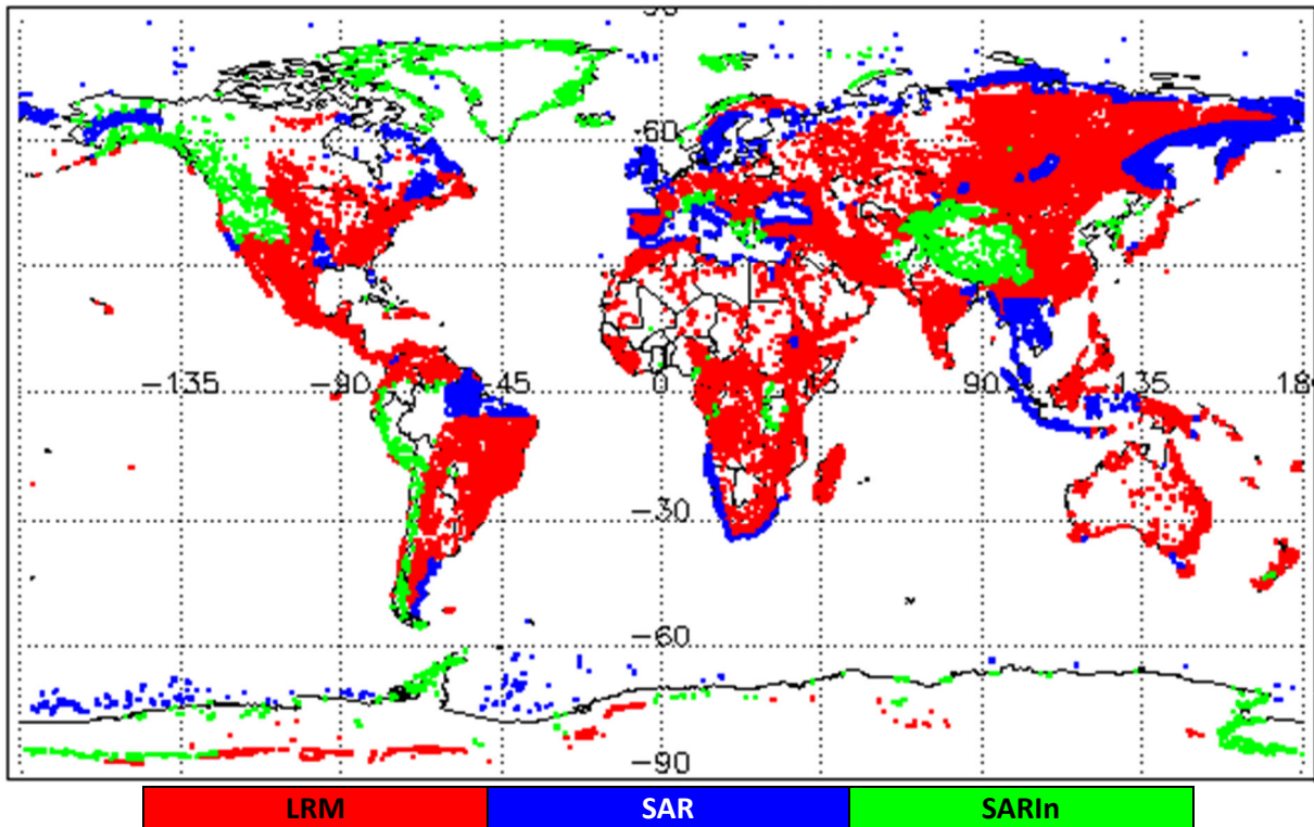
Figure 1 - Global plot showing areas of loss of track in all SIRAL modes L0 data during December 2019.
