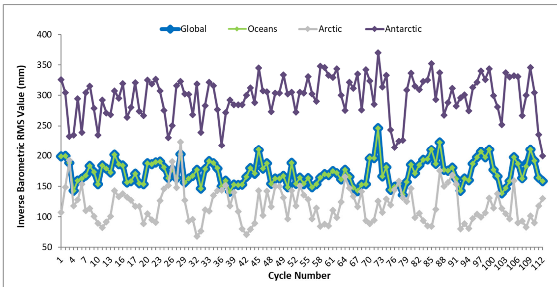
Figure 22 – Inverse Barometric Correction RMS value trend from beginning of mission
