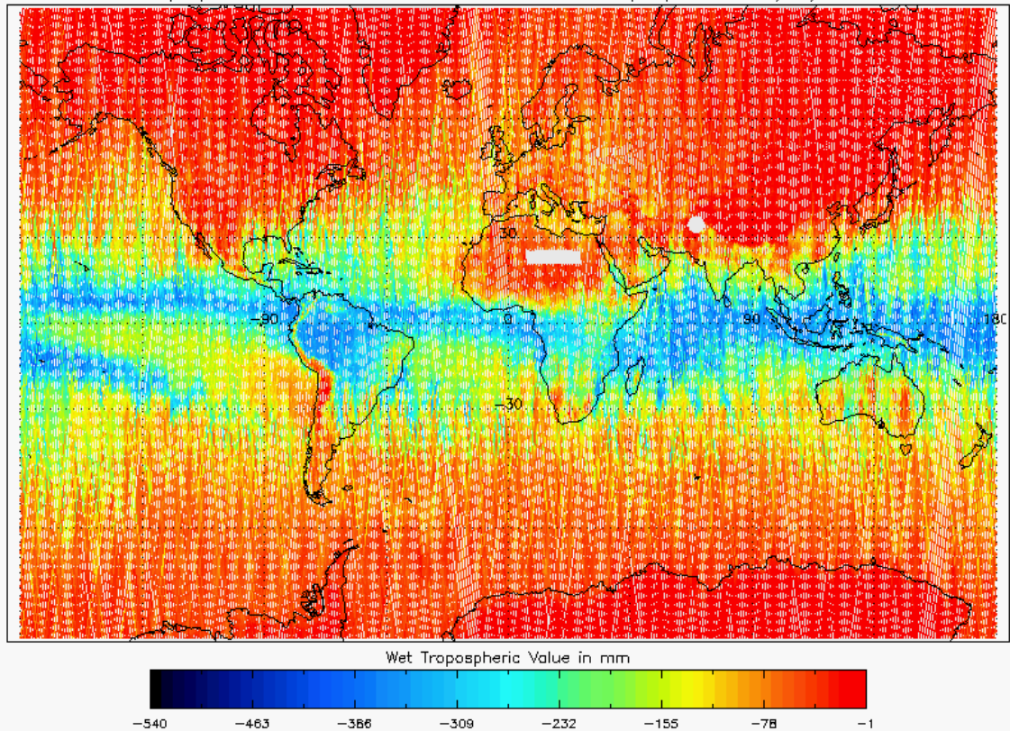
Figure 19 - Global plot of Wet Tropospheric Correction for cycle #112
