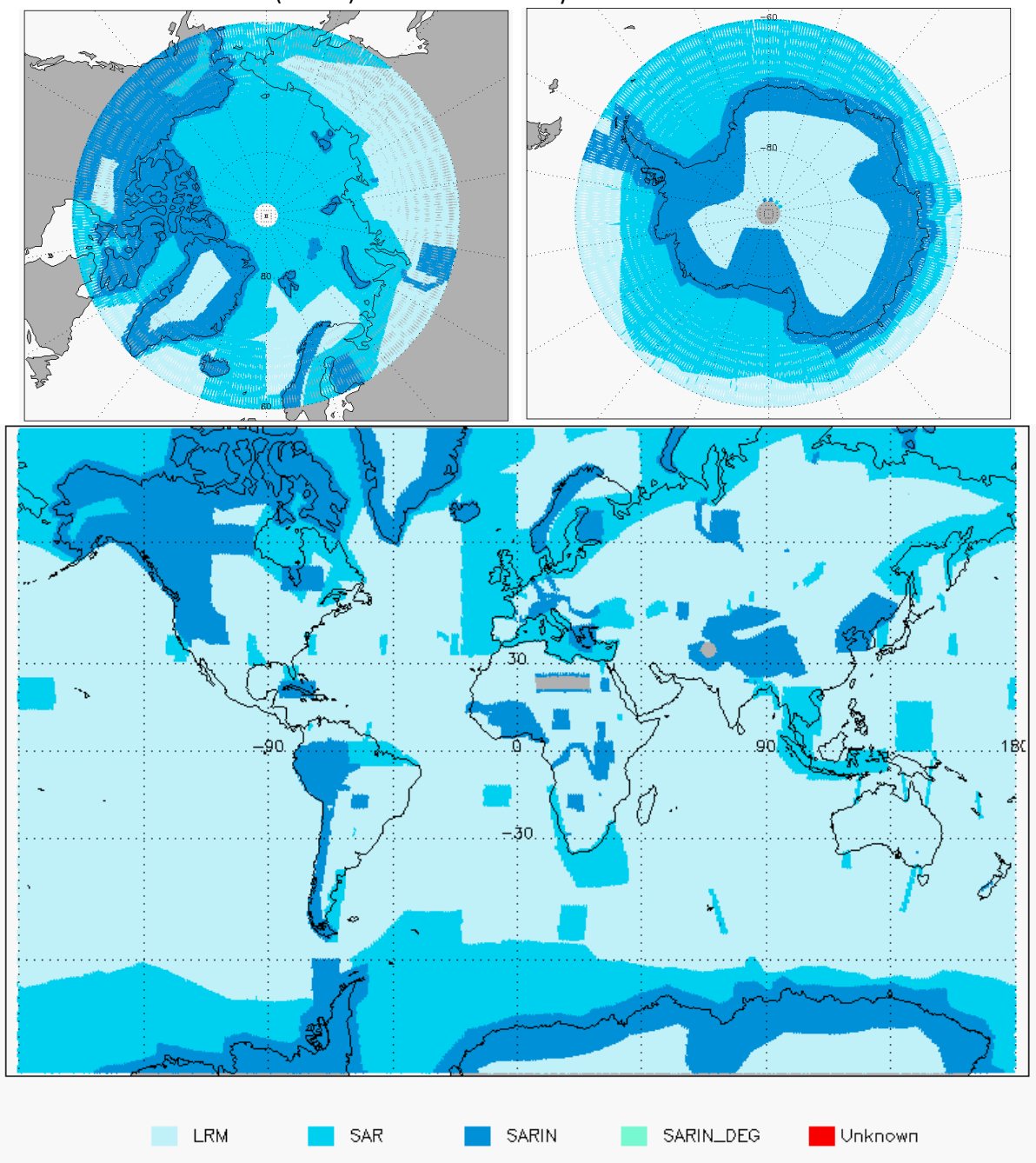
Figure 3 - Global and Polar plots of SIRAL Modes for cycle #112.
