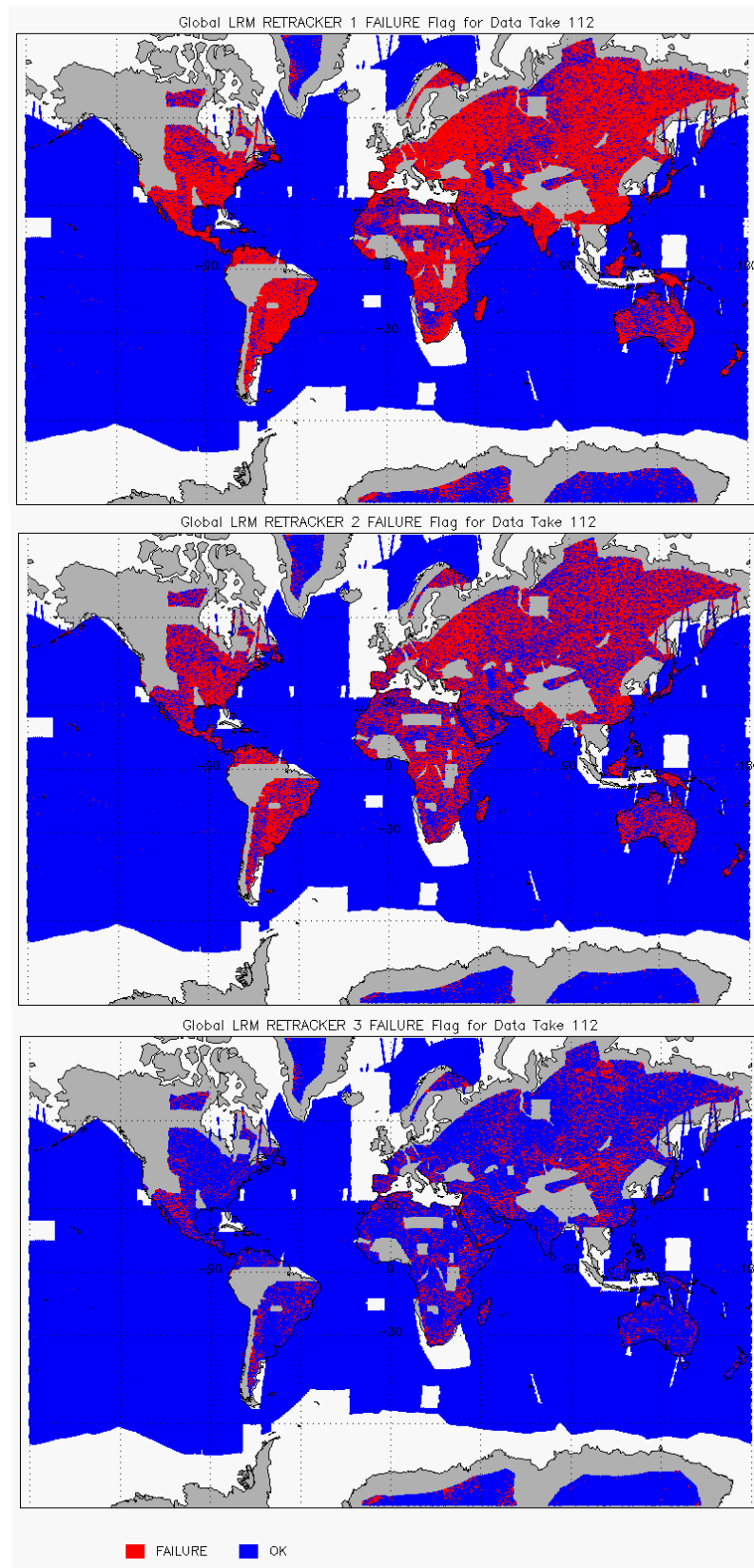
Figure 10 – Global plots showing Retracker Failure Flags for LRM mode for cycle #112: LRM CFI (top), LRM LIRT (middle), LRM OCOG (bottom)
