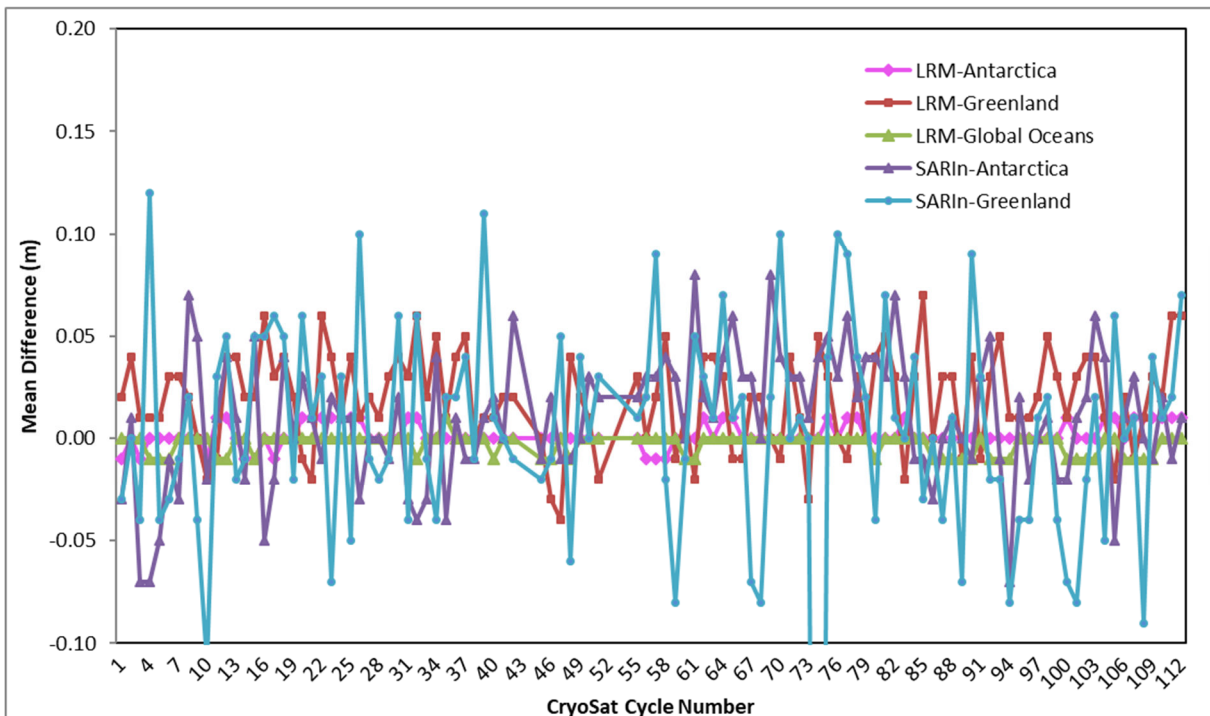
Figure 14 - Time series for Mean Difference in elevation at crossovers from beginning of the mission.
