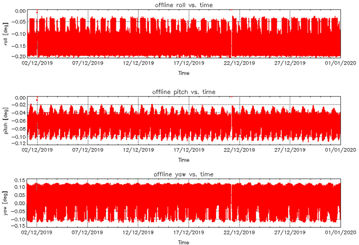
Figure 4 – Roll (top), Pitch (middle) and Yaw (bottom) values for L1B Products during cycle #112.
