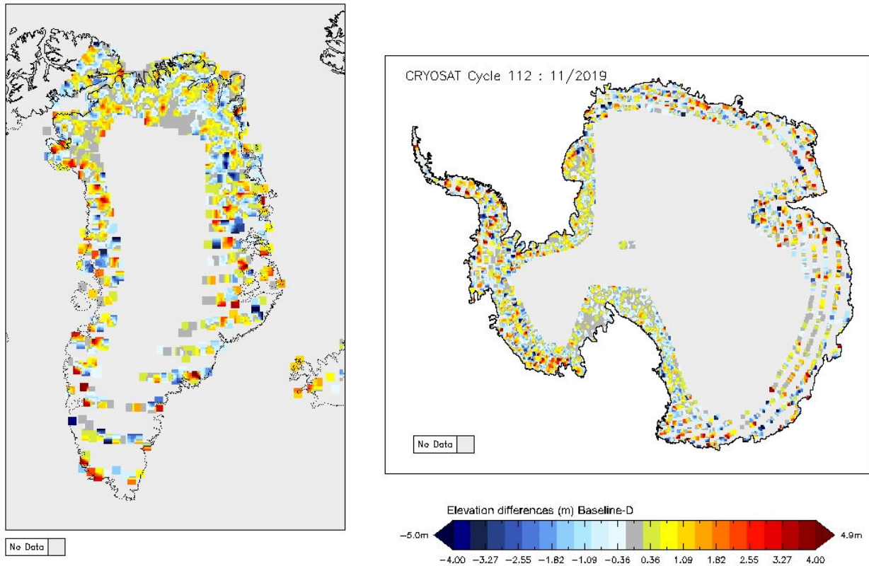
Figure 16 - Greenland and Antarctica maps of SARIn elevation differences for cycle #112.
