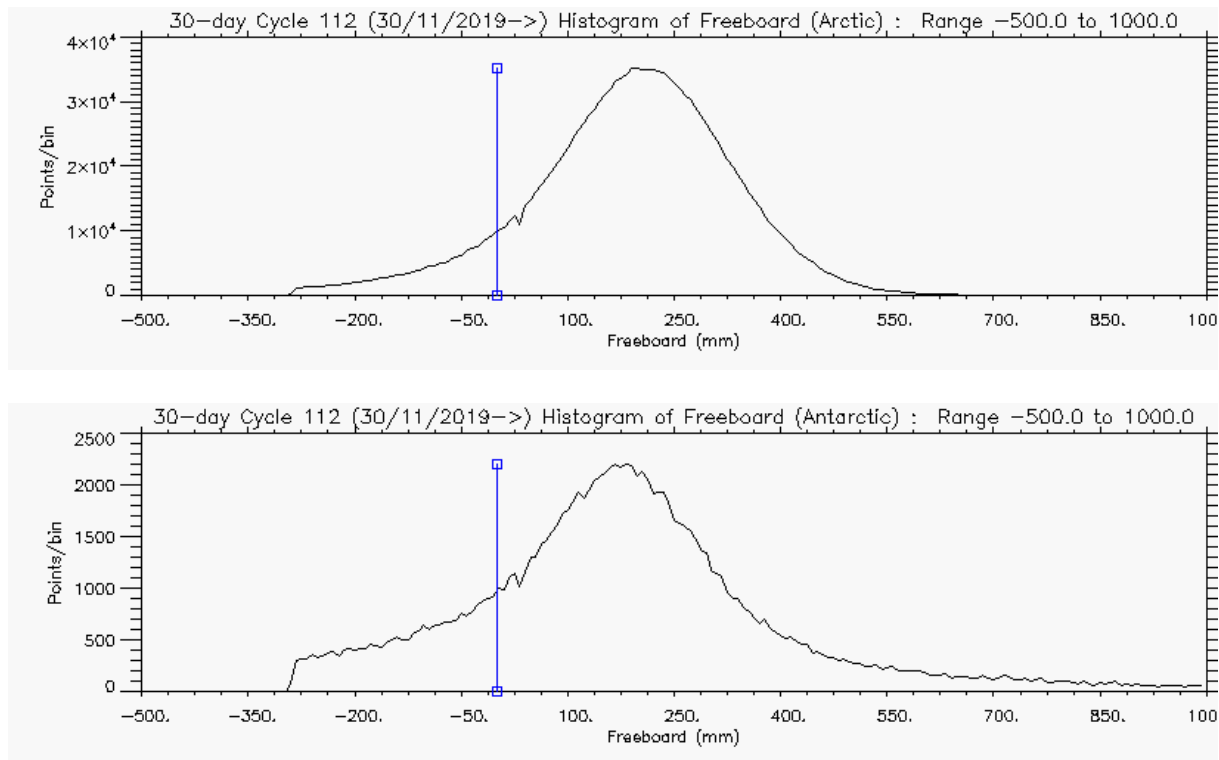
Figure 6 – Histogram of Freeboard for Arctic (above) and Antarctic (below) for cycle #112
