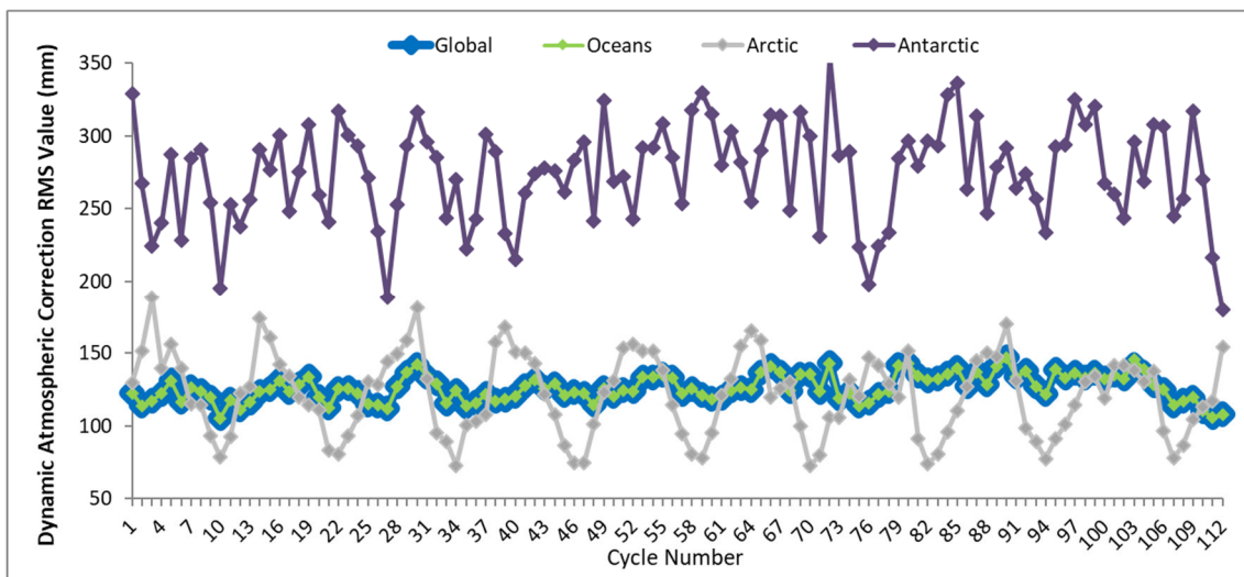
Figure 24 – Dynamic Atmospheric Correction RMS value trend from beginning of mission
