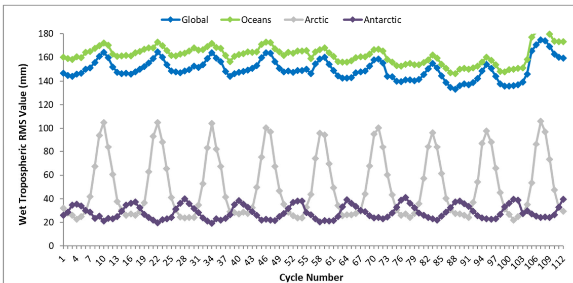
Figure 20 – Wet Tropospheric Correction RMS value trend from beginning of mission
