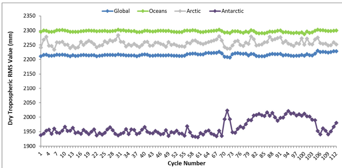
Figure 18 - Dry Tropospheric Correction RMS value trend from beginning of mission
