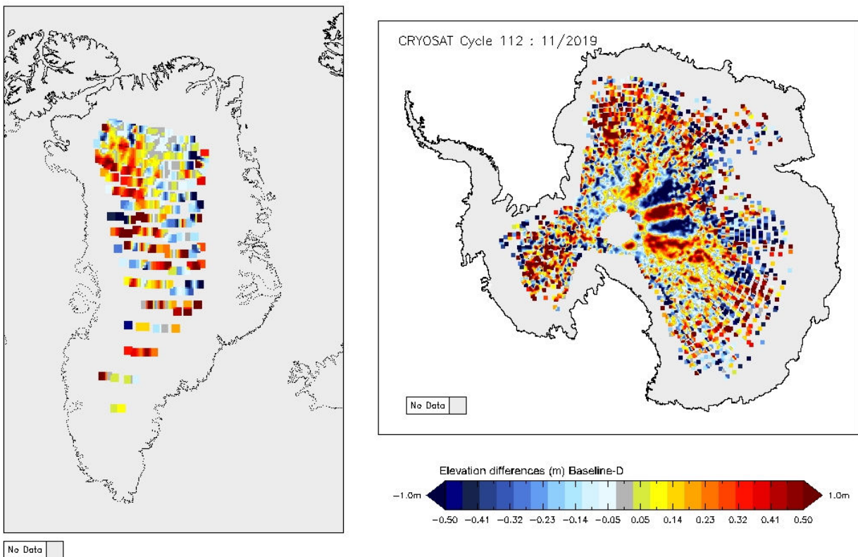
Figure 15 - Greenland and Antarctica maps of LRM elevation differences for cycle #112.
