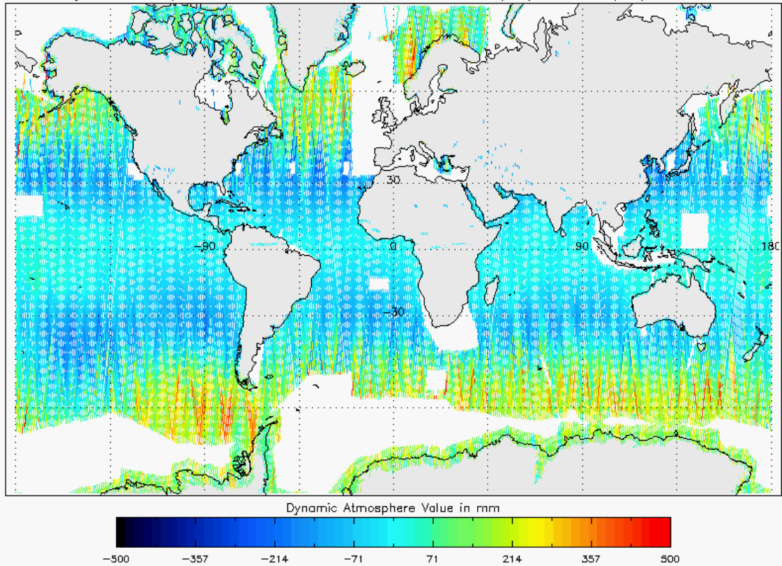
Figure 23 - Global plot of Dynamic Atmospheric Correction for cycle #112
