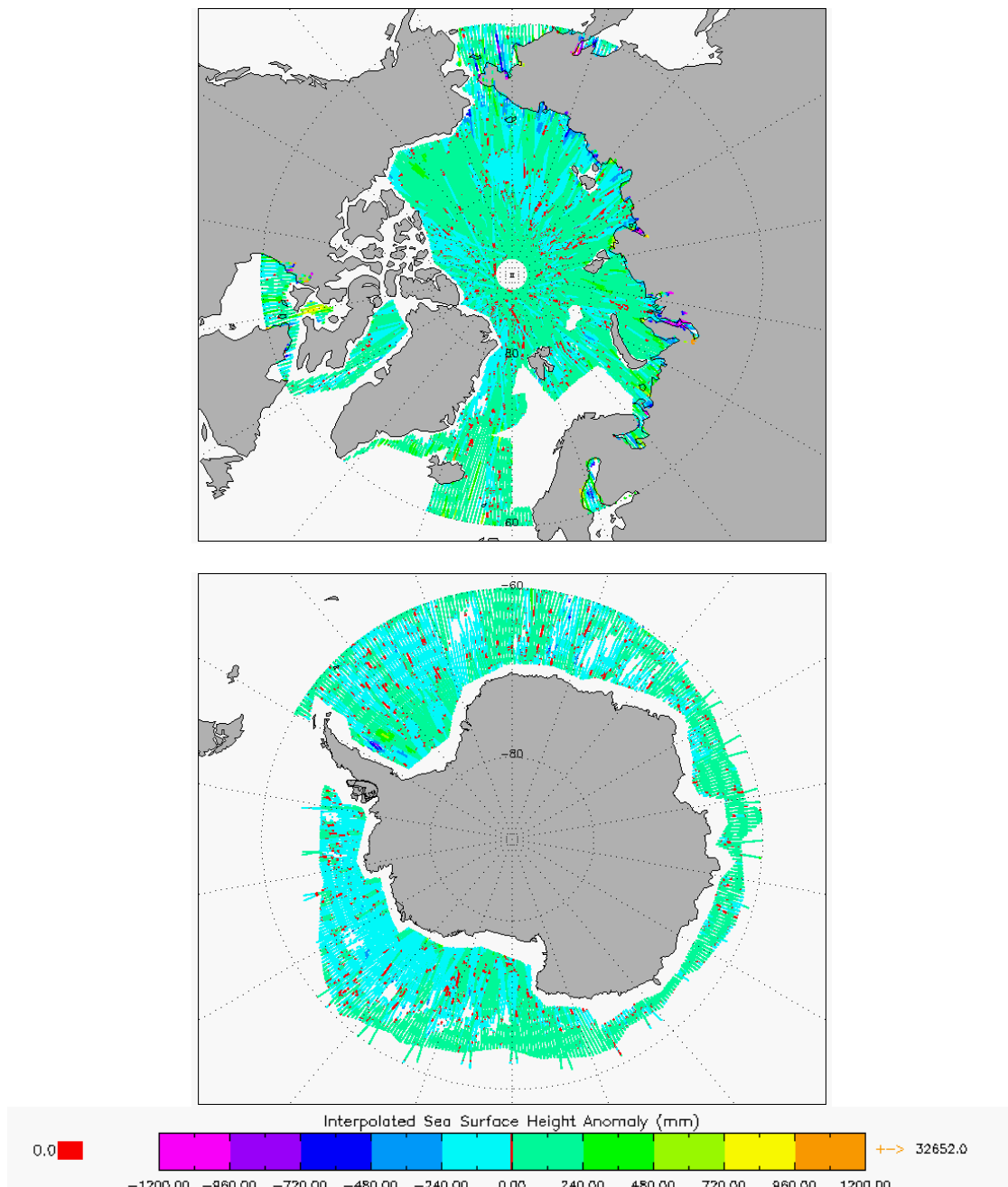
Figure 8 –Polar plots of SSHA for cycle #112.
