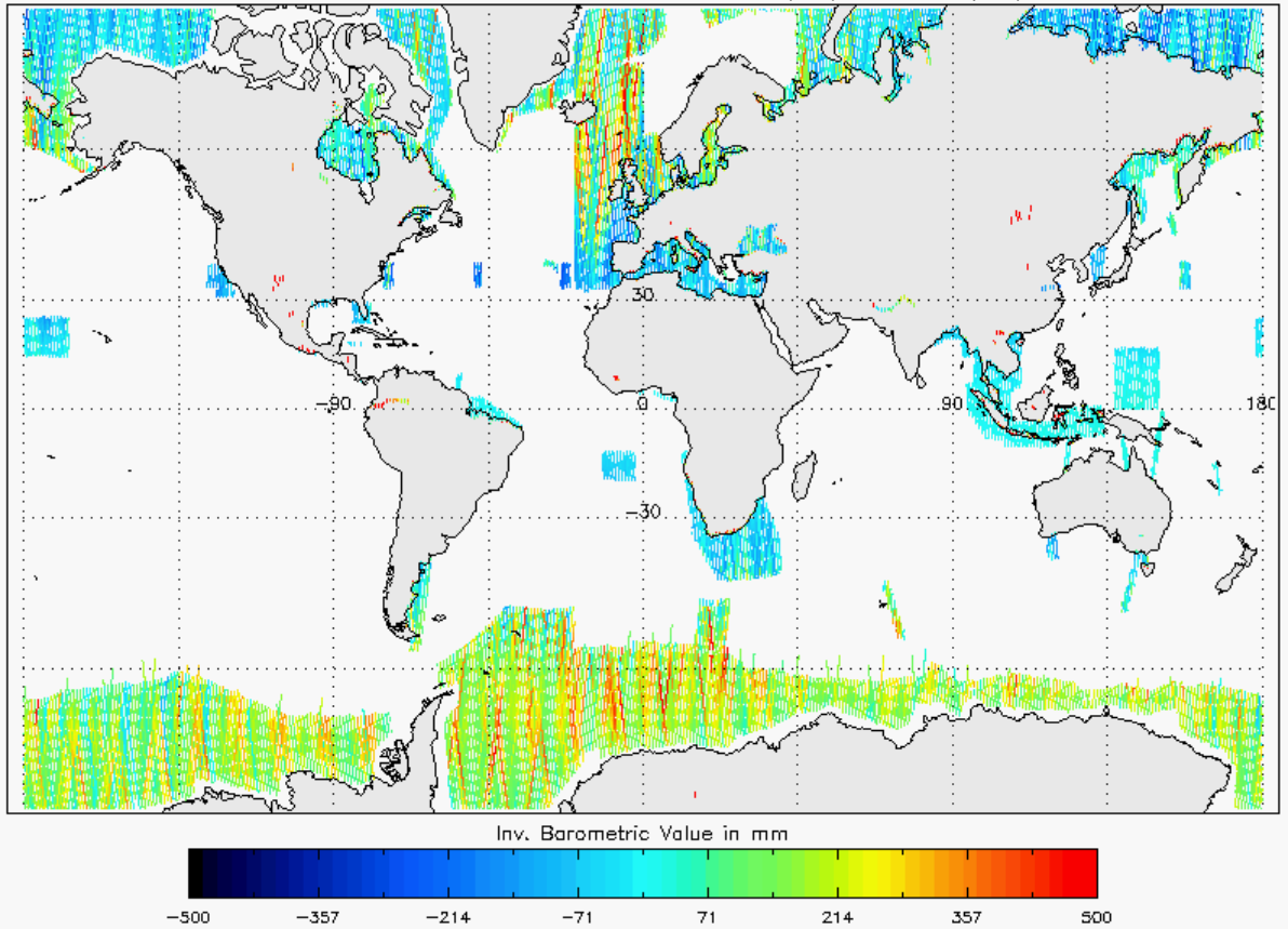
Figure 21 - Global plot of Inverse Barometric Correction for cycle #112
