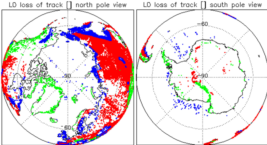
Figure 2 - Polar plots showing areas of loss of track in all SIRAL modes L0 data during December 2019.
