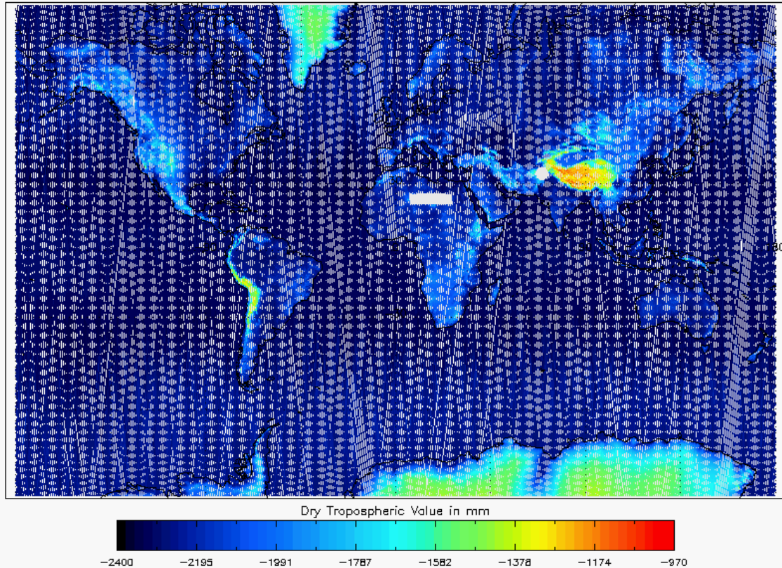
Figure 17 - Global plot of Dry Tropospheric Correction for cycle #112
