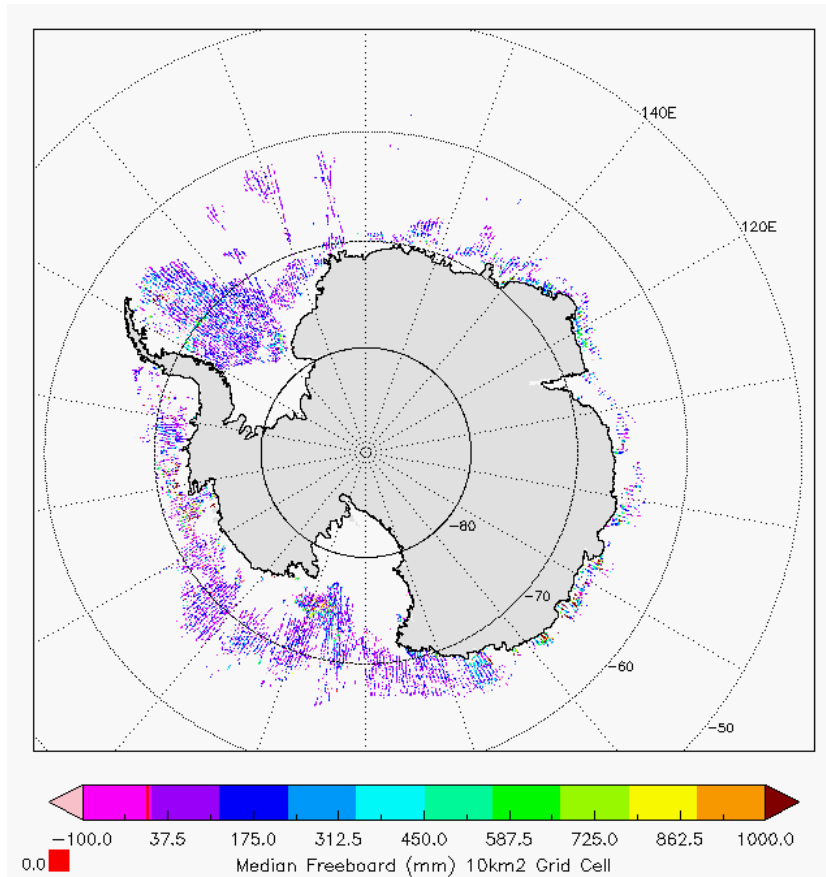
Figure 7 - Polar plots of 10km Gridded Freeboard values from L2 SAR products in cycle #112.
