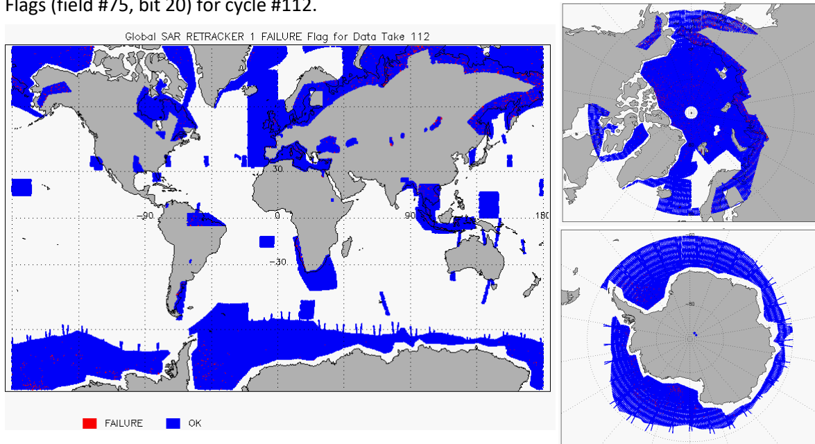
Figure 11 – Global plots showing Retracker Failure Flags for SAR mode for cycle #112
