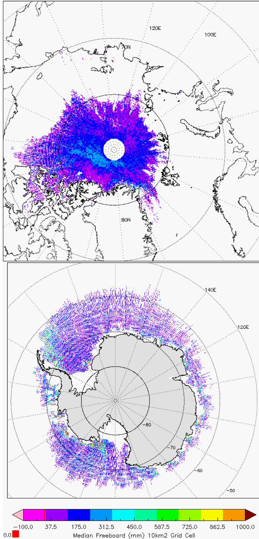
Figure 6 - Polar plots of 10km Gridded Freeboard values from L2 SAR products in cycle #110.
