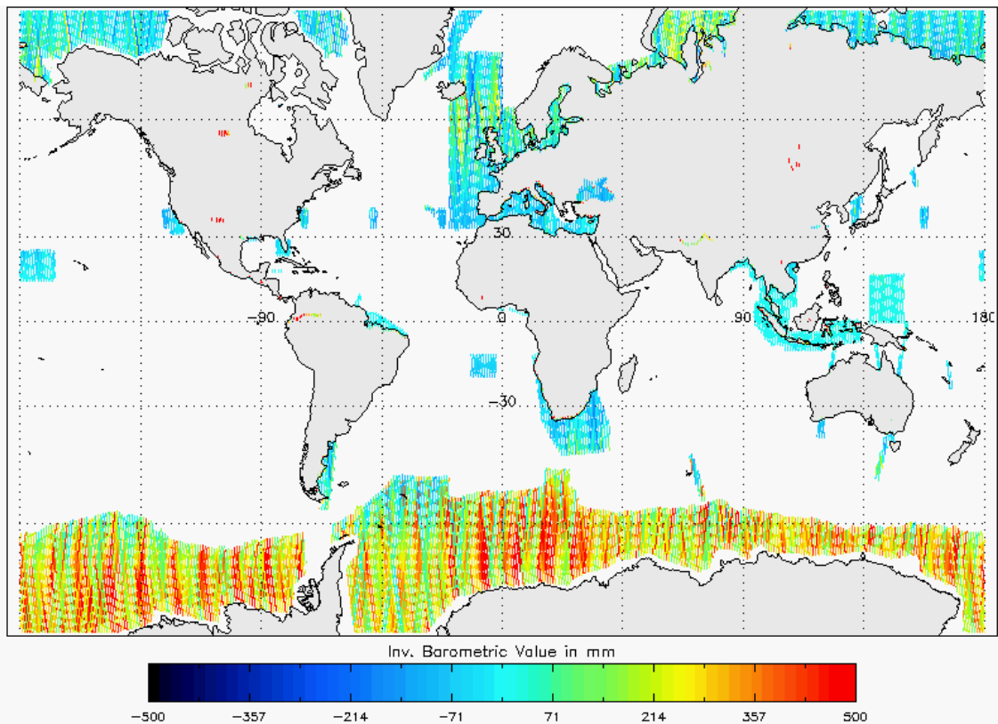
Figure 20 - Global plot of Inverse Barometric Correction for cycle #110
