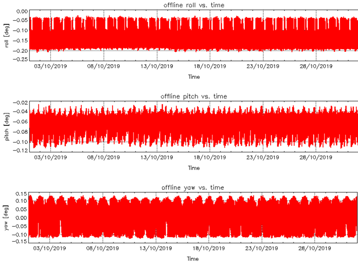
Figure 4 – Roll (top), Pitch (middle) and Yaw (bottom) values for L1B Products during cycle #110.
