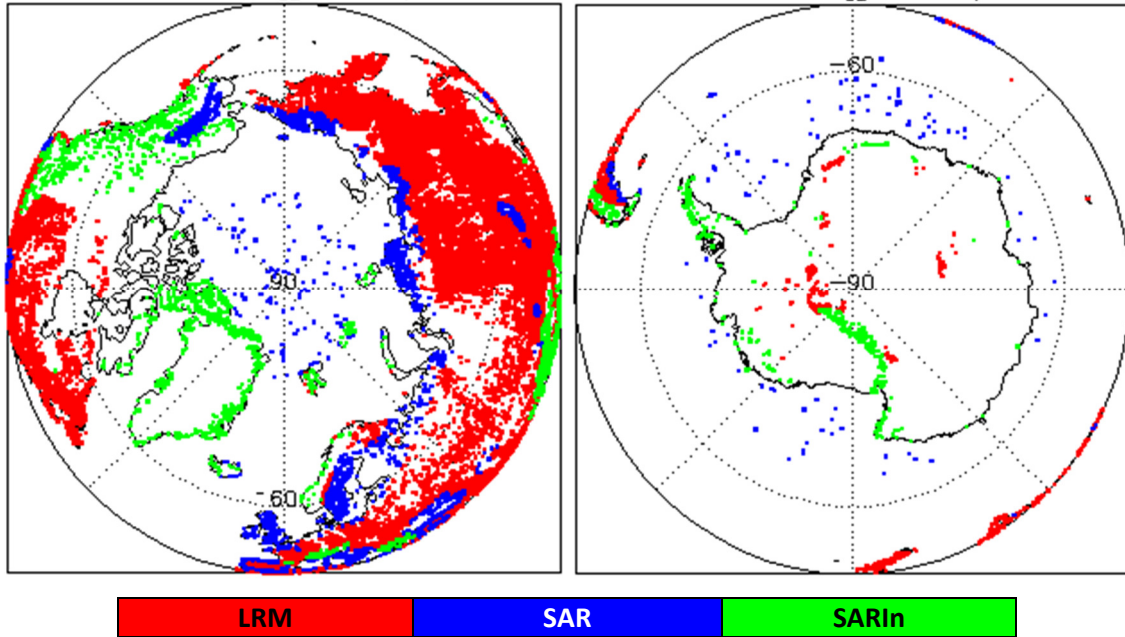
Figure 2 - Polar plots showing areas of loss of track in all SIRAL modes L0 data during October 2019.
