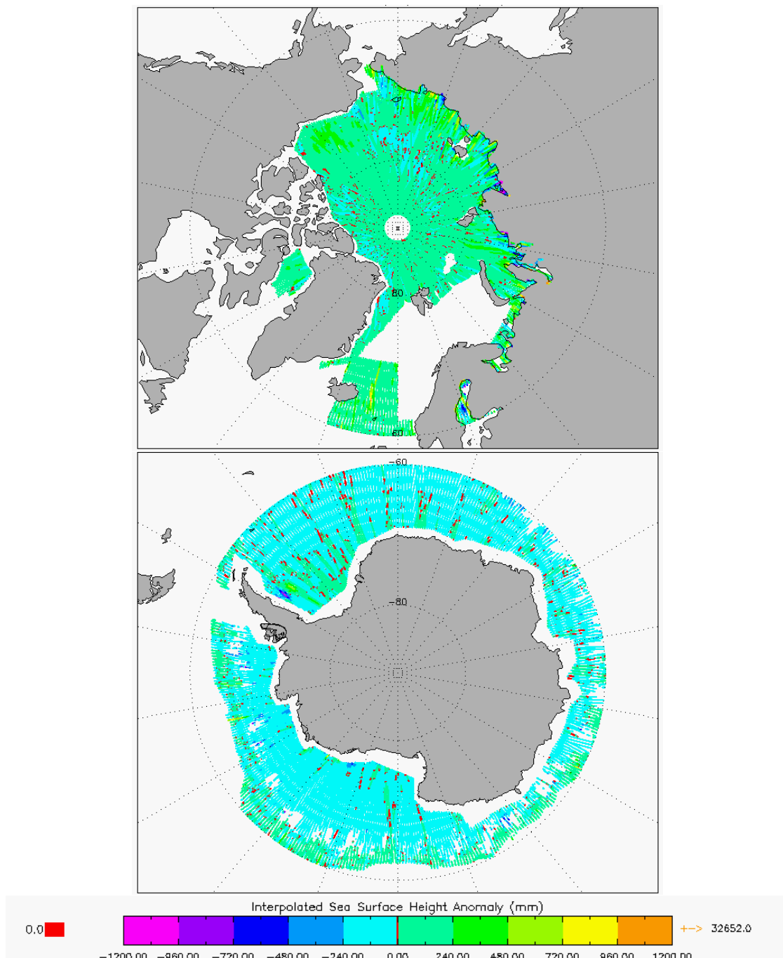
Figure 7 –Polar plots of SSHA for cycle #110.
