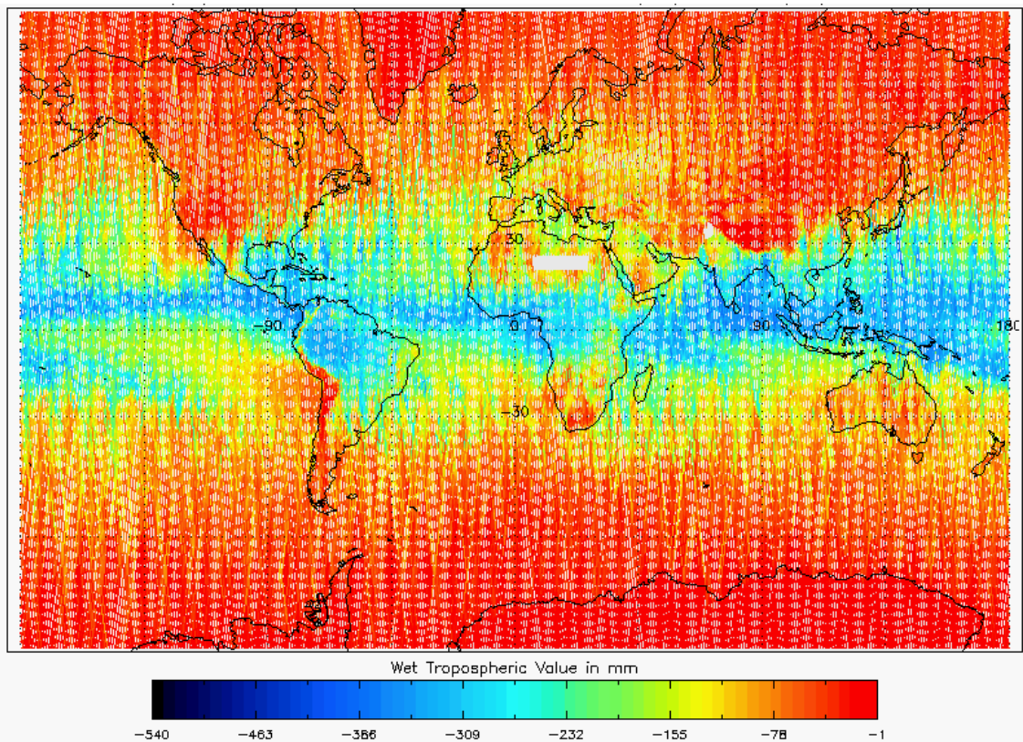
Figure 18 - Global plot of Wet Tropospheric Correction for cycle #110
