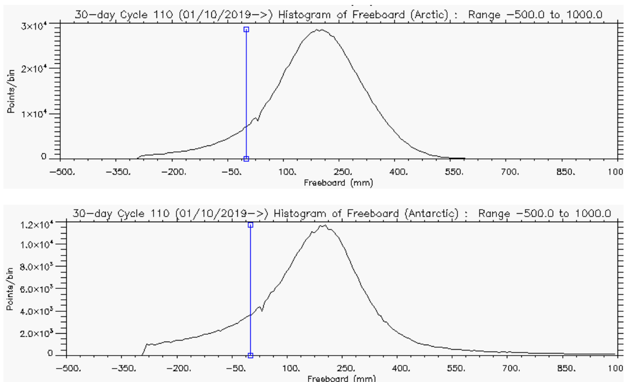
Figure 5 – Histogram of Freeboard for Arctic (above) and Antarctic (below) for cycle #110
