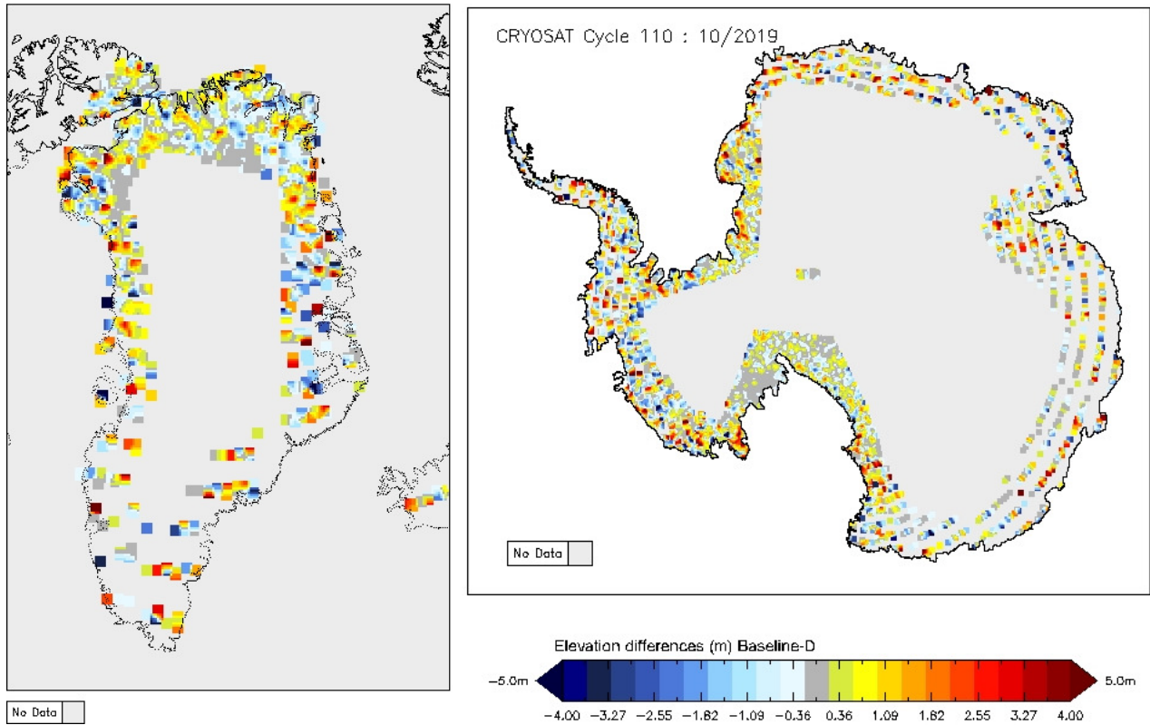
Figure 15 - Greenland and Antarctica maps of SARIn elevation differences for cycle #110
