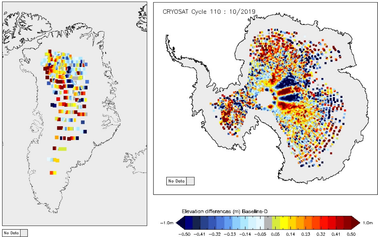
Figure 14 - Greenland and Antarctica maps of LRM elevation differences for cycle #110.
