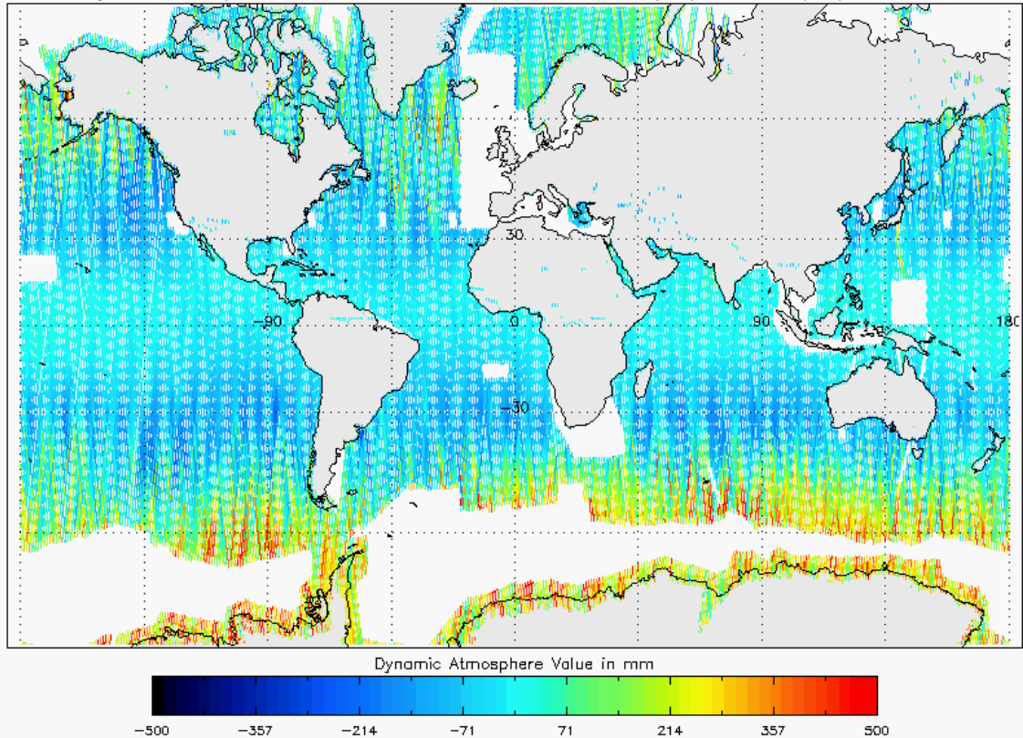
Figure 22 - Global plot of Dynamic Atmospheric Correction for cycle #110
