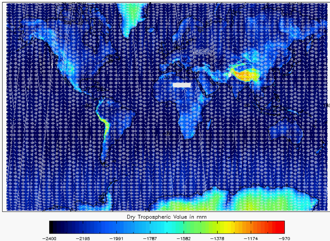
Figure 16 - Global plot of Dry Tropospheric Correction for cycle #110
