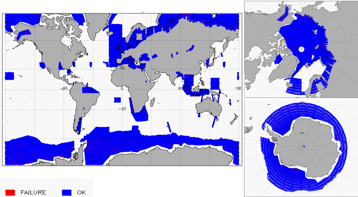
Figure 10 – Global plots showing Retracker Failure Flags for SAR mode for cycle #110
