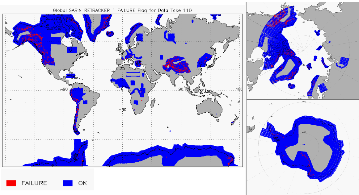
Figure 11 – Global plots showing Retracker Failure Flags for SARIn mode for cycle #110
