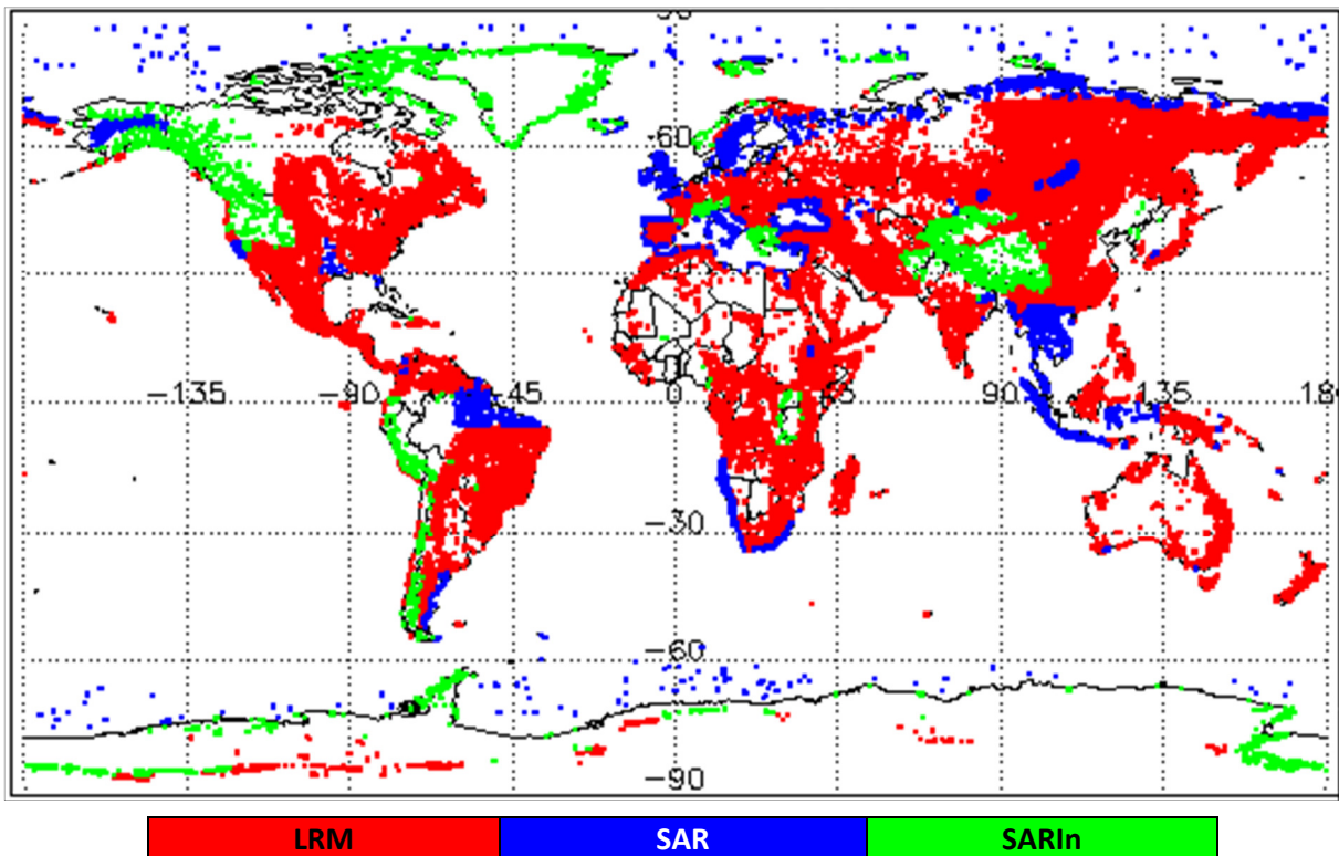
Figure 1 - Global plot showing areas of loss of track in all SIRAL modes L0 data during October 2019.
