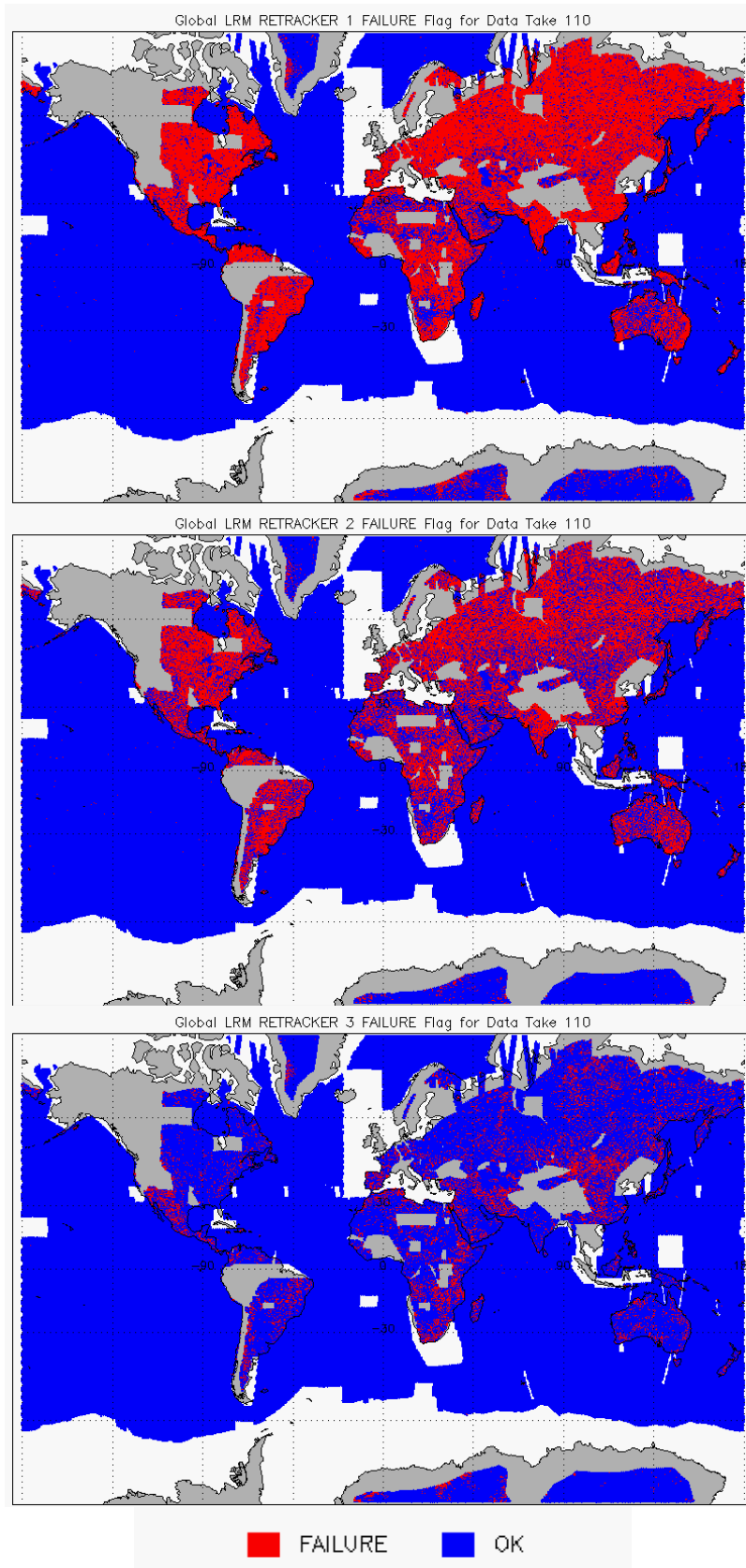
Figure 9 – Global plots showing Retracker Failure Flags for LRM mode for cycle #110:
