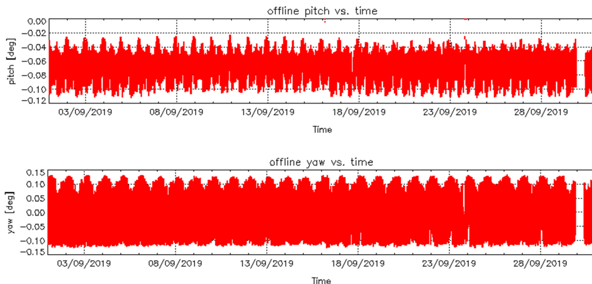
Figure 4 – Roll (top), Pitch (middle) and Yaw (bottom) values for L1B Products during cycle #109.
