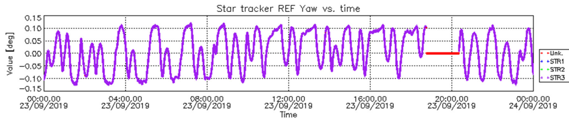
Figure 5 – Pitch values extracted from Star Tracker for 23/09/2019
